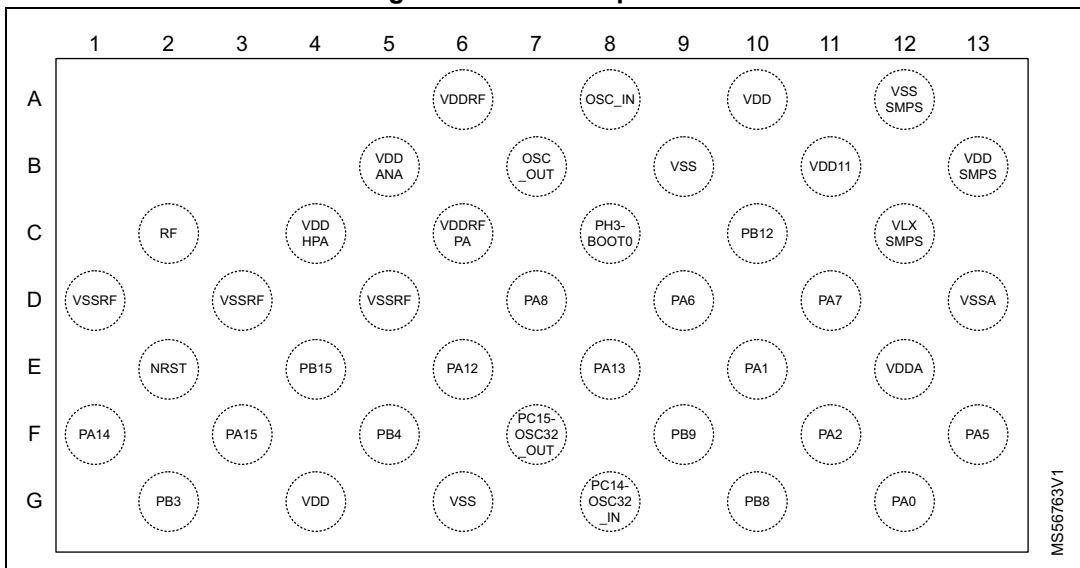
Figure 8. WLCSFP41 pinout (1)
