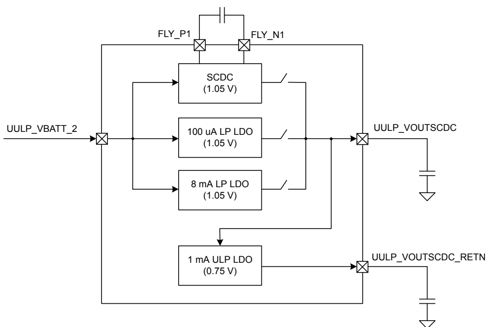
Figure 7.3. Block Diagram
