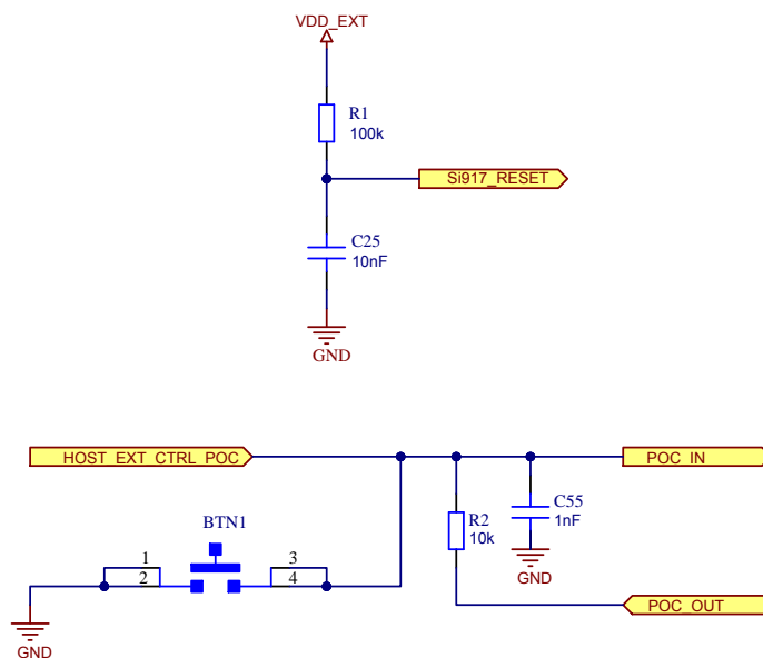
Figure 8.8. Reset Configuration
