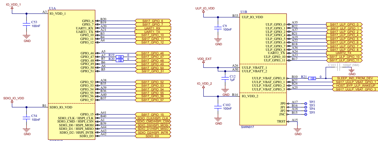
Figure 8.3. GPIO Supply Domains
