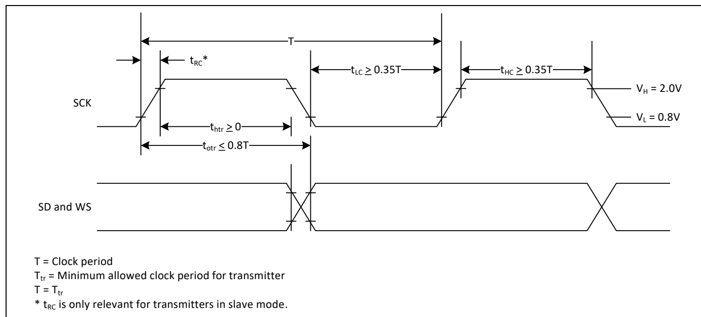
Figure 14. I 2 S Transmitter Timing
