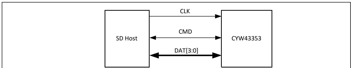
Figure 17. Signal Connections to SDIO Host (SD 4-Bit Mode)
