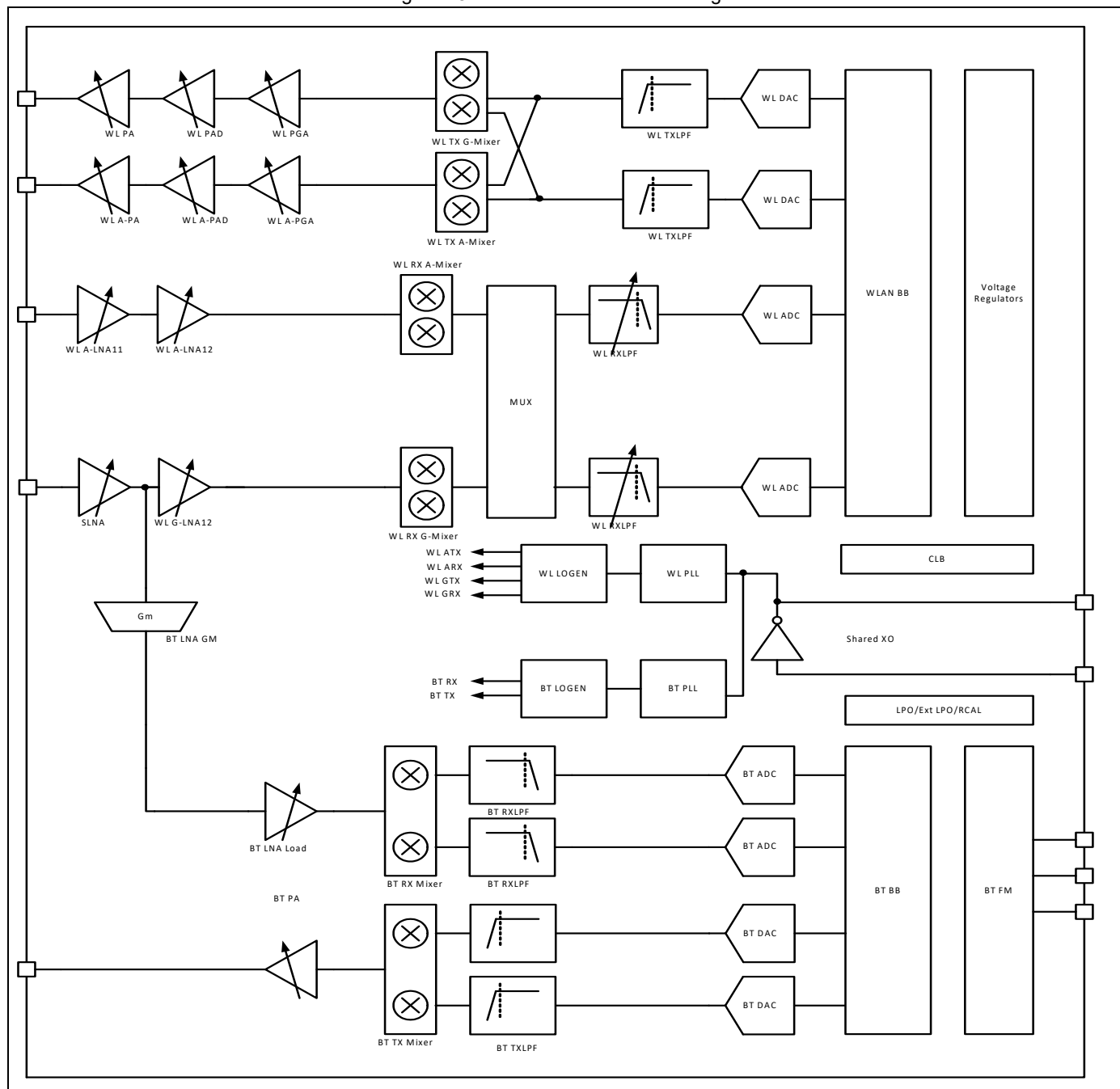
Figure 28. Radio Functional Block Diagram
