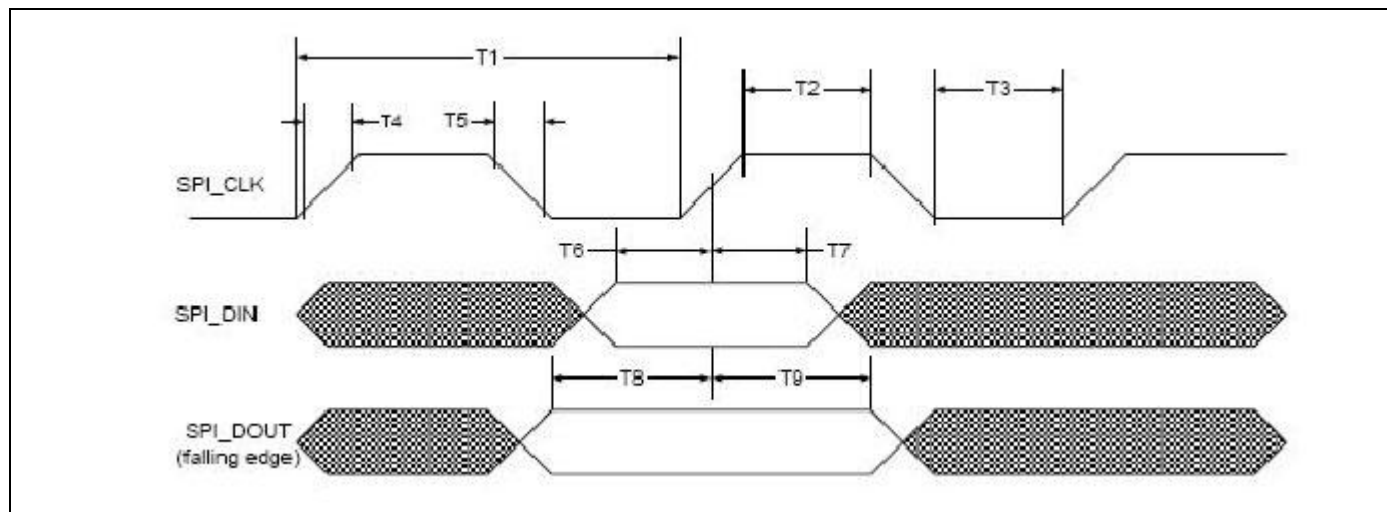
Figure 41. gSPI Timing
