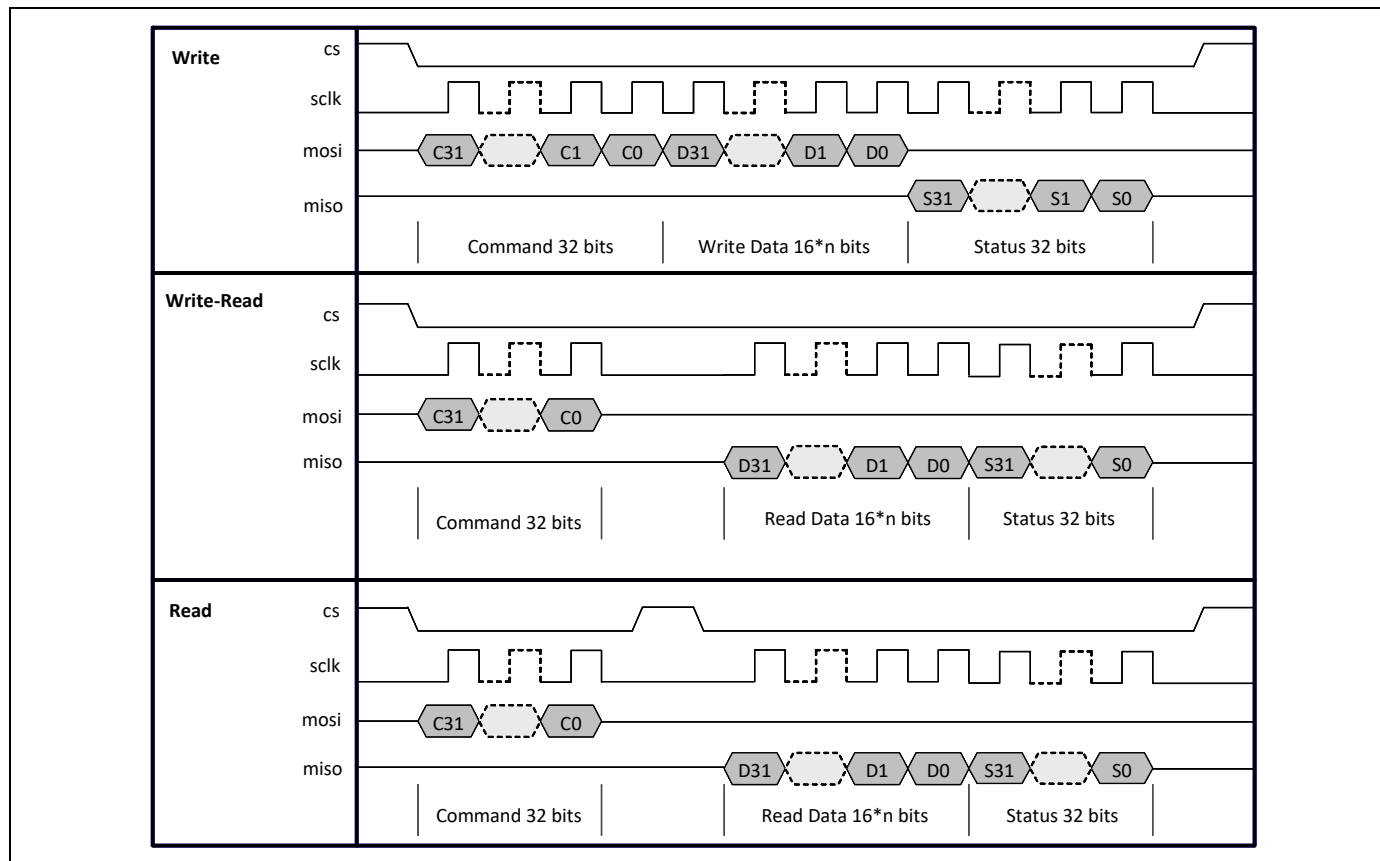
Figure 24. gSPI Signal Timing with Status (Response Delay = 0; 32-bit Big Endian)
