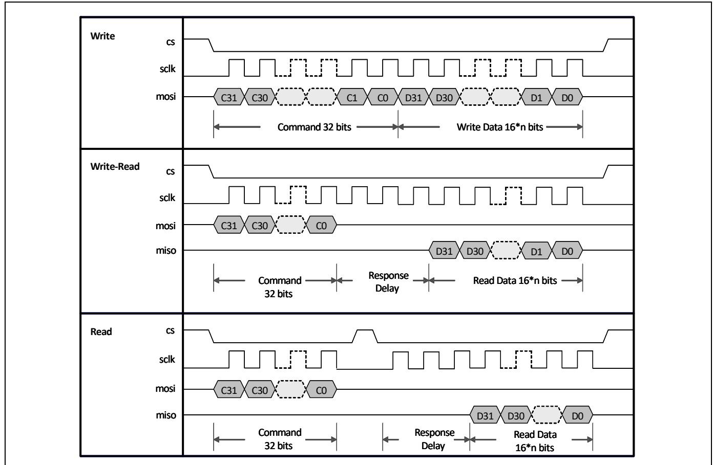
Figure 23. gSPI Signal Timing Without Status (32-bit Big Endian)
