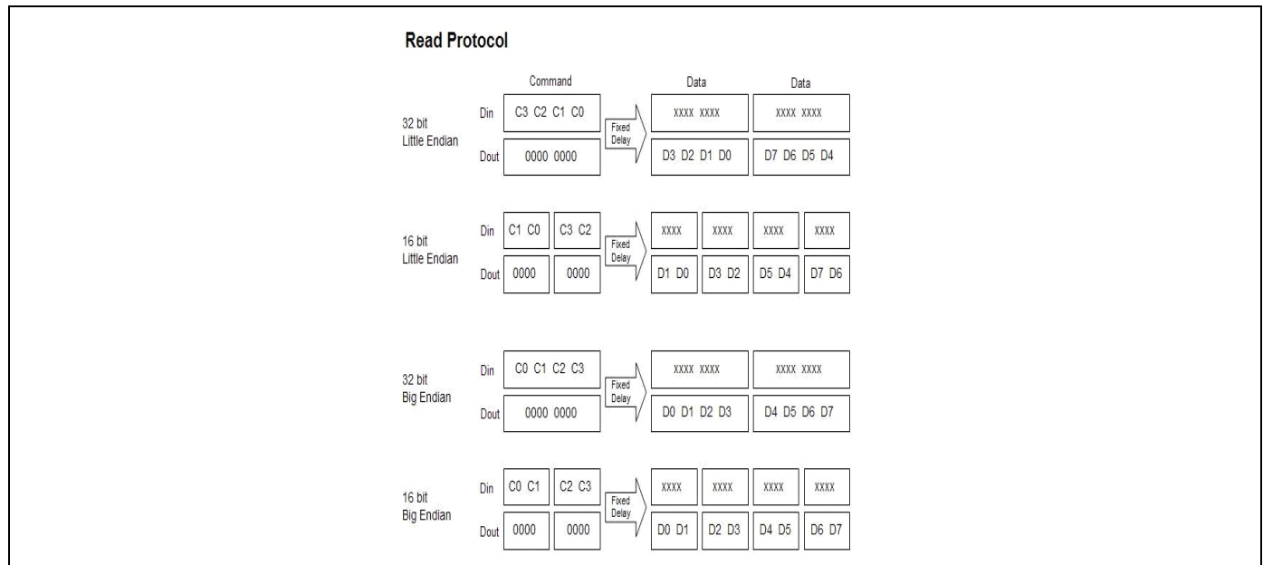
Figure 21. gSPI Read Protocol
