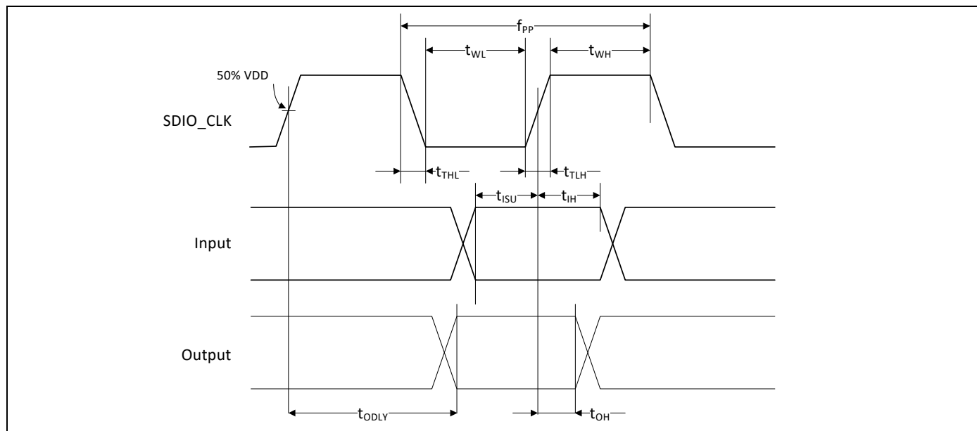
Figure 33. SDIO Bus Timing (High-Speed Mode)
