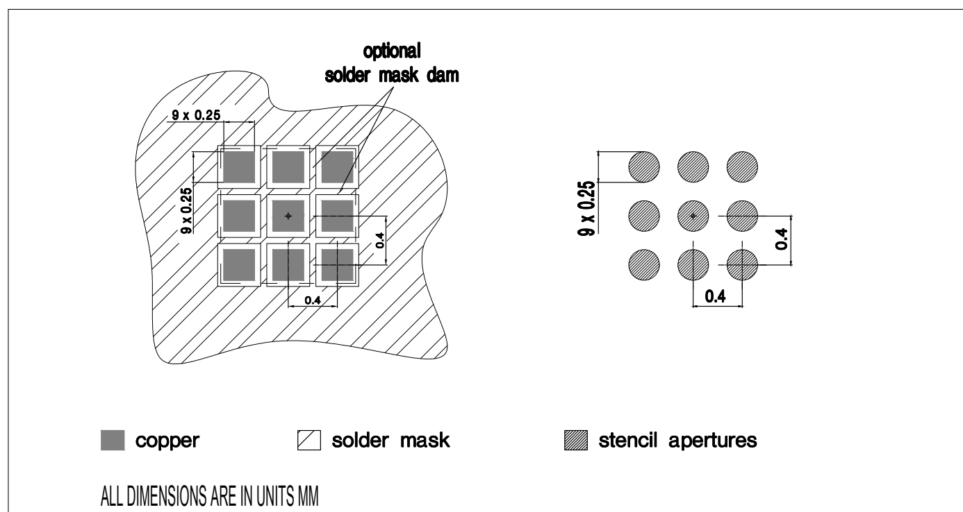
Figure 5: Footprint Recommendation
