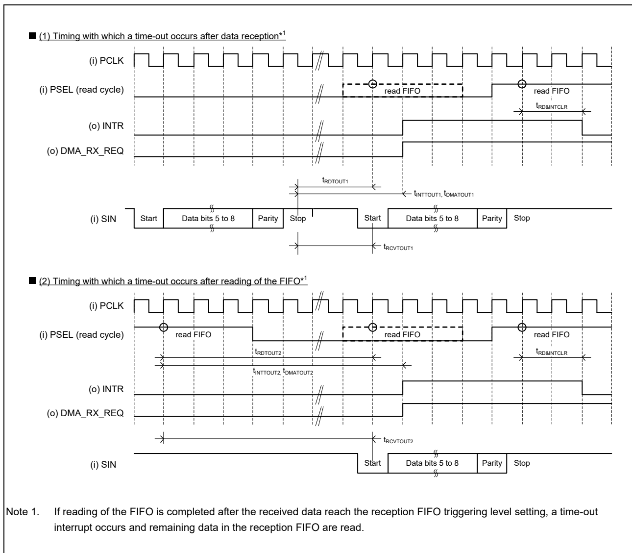
Figure 31.4-8 Time-out Timing
