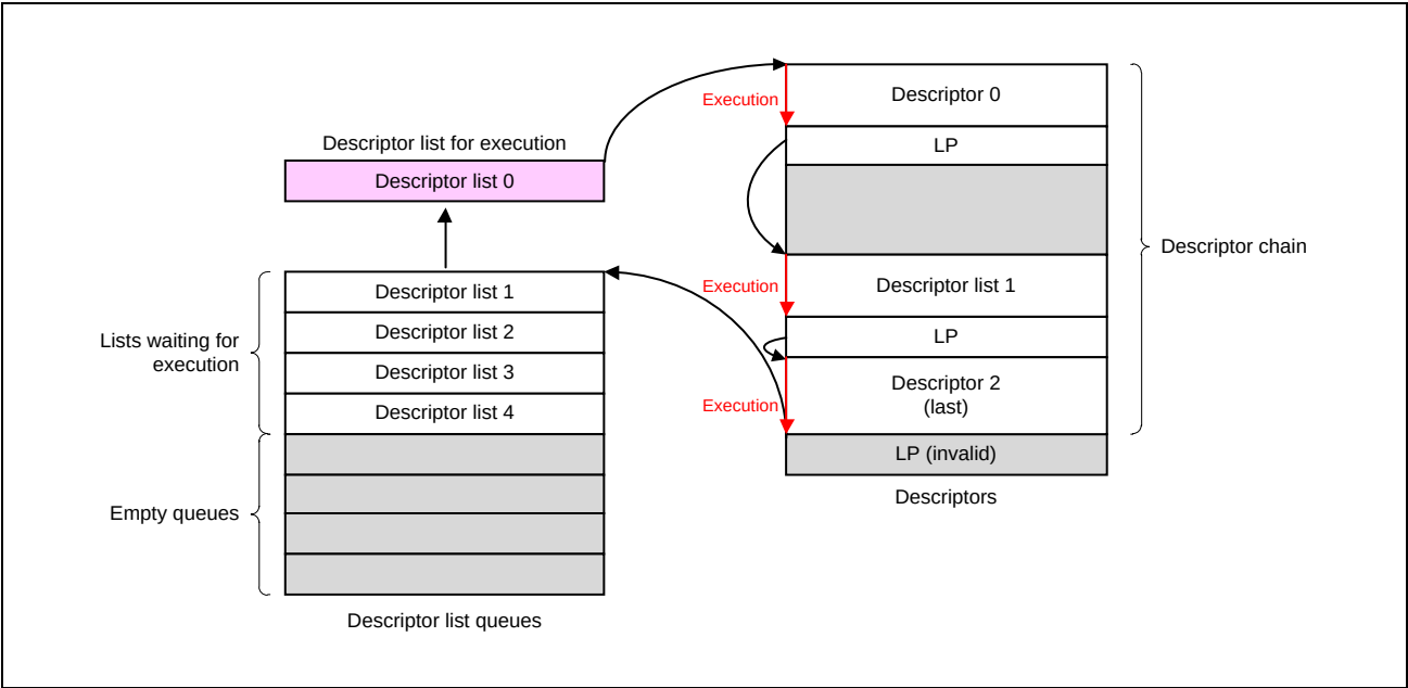
Figure 27.7-1 Descriptor Chain
