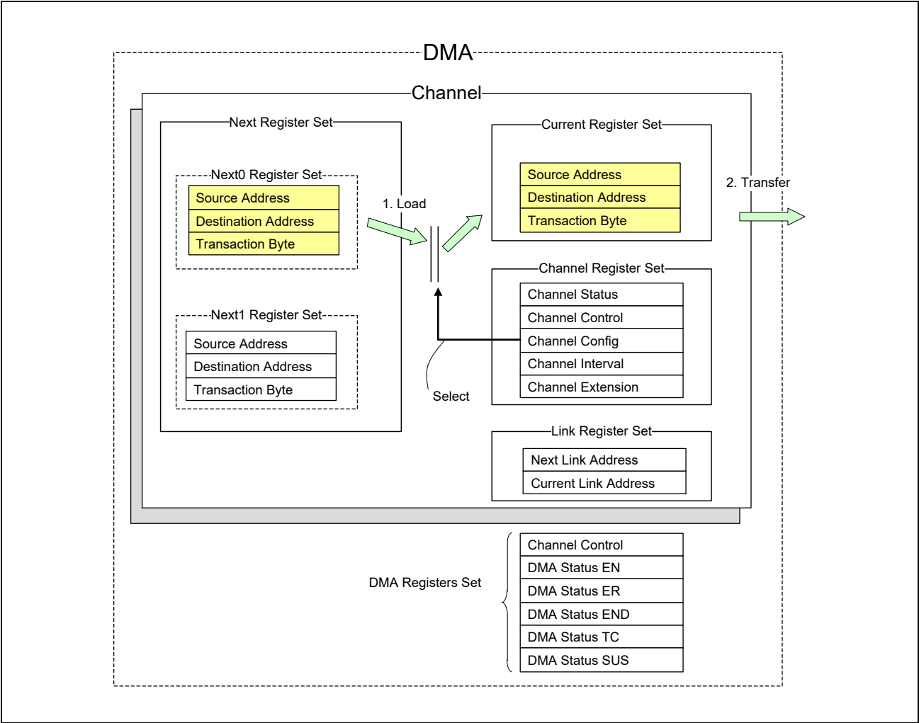
Figure 18.5-1 Register Configuration
