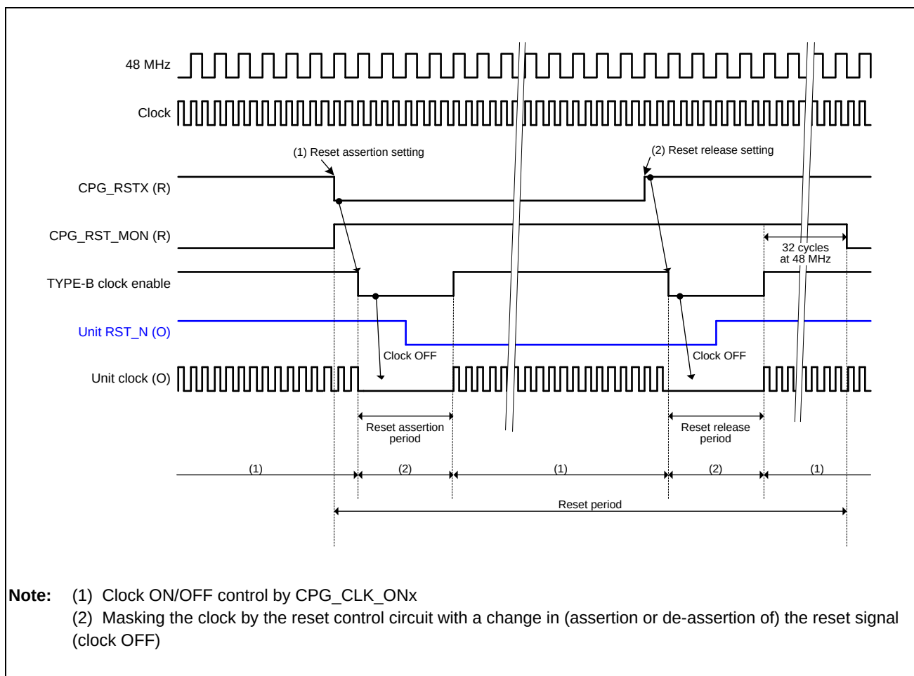
Figure 34.6-31 TYPE-B Reset Timing by the CPG Register
