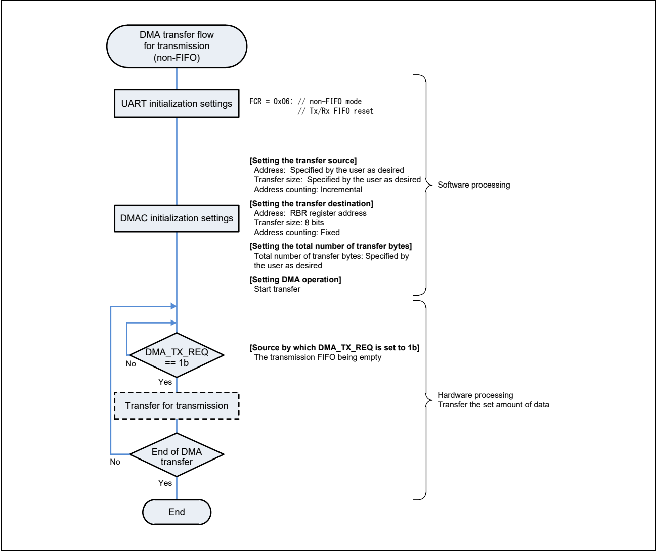
Figure 31.5-5 DMA Transfer Flow for Transmission (in (4) Non-FIFO Mode)
