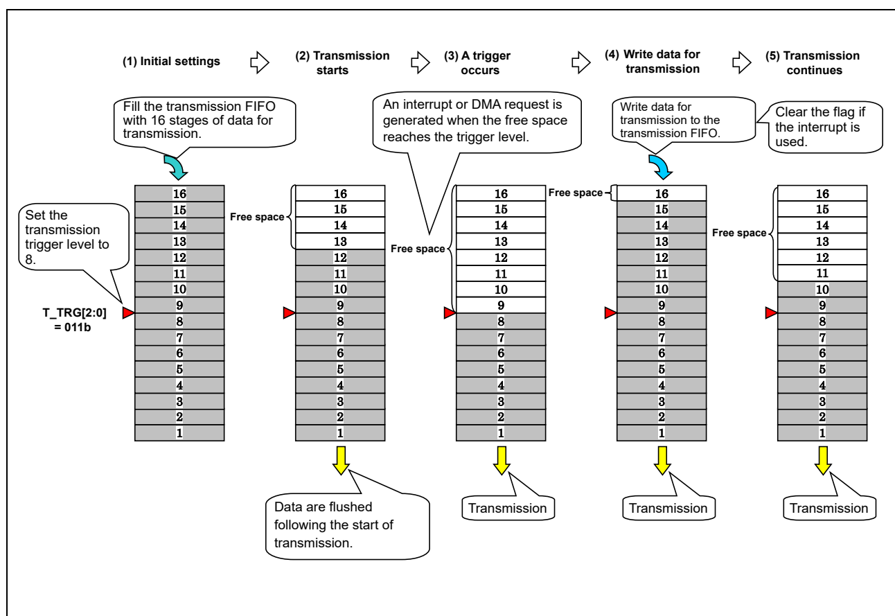
Figure 30.4-18 Operation of the Transmission FIFO when the Transmission Trigger Level is Set
