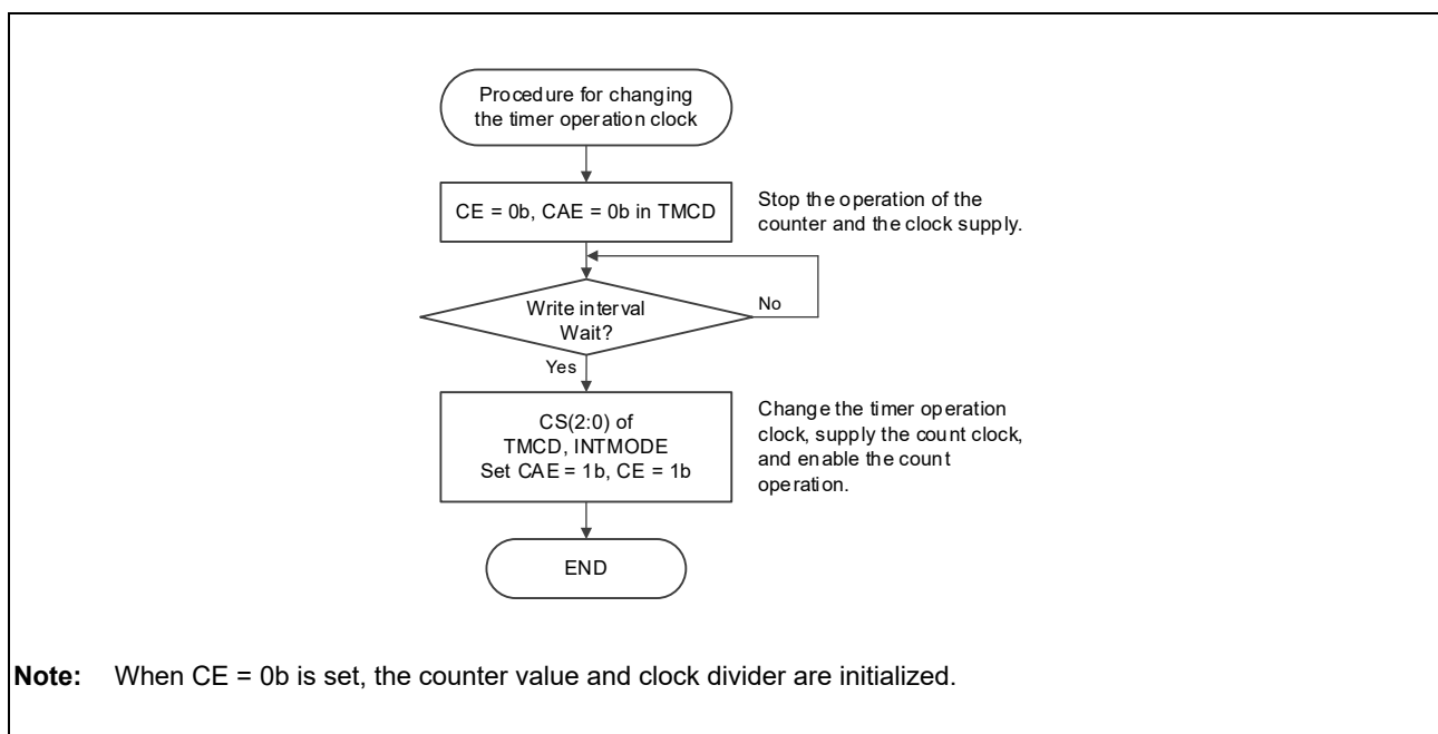
Figure 16.4-6 Procedure for Changing the Timer Operation Clock (Counter Operation and Clock Supply Stop)
