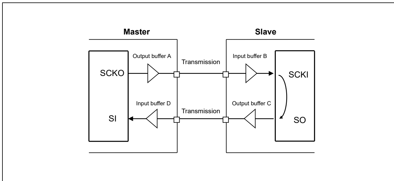
Figure 30.6-1 Master and Slave Connection
