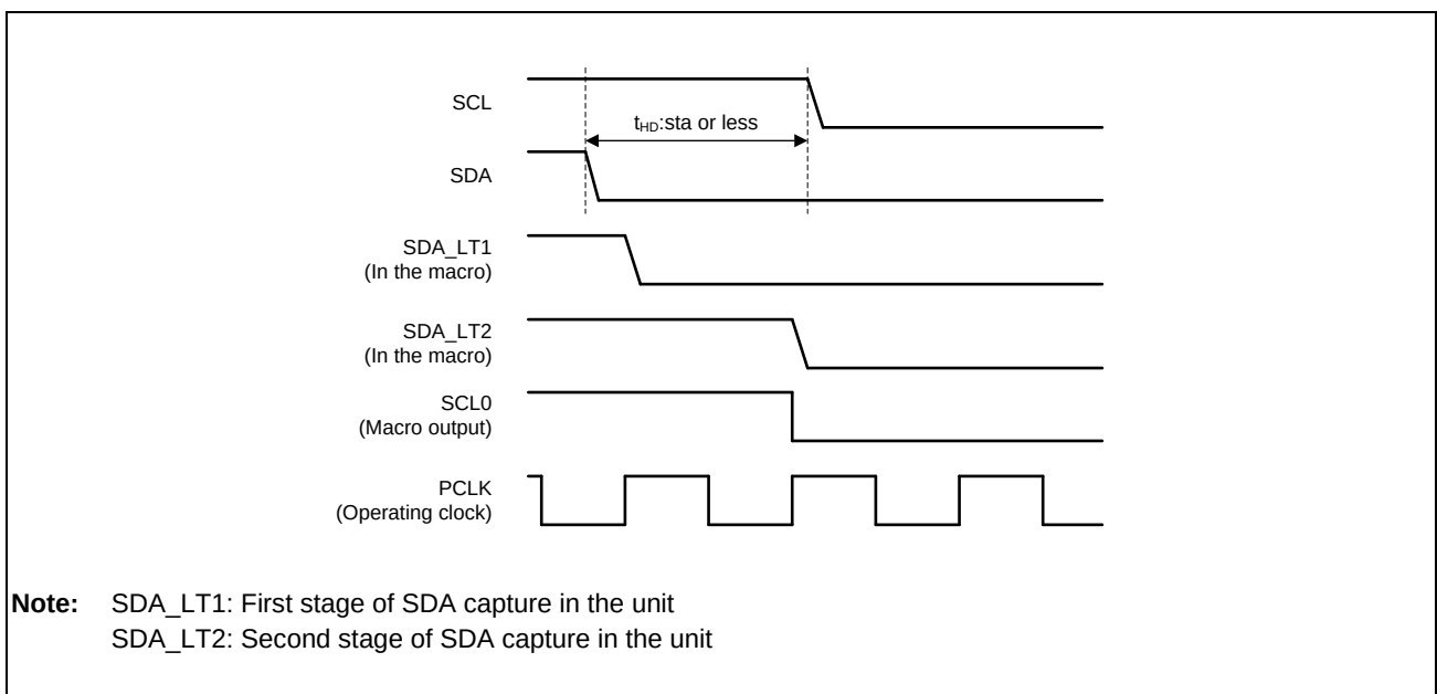
Figure 29.9-2 Timing Example where Start Condition Hold Time is Not Satisfied
