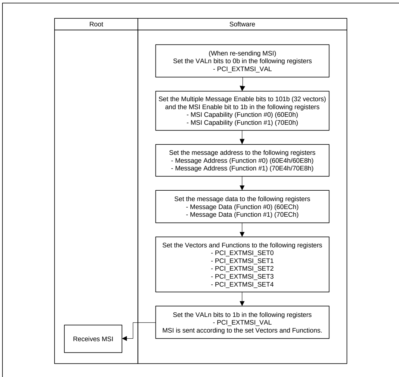
Figure 27.7-4 MSI Issuing Flow
