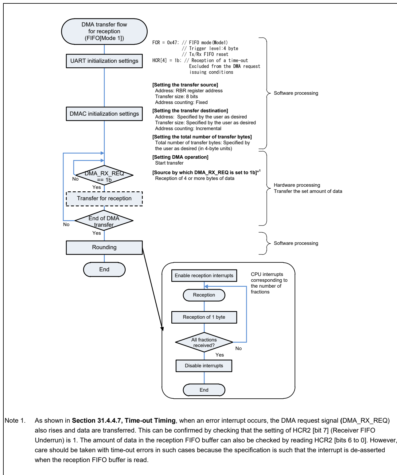
Figure 31.5-4 DMA Transfer Flow for Reception (a Time-out in Mode 1 when the FIFO Buffer is in Use is Excluded from the DMA Request Issuing Conditions)
