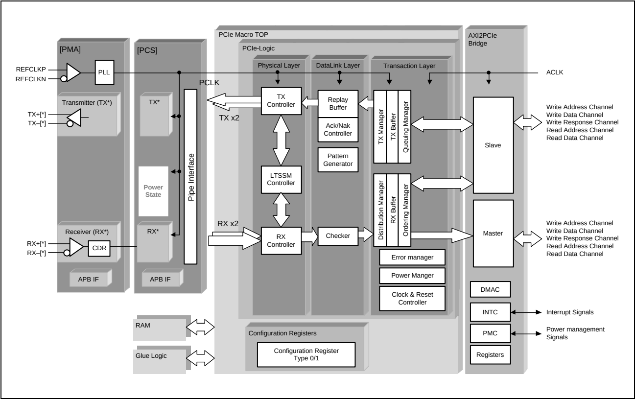
Figure 27.3-1 Block Diagram
