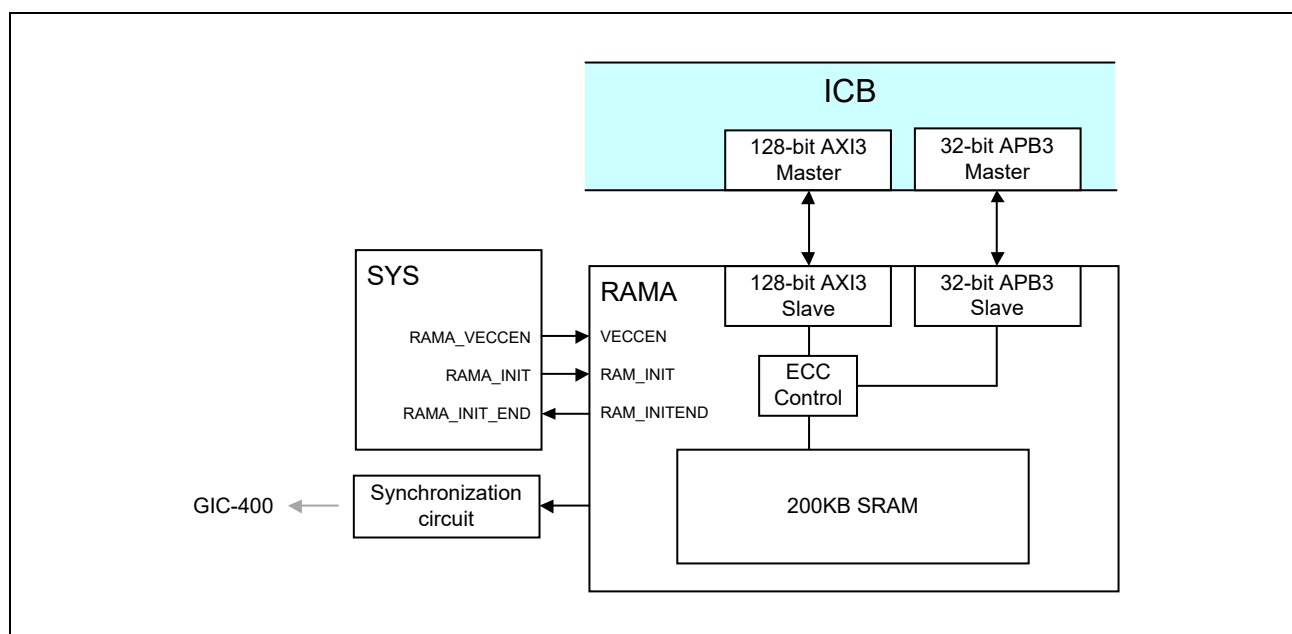
Figure 12.1-1 Connection Diagram
