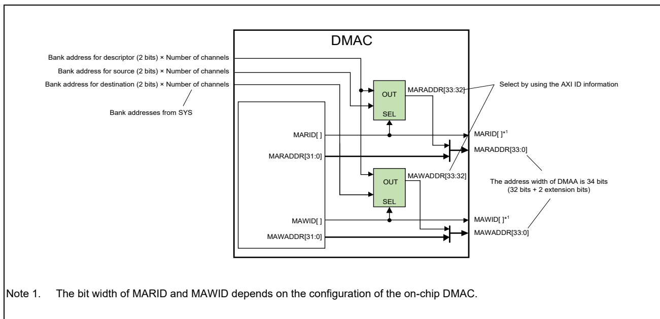
Figure 6.3-2 Schematic of Address Bus Width Extension (Address Extension 2)
