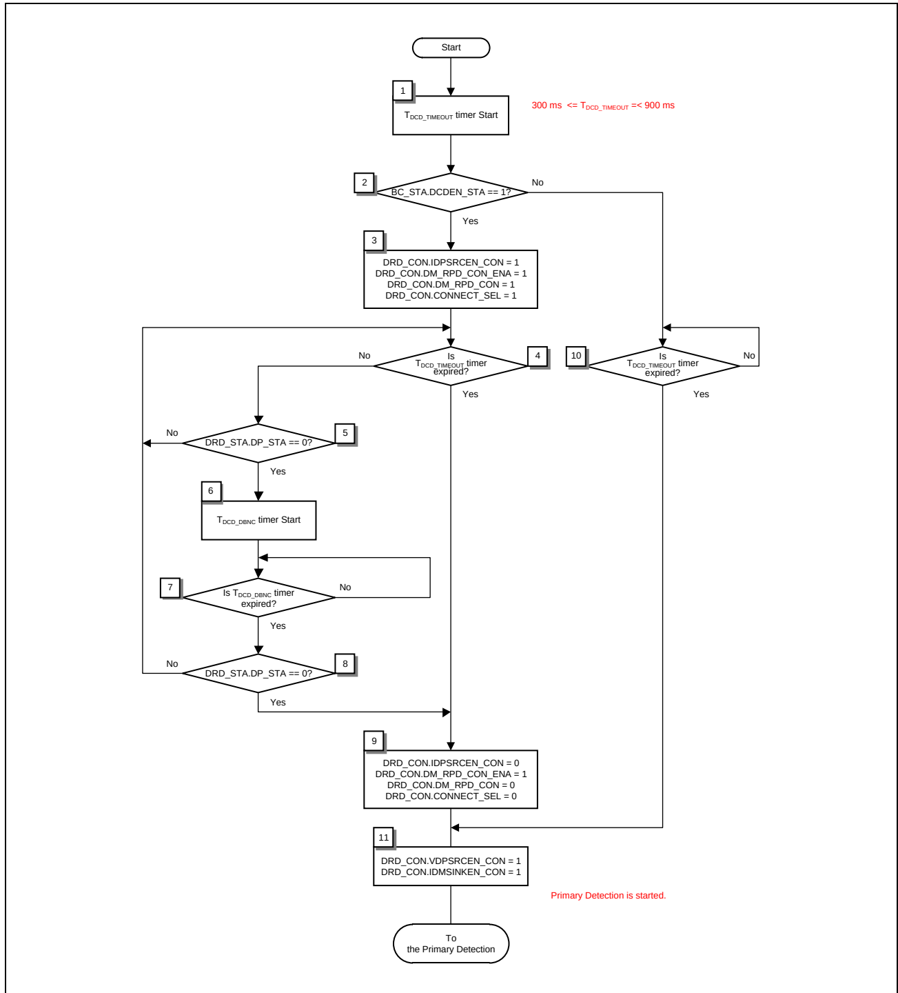
Figure 26.4-7 Good Battery Algorithm Flowchart (DCD Flow)
