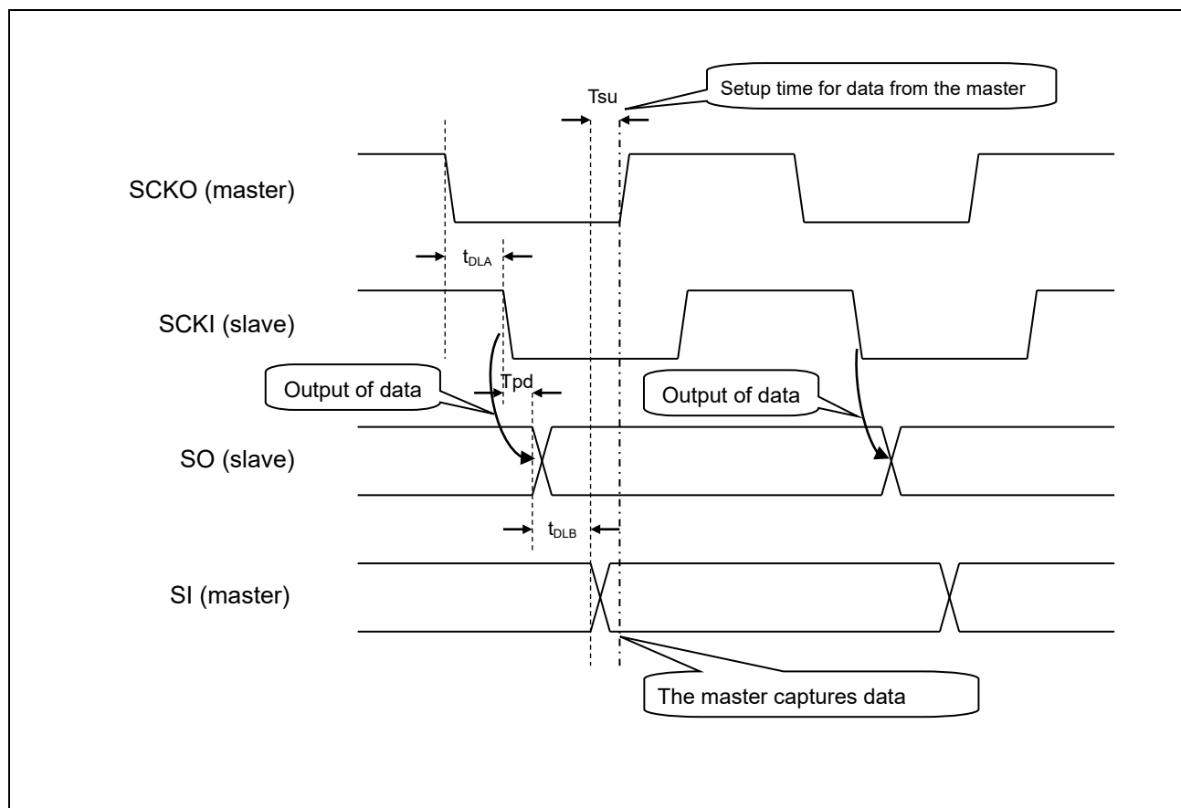
Figure 30.6-2 Timing of Data Reception by the Master
