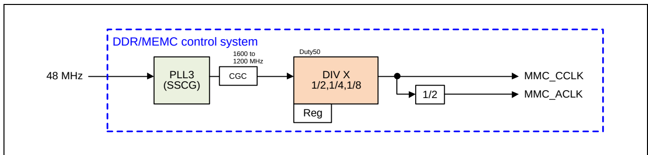
Figure 34.6-21 Block Diagram of the LPDDR4 Control System (PLL3 Peripheral)
