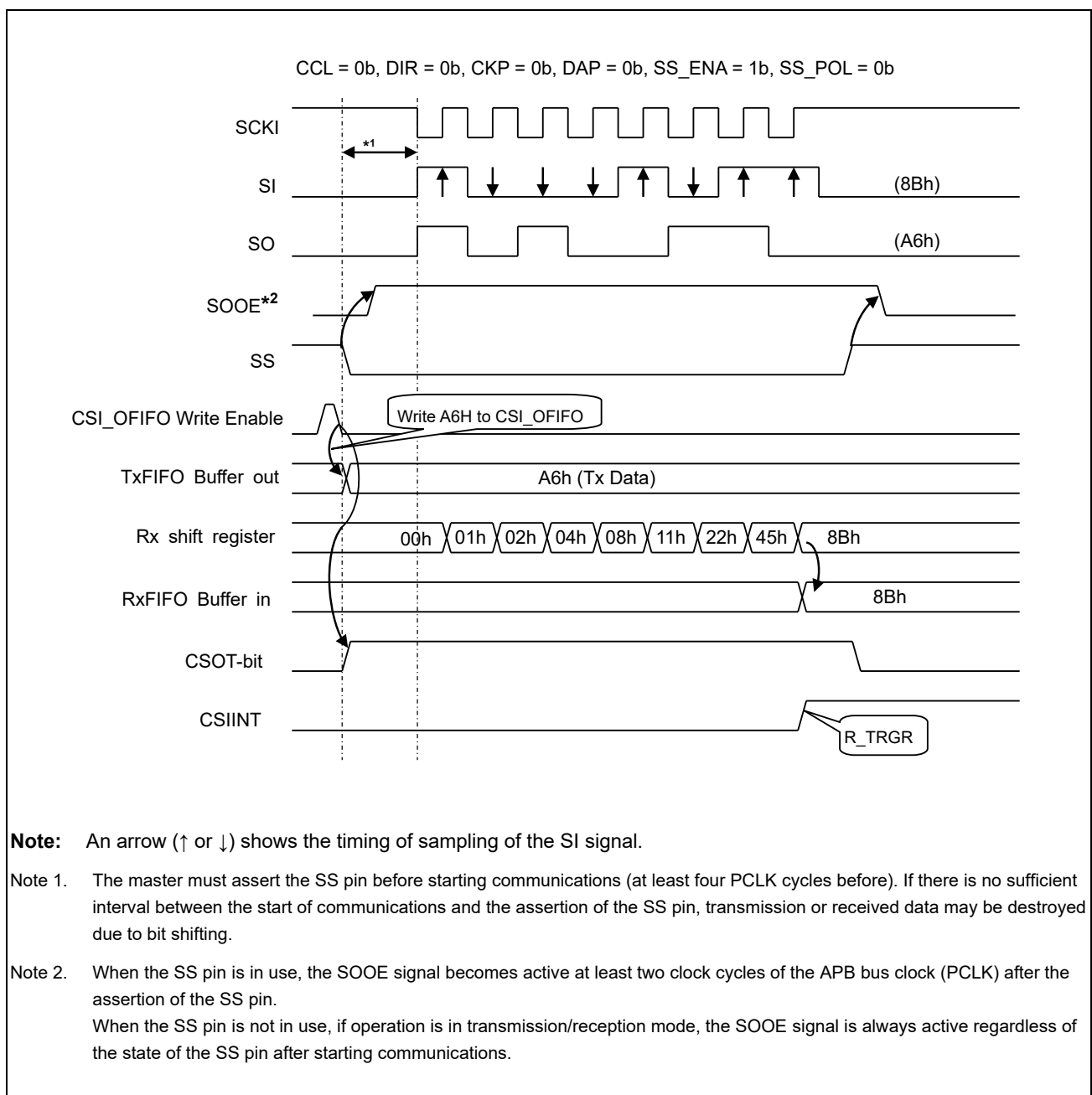
Figure30.5-3 Timing of Single-Word Transfer (in Slave Transmission/Reception Mode)
