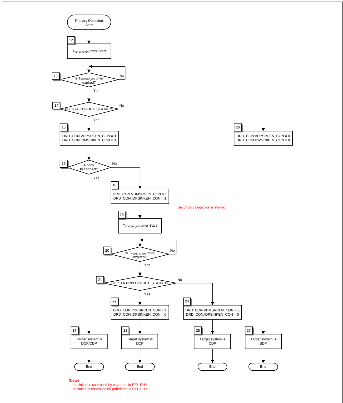
Figure 26.4-8 Good Battery Algorithm Flowchart (Primary &amp; Secondary Detection Flow)
