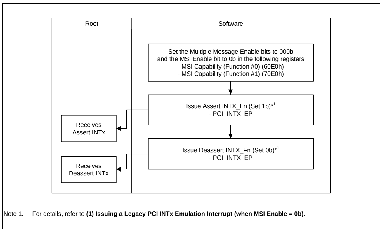
Figure 27.7-3 Legacy Interrupt Issuing Flow
