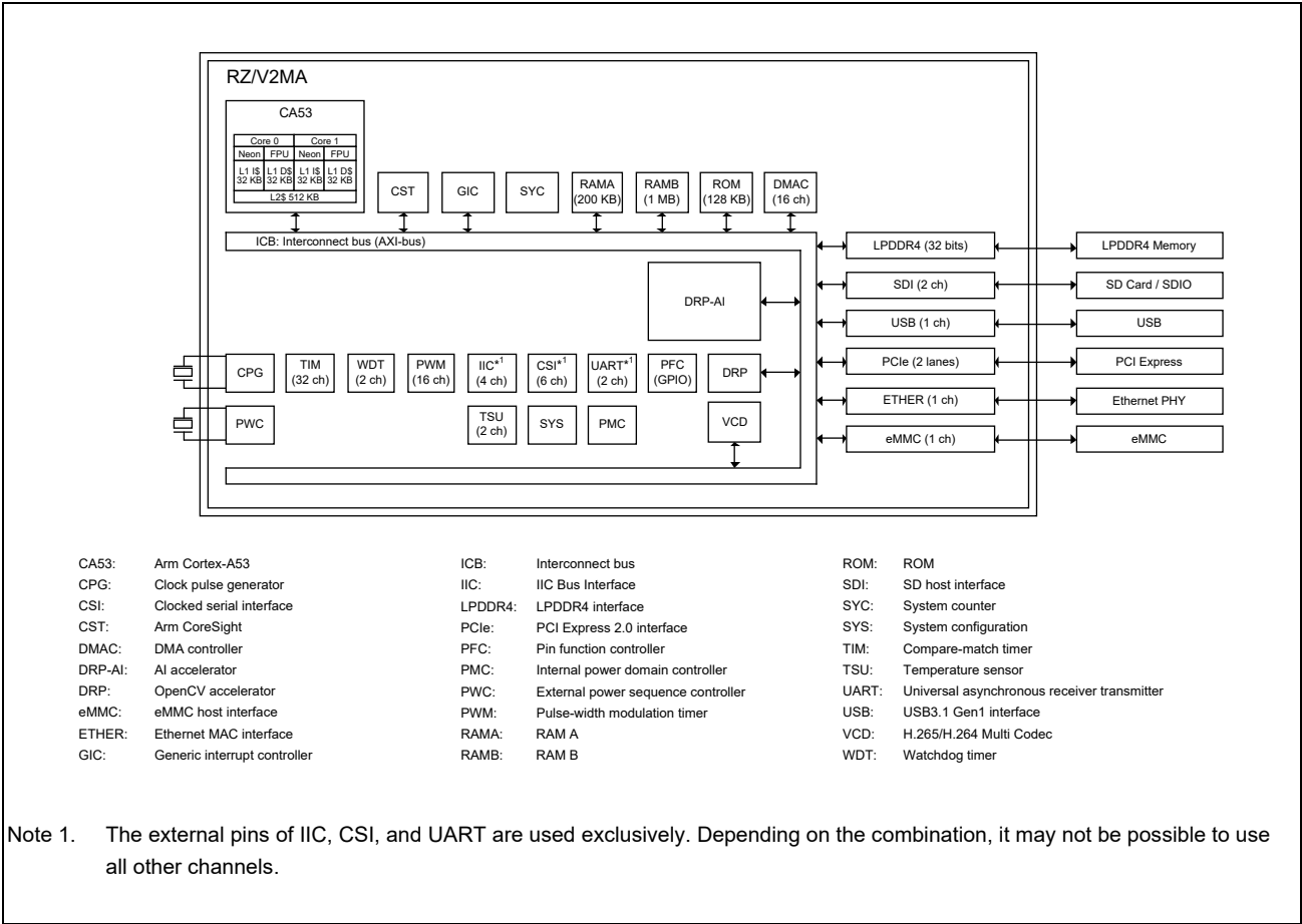
Figure 1.4-1 Block Diagram
