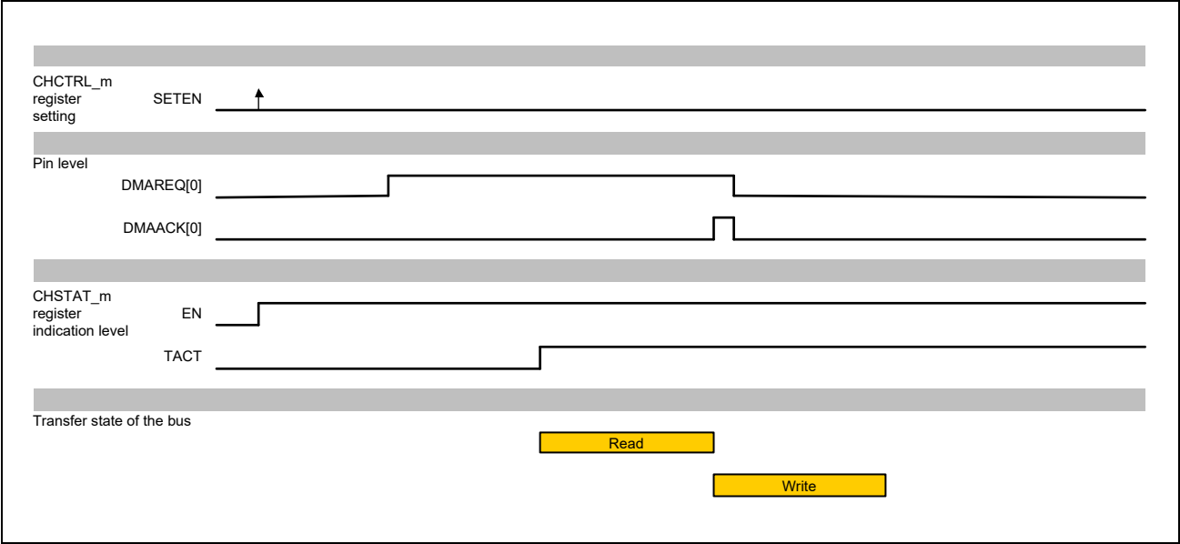
Figure 18.6-26 DMAC State Example 1 (Hardware Request)
