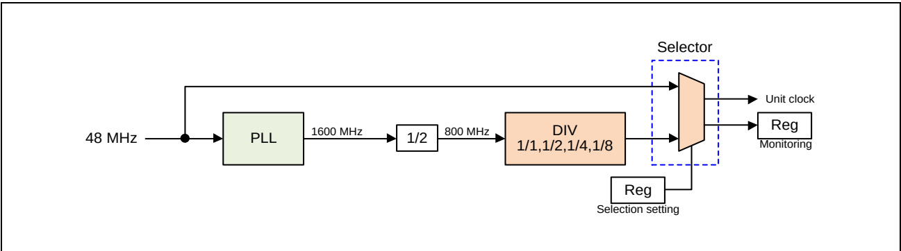
Figure 34.6-13 Schematic View of the Allocation of the Dynamic Switching Selector
