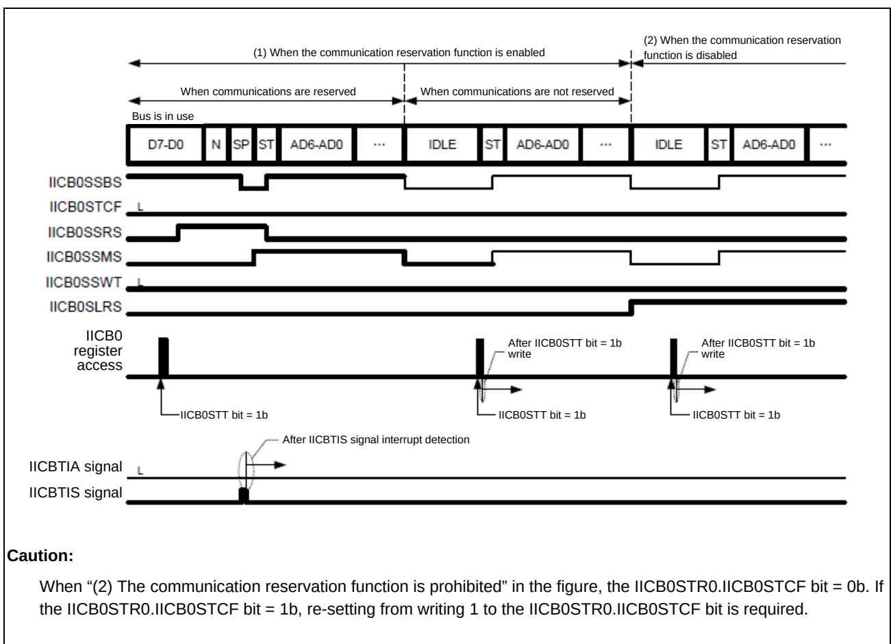
Figure 29.6-16 Timing of Effective Writing to the IICB0DAT Register
