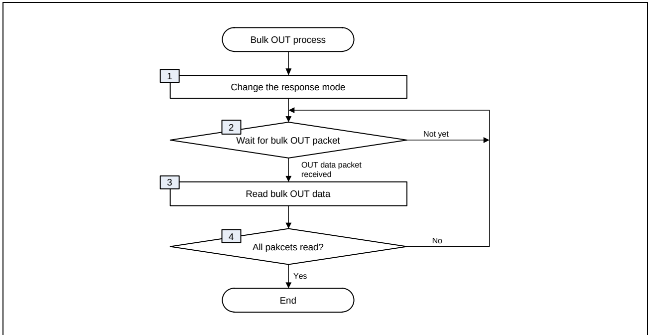
Figure 26.6-31 Bulk OUT Process Flow
