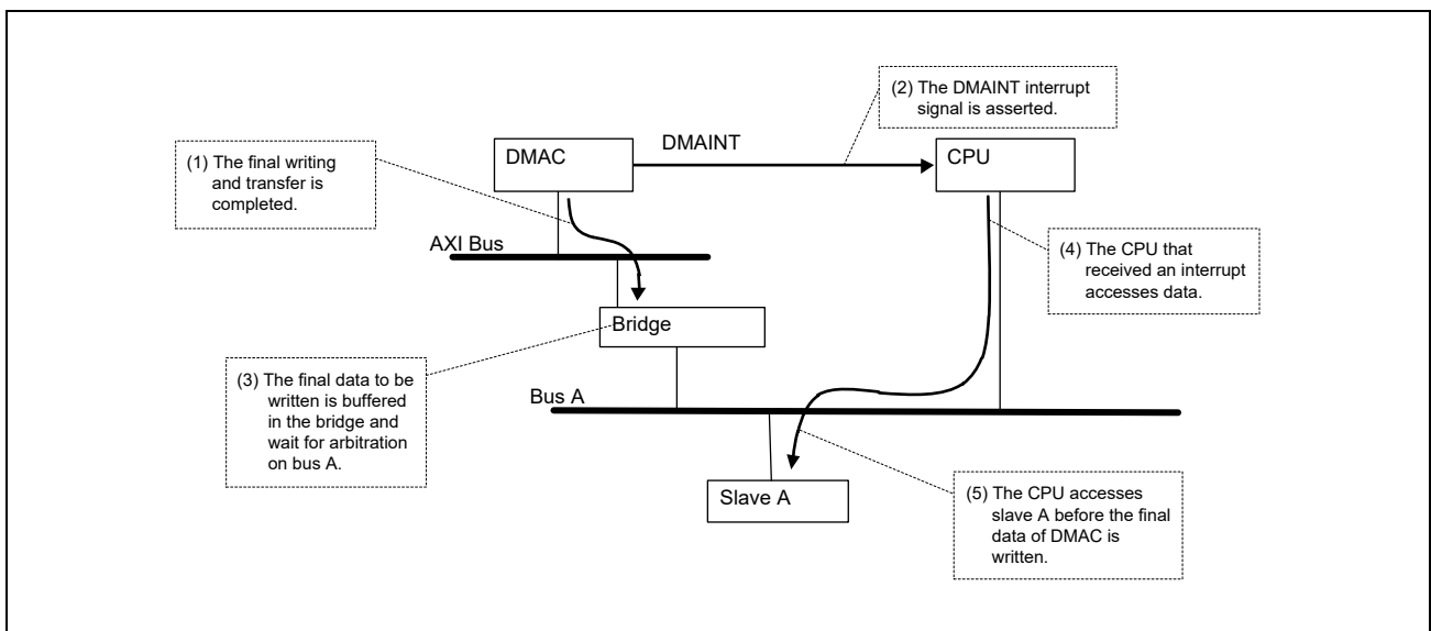
Figure 18.8-1 Example when Access by the CPU Overtakes Writing of the Final Data by the DMAC
