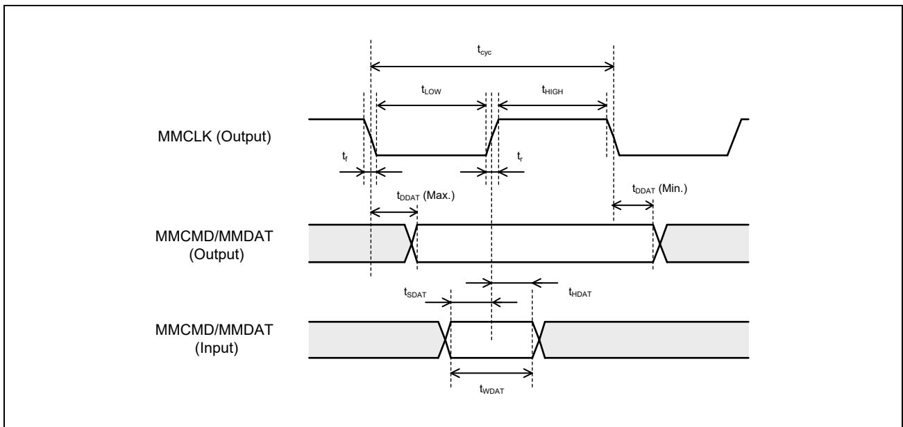
Figure 40.5-10 eMMC Timing
