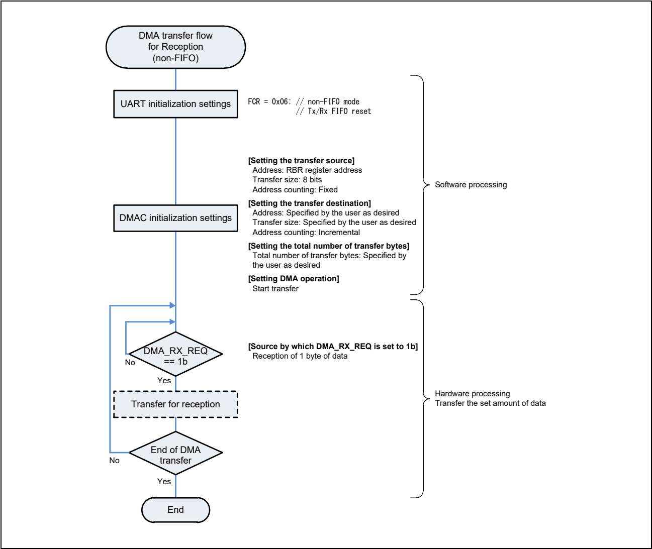
Figure 31.5-1 DMA Transfer Flow for Reception (in (1) Non-FIFO Mode)
