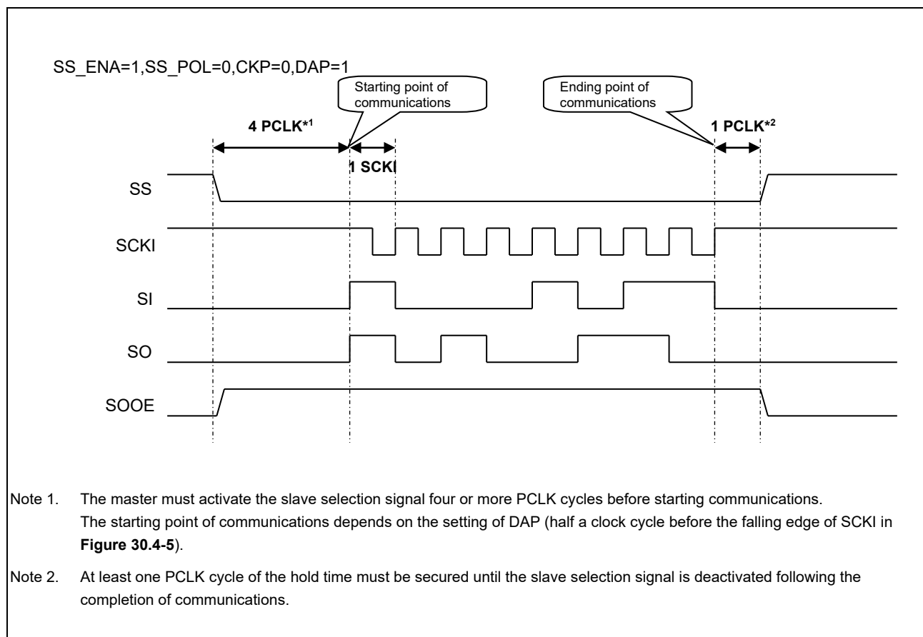
Figure 30.4-5 Slave Selection Signal Control Timing (when DAP = 1b for Slave)
