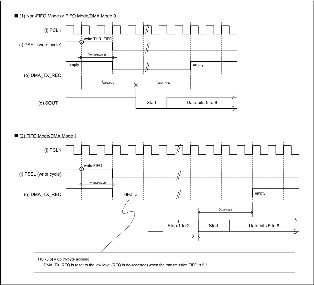
Figure 31.4-9 DMA Request Timing for Transmission
