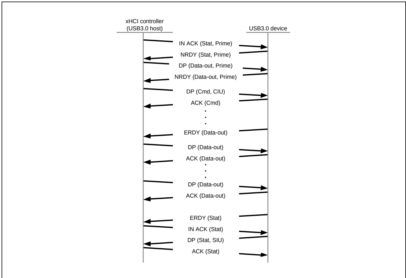
Figure 26.6-36 Example SuperSpeed UASP Data-OUT Transfer
