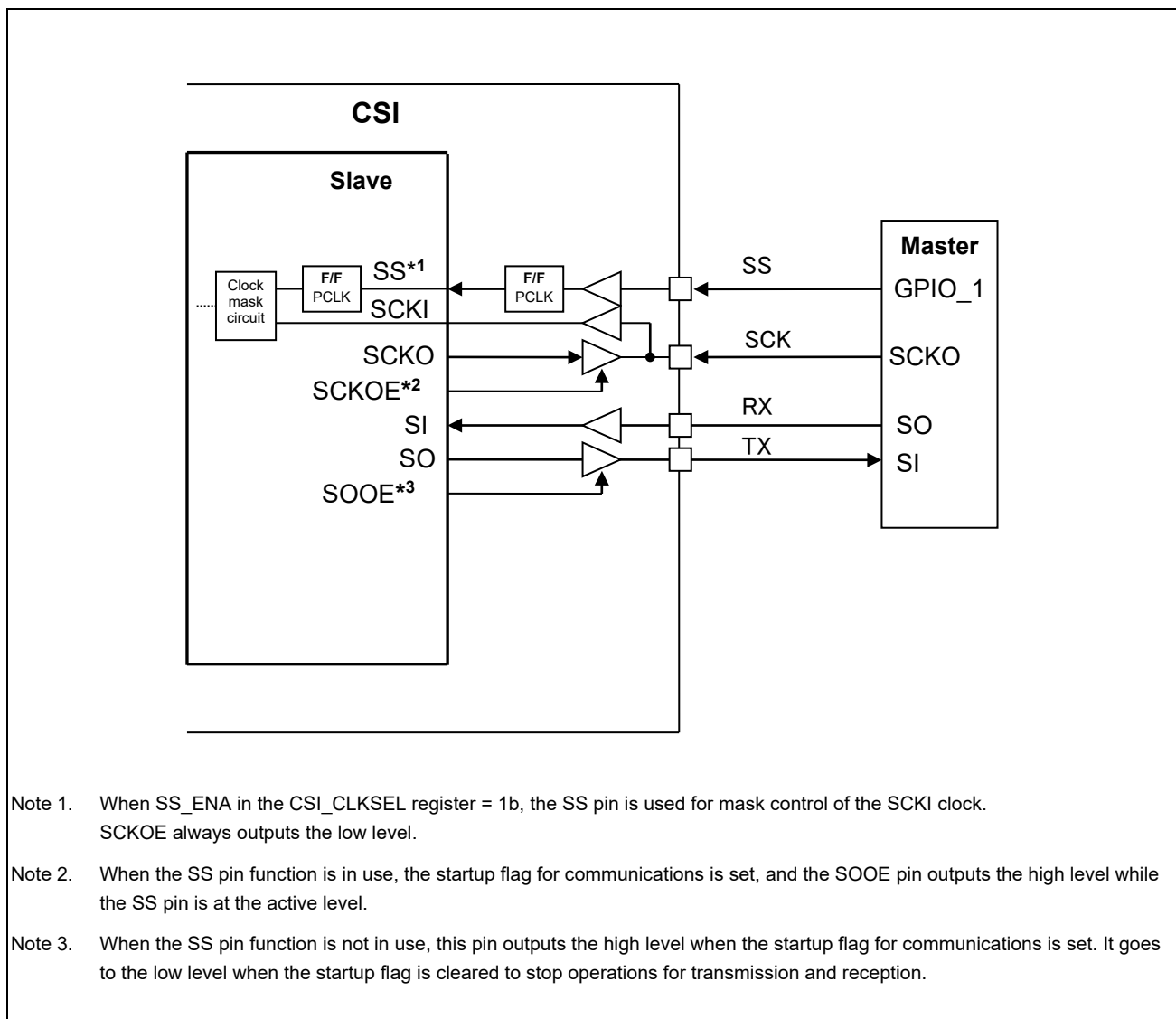
Figure 30.4-15 Example of Connection in Slave Transmission/Reception Mode
