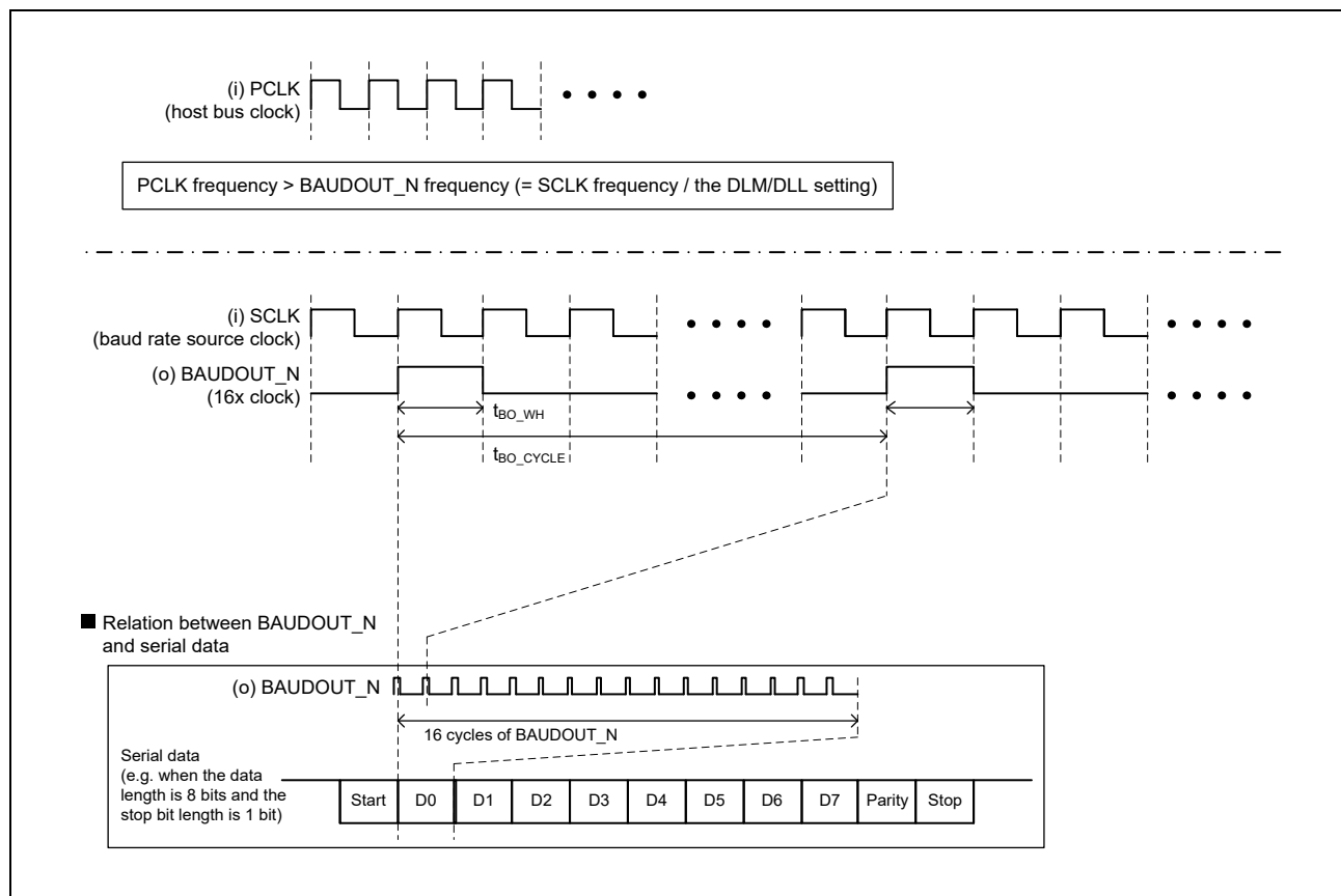
Figure 31.4-1 Clock Timing
