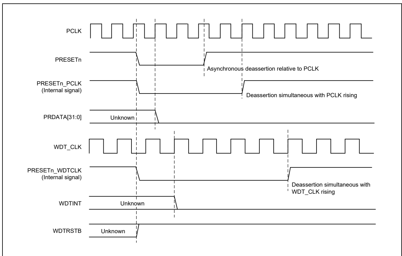
Figure 15.2-1 Reset Timing
