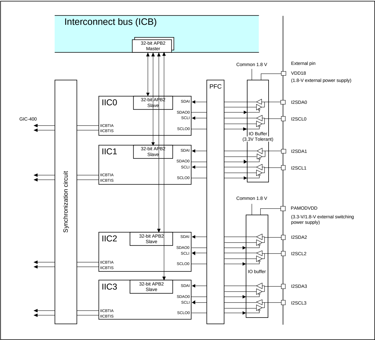
Figure 29.1-1 Connection Configuration
