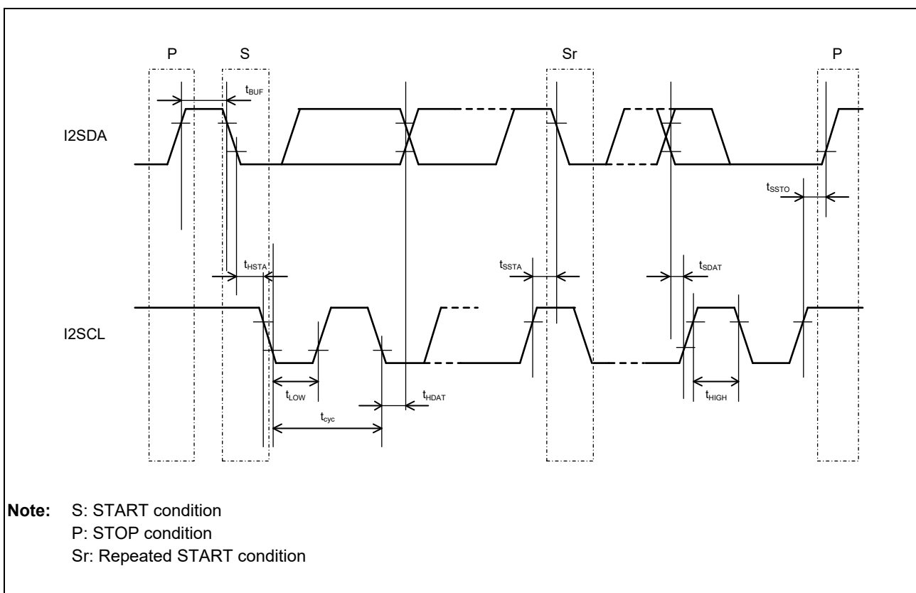
Figure 40.5-1 IIC Timing
