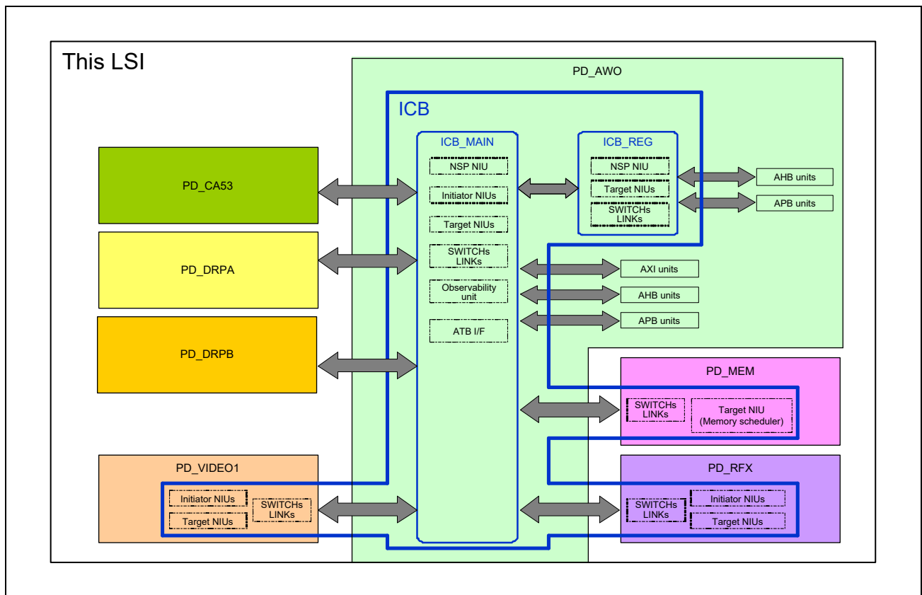
Figure 35.2-1 Internal Configuration
