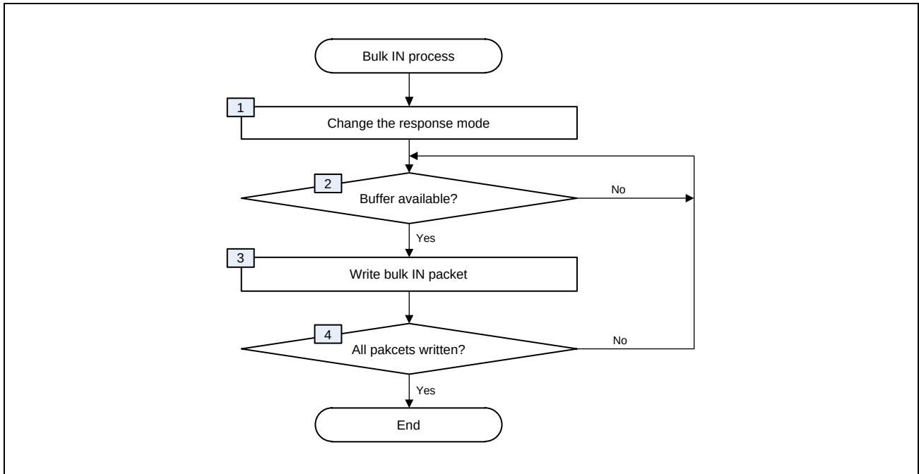
Figure 26.6-30 Bulk IN Process Flow
