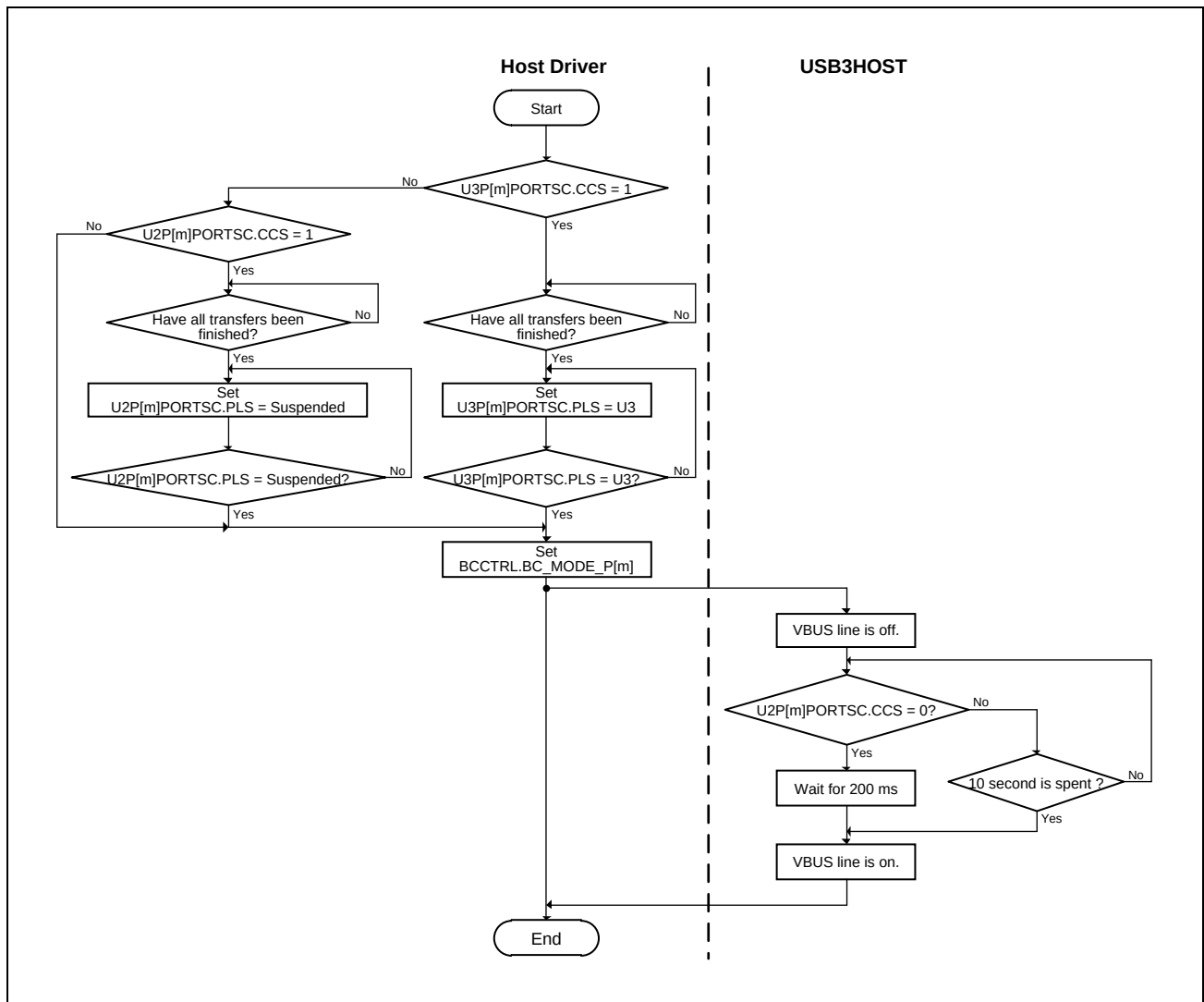
Figure 26.5-2 Host Driver's Flow to Set BC Mode (m = 1)
