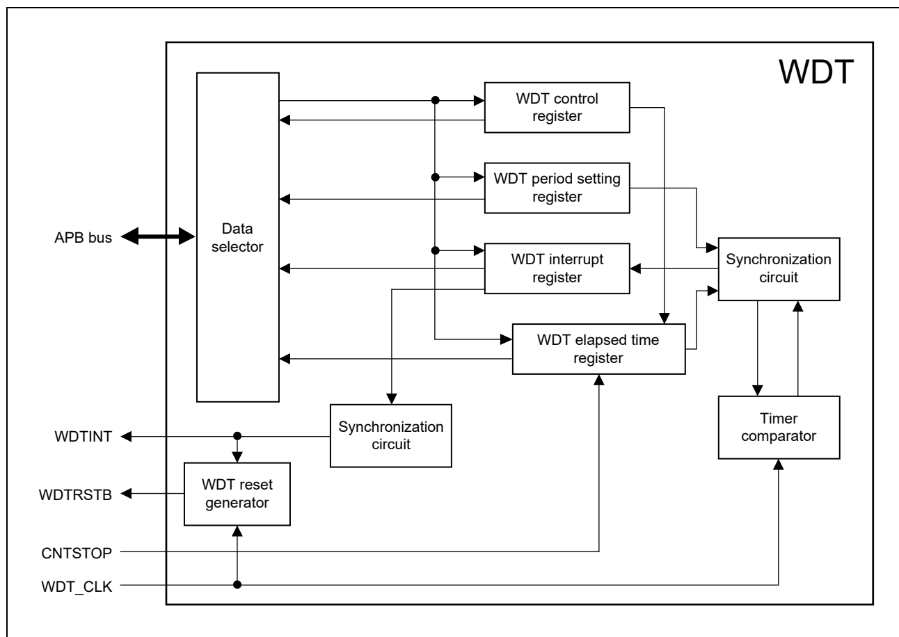
Figure 15.2-2 Block Diagram
