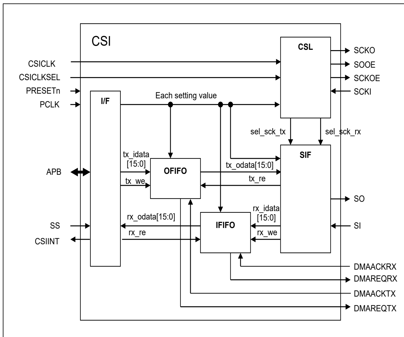
Figure 30.1-1 Block Diagram
