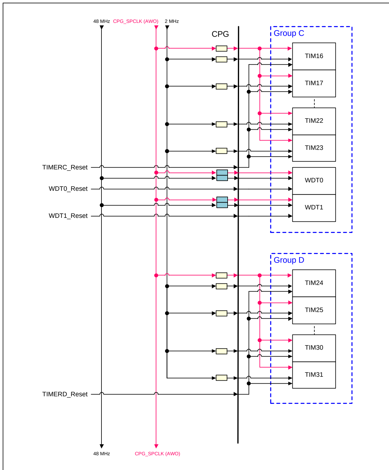
Figure 34.6-23 Block Diagram of Groups C and D
