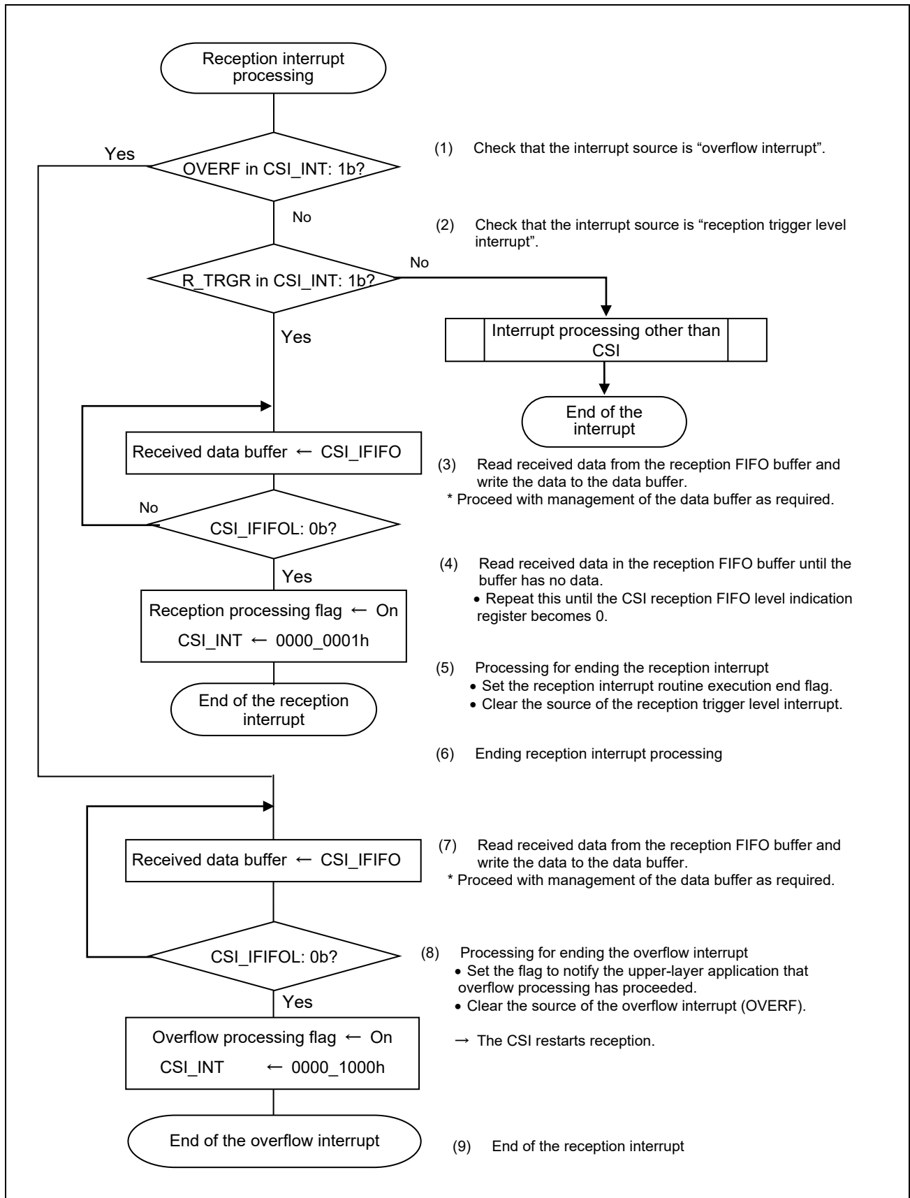
Figure 30.4-14 Flow of Operations with Interrupt Transfer in Slave Reception-only Mode (3/3)
