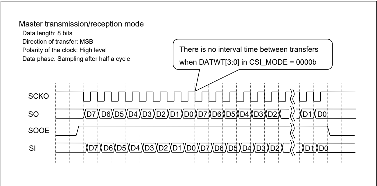
Figure 30.4-1 Interval Time Timing (when DATWT[3:0] = 0000b)
