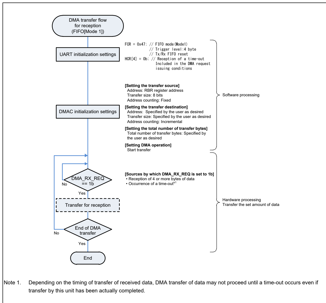
Figure 31.5-3 DMA Transfer Flow for Reception (a Time-out in Mode 1 when the FIFO Buffer is in Use is Included in the DMA Request Issuing Conditions)
