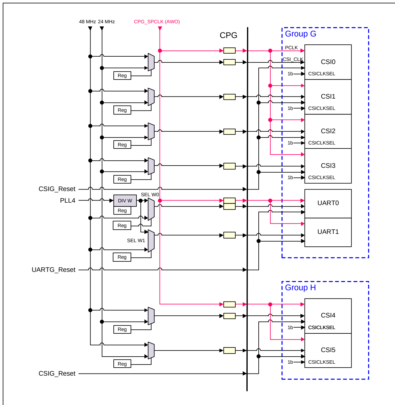
Figure 34.6-25 Block Diagram of Groups G and H
