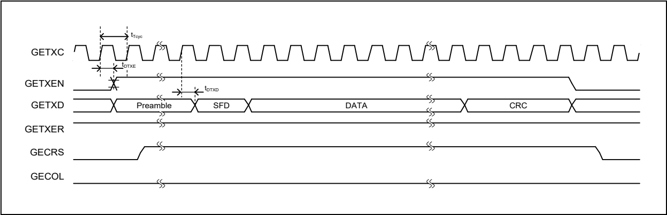
Figure 40.5-4 Transmission Timing
