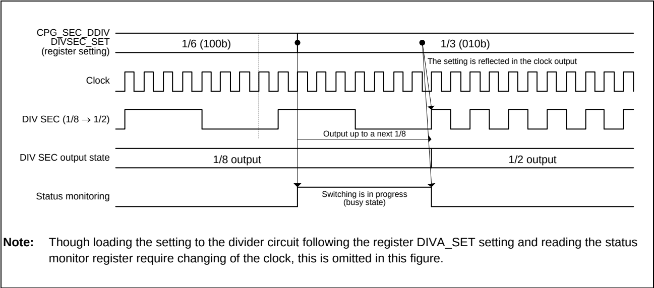
Figure 34.6-12 Timing Chart of Clock Switching of the Dynamic Switching Variable Divider (Duty50 Type)
