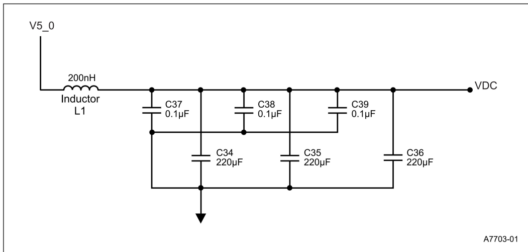
Figure 5. V_DC to V_5 Decoupling Circuit Example
