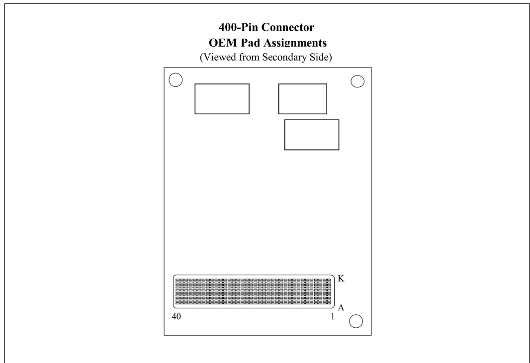
Figure 2. 400-Pin Connector Footprint Pad Numbers, Module Secondary Side
