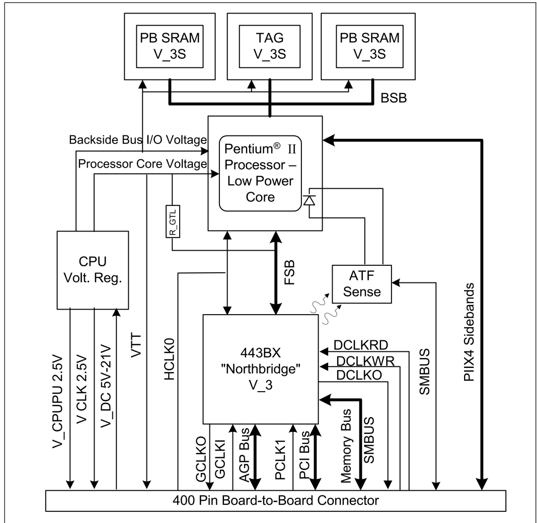
Figure 1. Block Diagram of the Pentium II Processor – Low-Power Module
