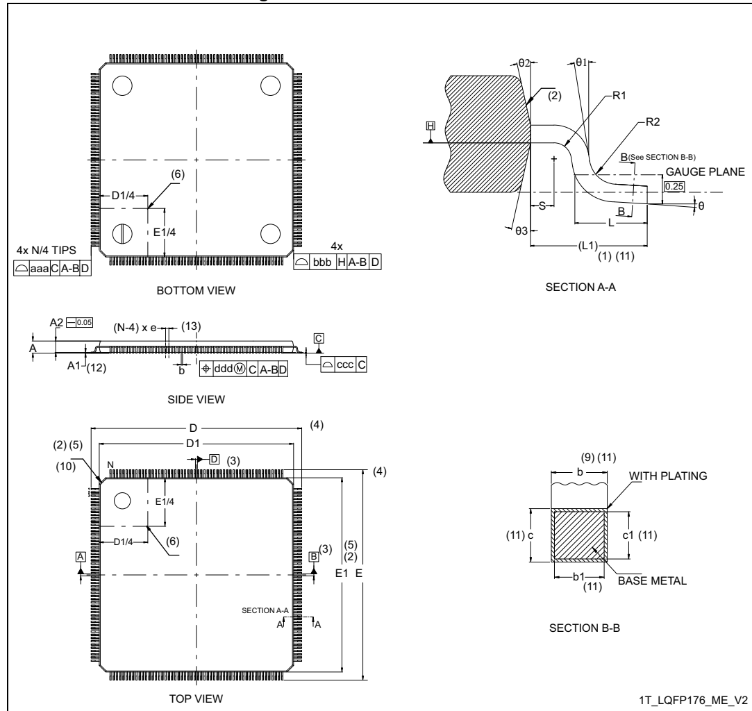
Figure 75. LQFP176 - Outline (15)
