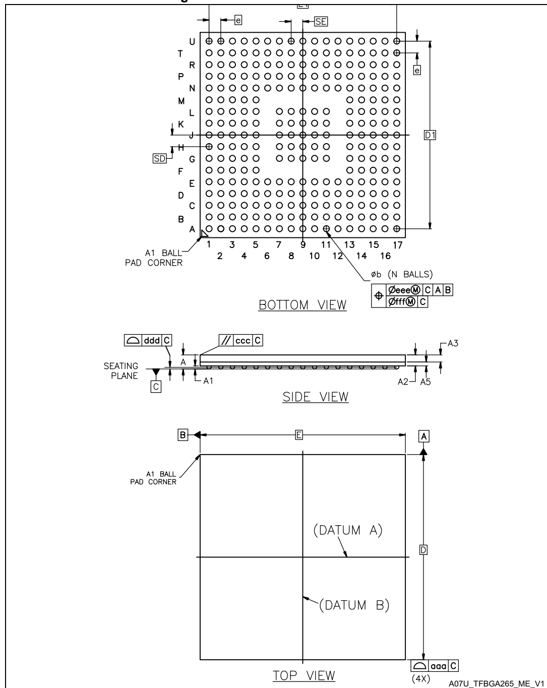
Figure 79. TFBGA240+25 - Outline
