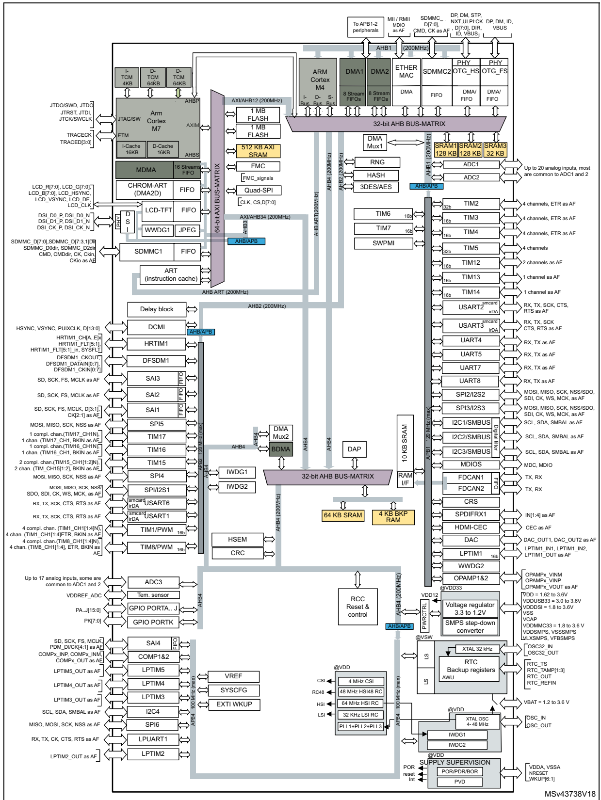
Figure 1. STM32H757xI block diagram
