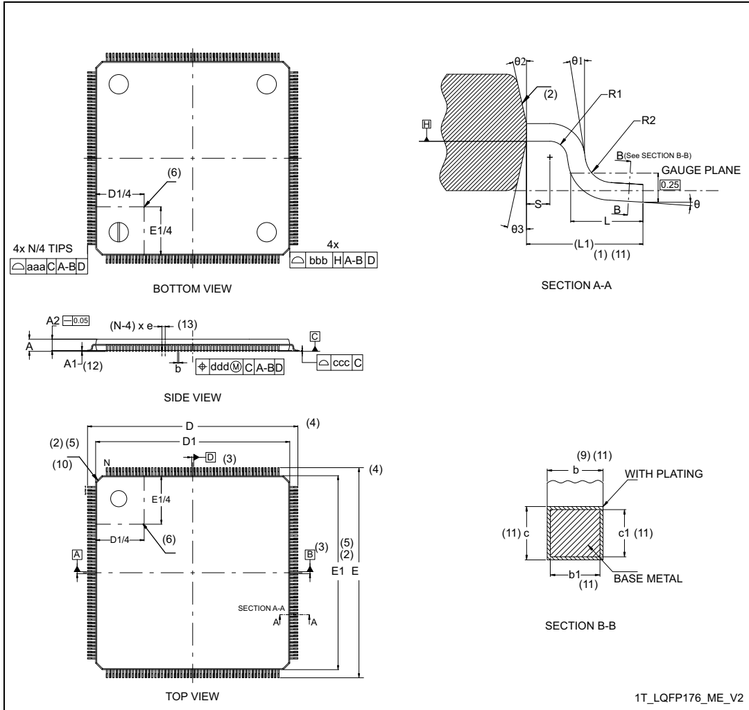
Figure 75. LQFP176 - Outline (15)
