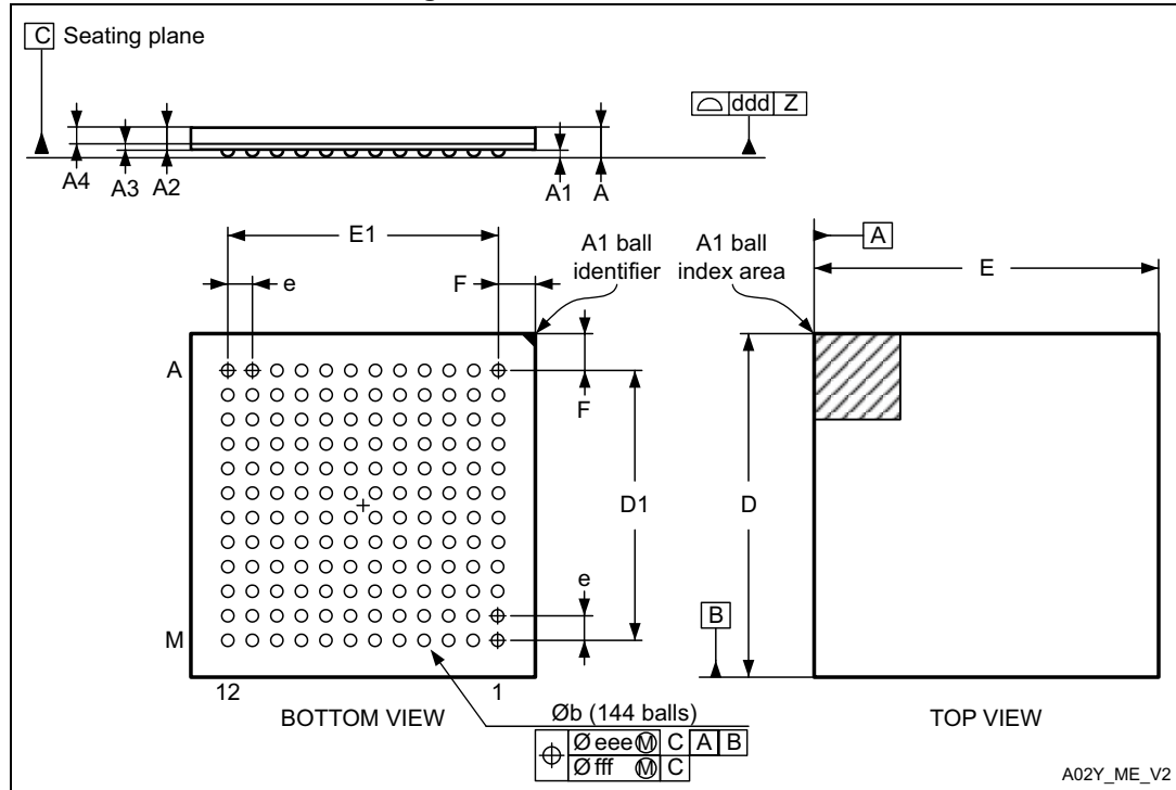
Figure 75. UFBGA144 outline
