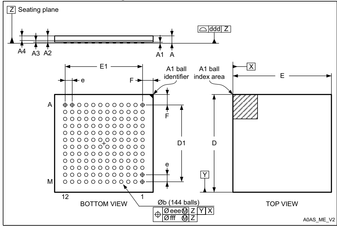
Figure 73. UFBGA144 outline
