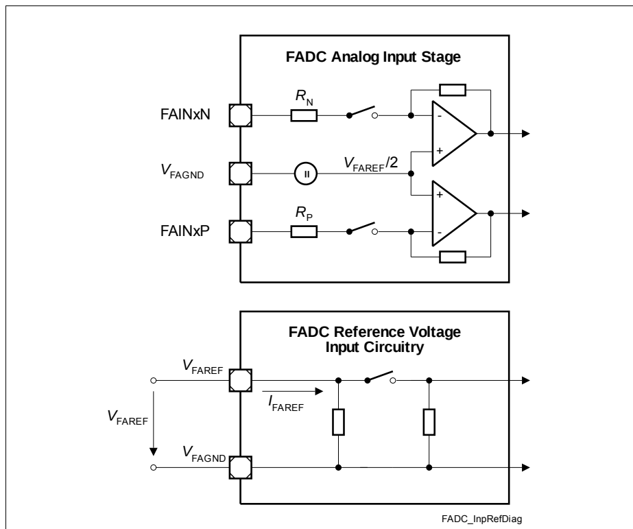
Figure 4 FADC Input Circuits
