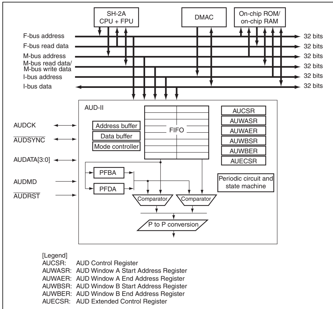
Figure 21.1 Block Diagram of AUD-II
