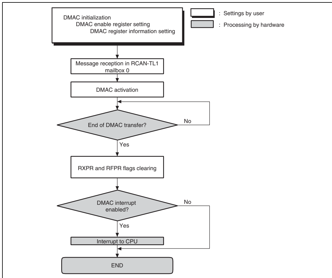
Figure 18.27 DMAC Transfer Flowchart
