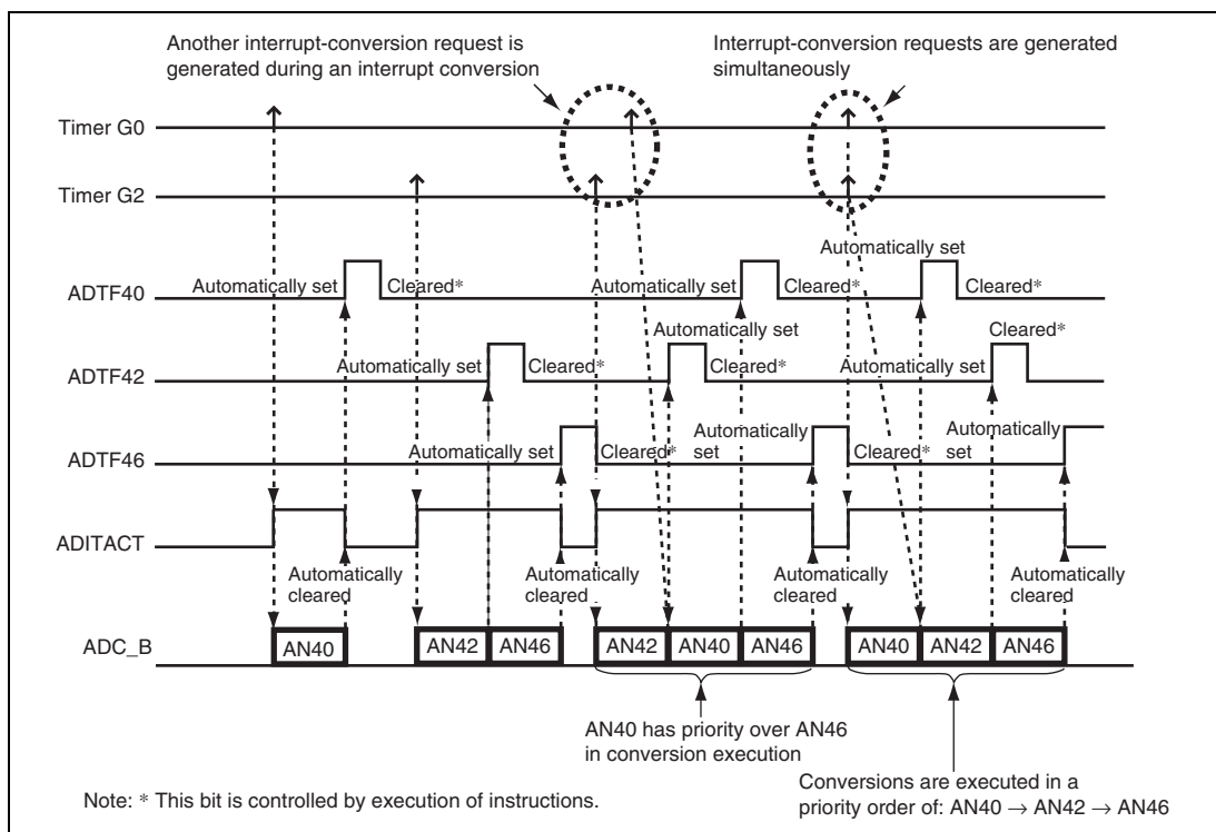
Figure 19.6 Example Operation of Interrupt Conversion
