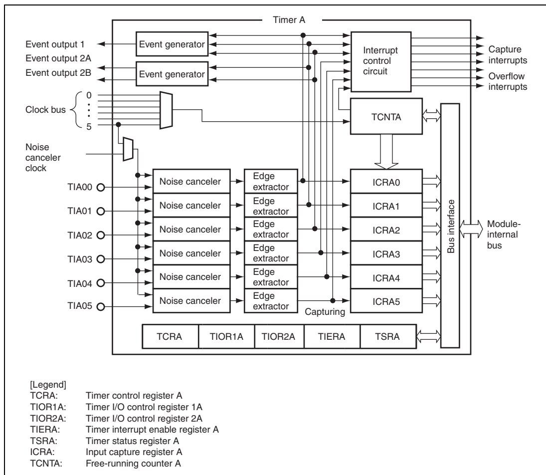
Figure 13.5 Block Diagram of Timer A
