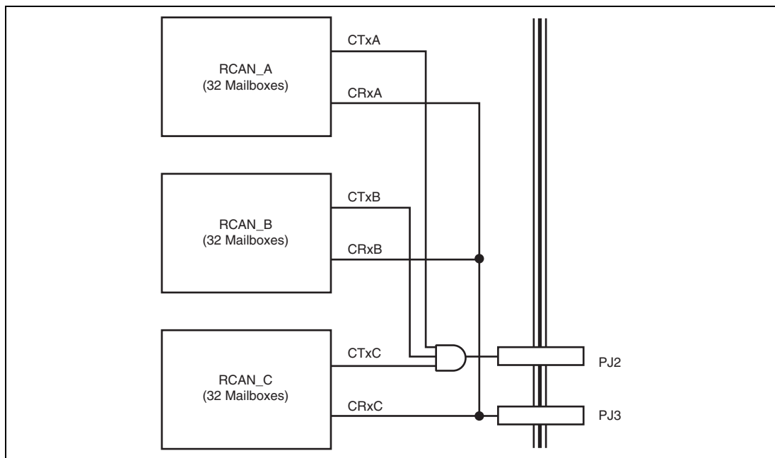
Figure 18.31 Connection Example when Using RCAN-TL1 as 1-Channel Module (96 Mailboxes × 1 Channel)
