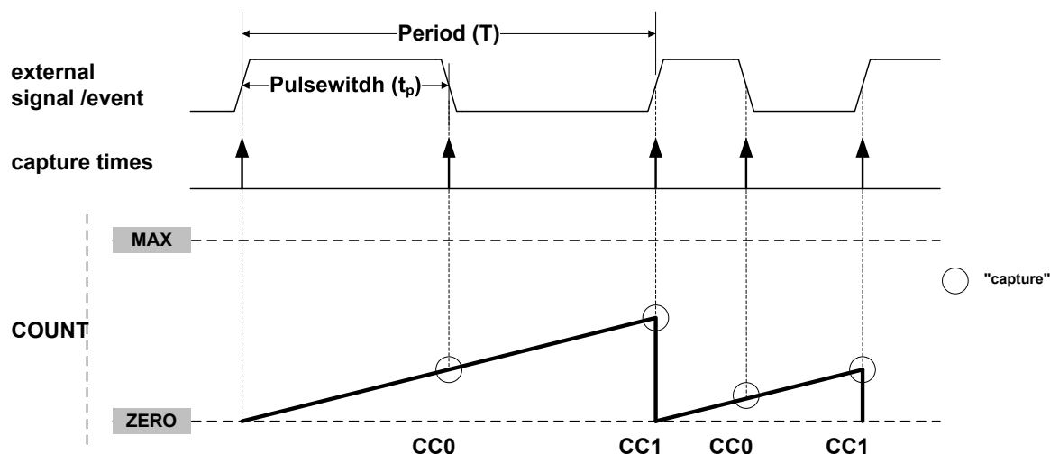
Figure 41-16. PWP Capture
