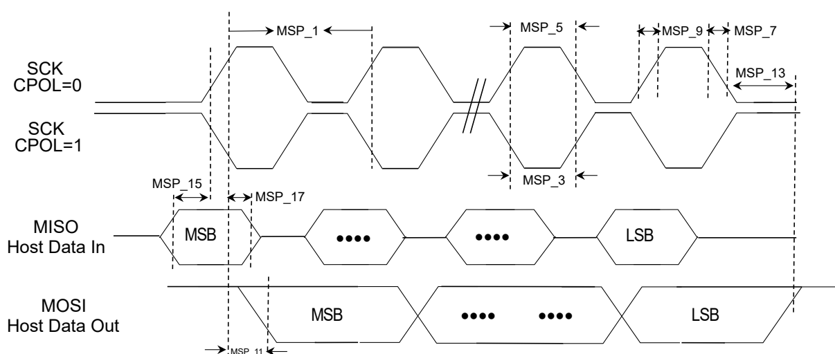
Figure 43-44. SPI Host Module CPHA = 0 Timing Diagrams
