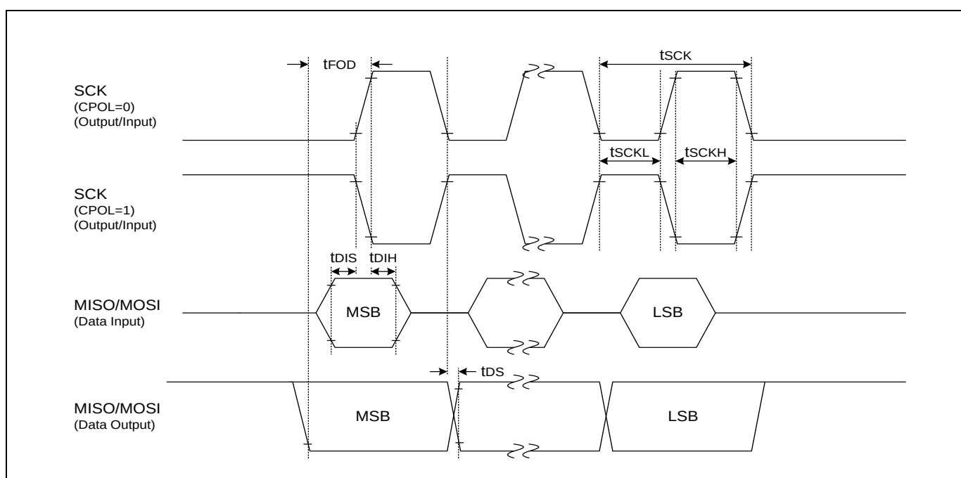
Figure 7.2 SPI Timing
