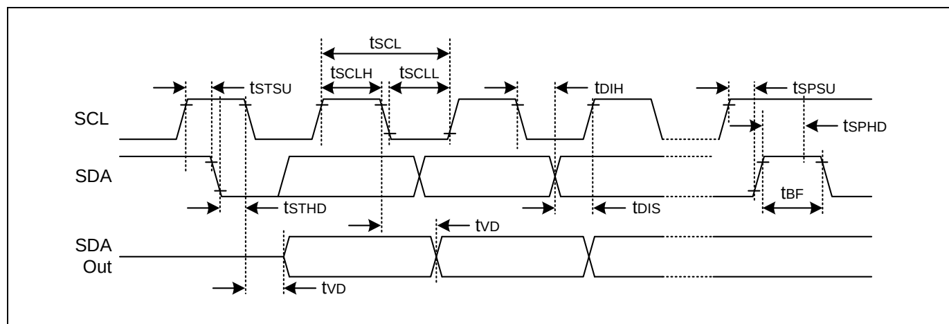
Figure 7.5 I2C Timing
