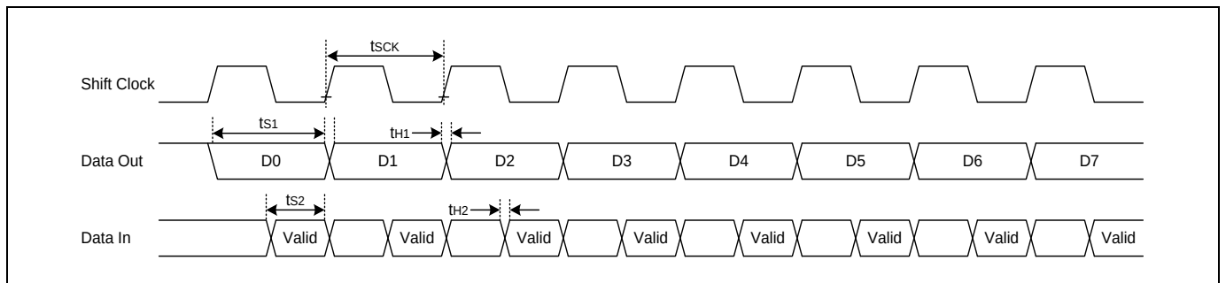
Figure 7.4 Timing Waveform for the UART Module
