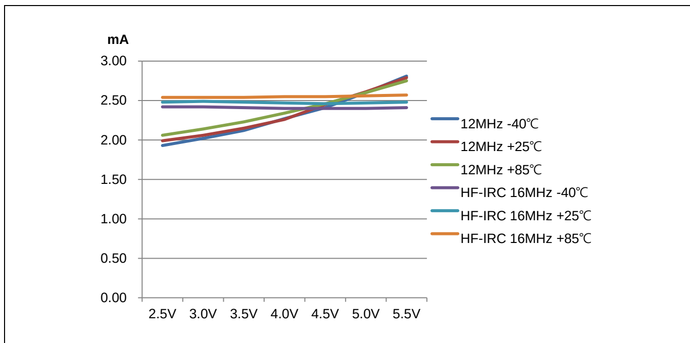
Figure 7.14 RUN (IDD1) Current
