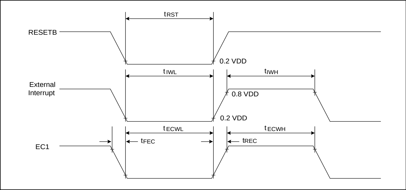
Figure 7.1 AC Timing
