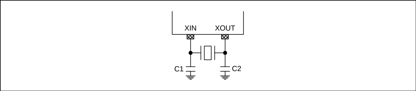
Figure 7.8 Crystal/Ceramic Oscillator
