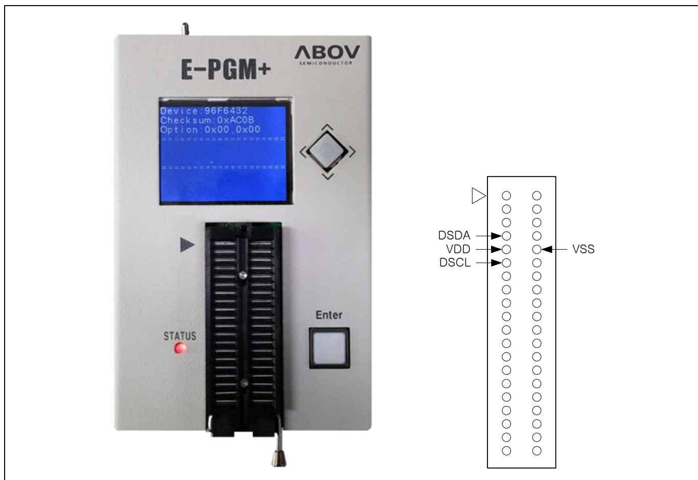
Figure 1.3 E-PGM+(Single writer)
