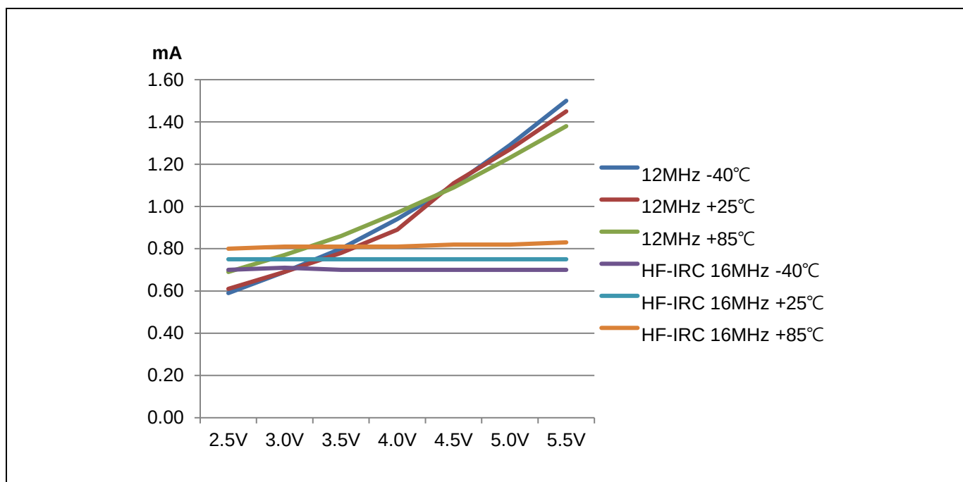
Figure 7.15 IDLE (IDD2) Current
