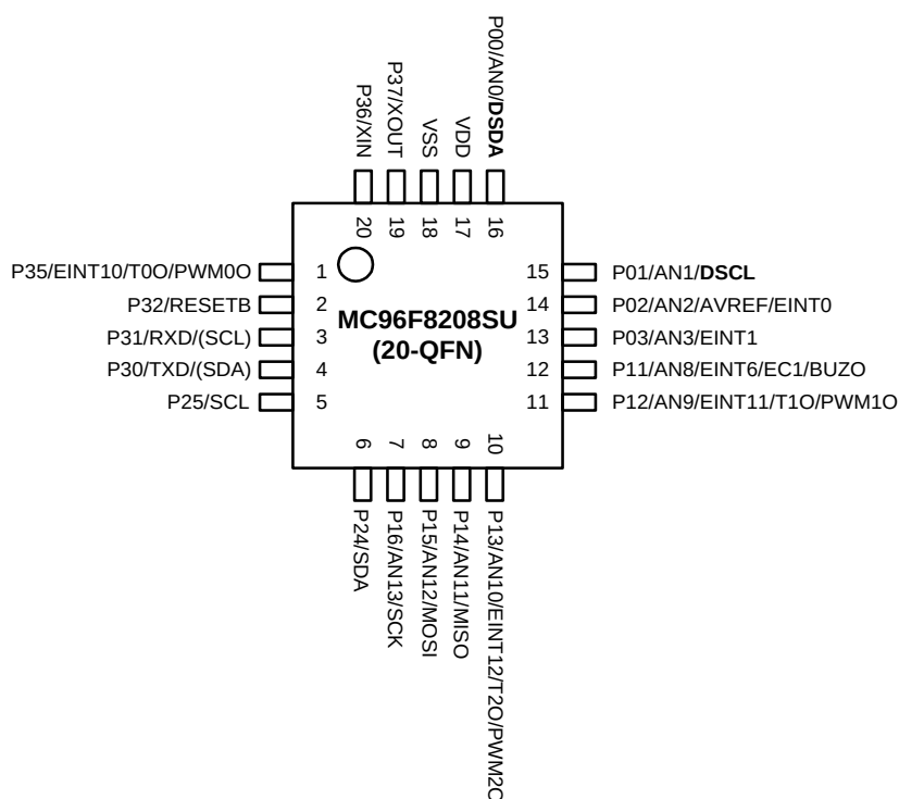
Figure 3.1 MC96F8208SD/R/B 20SOP/TSSOP/PDIP Pin Assignment
