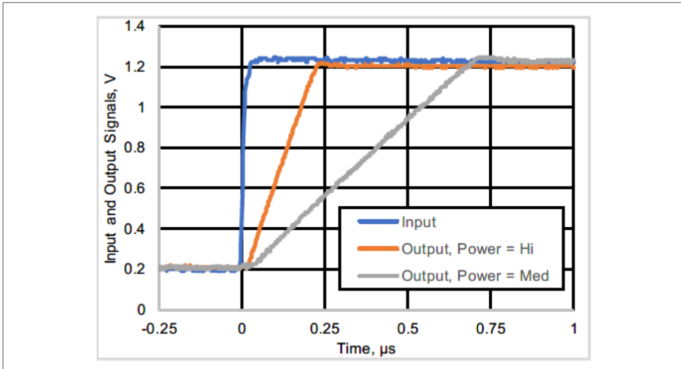
Figure 17 Opamp step response, rising
