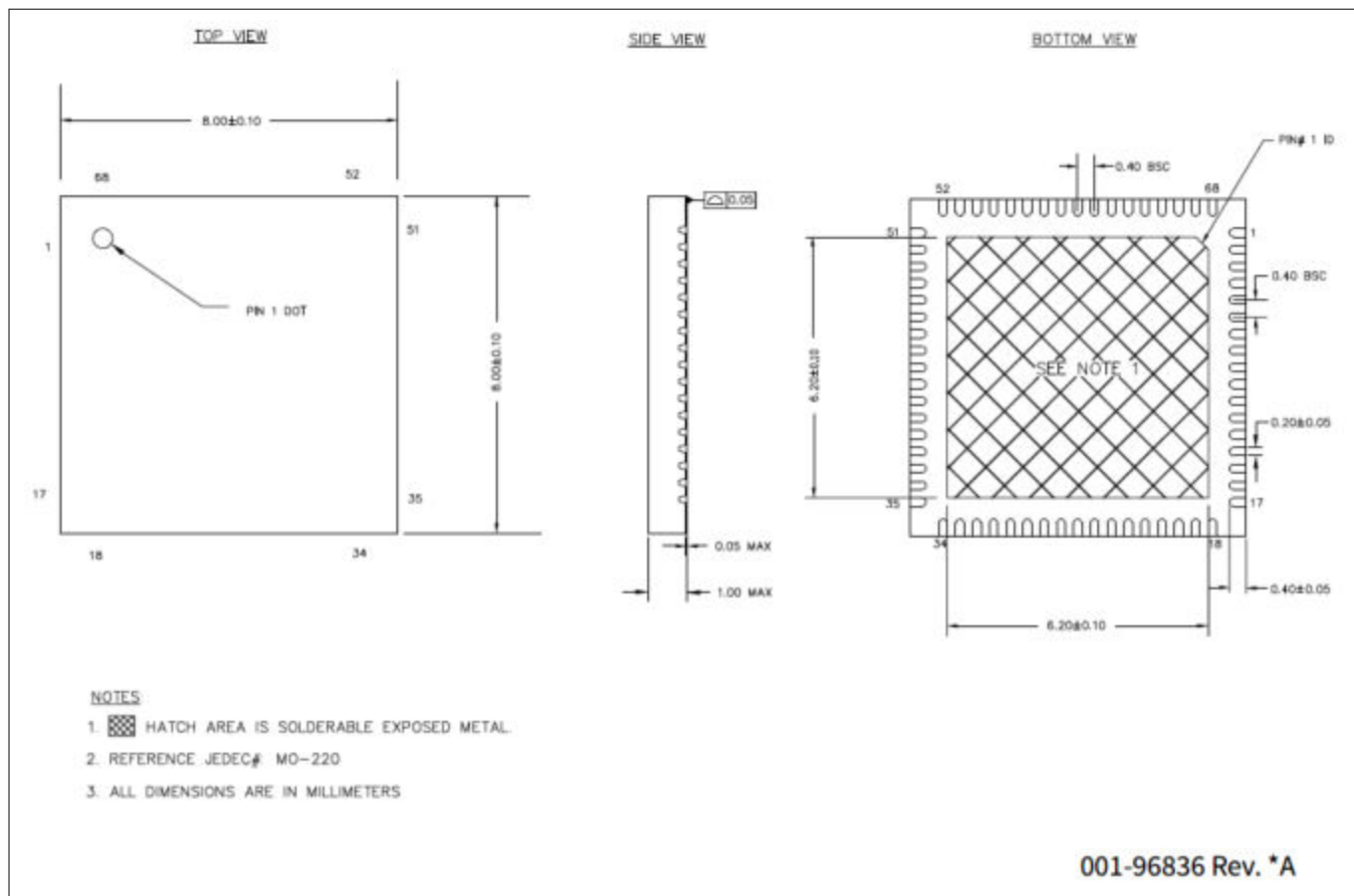
Figure 19 68-QFN 8.0 × 8.0 × 1.0 mm LT68D, 6.2 × 6.2 mm EPAD (PG-VQFN-68)
