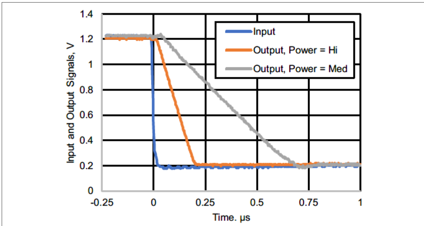
Figure 18 Opamp step response, falling
