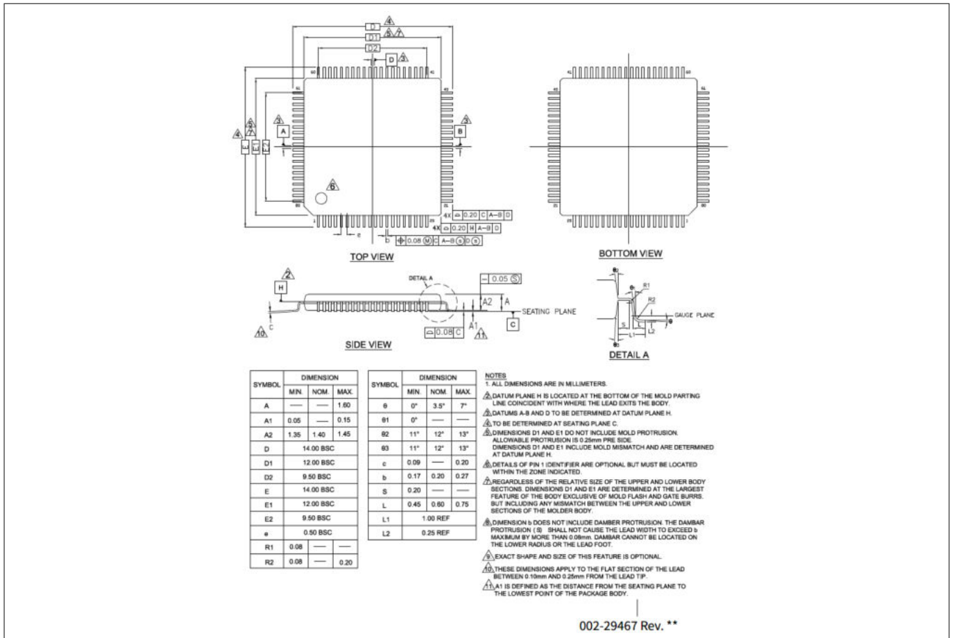
Figure 20 80-pin TQFP ((12.0 × 12.0 × 1.6 mm) AZ80A) package outline (PG-TQFP-80)
