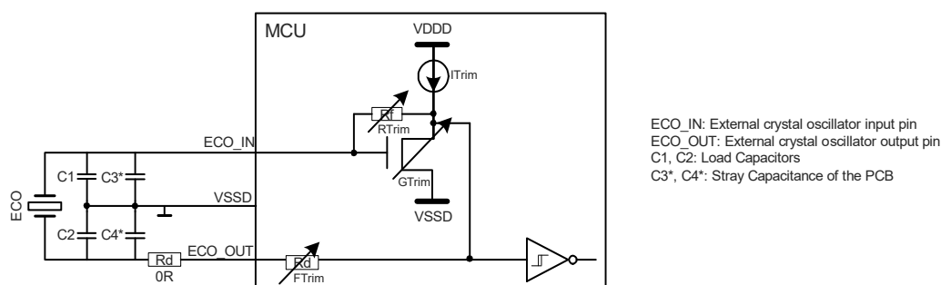
Figure 26-22. ECO Connection Scheme [53]
