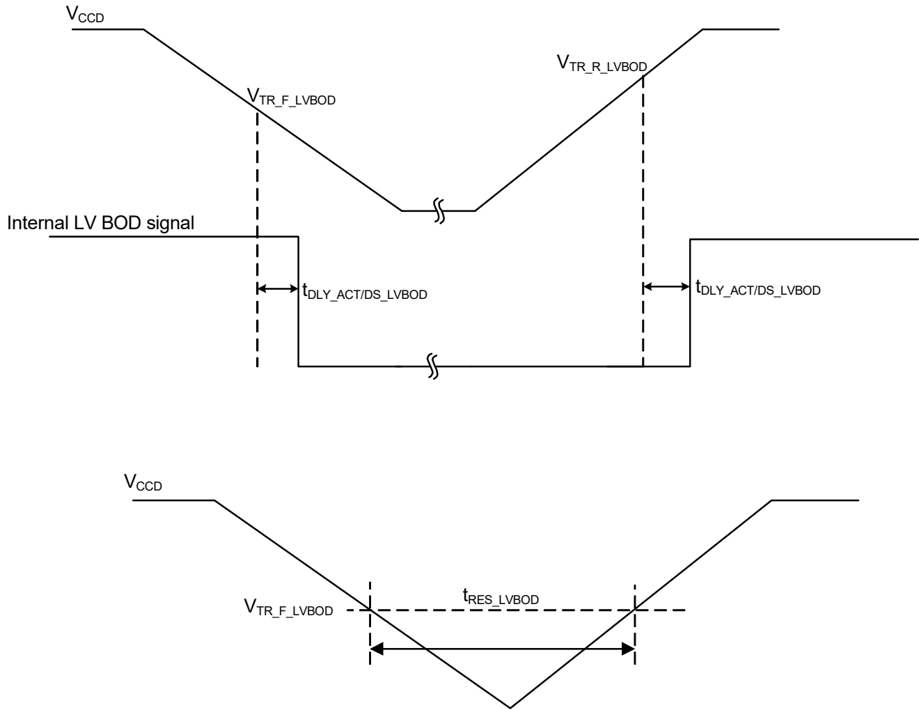
Figure 26-17. Low-Voltage BOD Specifications
