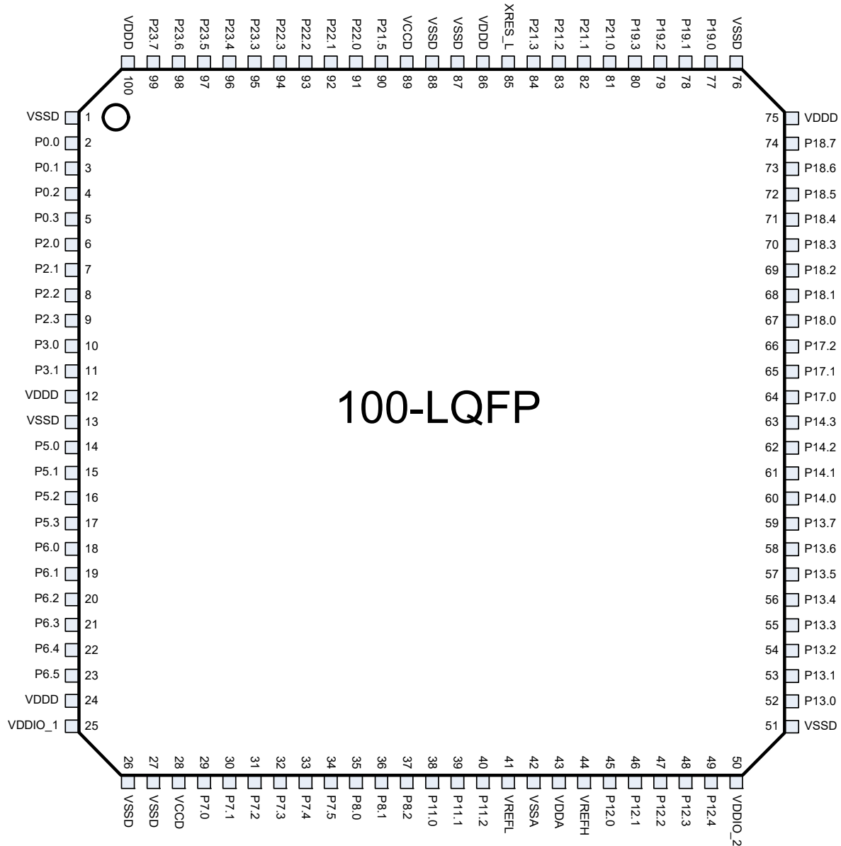
Figure 9-1. 100-LQFP Pin Assignment
