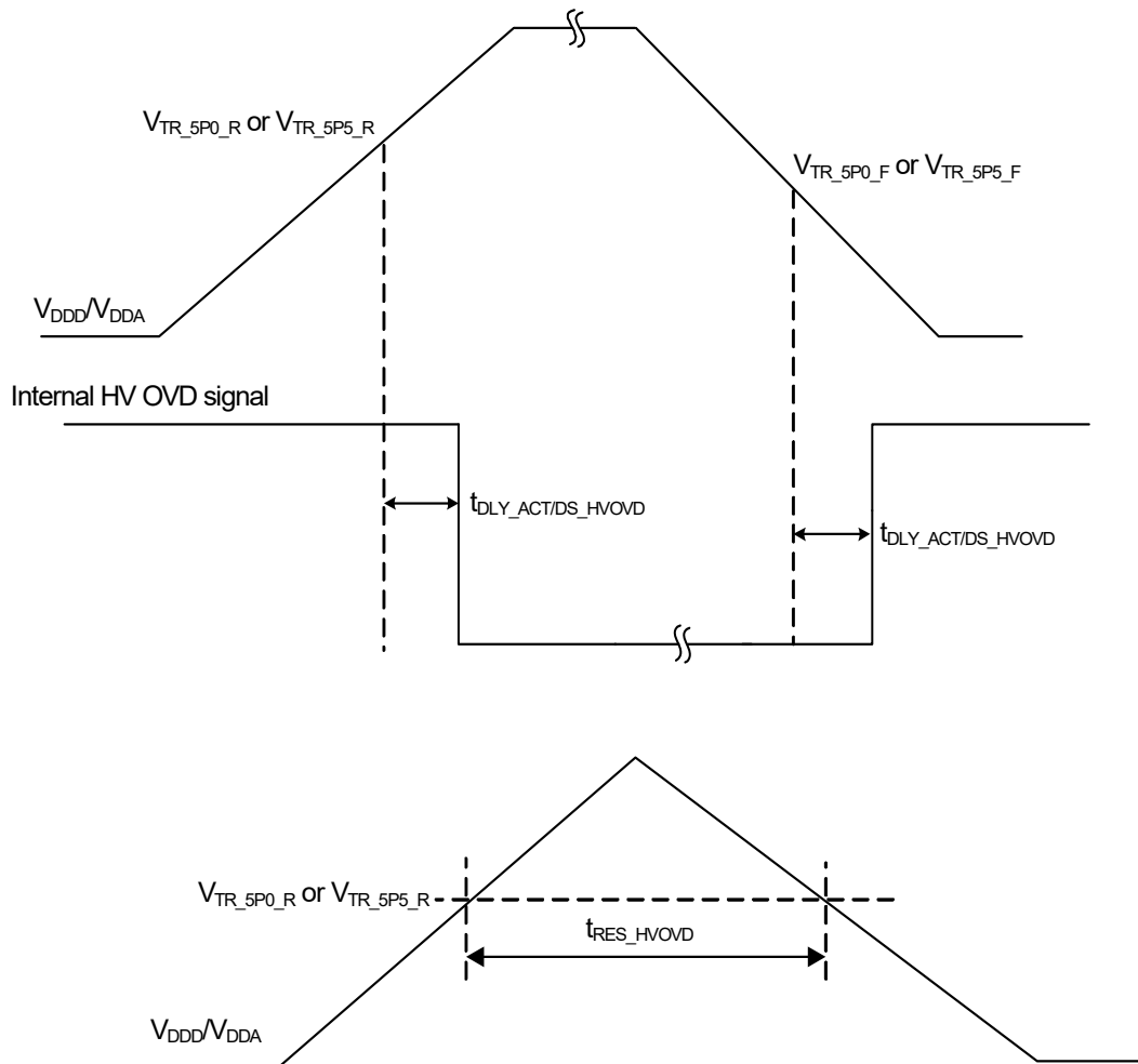
Figure 26-18.High-Voltage OVD Specifications
