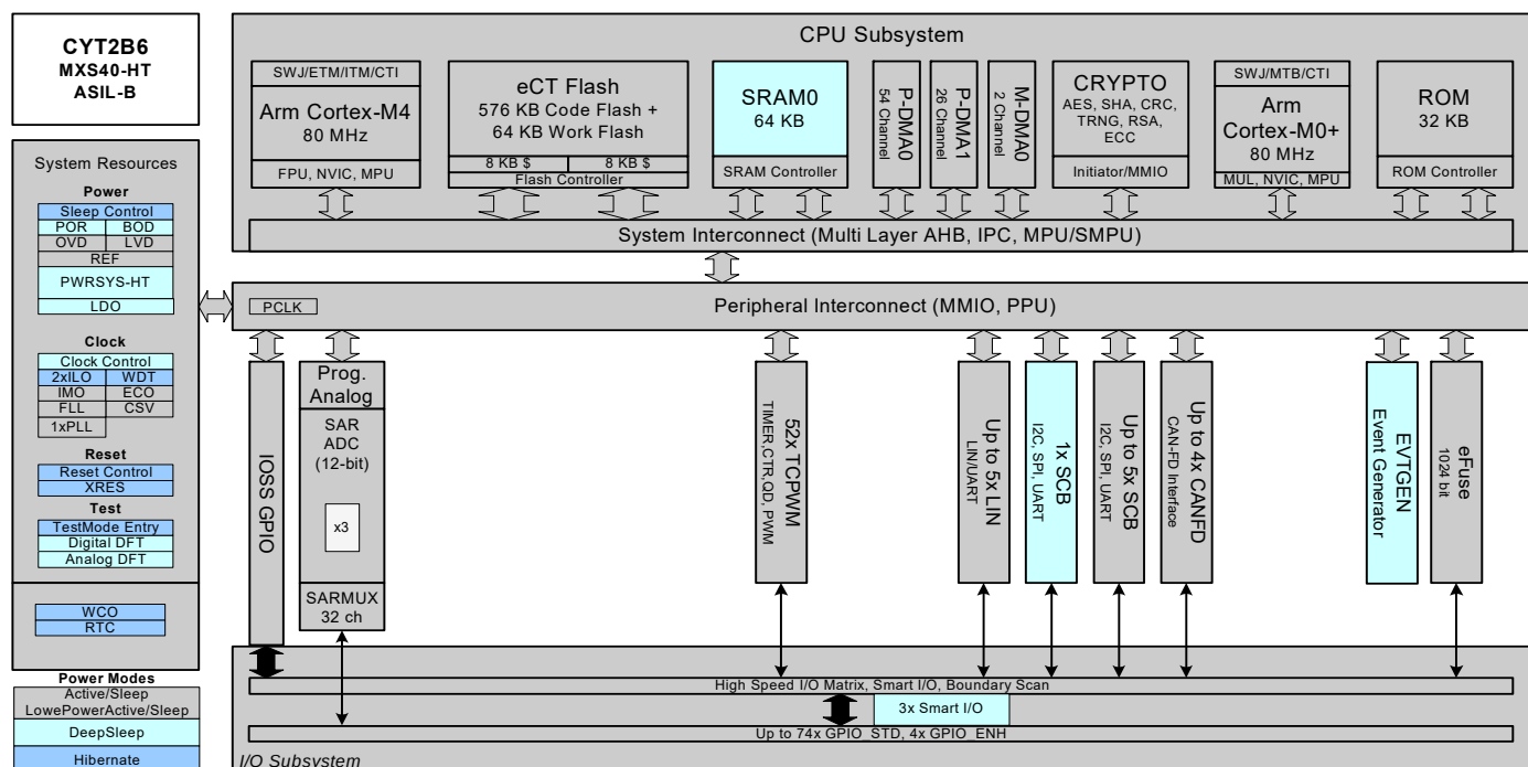
Figure 2-1. Block Diagram
