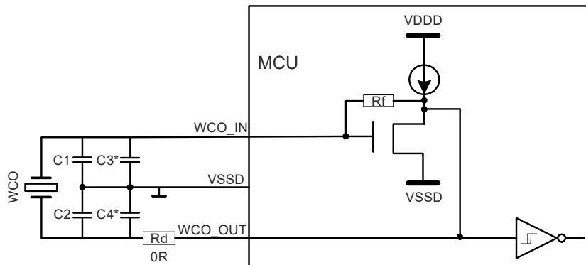
Figure 26-23.WCO Connection Scheme [55]
