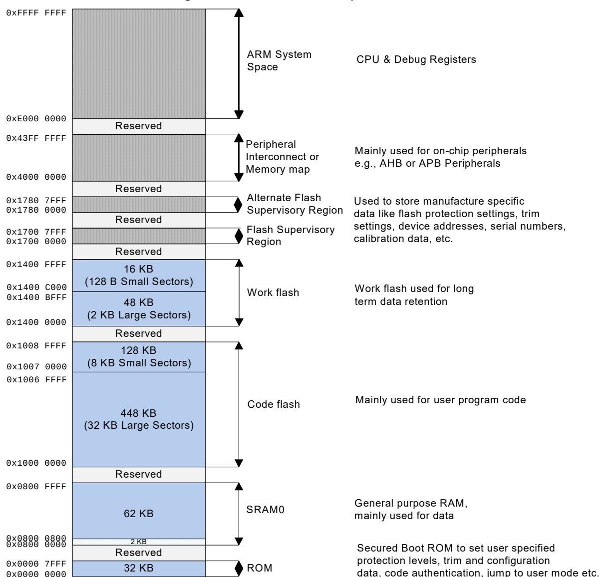
Figure 4-1.CYT2B6 Address Map [14, 15]
