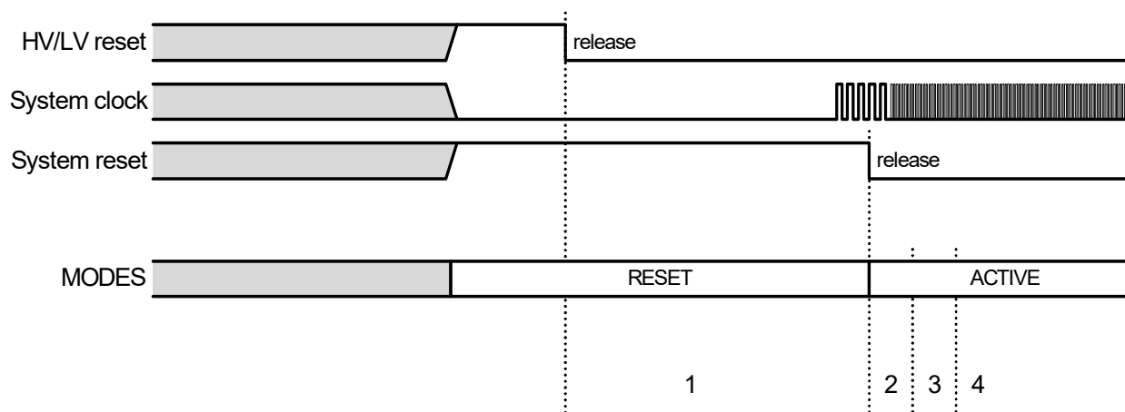
Figure 26-3.Reset Sequence
