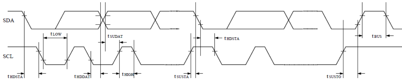
Figure 12. I2C Timing
