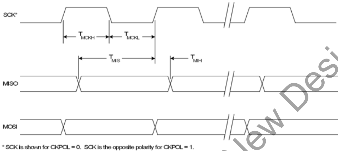
Figure 30.9. SPI Master Timing (CKPHA = 1)
