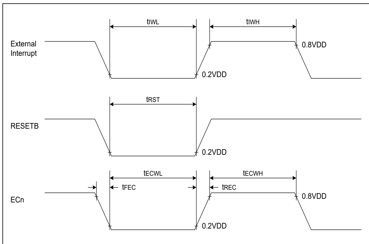
Figure 34. AC Timing
