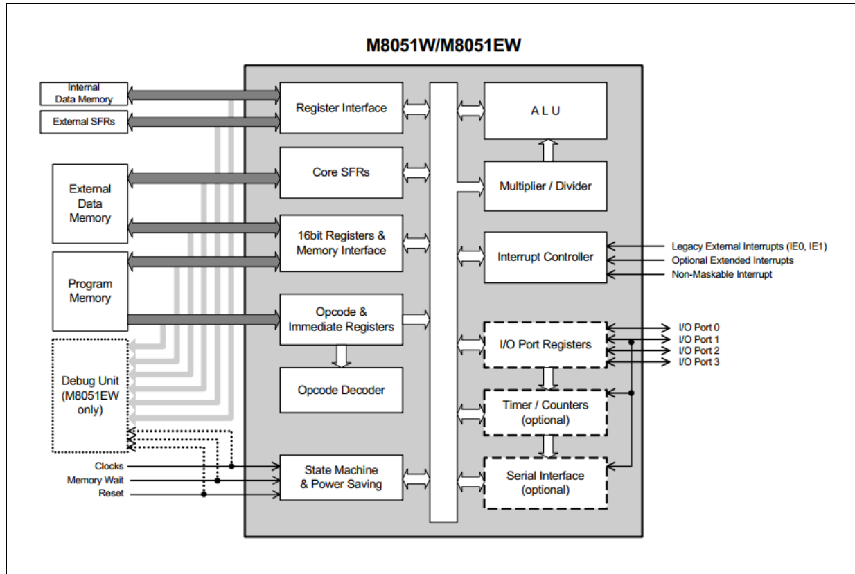
Figure 11. M8051EW Architecture
