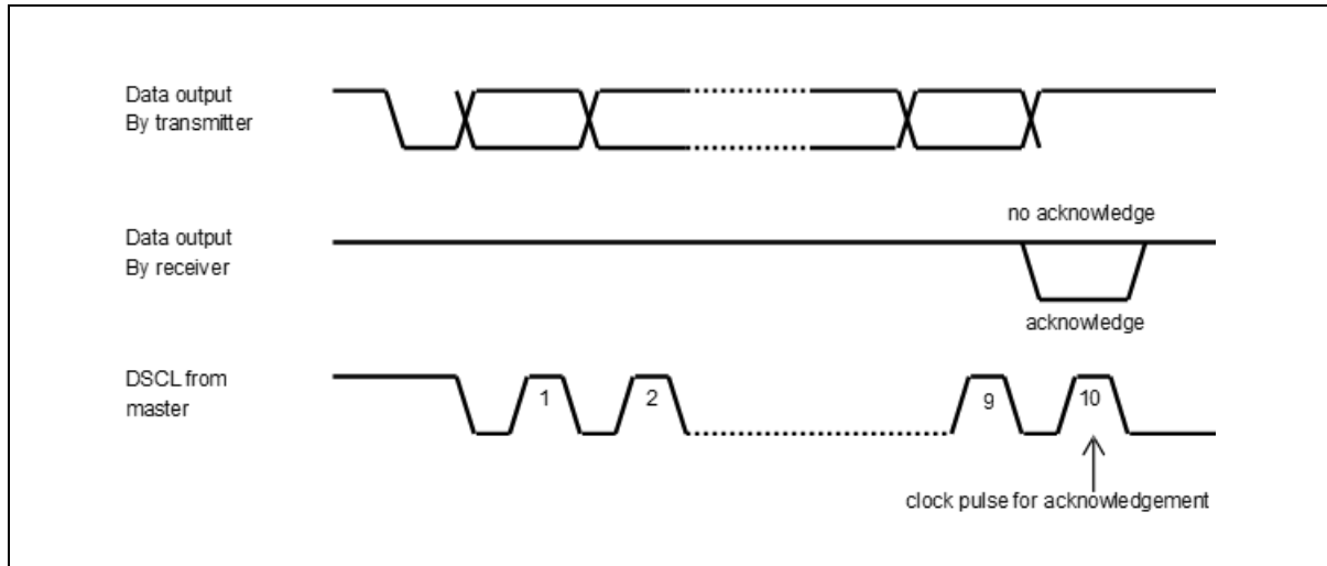
Figure 66. Acknowledge on the Serial Bus
