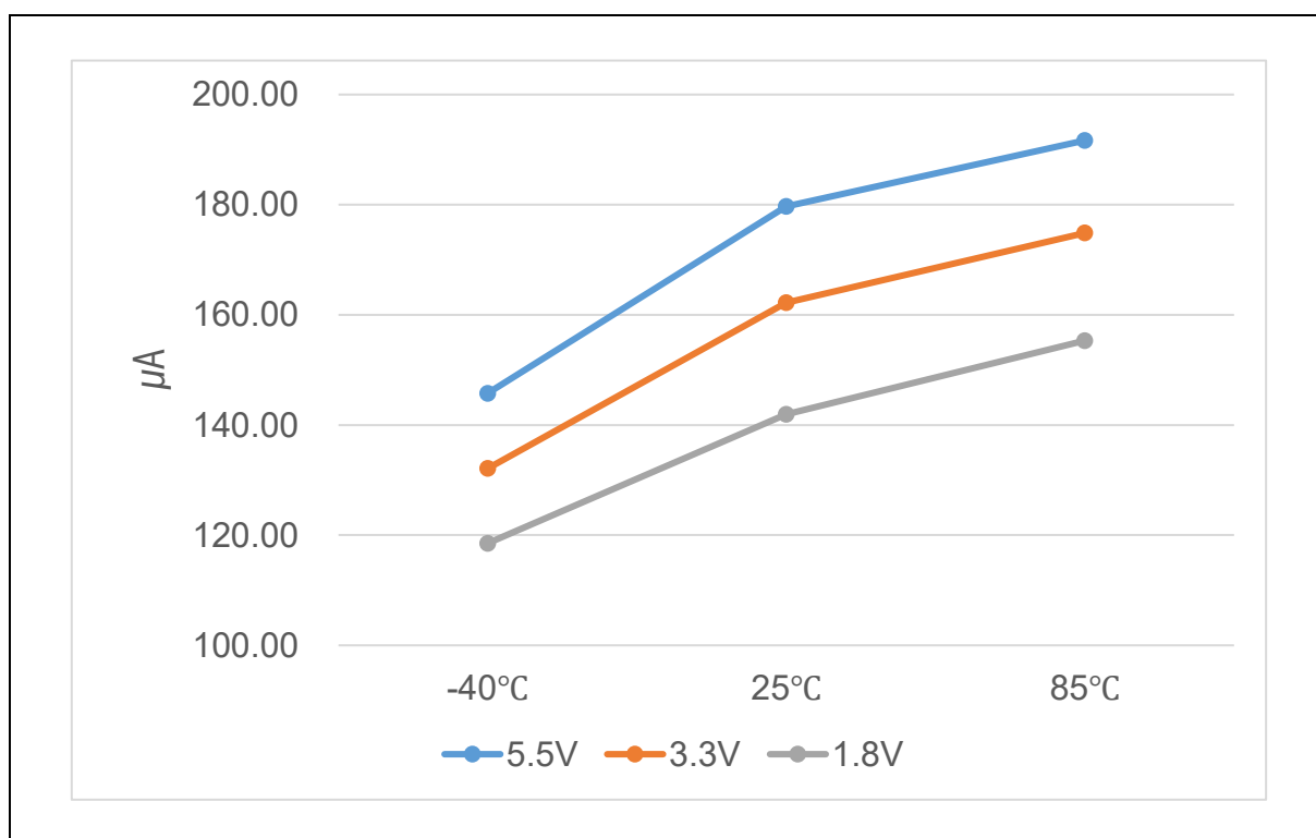
Figure 54. IDLE (IDD2, fLSI = 128 kHz) Current
