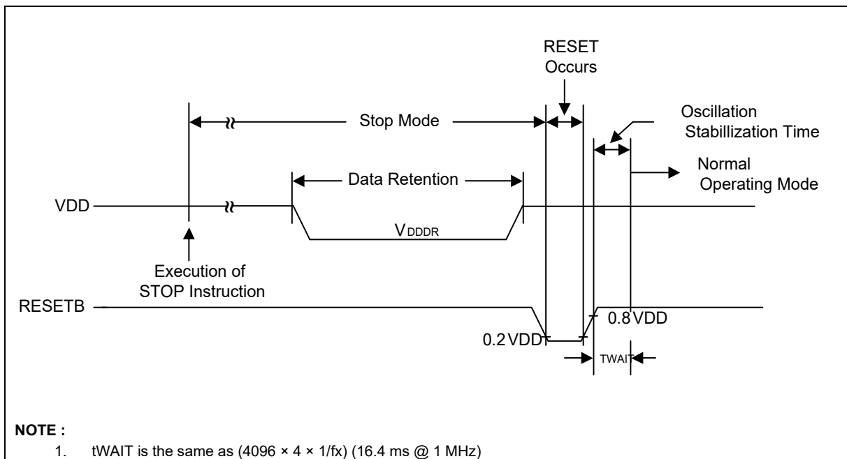
Figure 42. Stop Mode Release Timing when Initiated by RESETB
