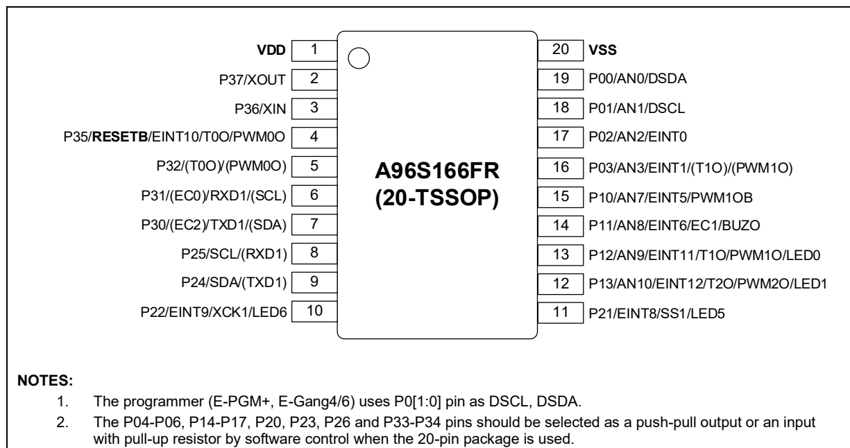
Figure 5. A96S166 20-TSSOP Pin Assignment
