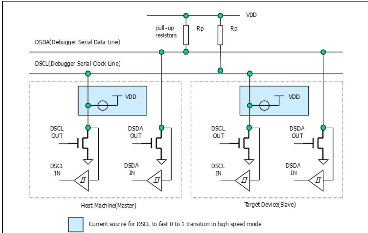
Figure 68. Connection of Transmission
