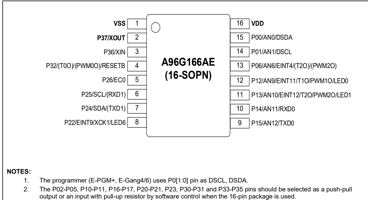
Figure 2. A96G166 16-SOPN Pin Assignment
