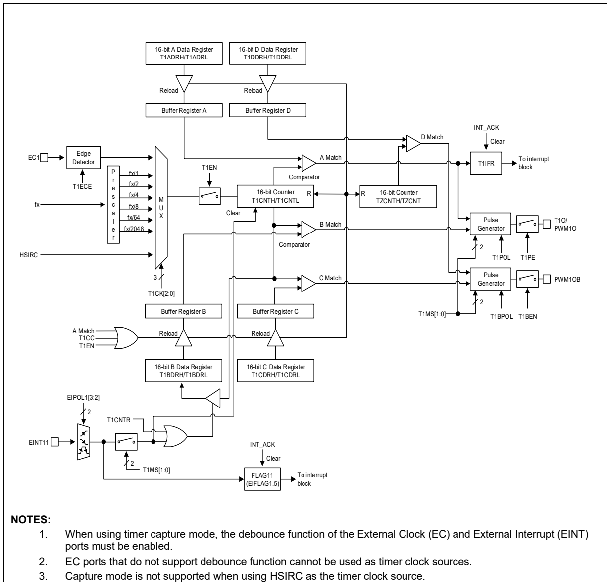
Figure 23. 16-bit Timer 1 Block Diagram
