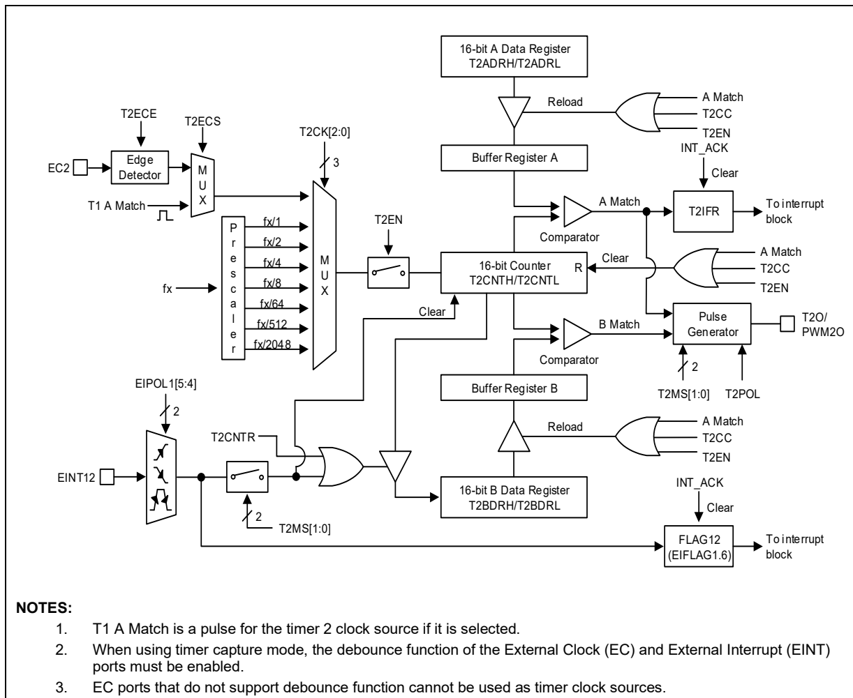
Figure 24. 16-bit Timer 2 Block Diagram
