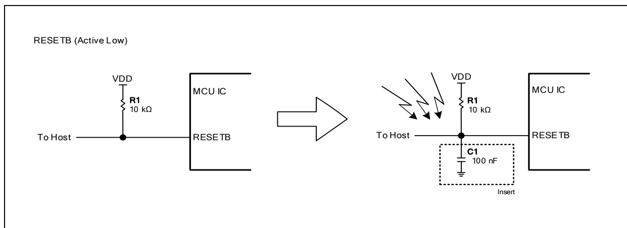
Figure 51. Filters Used on a Reset Pin
