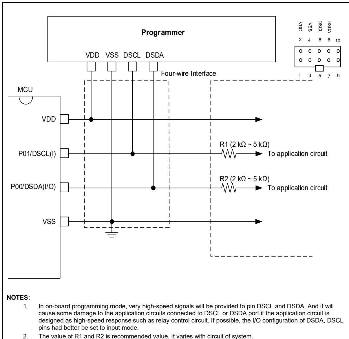
Figure 69. PCB Design Guide for On-Board Programming
