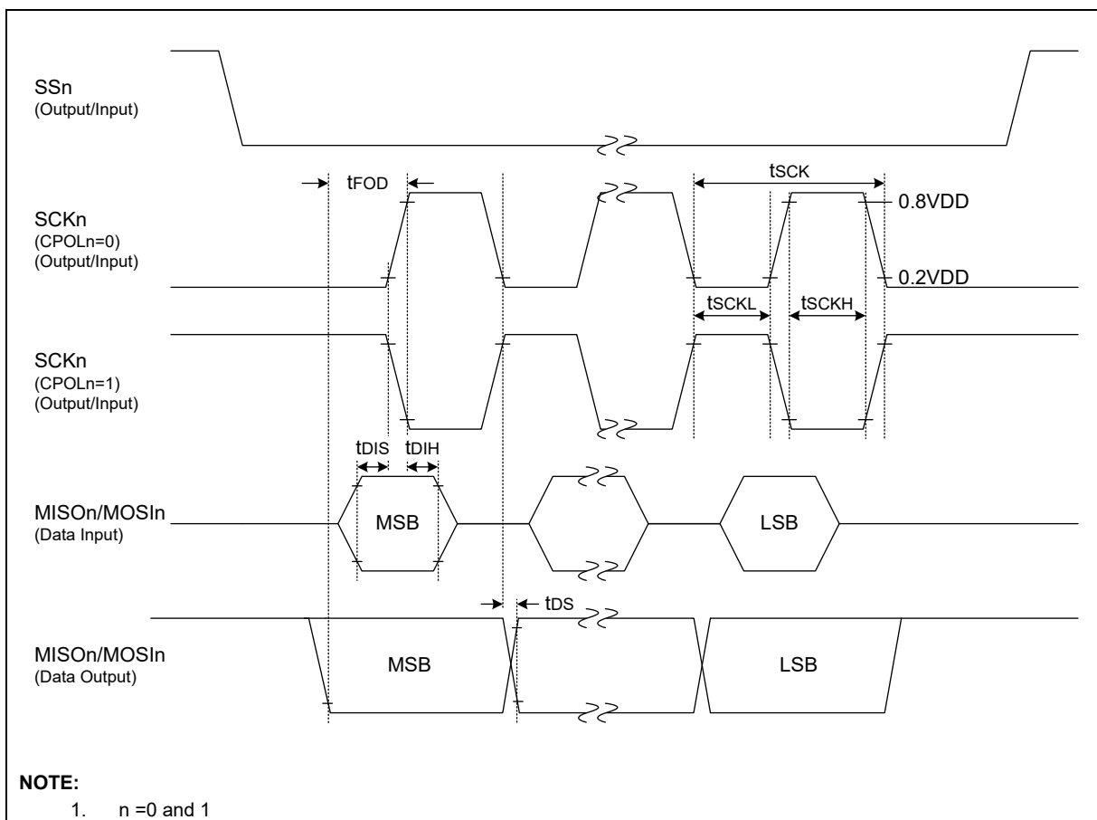
Figure 39. SPI0/1 Timing
