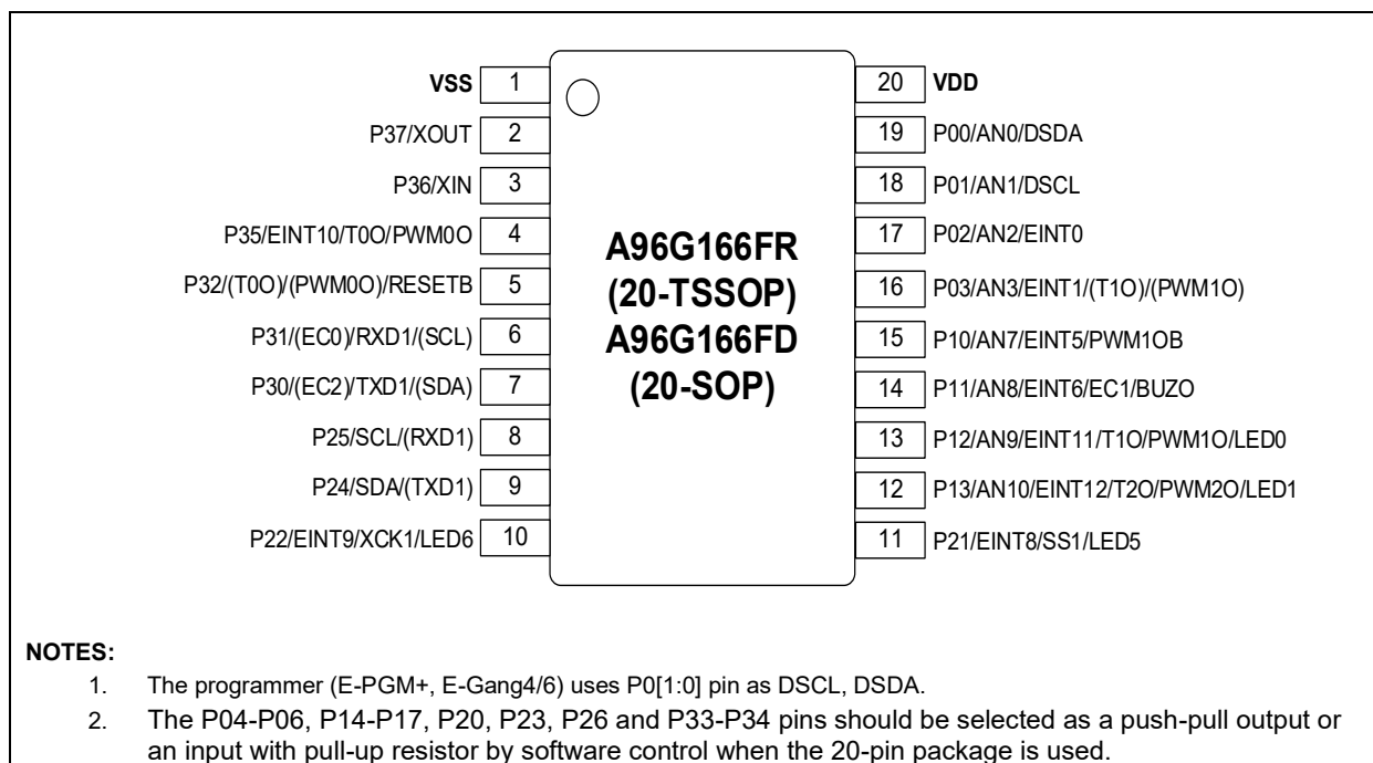
Figure 3. A96G166 20-TSSOP/20-SOP Pin Assignment
