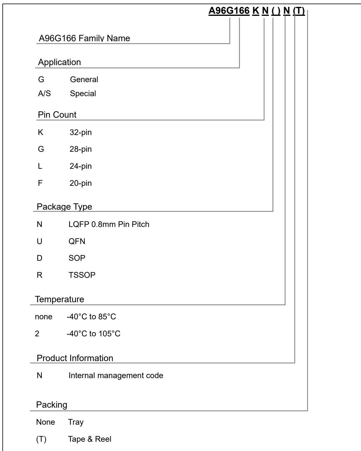
Figure 77. A96G166/A96A166/A96S166 Device Numbering Nomenclature
