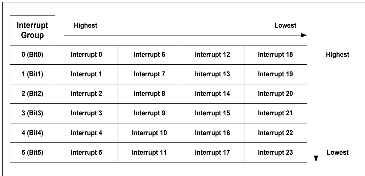
Figure 16. Interrupt Group Priority Level
