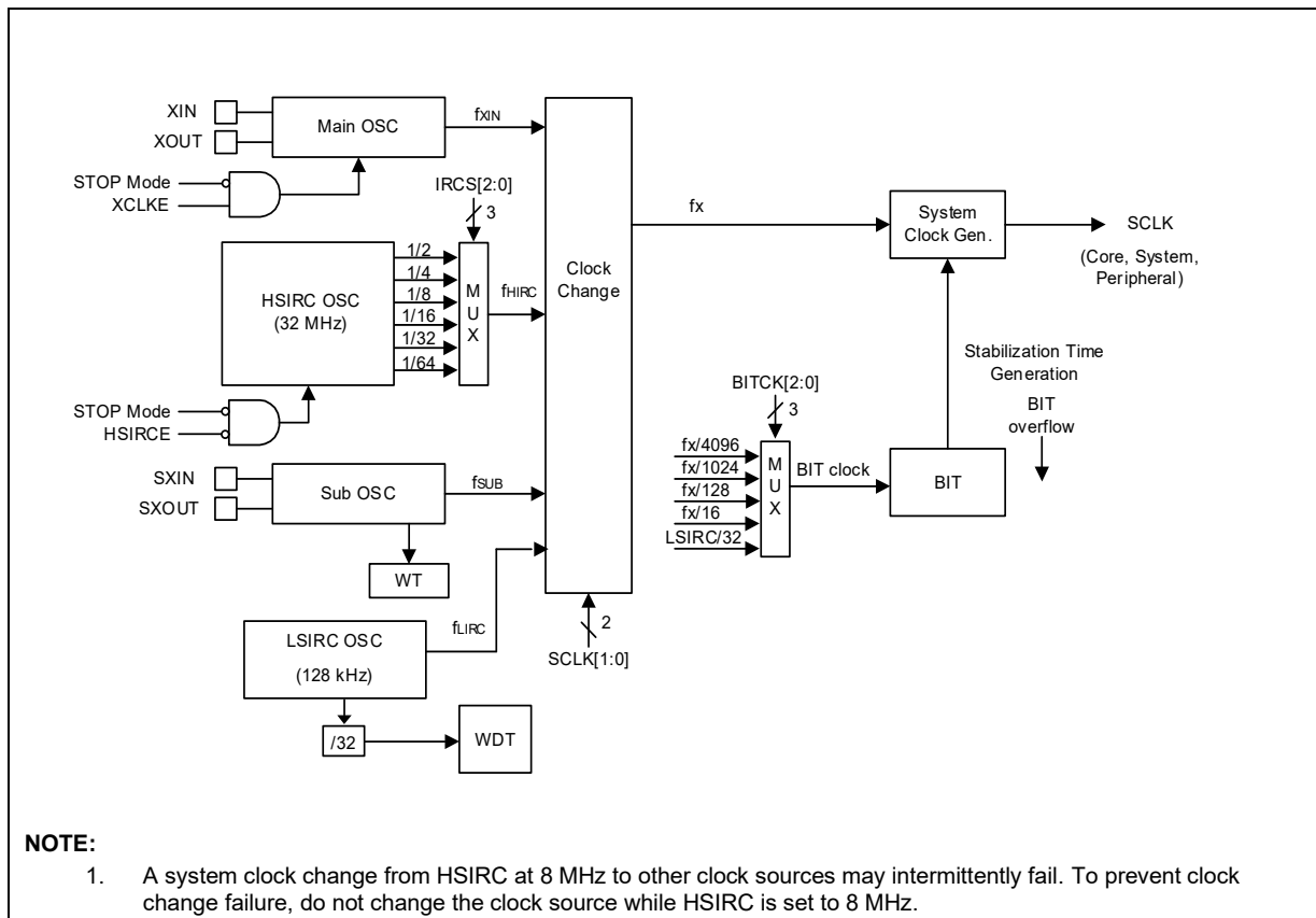
Figure 18. Clock Generator Block Diagram
