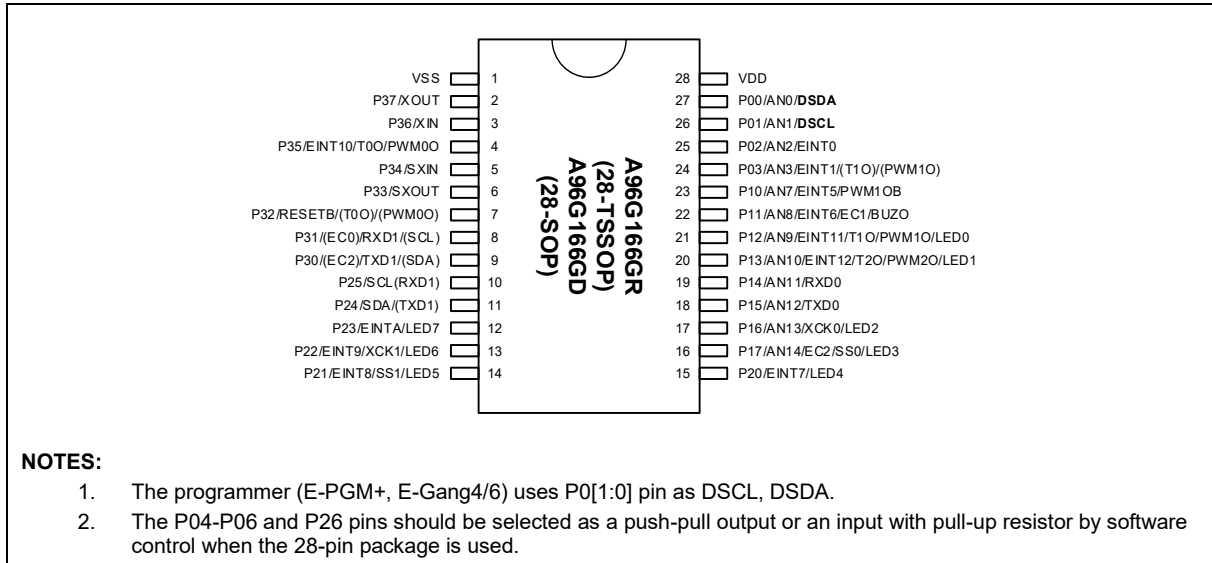
Figure 7. A96G166 28-TSSOP/28-SOP Pin Assignment
