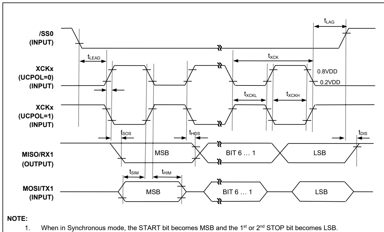
Figure 38. SPI/Synchronous Slave Mode Timing (UCPHA = 1, MSB First)
