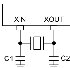
Figure 43. Crystal/Ceramic Oscillator
