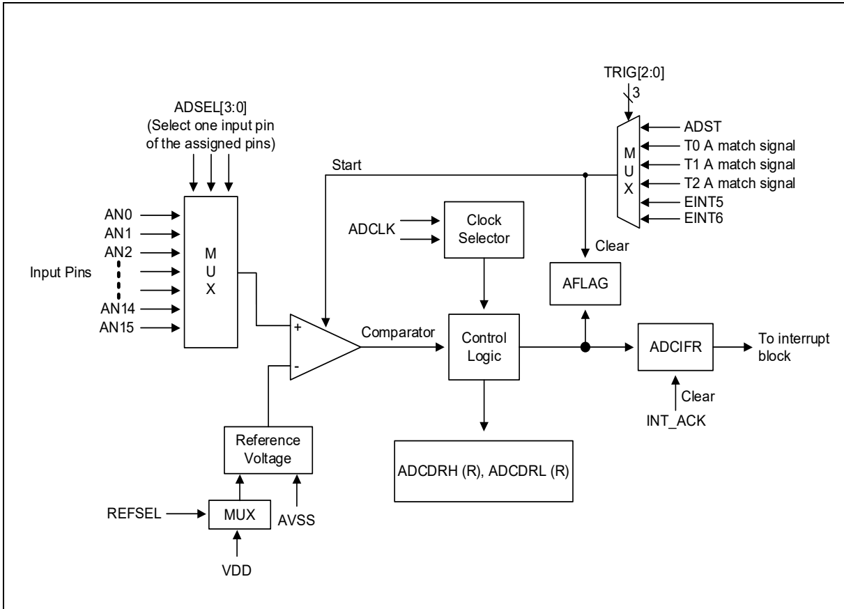
Figure 26. 12-bit ADC Block Diagram
