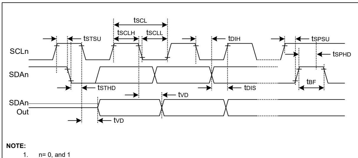
Figure 40. I2C Timing
