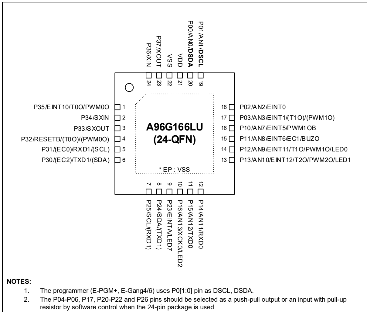
Figure 6. A96G166 24-QFN Pin Assignment
