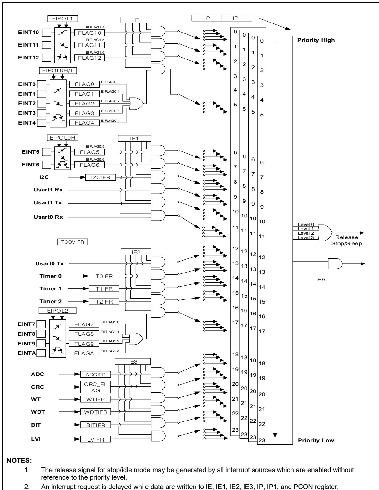
Figure 17. Interrupt Controller Block Diagram
