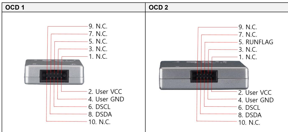
Figure 58. OCD 1 and OCD 2 Connector Pin Diagram
