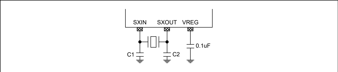
Figure 7-9. Crystal Oscillator
