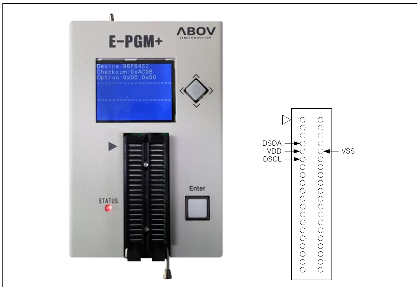
Figure 1-4. E-PGM+(Single Writer)
