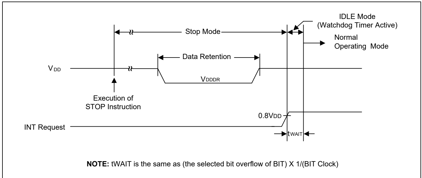
Figure 7-5. Stop Mode Release Timing When Initiated by Interrupts
