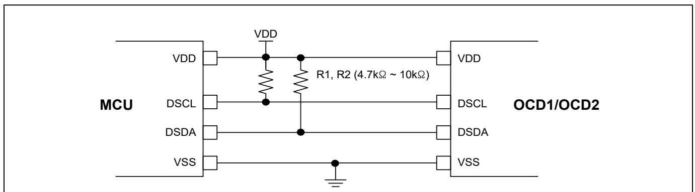
Figure 1-3. Recommended Circuit for Debugger(OCD1/OCD2) Connection
