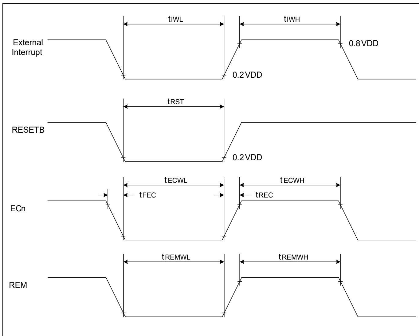
Figure 7-2. AC Timing
