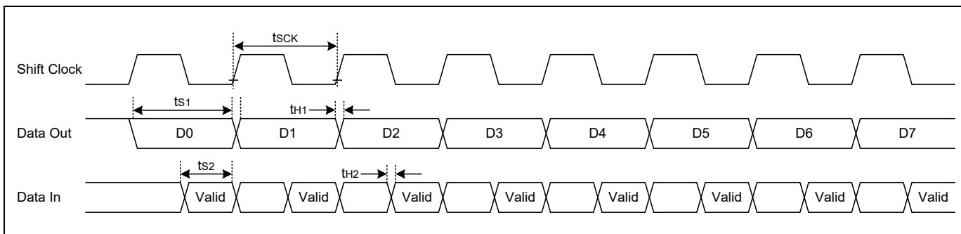
Figure 7-4. Timing Waveform for UART Module
