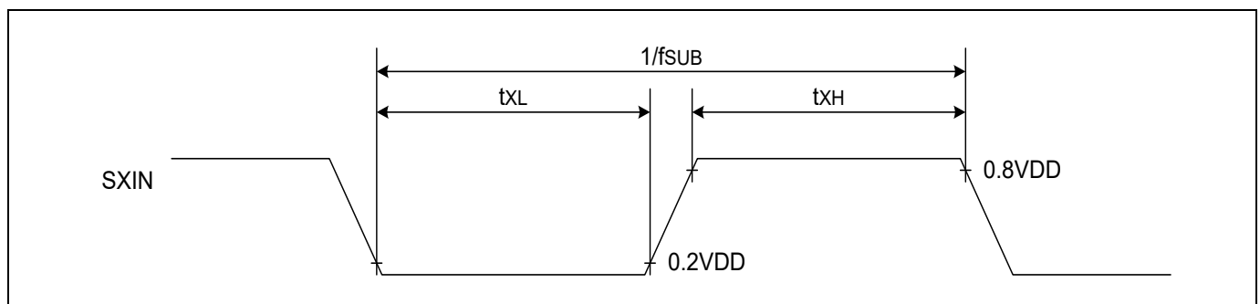
Figure 7-12. Clock Timing Measurement at SXIN
