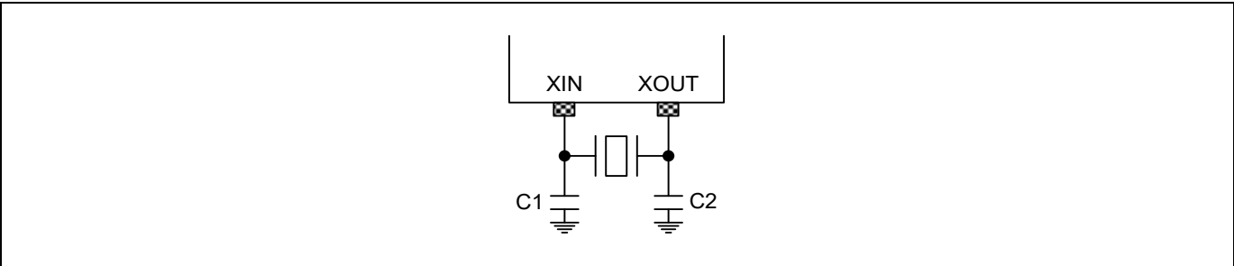
Figure 7-7. Crystal/Ceramic Oscillator
