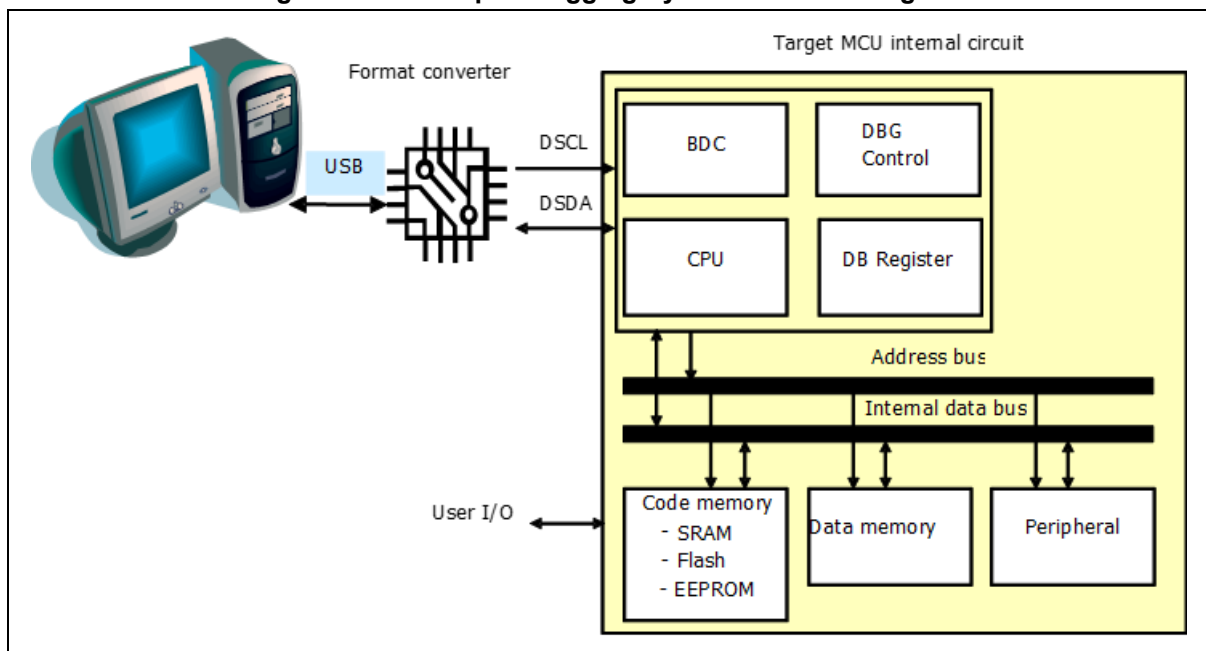
Figure 55. On-Chip Debugging System in Block Diagram
