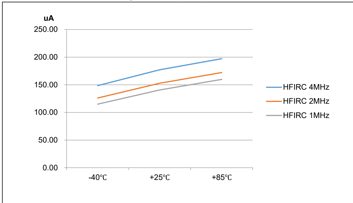
Figure 47. STOP (IDD5) Current
