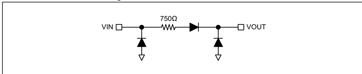
Figure 5. VIN and VOUT Port Structure
