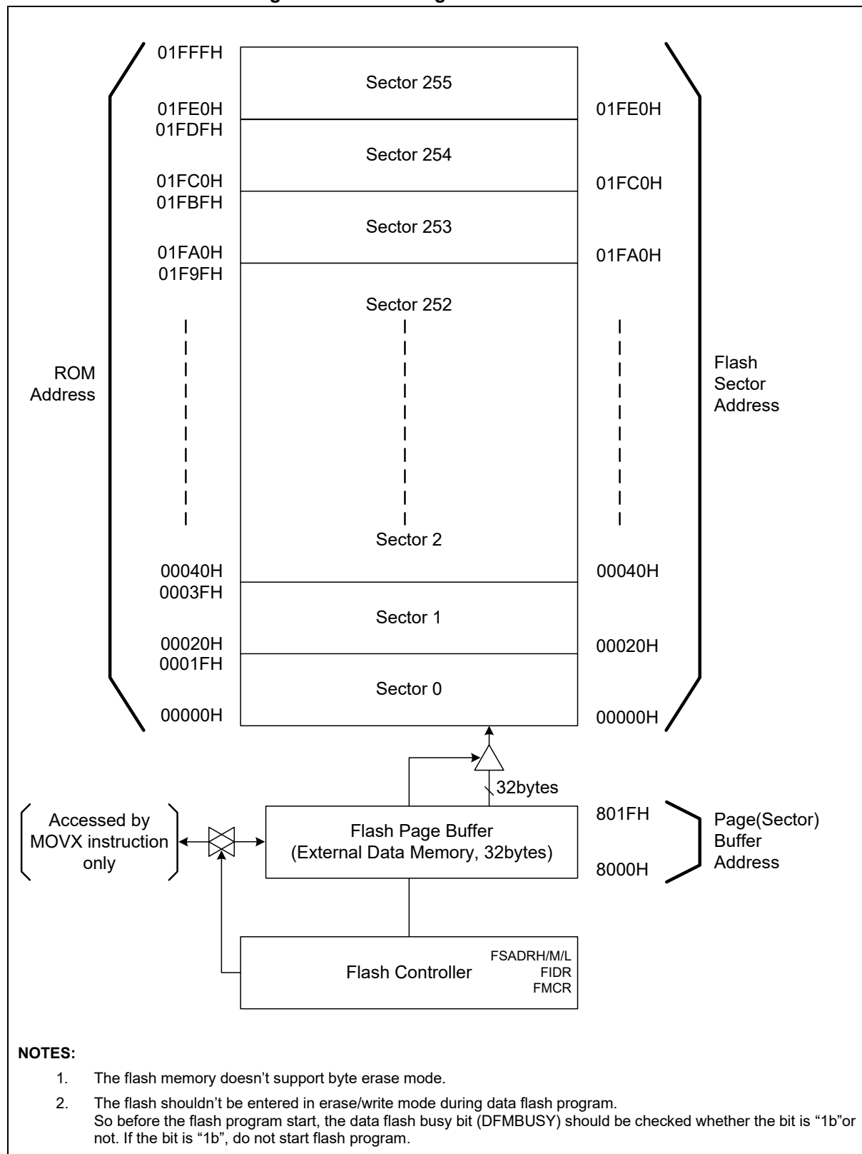
Figure 35. Flash Program ROM Structure
