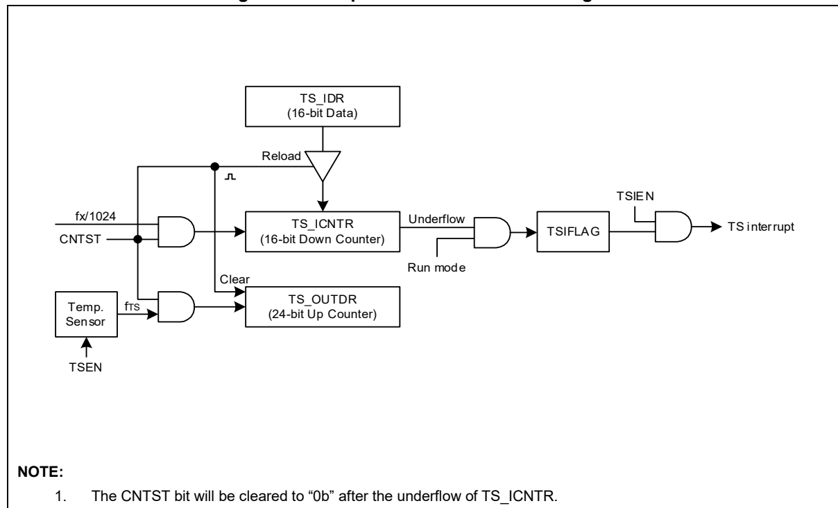
Figure 33. Temperature Sensor Block Diagram
