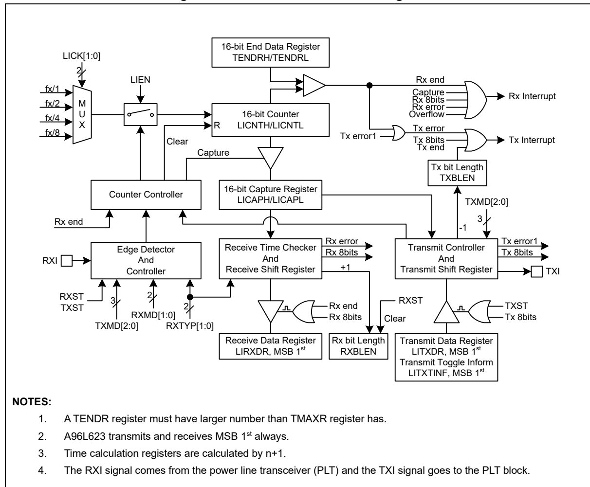
Figure 19. Line Interface in Block Diagram
