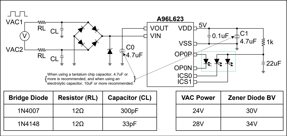
Figure 32. Application Circuit for PLT
