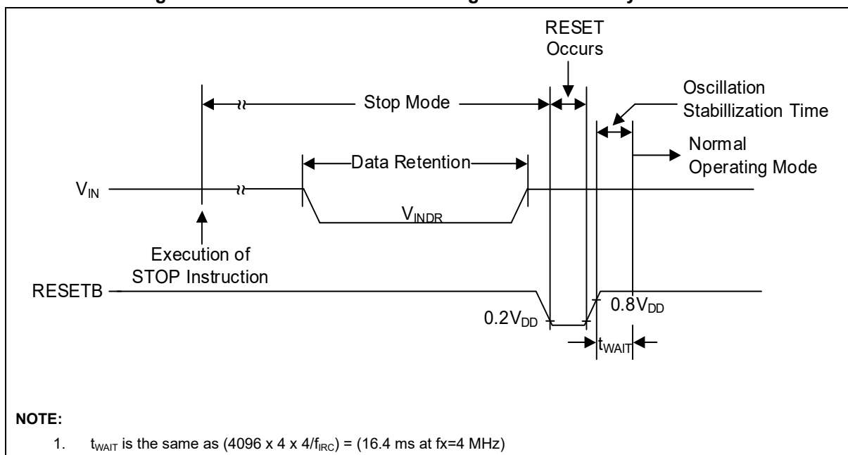
Figure 44. STOP Mode Release Timing when Initiated by RESETB
