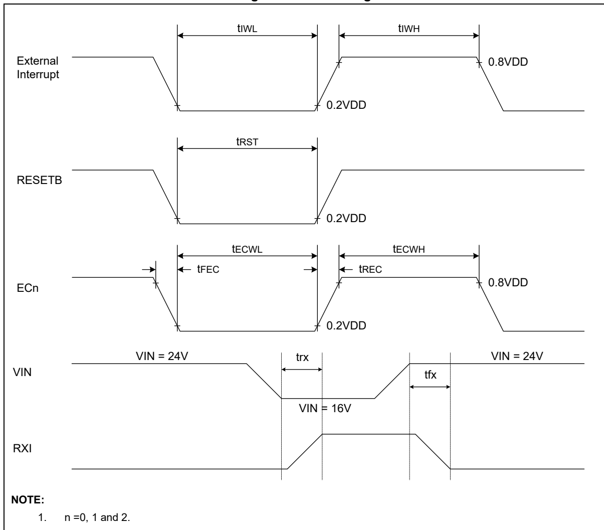
Figure 39. AC Timing
