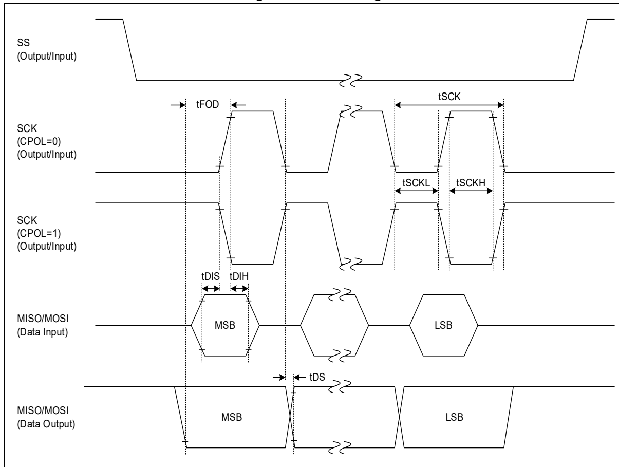
Figure 40. SPI Timing
