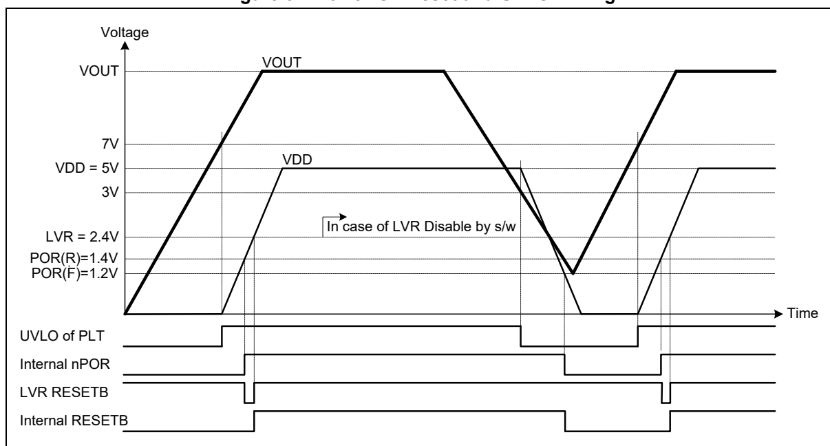
Figure 37. Power-On Reset and UVLO Timing
