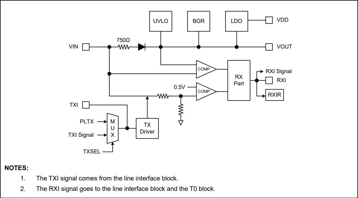
Figure 32. Application Circuit for PLT
