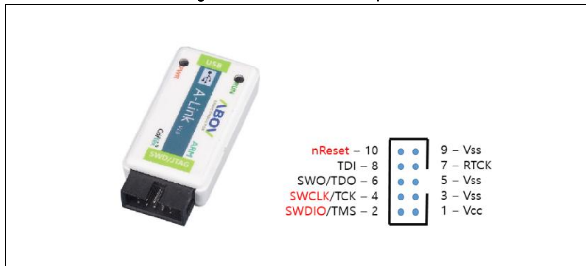
Figure 2. A-Link and Pin Description
