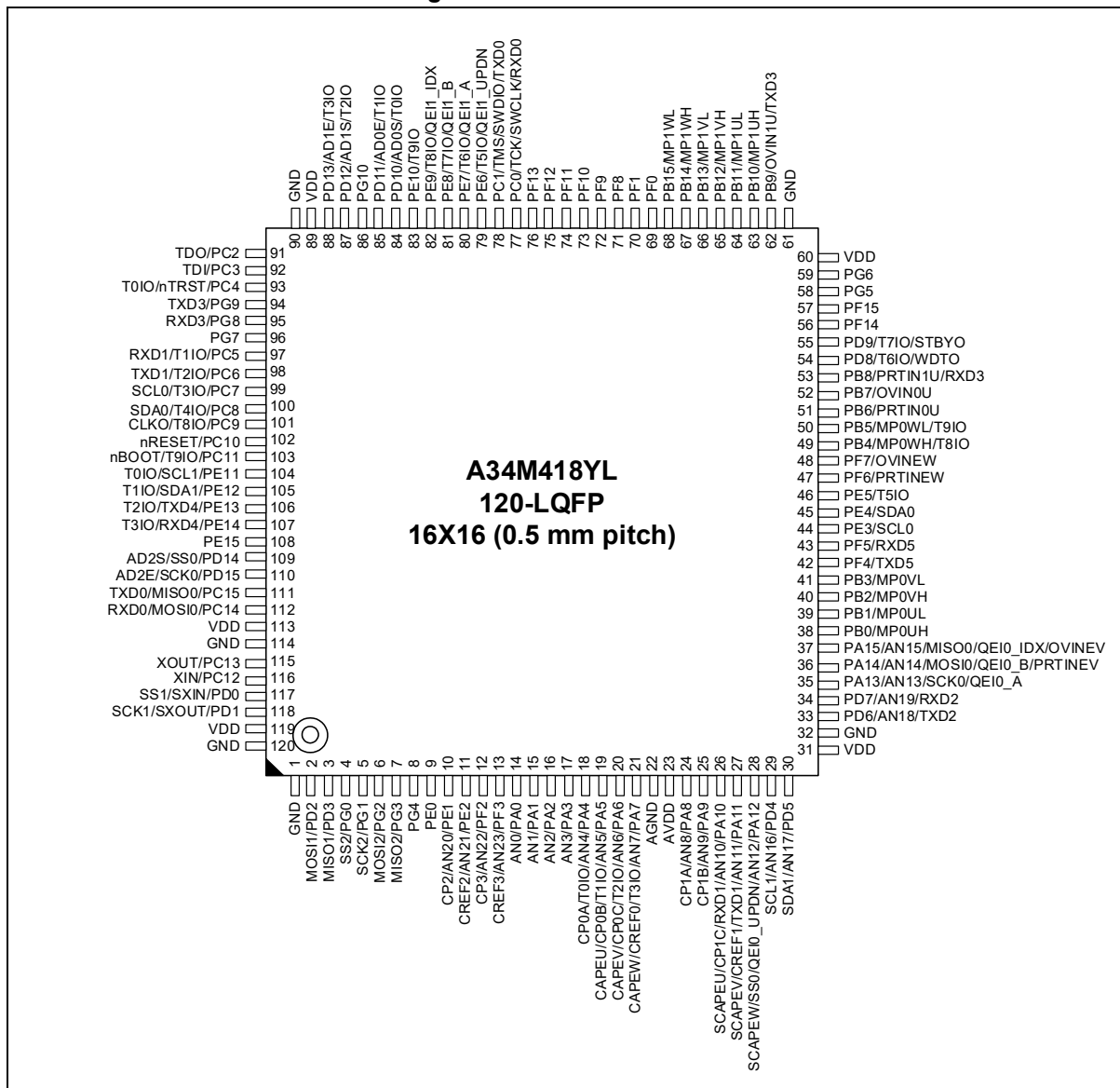
Figure 4. 120-LQFP Pinouts
