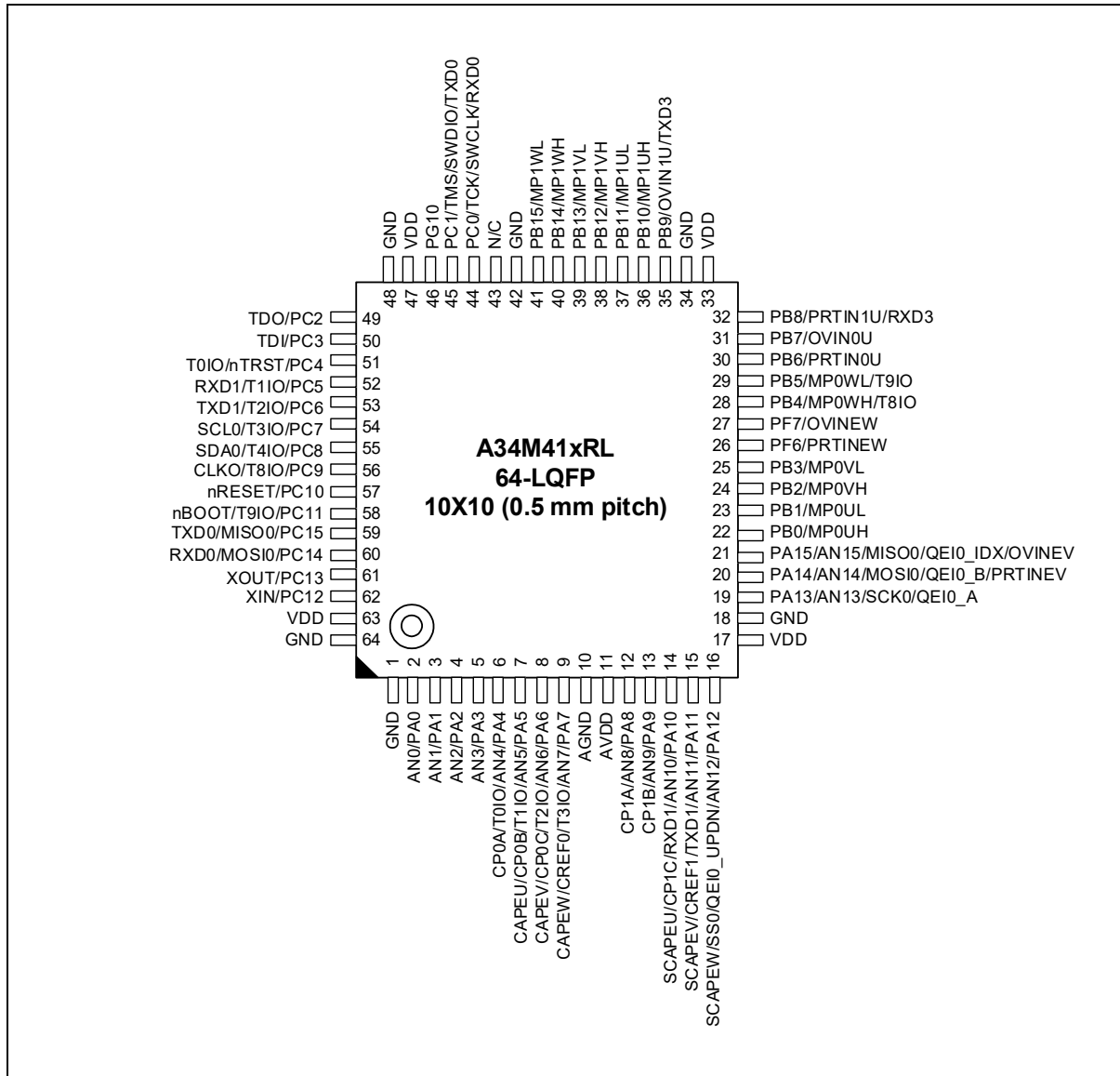
Figure 6. 64-LQFP Pinouts
