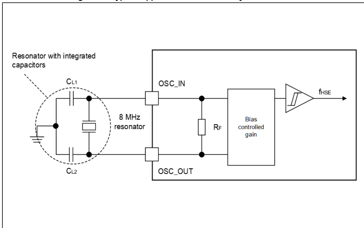
Figure 15. Typical Application with 8 MHz Crystal Oscillator
