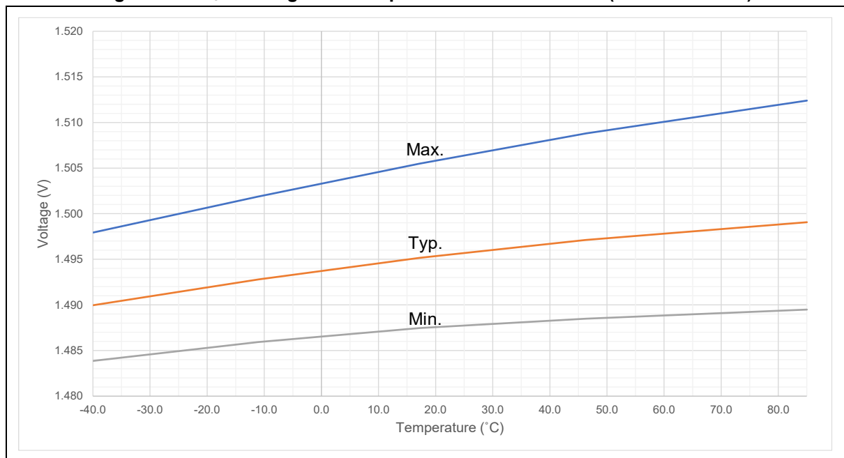
Figure 10. V CORE Voltage and Temperature Characteristics (-40°C to +85°C)
