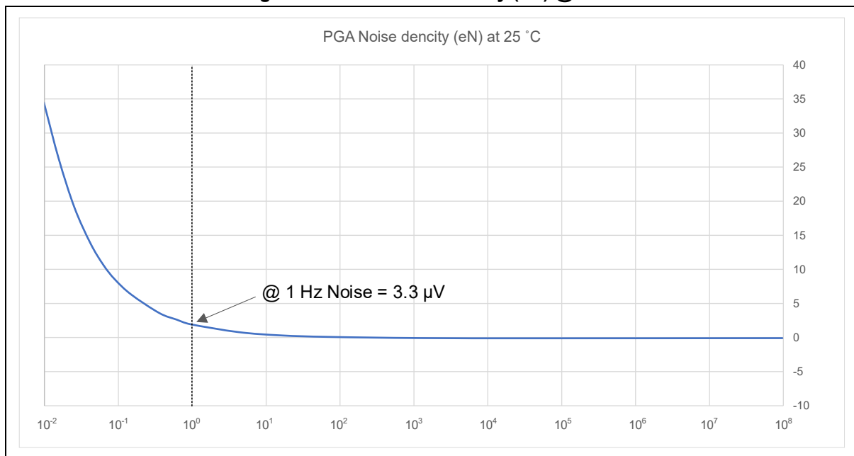
Figure 20. PGA Noise Density (eN) @ 25°C
