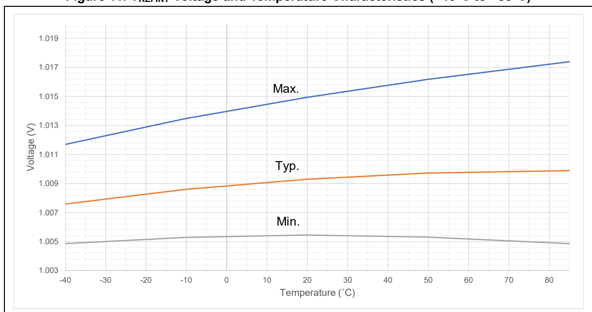
Figure 11. V REFINT Voltage and Temperature Characteristics (-40°C to +85°C)
