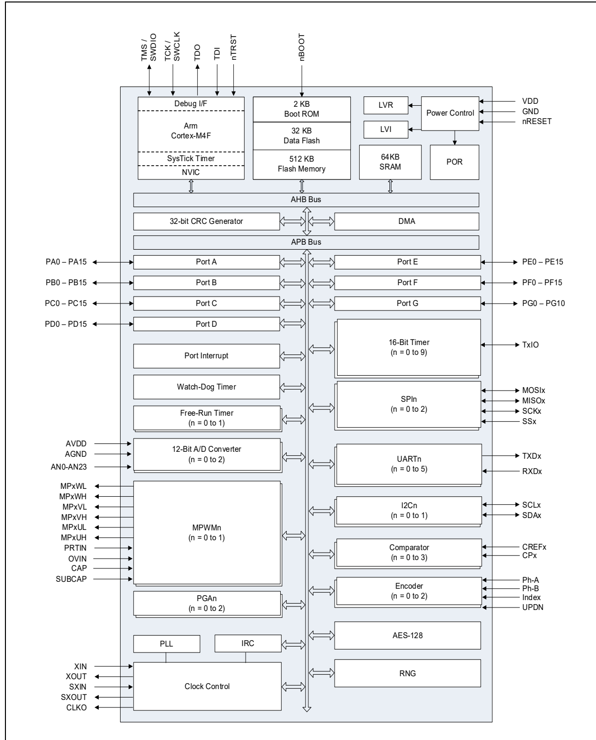
Figure 1. A34M41x Block Diagram
