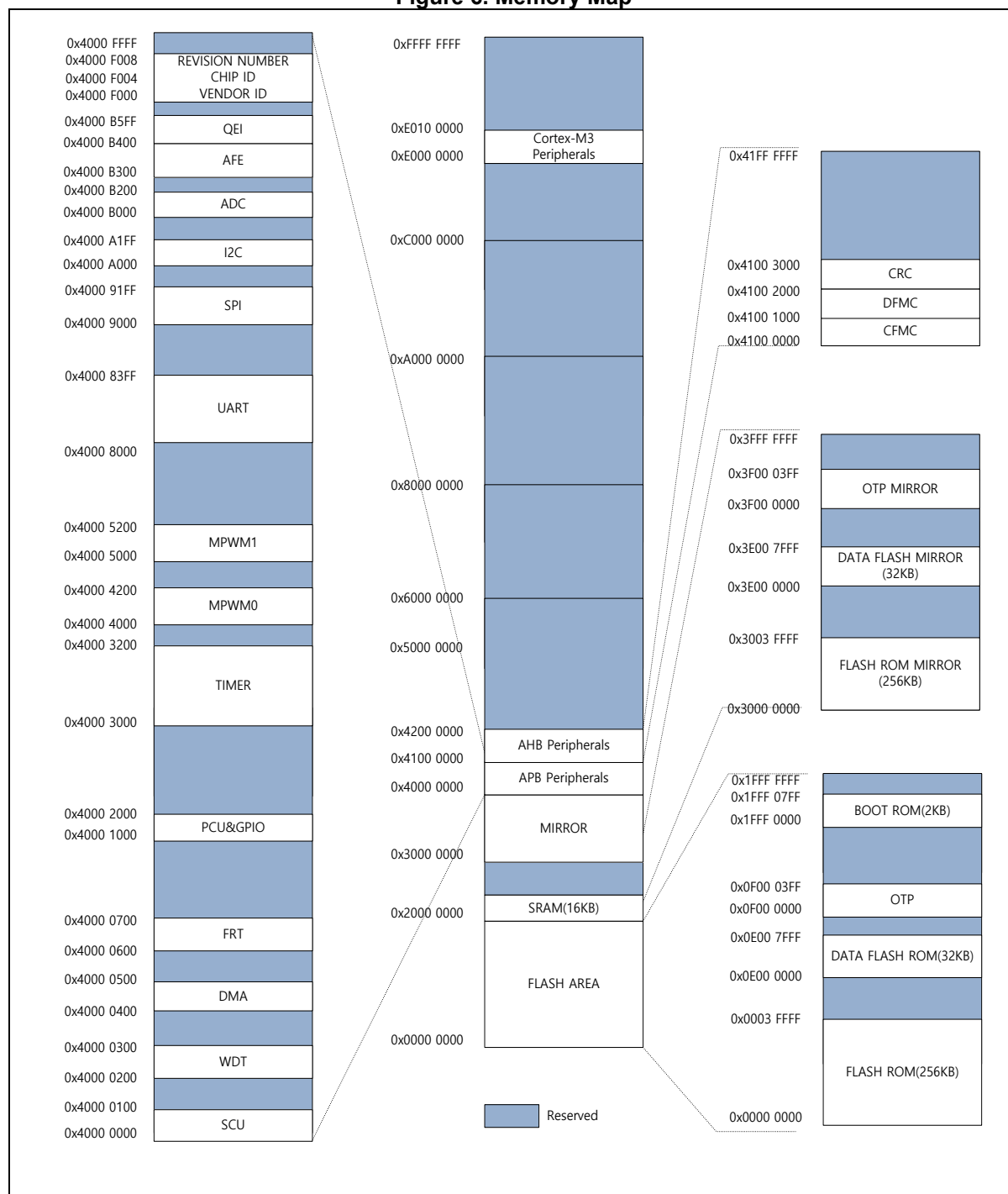
Figure 6. Memory Map
