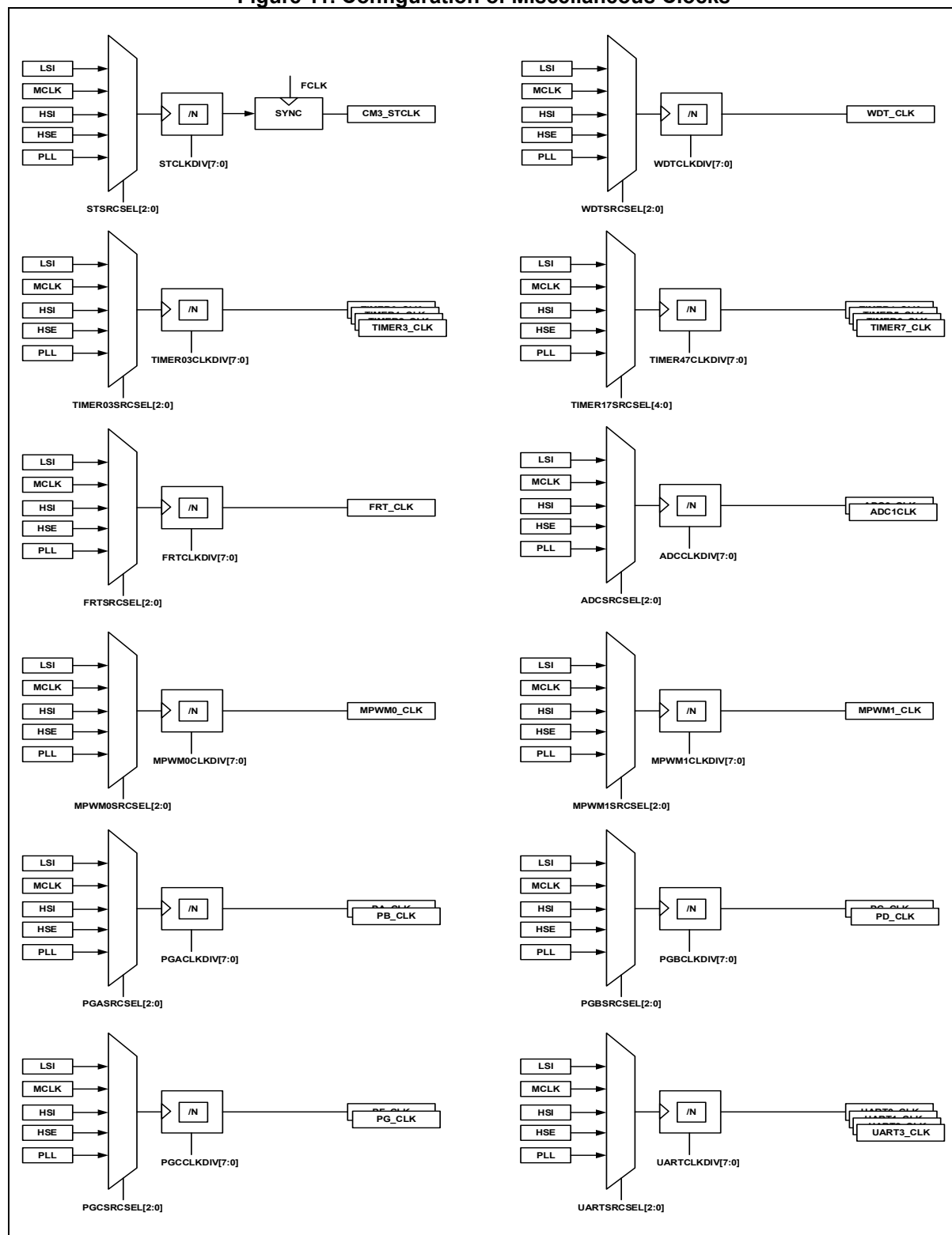
Figure 11. Configuration of Miscellaneous Clocks
