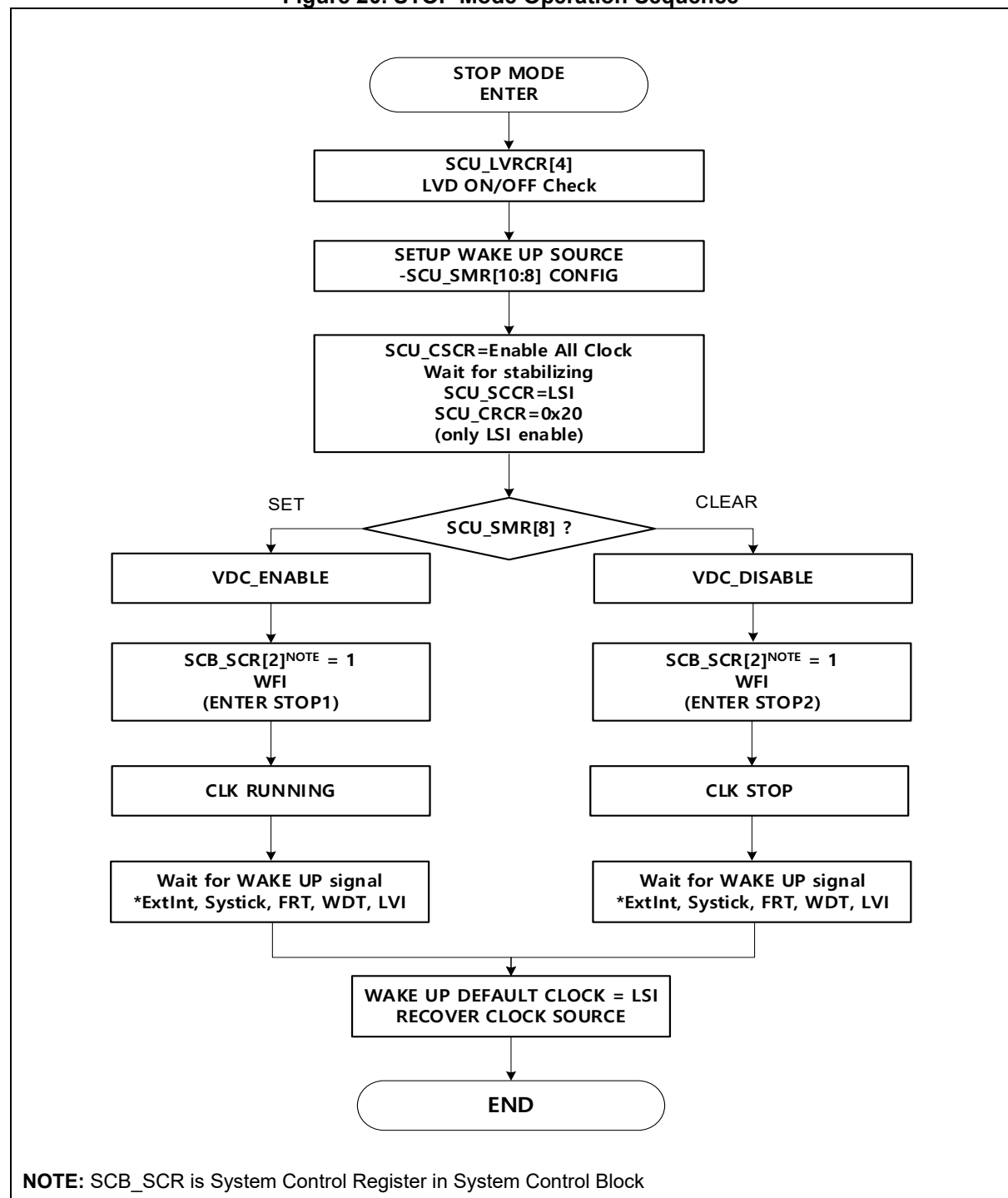
Figure 20. STOP Mode Operation Sequence
