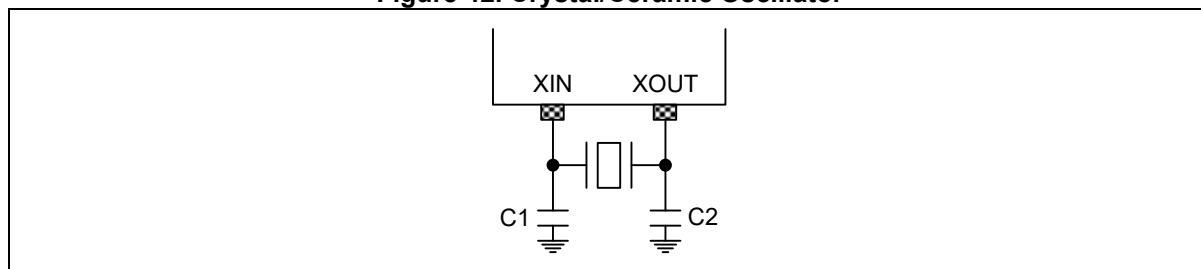
Figure 43. External Clock
