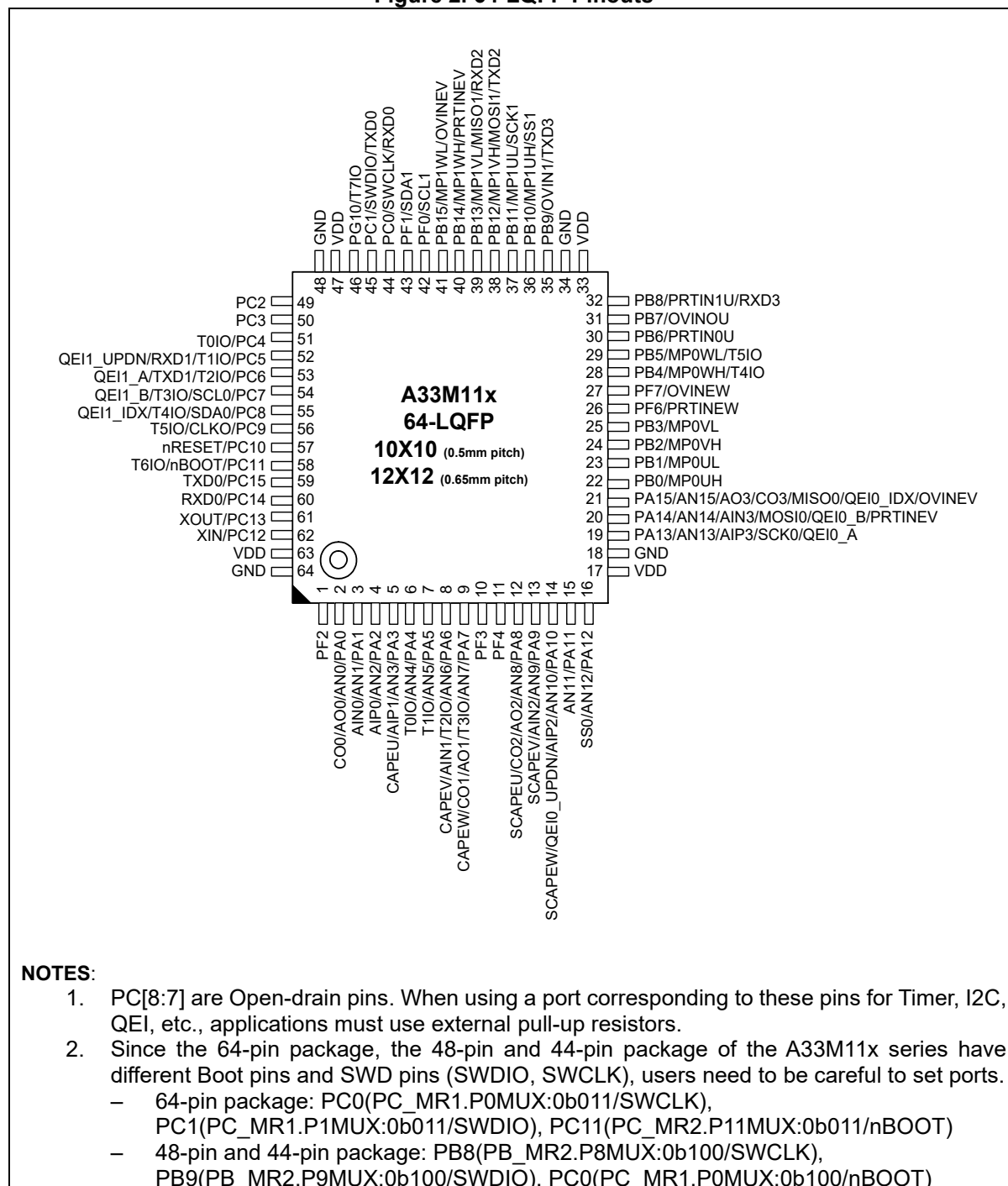
Figure 2. 64-LQFP Pinouts
