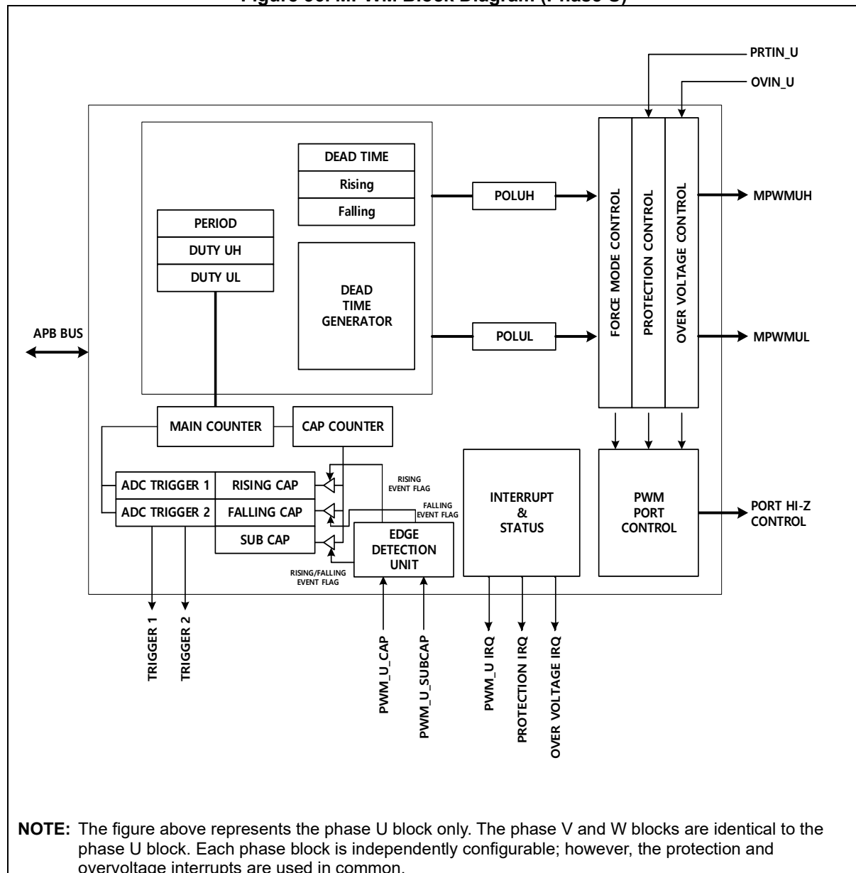
Figure 36. MPWM Block Diagram (Phase U)
