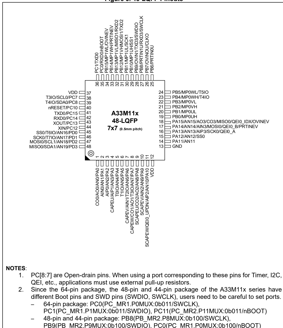
Figure 3. 48-LQFP Pinouts
