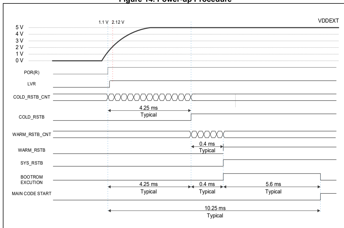
Figure 14. Power-up Procedure
