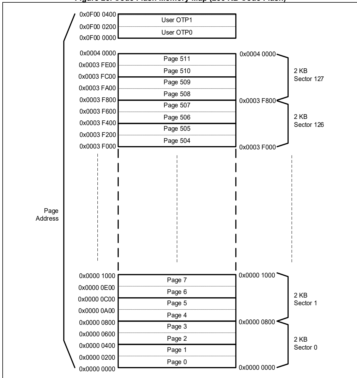
Figure 25. Code Flash Memory Map (256 KB Code Flash)
