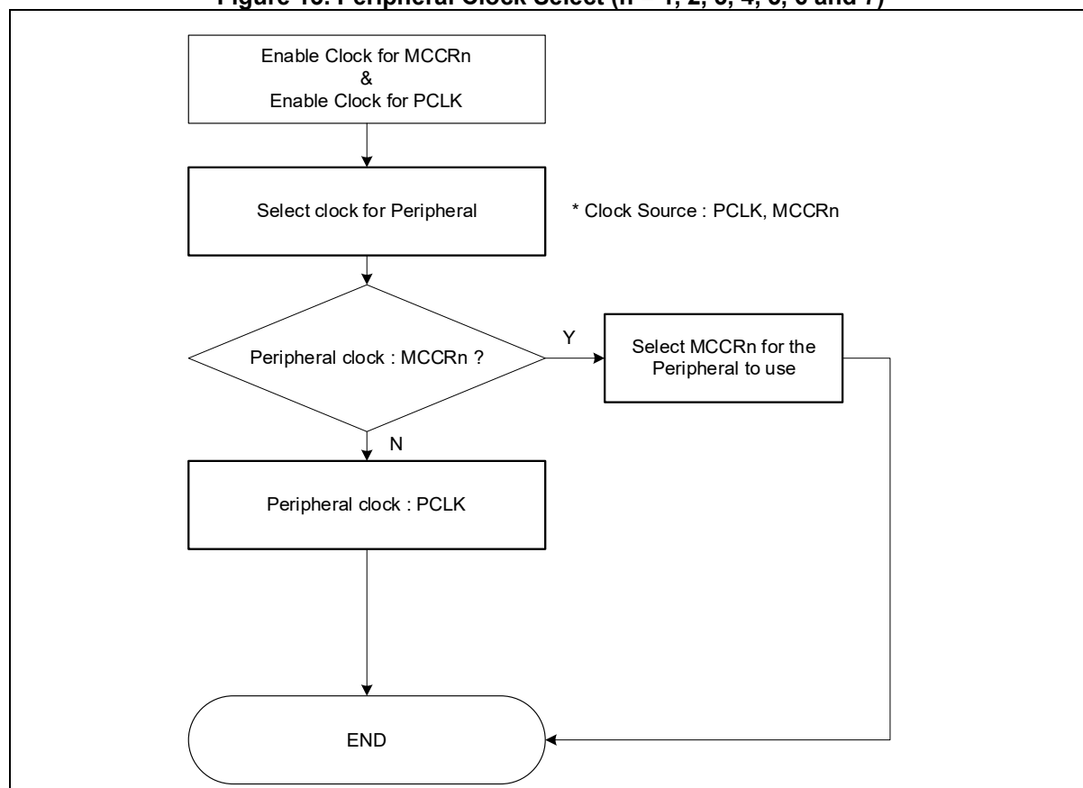
Figure 13. Peripheral Clock Select (n = 1, 2, 3, 4, 5, 6 and 7)
