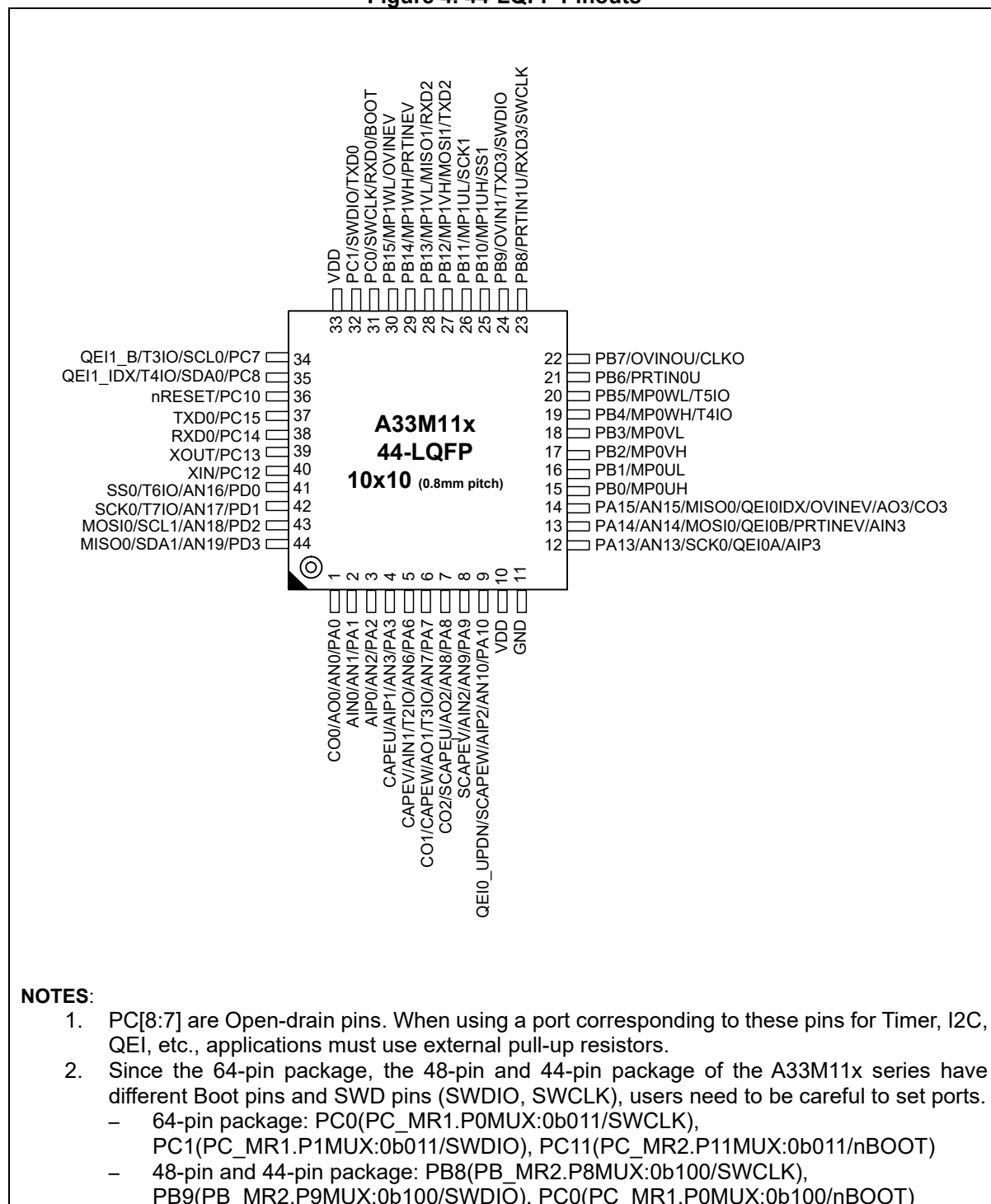
Figure 4. 44-LQFP Pinouts
