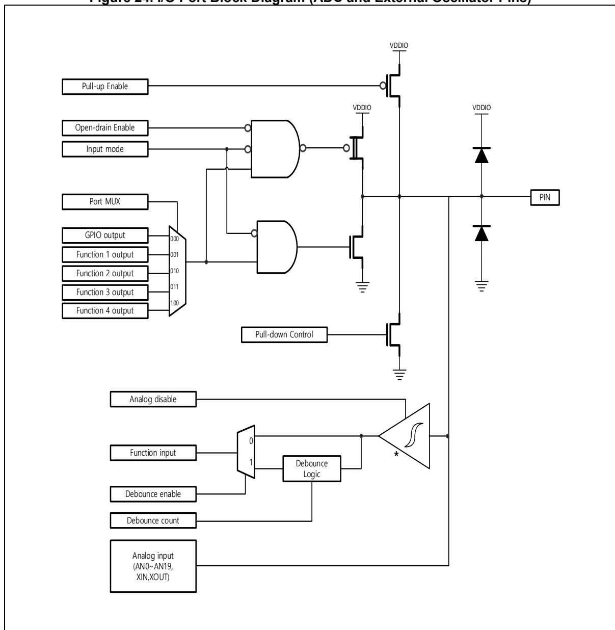
Figure 24. I/O Port Block Diagram (ADC and External Oscillator Pins)
