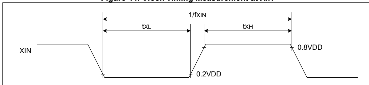
Figure 44. Clock Timing Measurement at XIN
