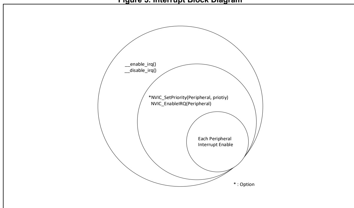
Figure 5. Interrupt Block Diagram
