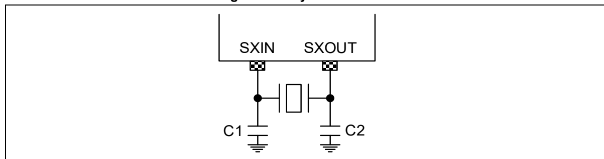
Figure 16. Crystal Oscillator
