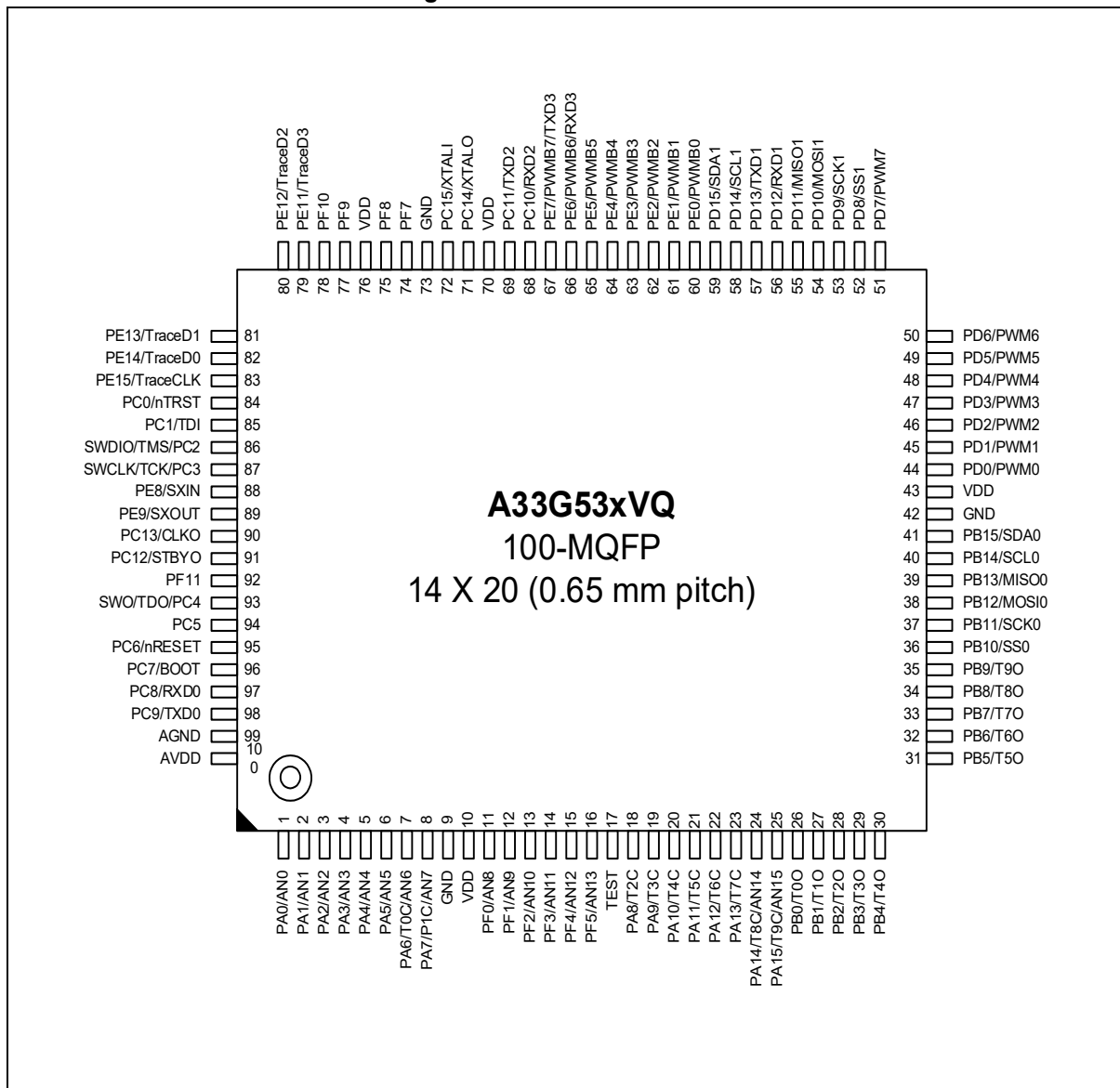
Figure 4. 100-MQFP Pinouts
