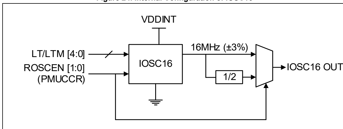
Figure 24. Internal Configuration of IOSC16
