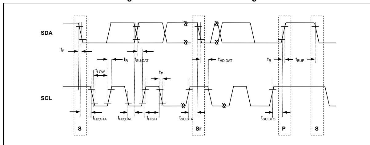
Figure 19. I2C Interface Bus Timing
