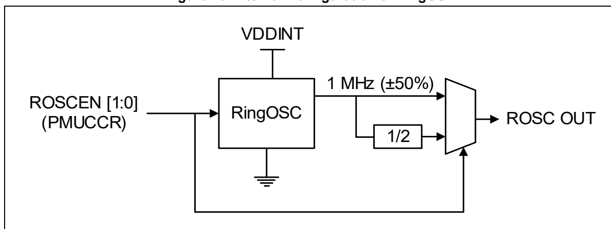
Figure 23. Internal Configuration of RingOSC
