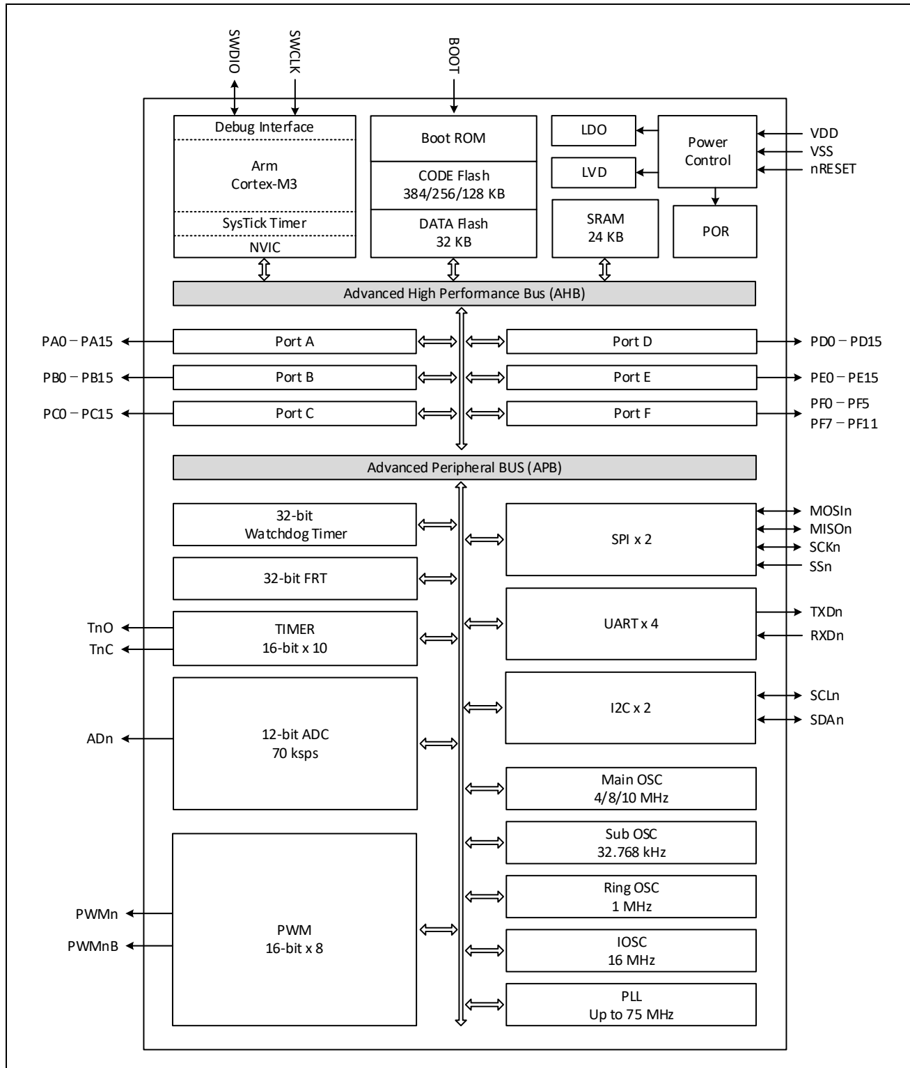
Figure 1.2. Internal block diagram of A33G52x microcontroller
