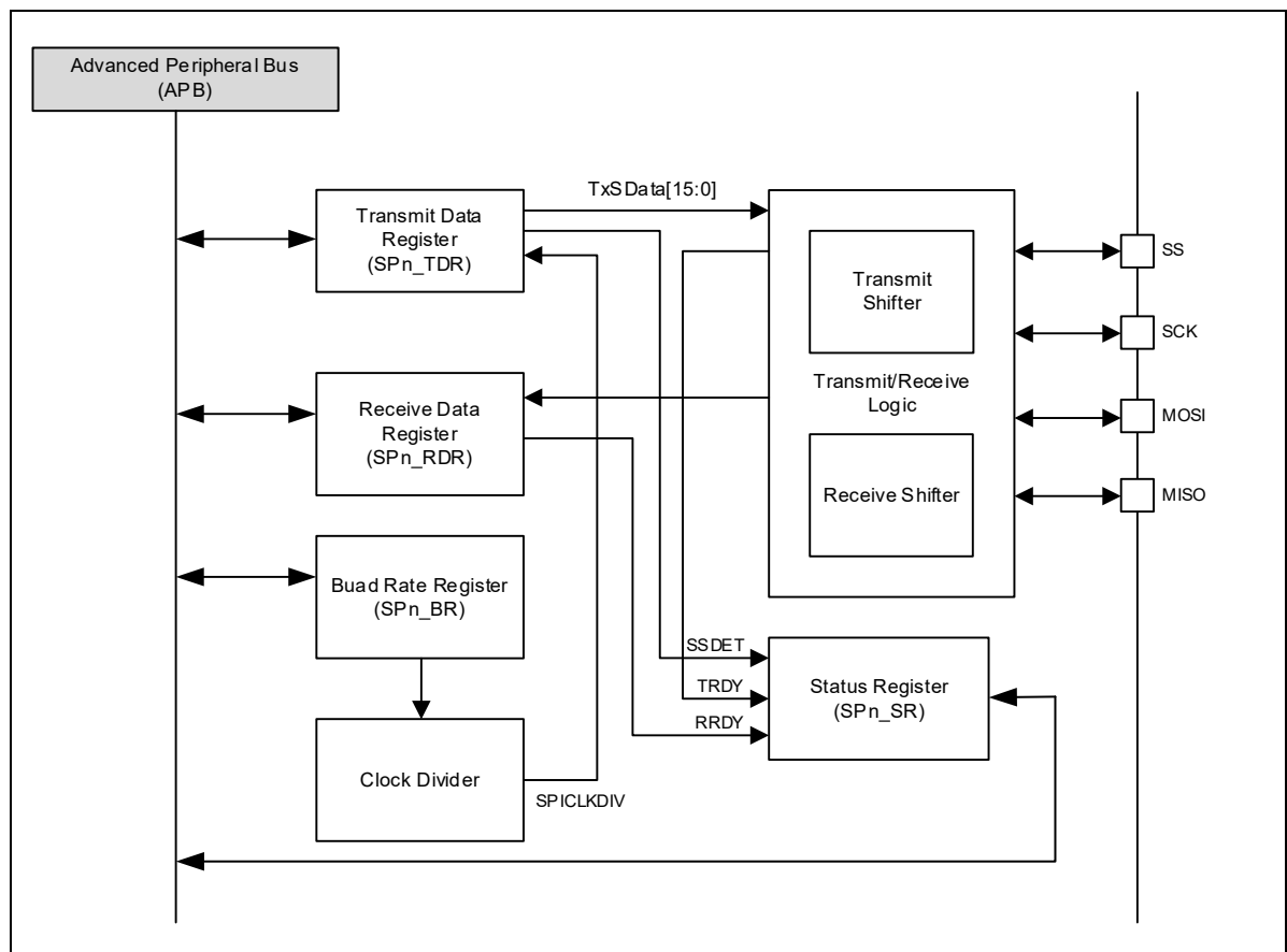
Figure 12.1. Block diagram of SPI
