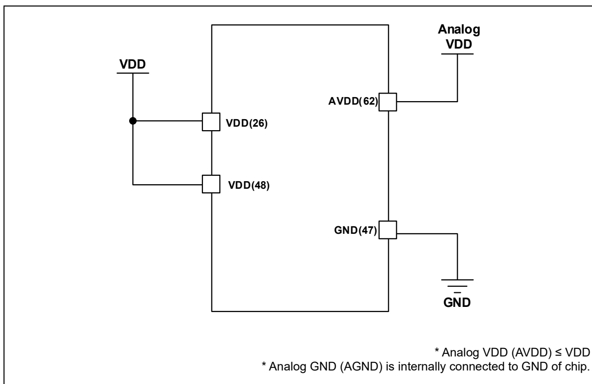
Figure 16.14. Power configuration of (64-LQFP-12/ 64-LQFP-10)
