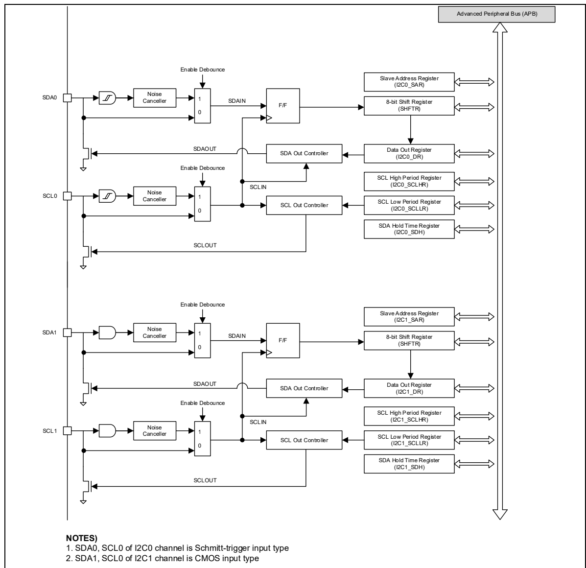
Figure 10.1. Block diagram of I2C interface
