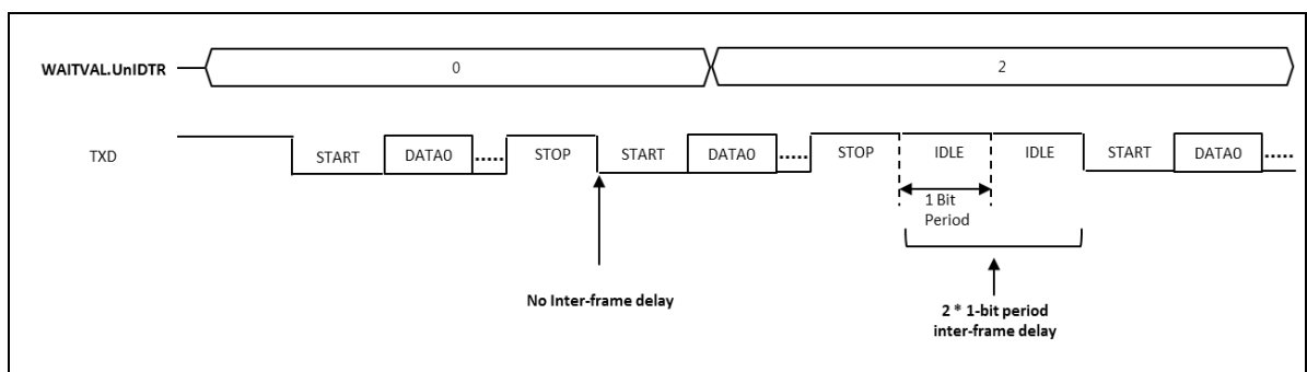
Figure 11.8. Timing diagram of inter-frame delay transmission
