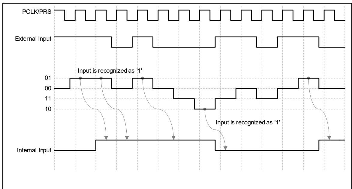
Figure 4.10. Timing of debounce function
