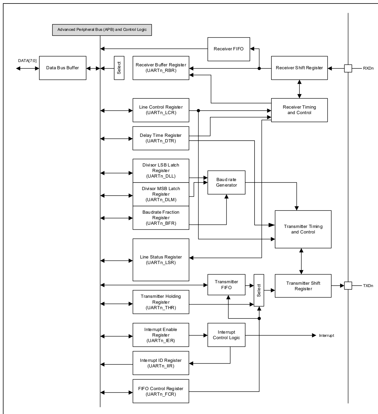
Figure 11.1. Block diagram of UART
