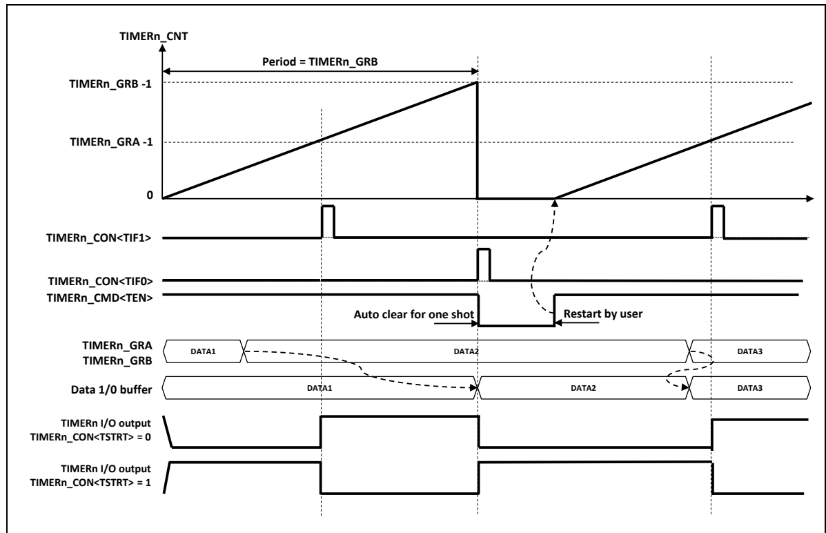
Figure 8.4. One-shot mode operation of 16-bit timer
