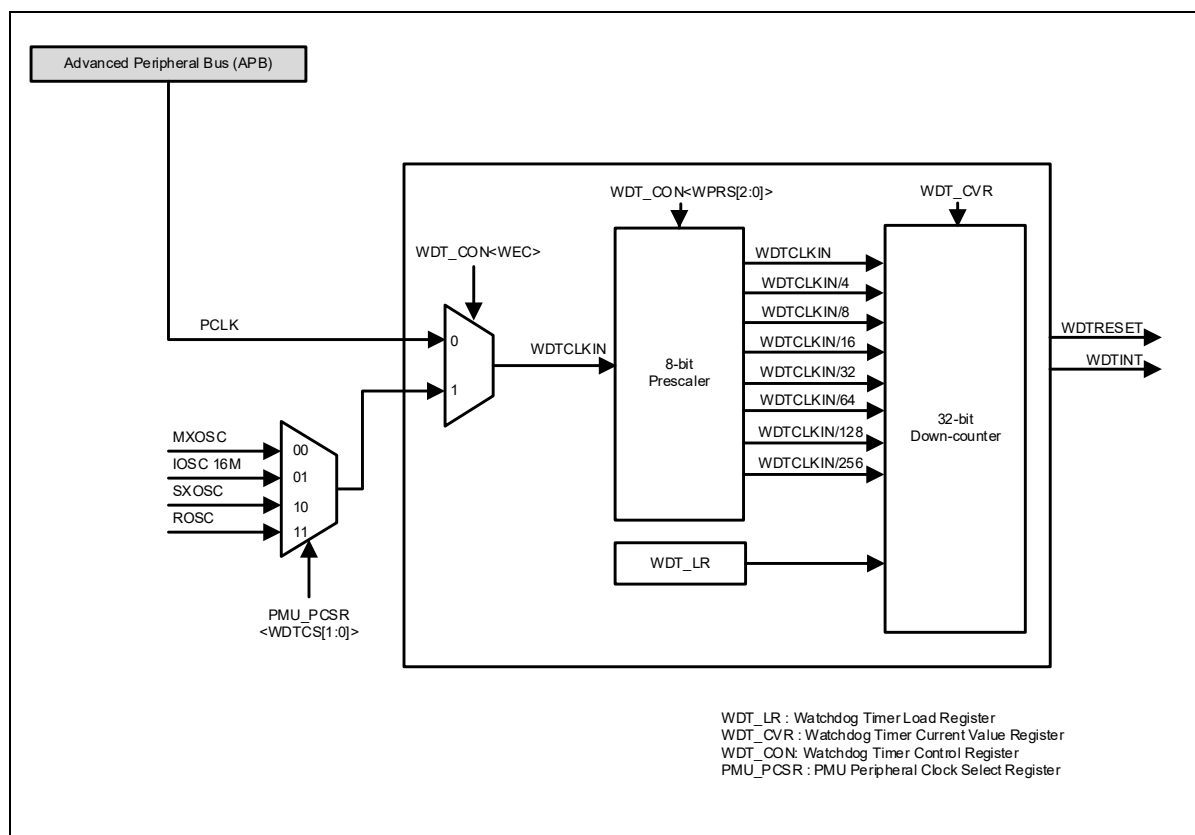
Figure 6.1. Block diagram of WDT
