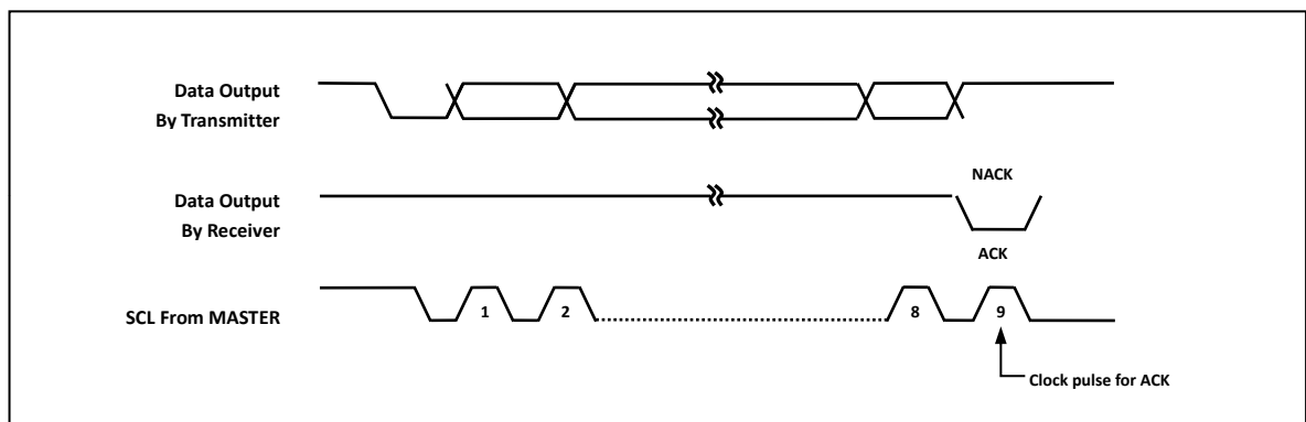
Figure 10.5. Acknowledge on I 2 C bus
