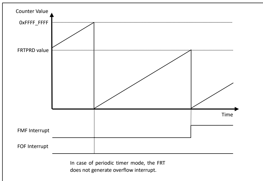
Figure 7.4. Operating example in periodic mode-2
