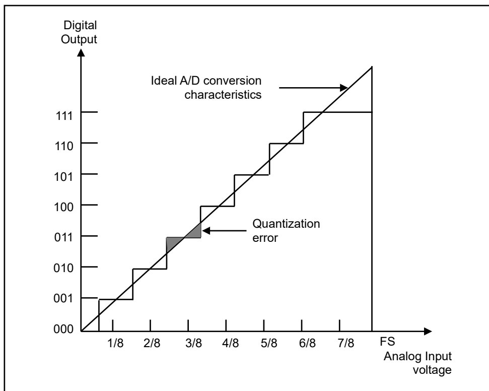
Figure 13.3. Definition of A/D conversion resolution (1)
