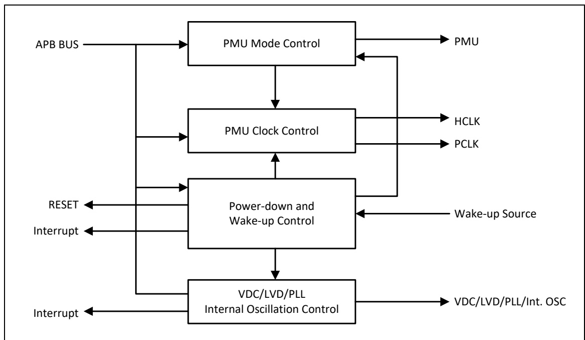
Figure 3.1. Block diagram of PMU
