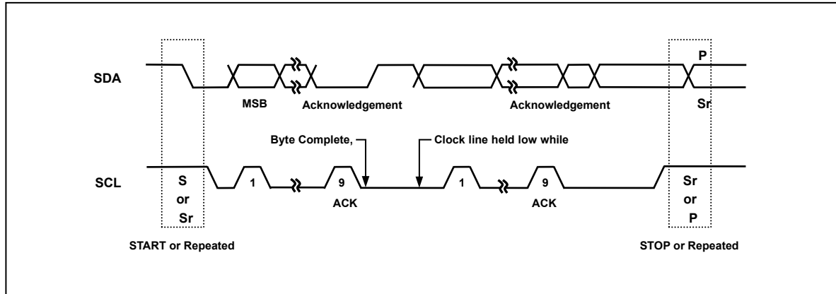
Figure 10.4. Data transfer on I 2 C bus
