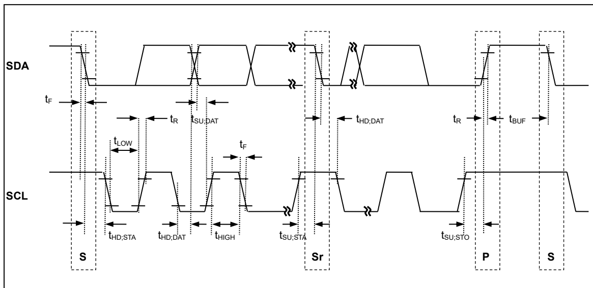
Figure 16.3. Timing of I2C interface bus
