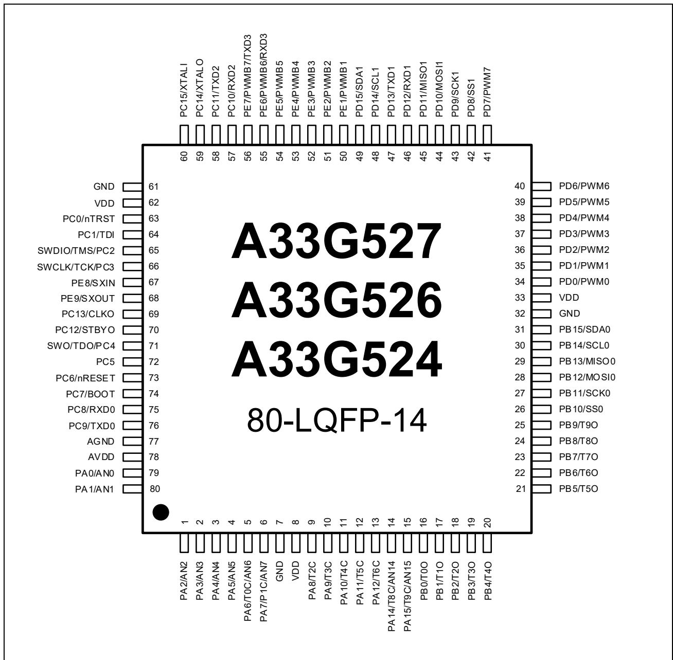
Figure 1.5. Pin layout of A33G527MM / A33G526MM / A33G524MM (80-LQFP-14)
