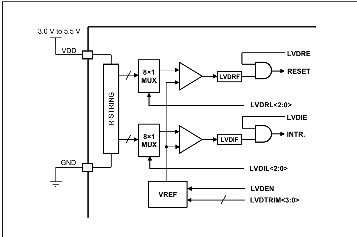
Figure 16.6. Internal configuration of LVDs
