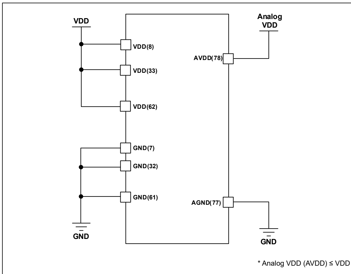
Figure 16.13. Power configuration of (80-LQFP-14/ 80-LQFP-12)
