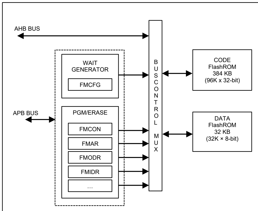
Figure 14.1. Block diagram of FMC (flash memory controller)
