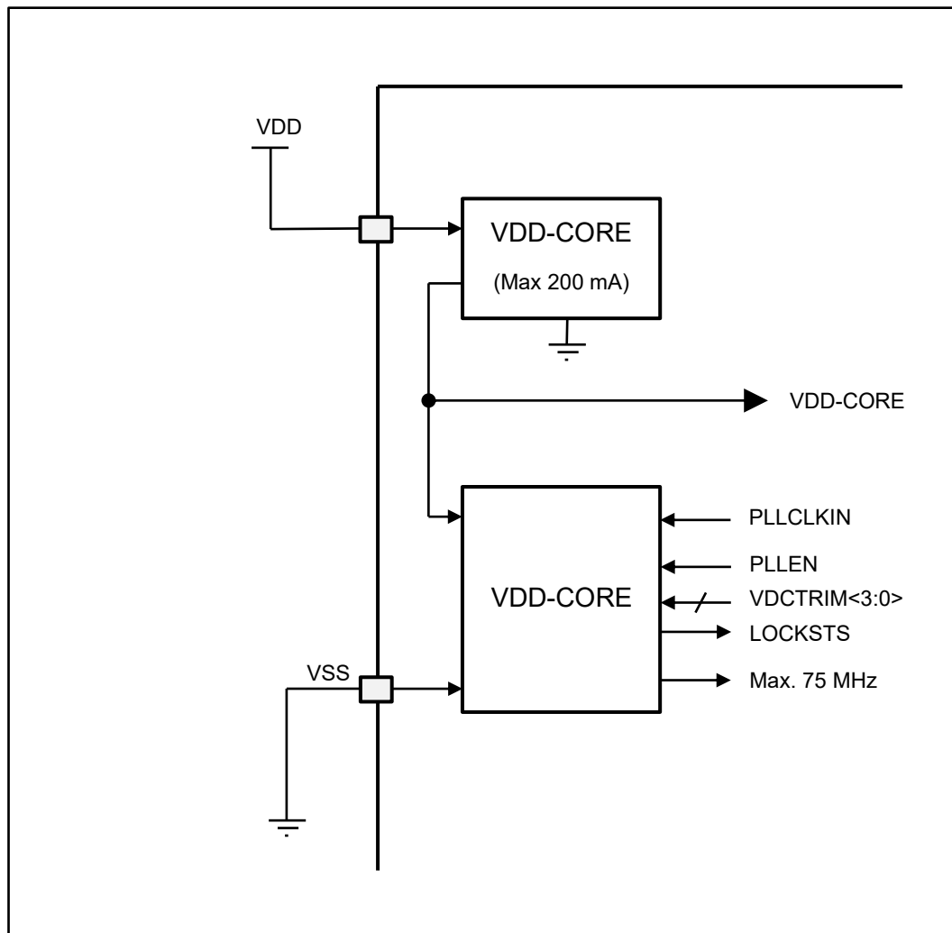
Figure 16.9. Configuration of PLL
