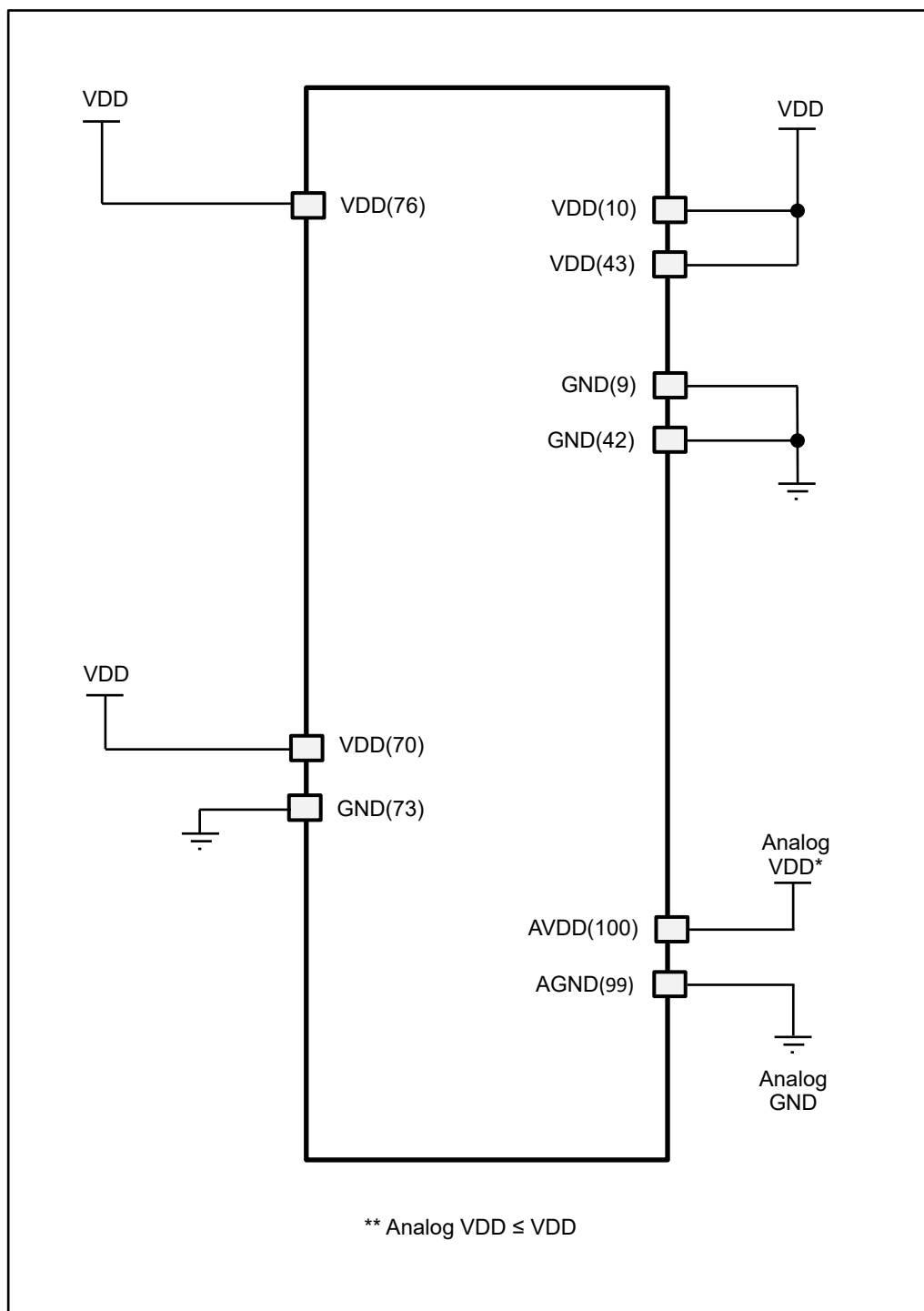
Figure 16.11. Power configuration of A33G52x (100-MQFP)
