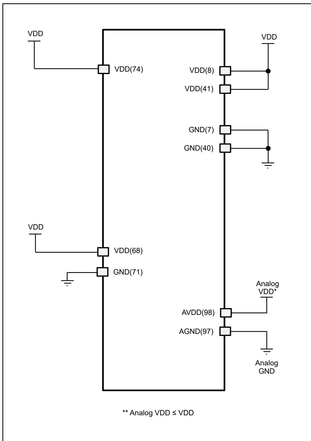
Figure 16.12. Power configuration of A33G52x (100-LQFP-14)
