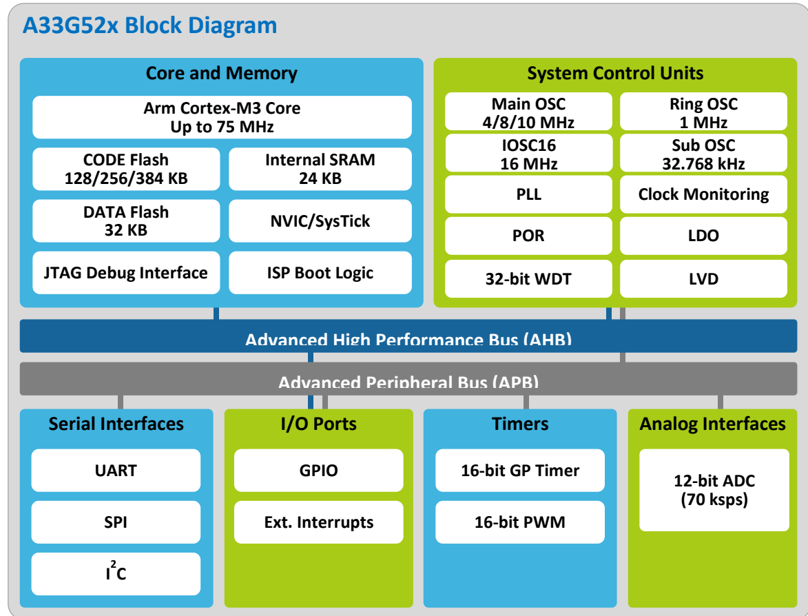
Figure 1.1. Block diagram of A33G52x series microcontroller
