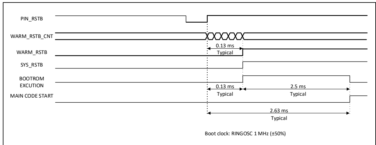
Figure 3.7. Warm reset timing of A33G52x
