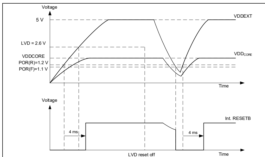
Figure 16.1. Reset timing
