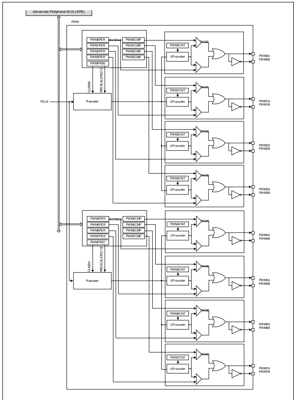
Figure 9.1. Block diagram of PWM
