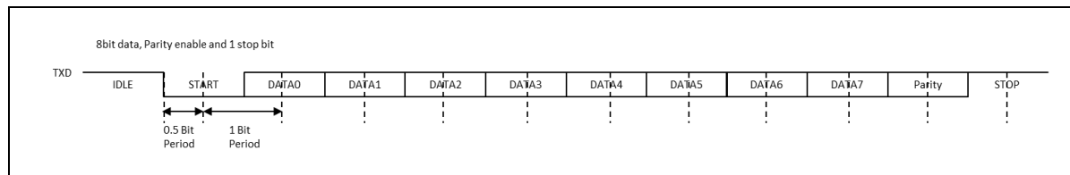
Figure 11.4. Example of transmit data format
