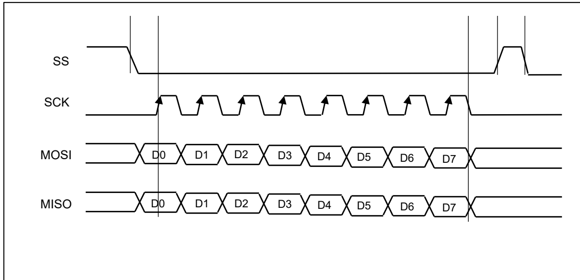
Figure 12.2. SPI timing diagram of SPI (CPHA=0, CPOL=0, MSBF=0)
