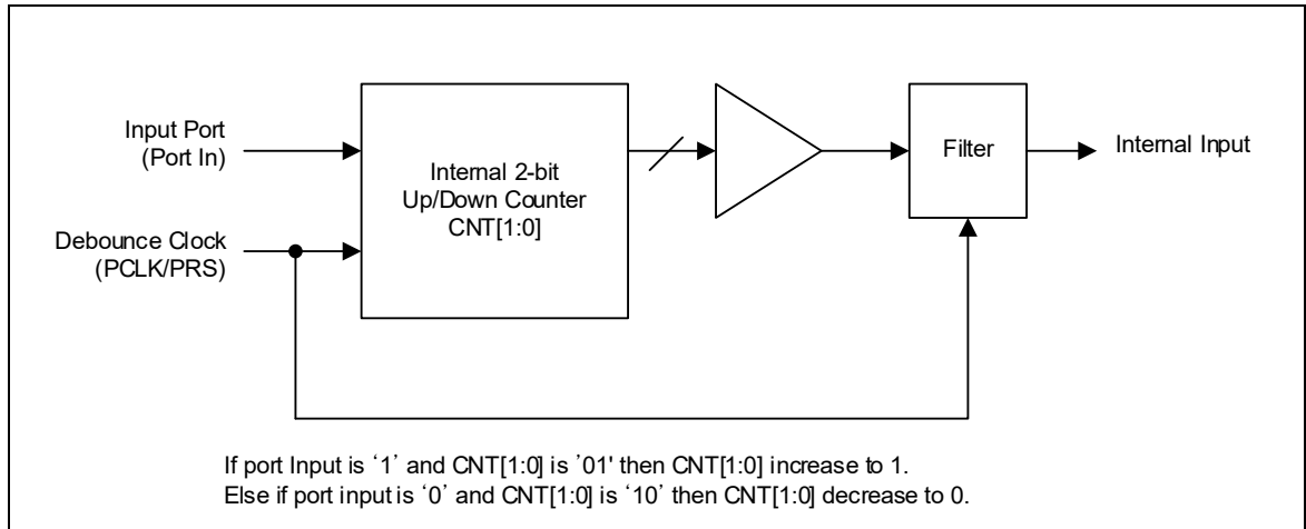
Figure 4.9. Simplified block diagram of debounce port
