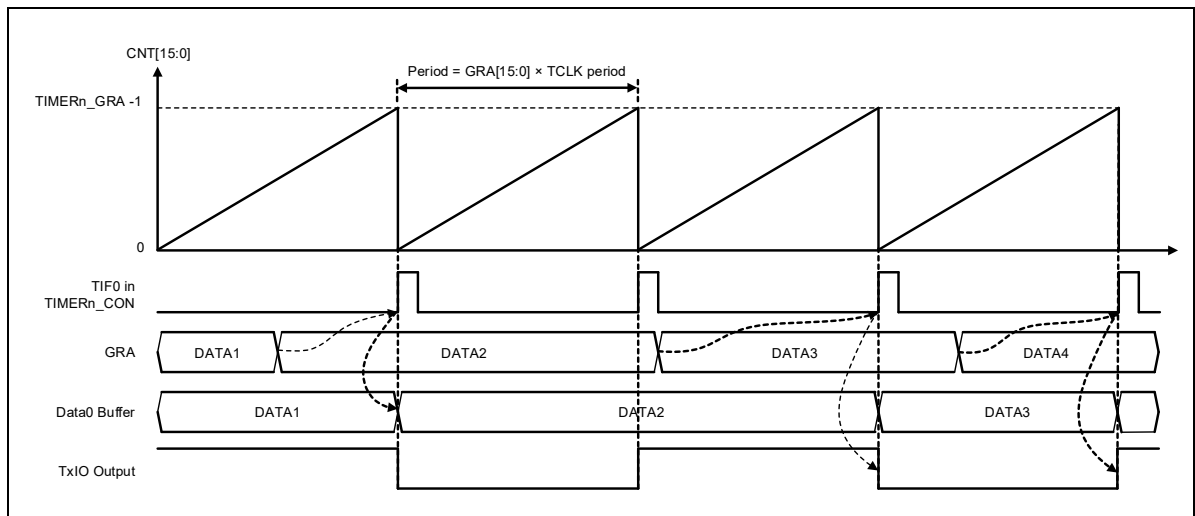
Figure 8.3. Periodic mode operation of 16-bit timer
