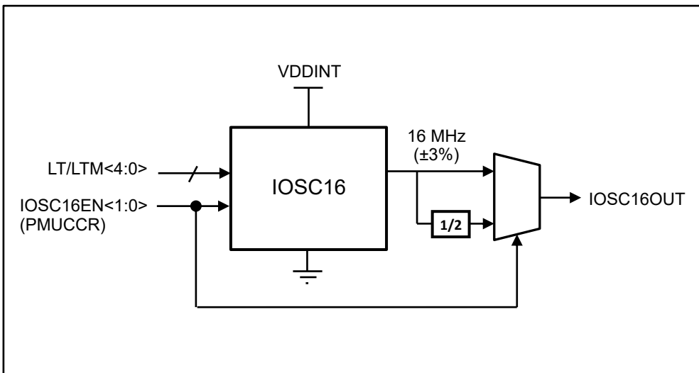
Figure 16.8. Internal configuration of IOSC16
