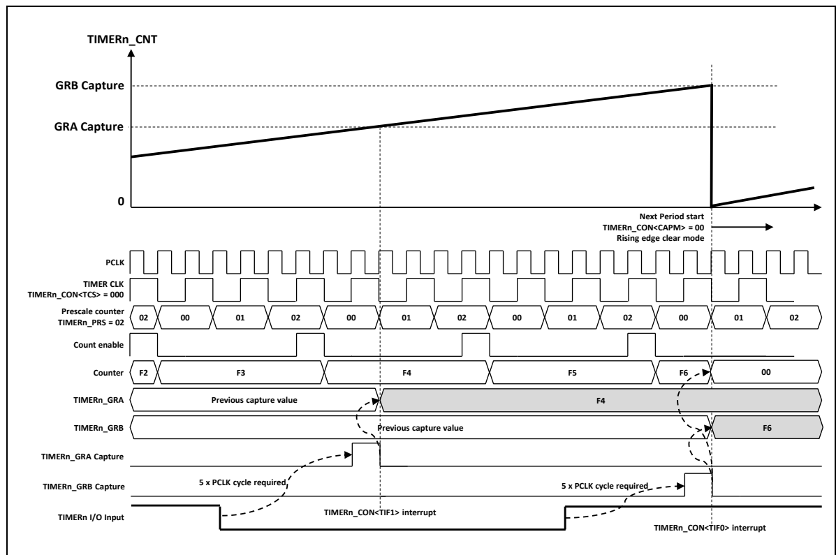
Figure 8.6. Capture mode operation of 16-bit timer
