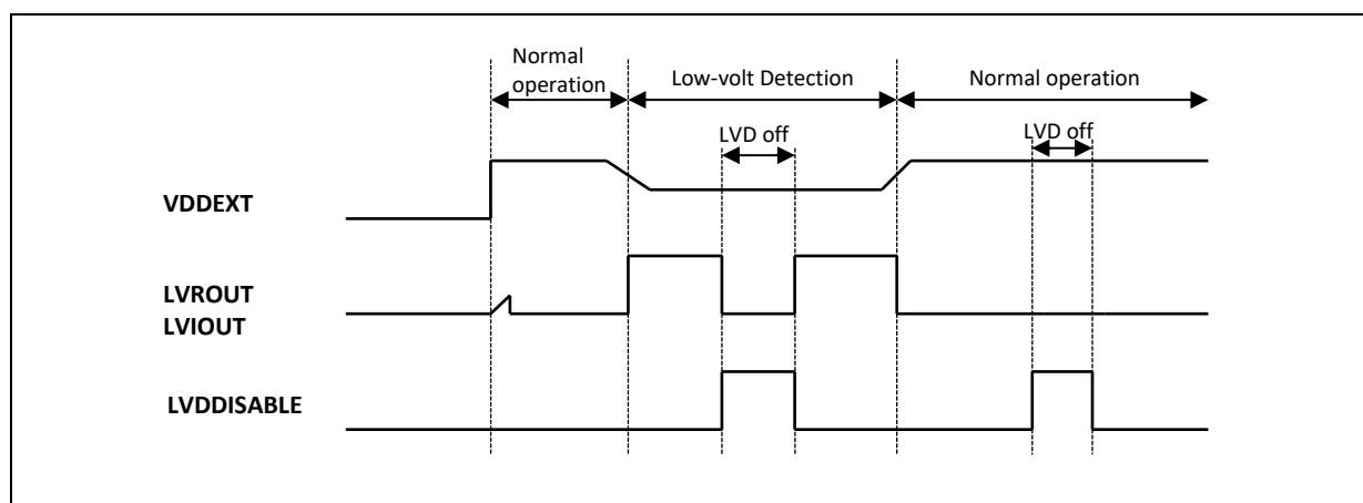
Figure 16.2. Reset timing
