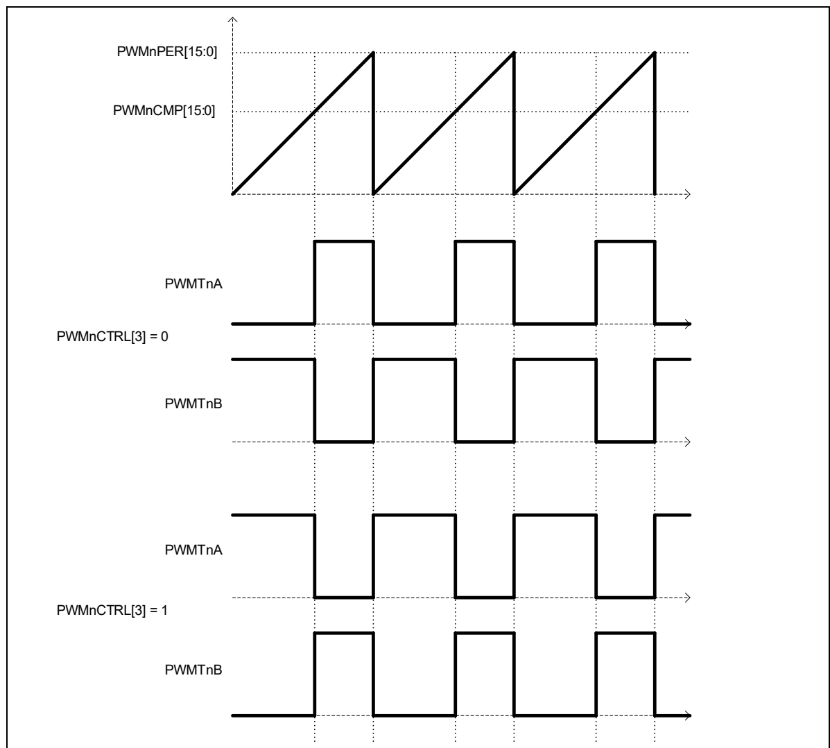
Figure 9.2. Block diagram of PWM output timing
