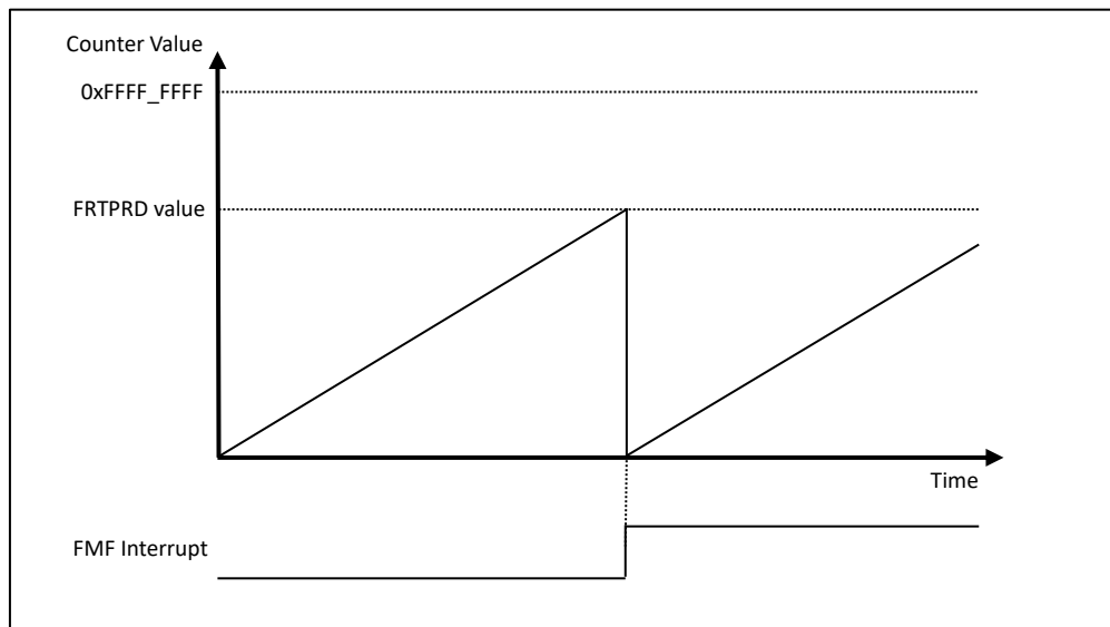
Figure 7.3. Operating example in periodic mode-1
