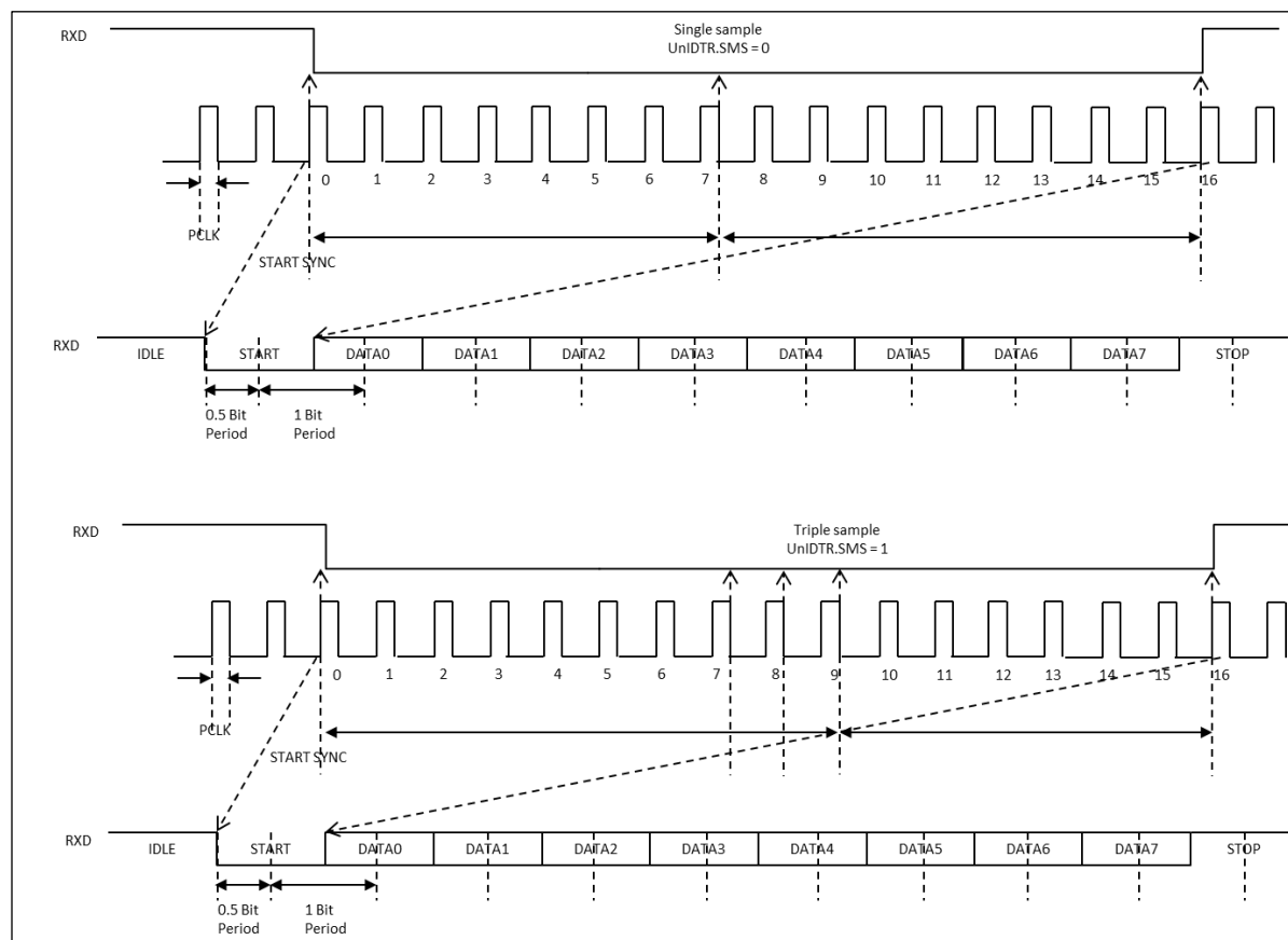
Figure 11.6. Timing diagram of the start bit detection in single sampling mode and multi sampling mode.
