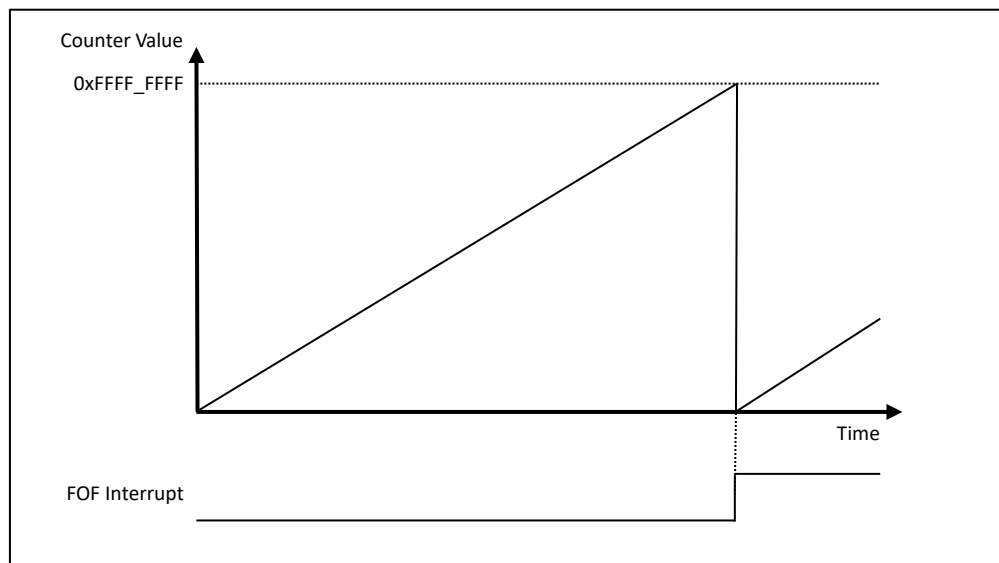
Figure 7.2. Operating timing in free-run mode
