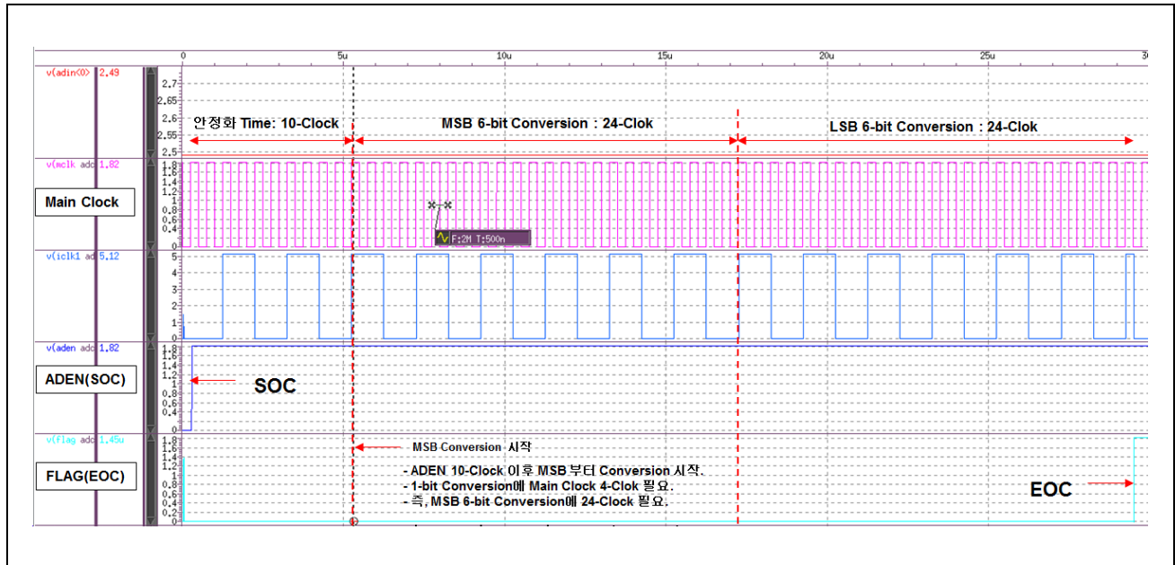
Figure 13.2. A/D conversion timing
