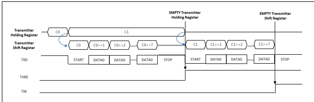
Figure 11.5. Diagram of transmit interrupt timing
