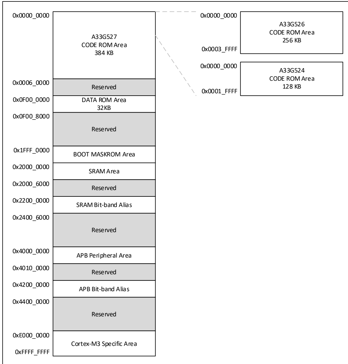
Figure 1.9. Overall memory map
