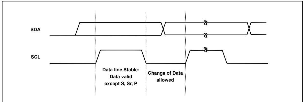
Figure 10.2. Bit transfer on I2C interface bus
