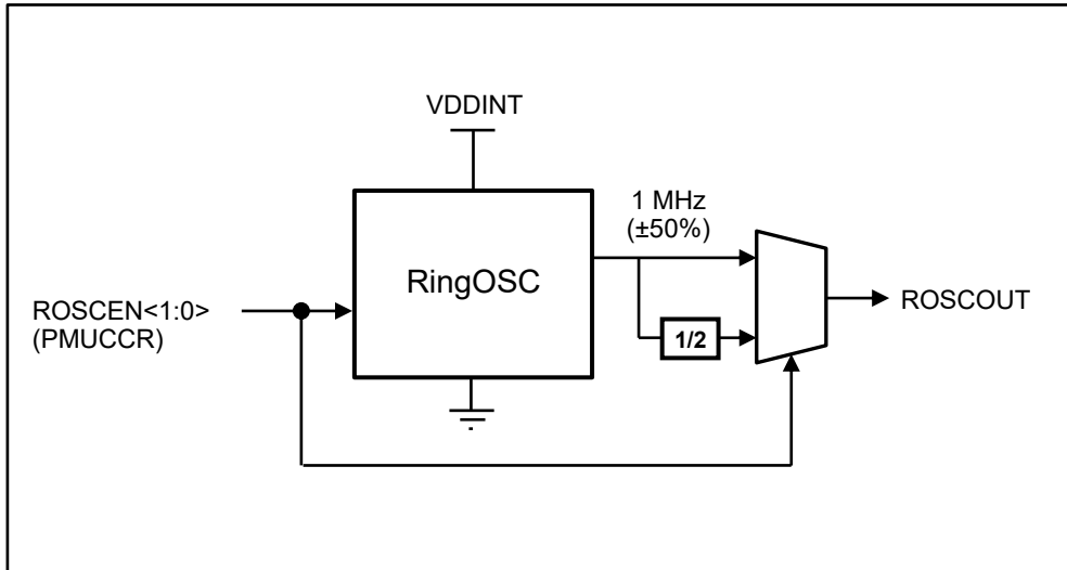
Figure 16.7. Internal configuration of RingOSC
