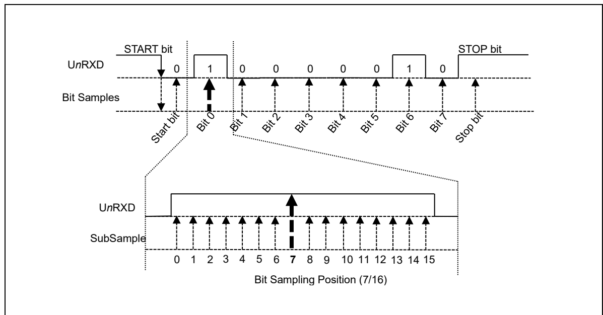
Figure 11.2. Sampling method in 8-bit data receiving
