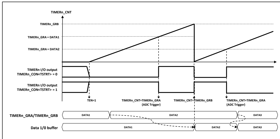
Figure 8.5. PWM mode operation of 16-bit timer
