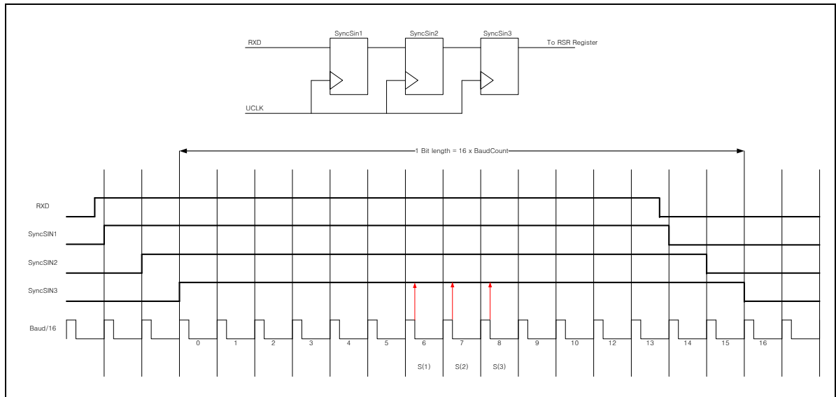
Figure 11.7. Timing diagram of data smapling
