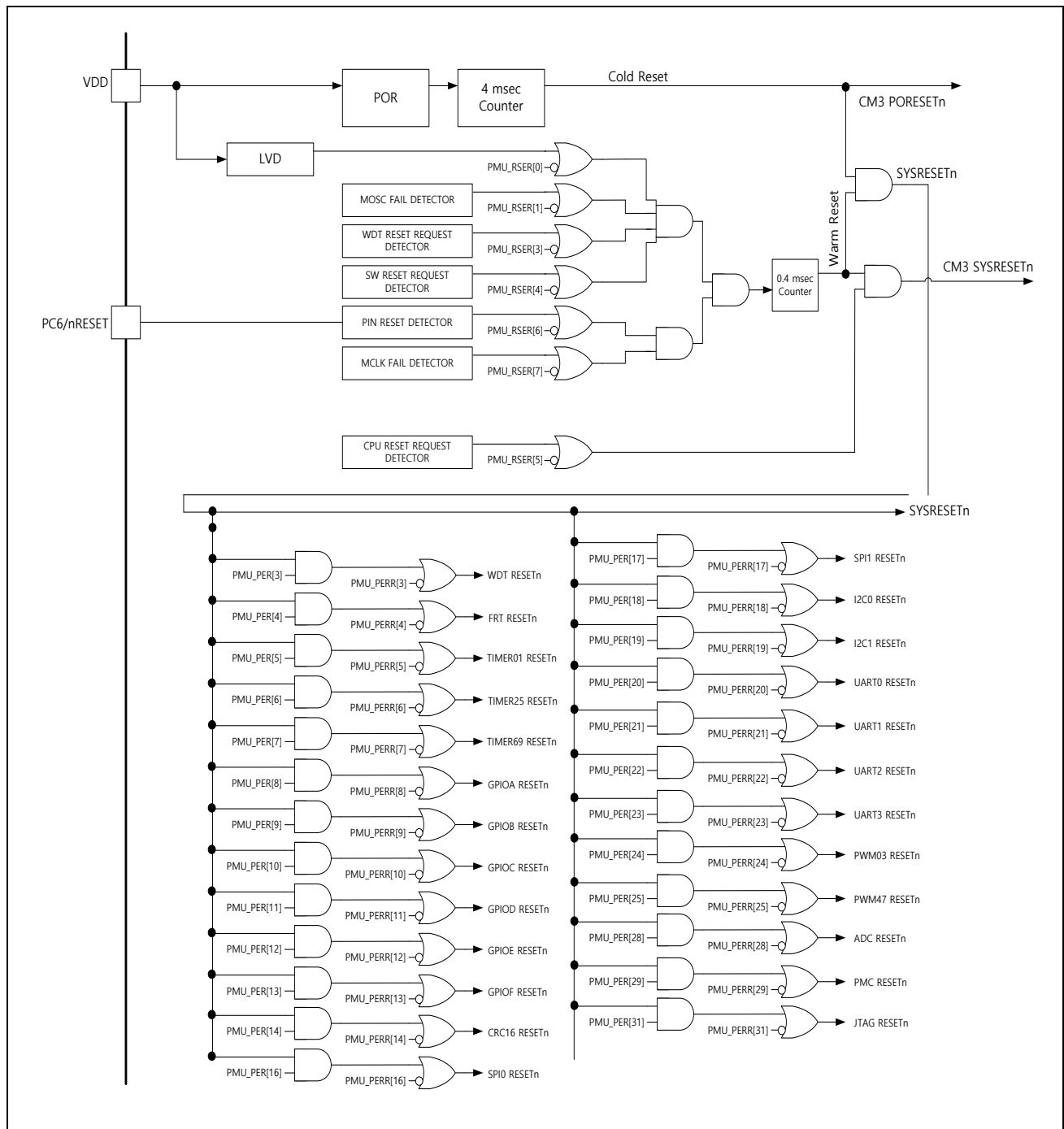
Figure 3.3. Block diagram of A33G52x PMU reset
