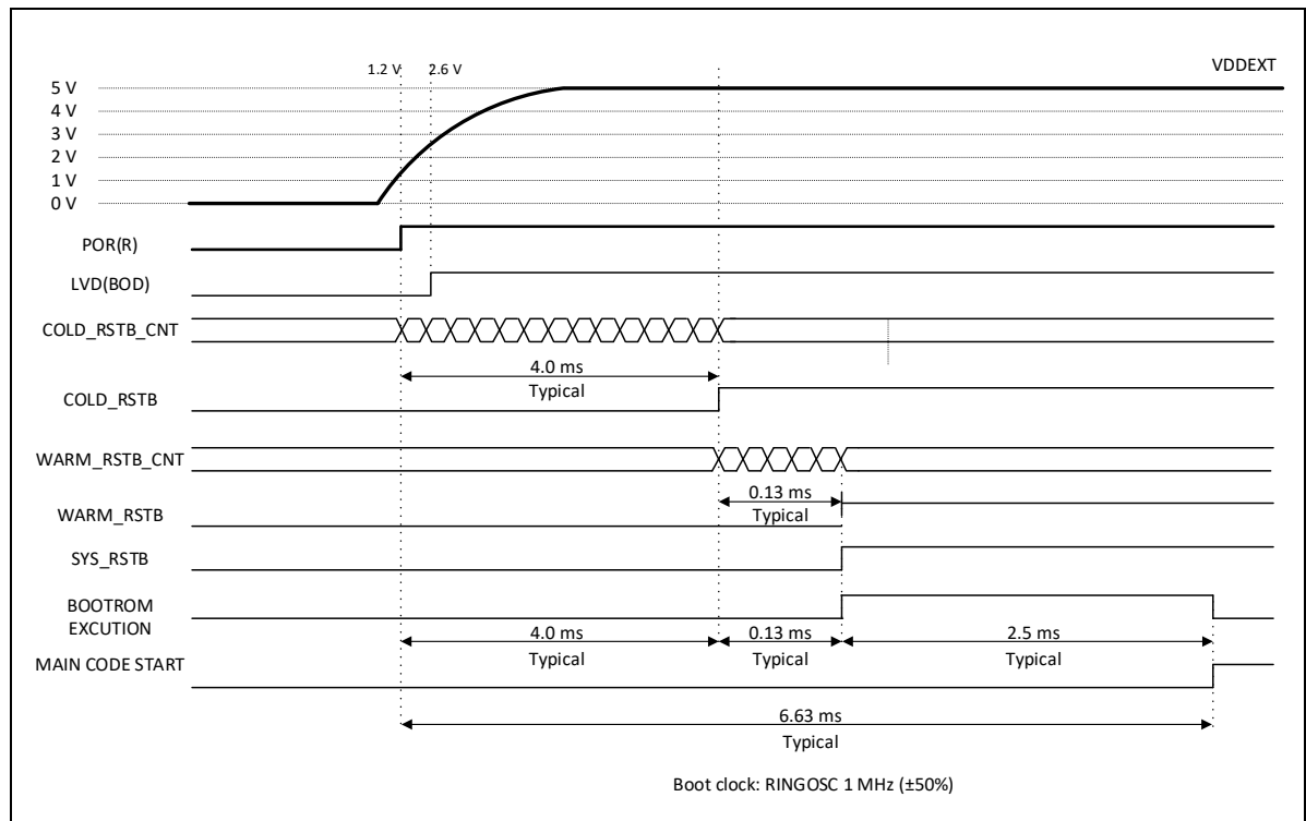
Figure 3.6. Cold reset timing of A33G52x
