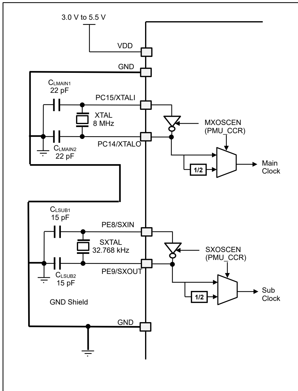
Figure 16.10. Configuration of main and sub oscillator
