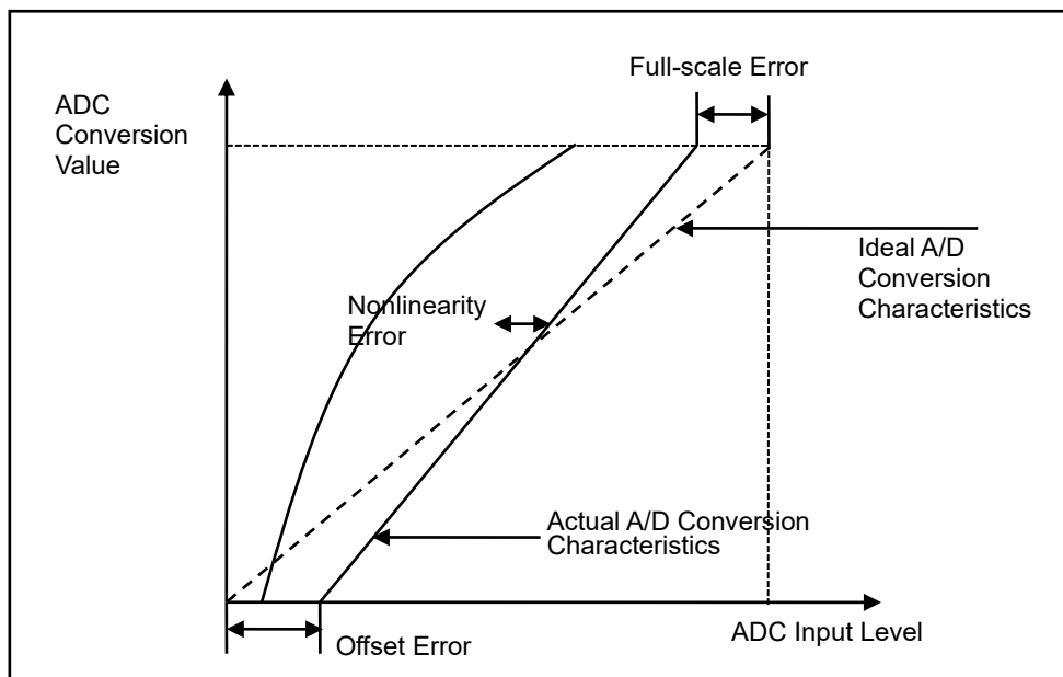
Figure 13.4. Definition of A/D conversion resolution (2)
