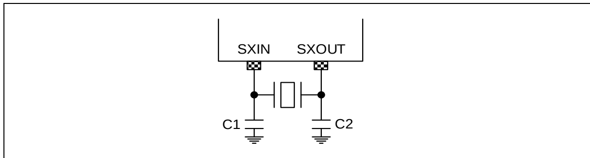
Figure 45. Crystal Oscillator
