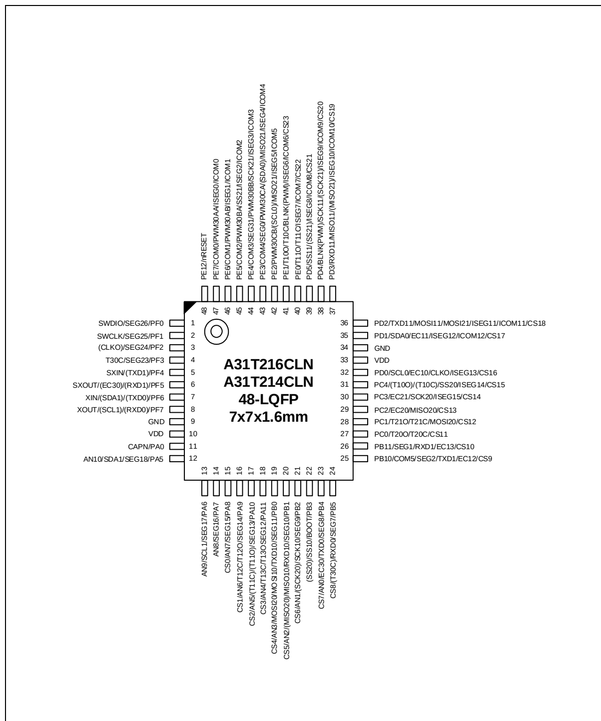
Figure 4. LQFP 48 Pinouts
