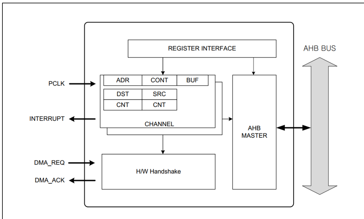
Figure 26. DMAC Block Diagram
