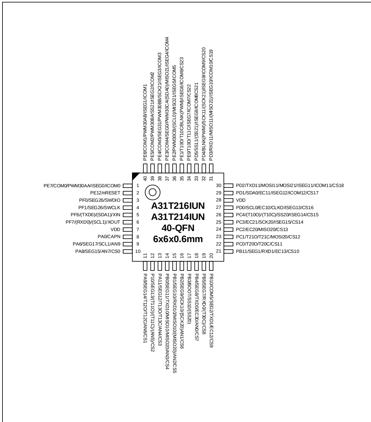
Figure 6. QFN 40 Pinouts
