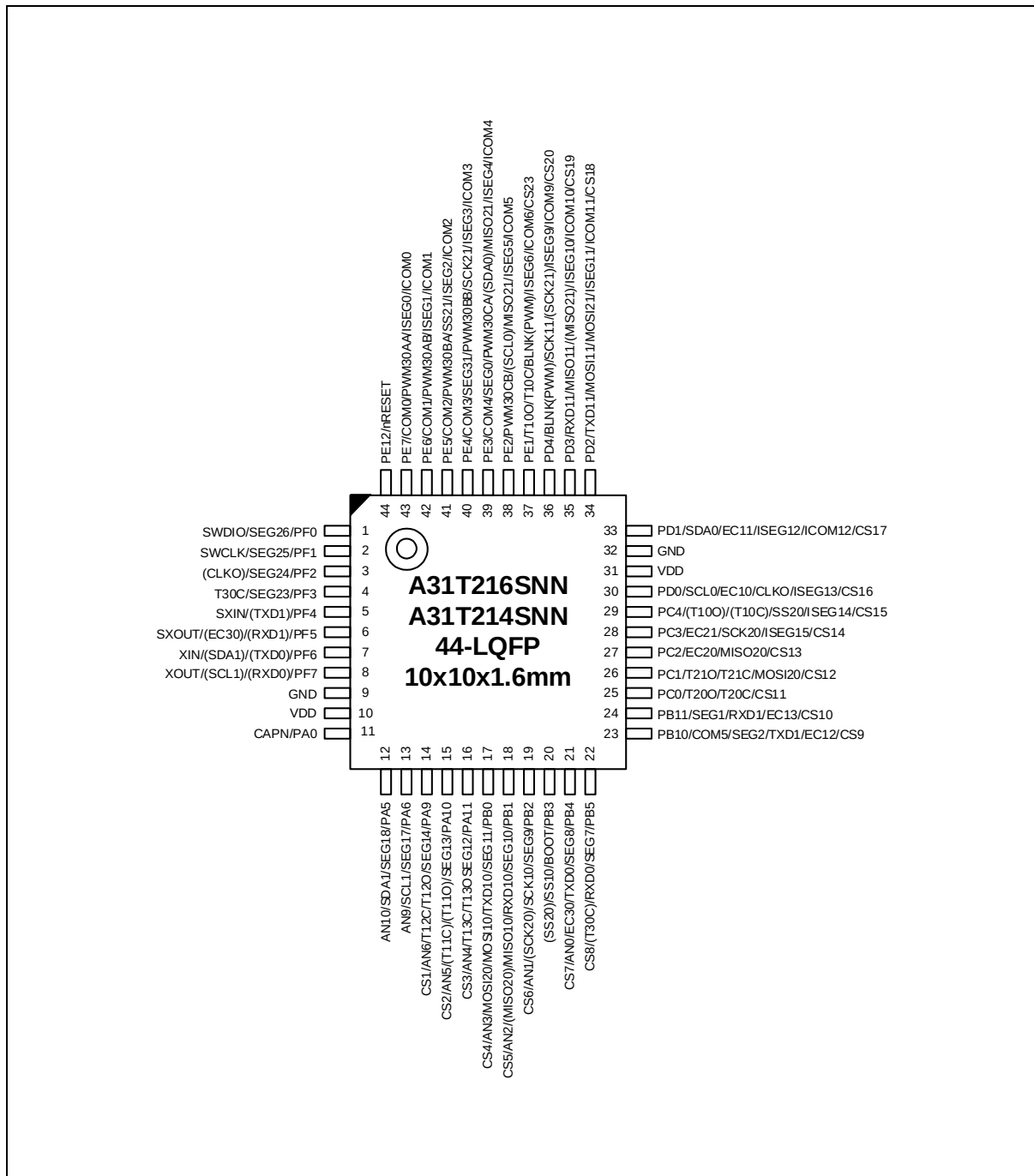
Figure 5. LQFP 44 Pinouts
