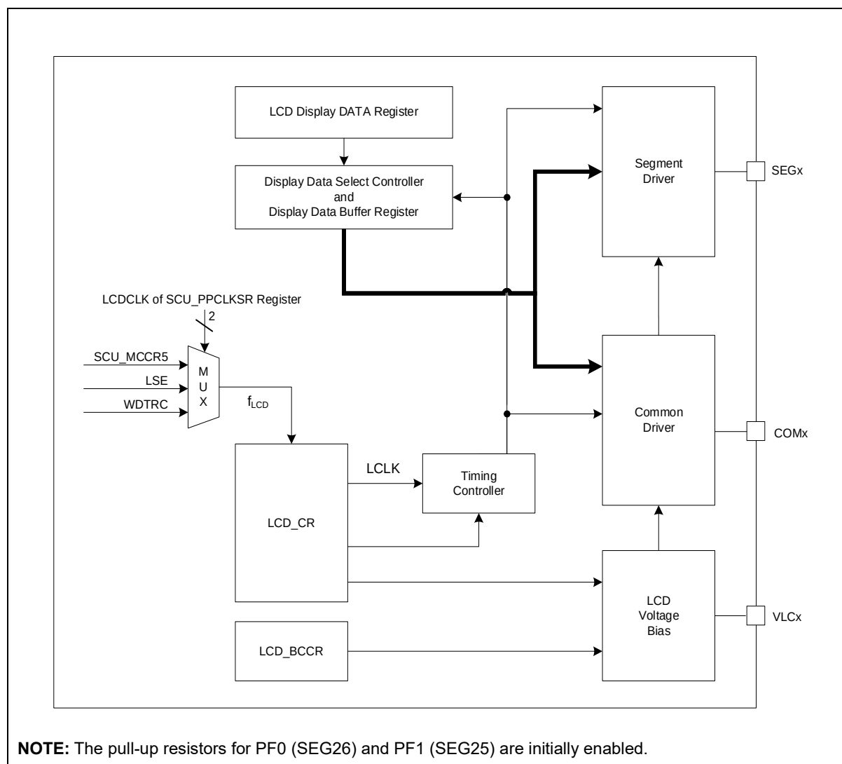
Figure 39. LCD Driver Block Diagram
