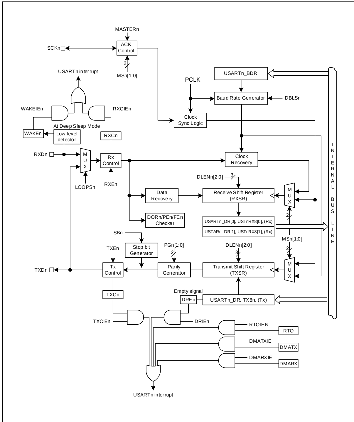
Figure 32. USART Block Diagram (n = 10 and 11)
