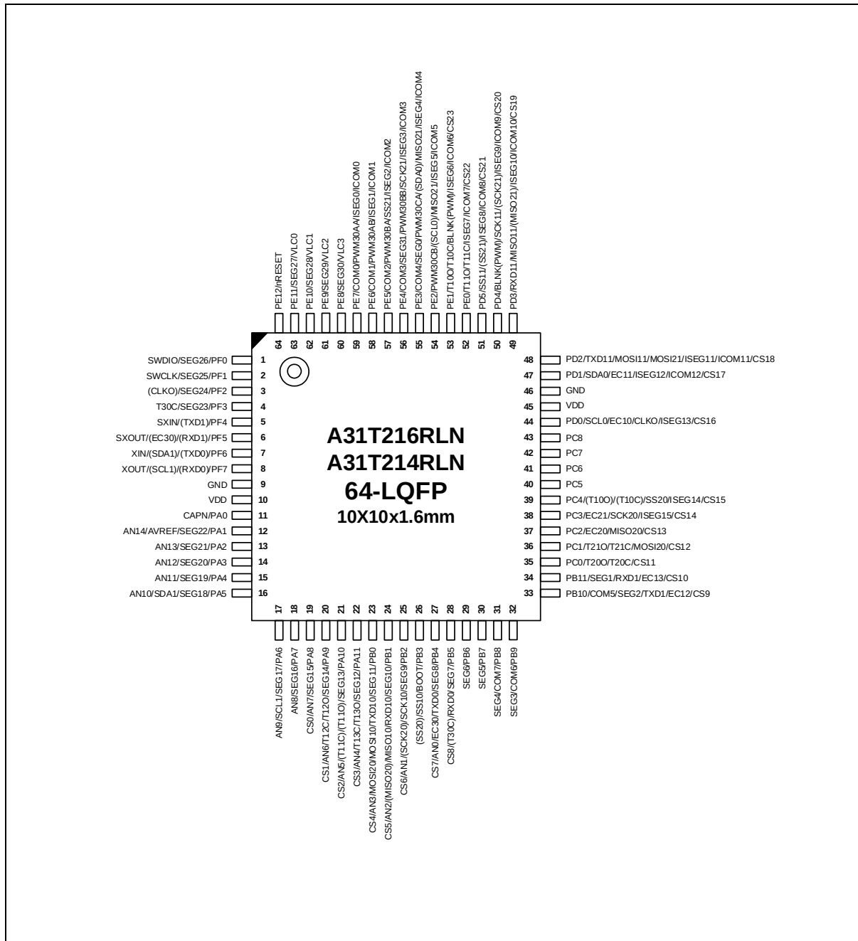
Figure 3. LQFP 64 Pinouts
