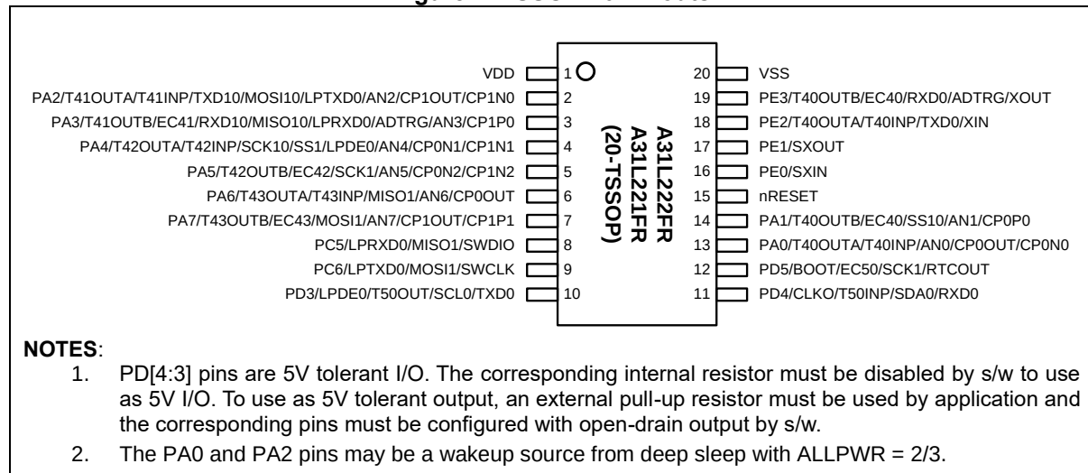
Figure 2. TSSOP-20 Pinouts
