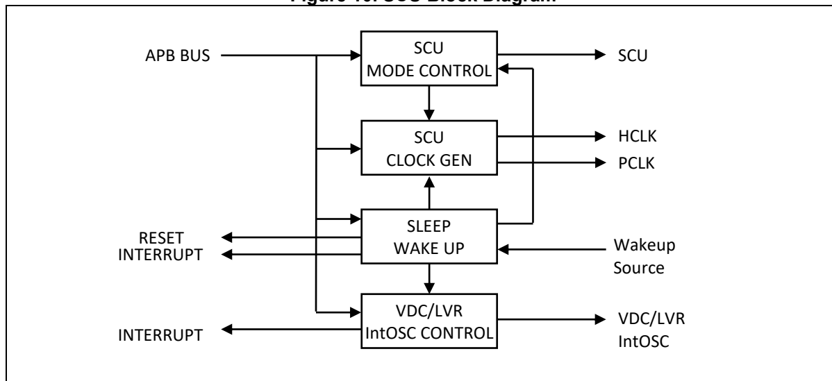
Figure 10. SCU Block Diagram
