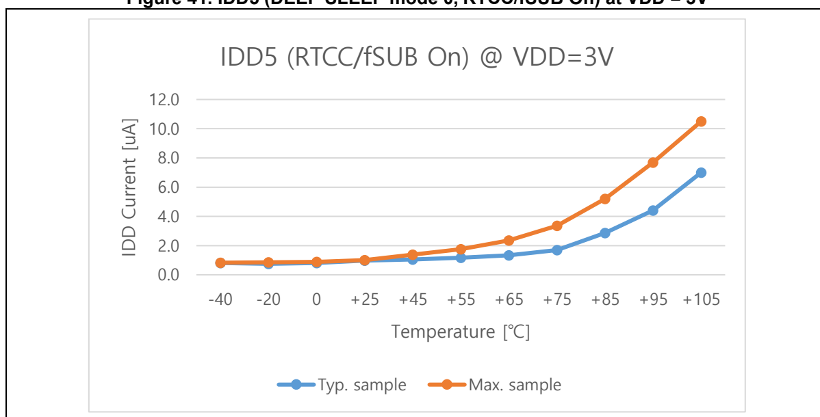
Figure 41. IDD5 (DEEP SLEEP mode 0, RTCC/fSUB On) at VDD = 3V
