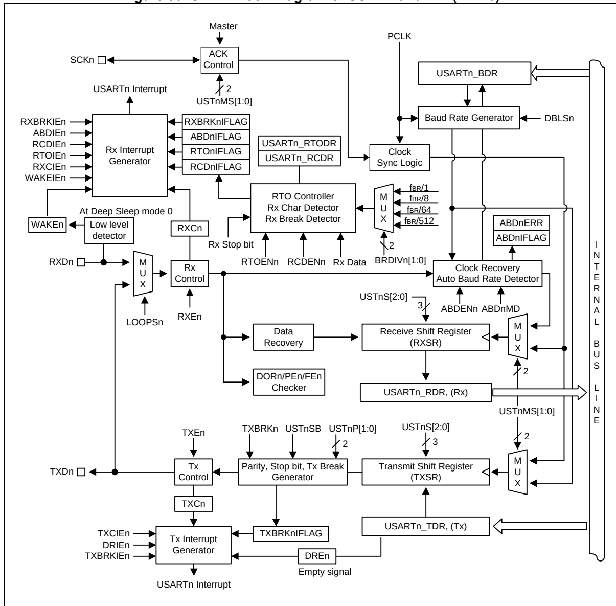
Figure 30. UART Block Diagram of USART and LIN (n = 10)
