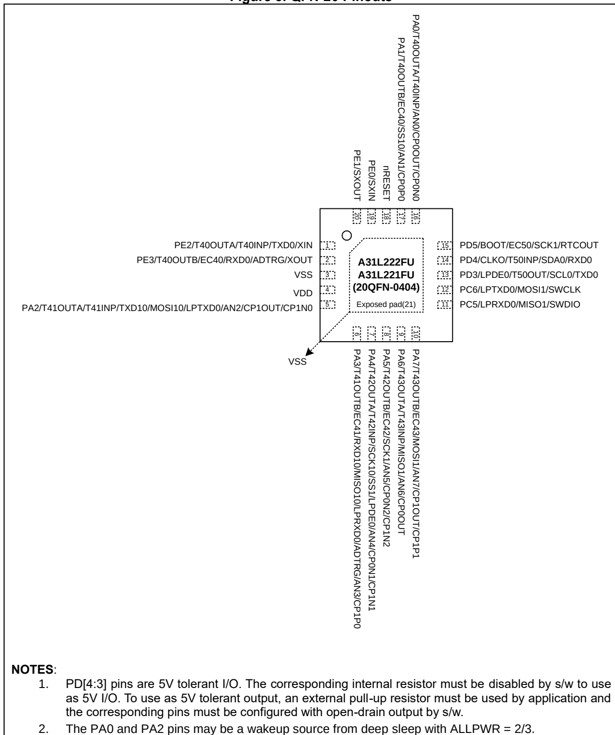
Figure 3. QFN-20 Pinouts
