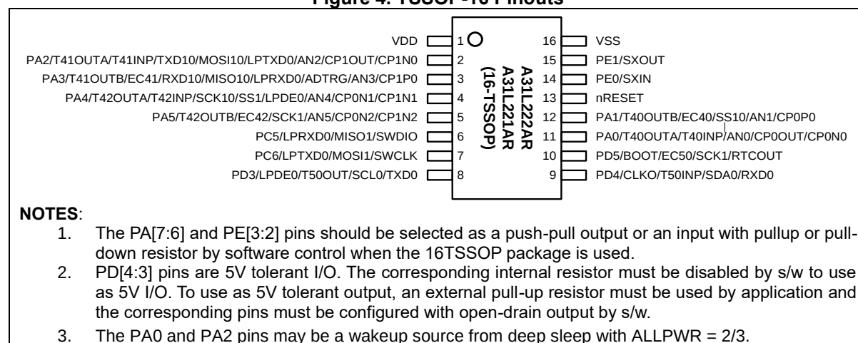
Figure 4. TSSOP-16 Pinouts
