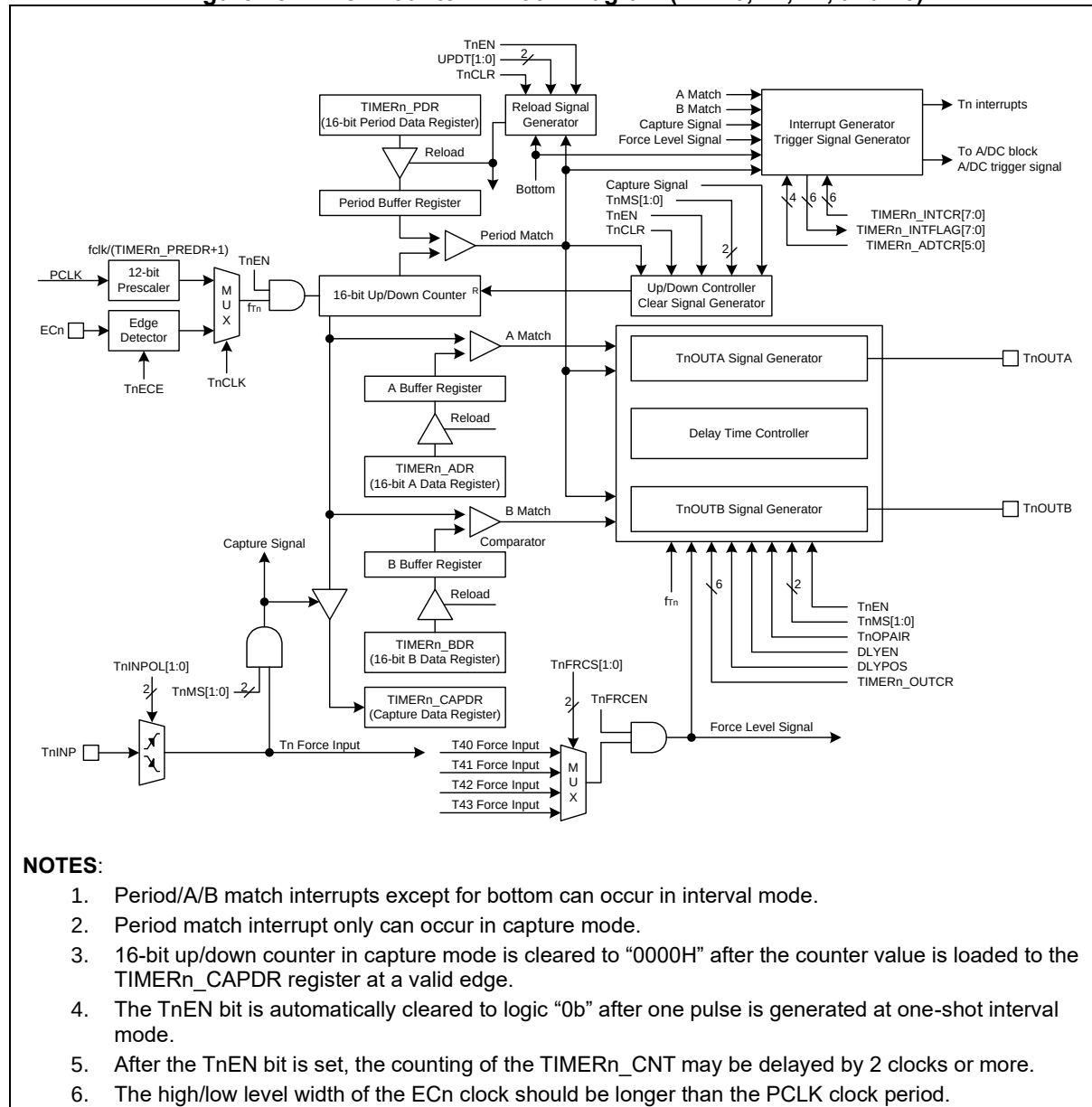
Figure 25. Timer Counter n Block Diagram (n = 40, 41, 42, and 43)
