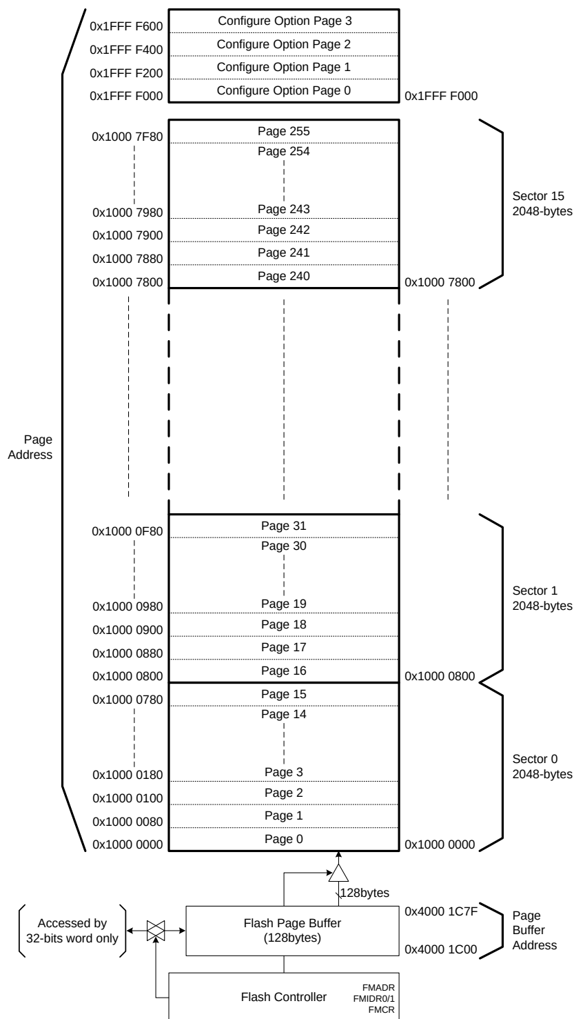
Figure 8. Built-in Flash Memory Block Diagram
