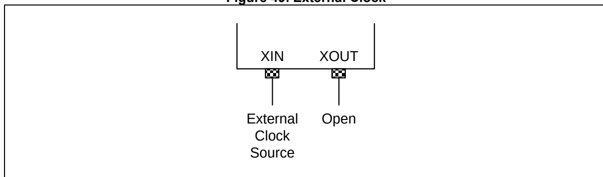
Figure 49. External Clock
