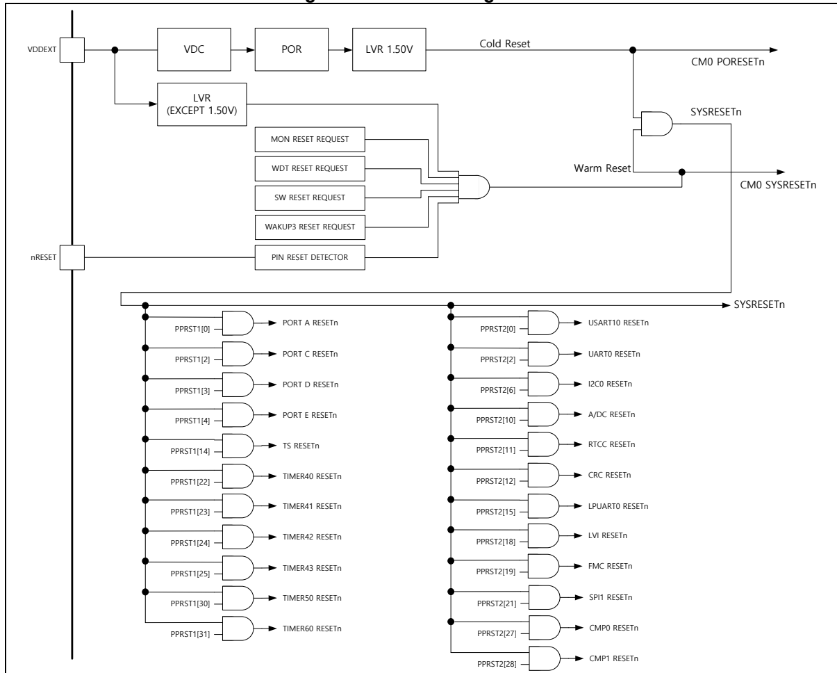
Figure 15. Reset Configuration
