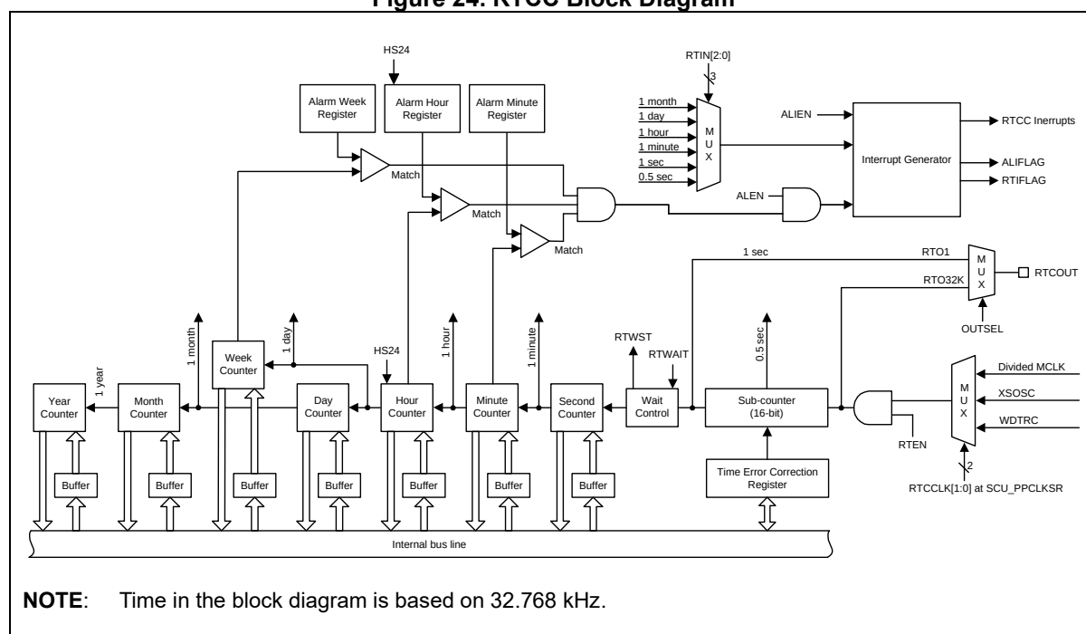
Figure 24. RTCC Block Diagram
