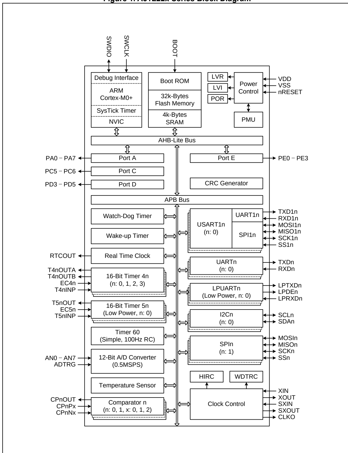
Figure 1. A31L22x Series Block Diagram
