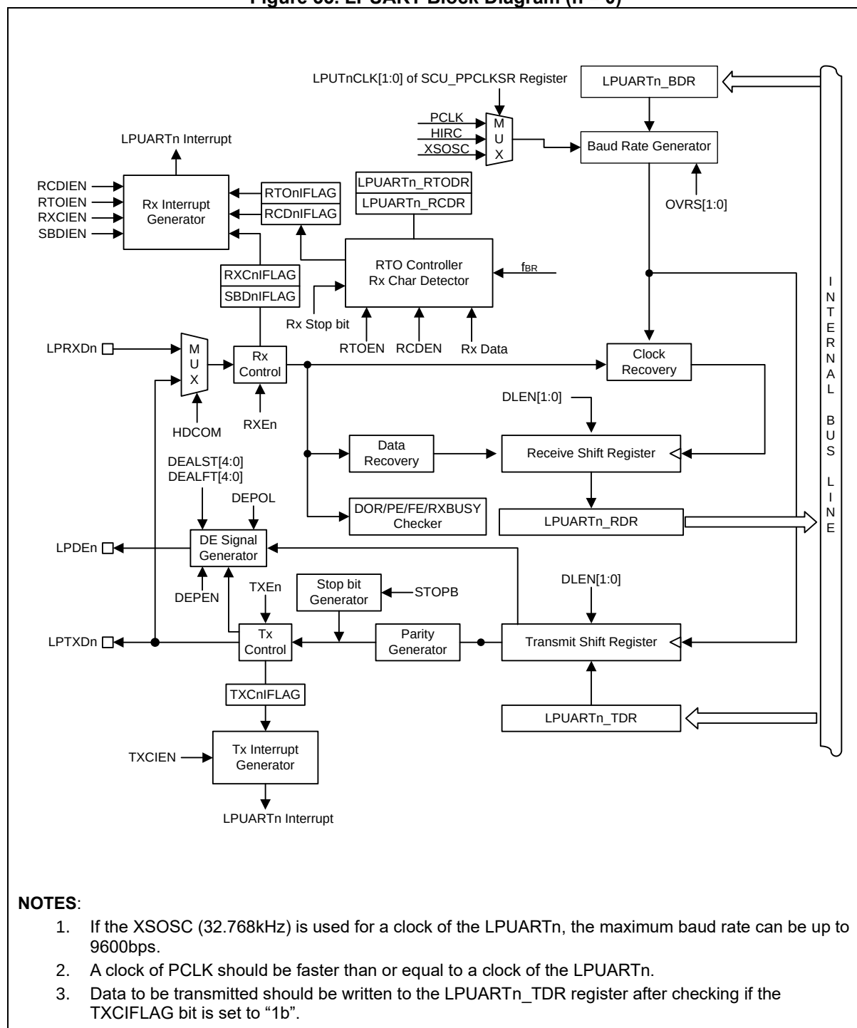
Figure 33. LPUART Block Diagram (n = 0)
