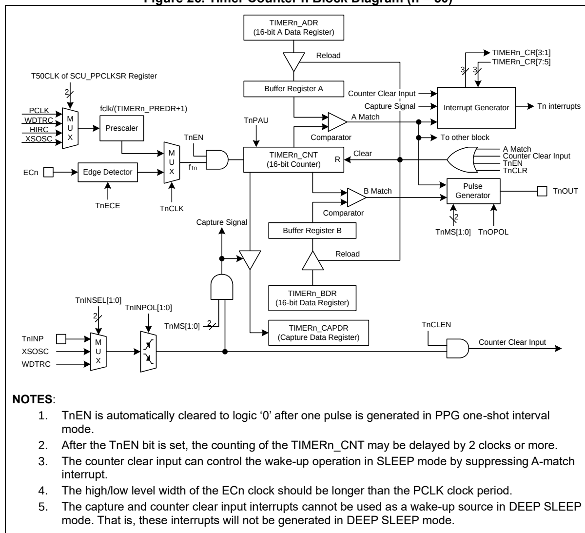
Figure 26. Timer Counter n Block Diagram (n = 50)
