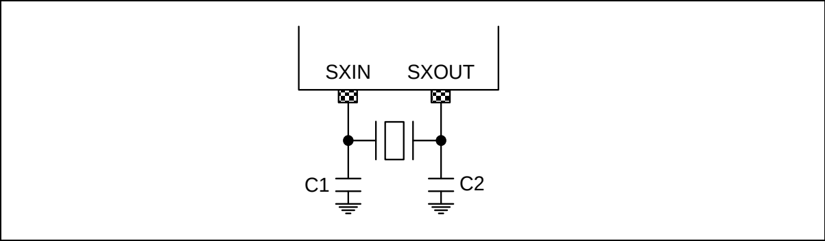
Figure 50. Crystal Oscillator
