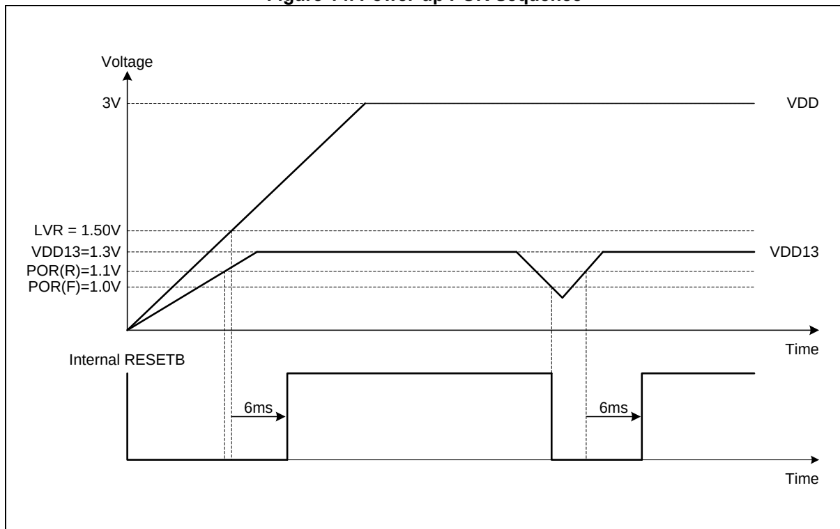
Figure 14. Power-up POR Sequence
