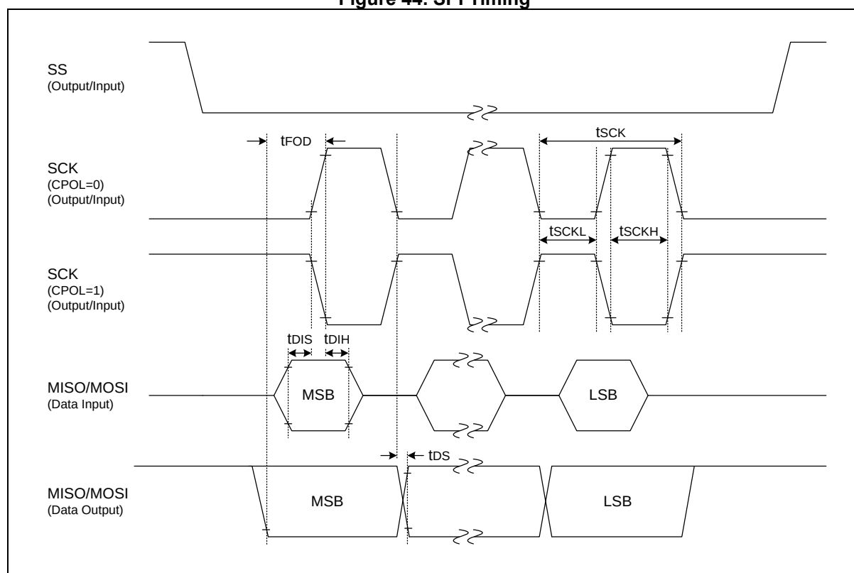
Figure 44. SPI Timing
