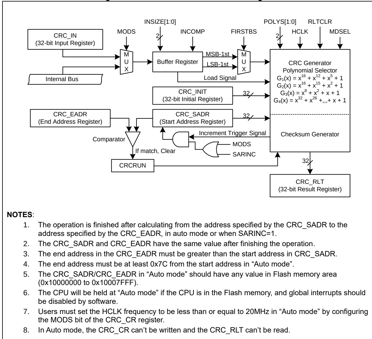
Figure 36. CRC and Checksum Block Diagram
