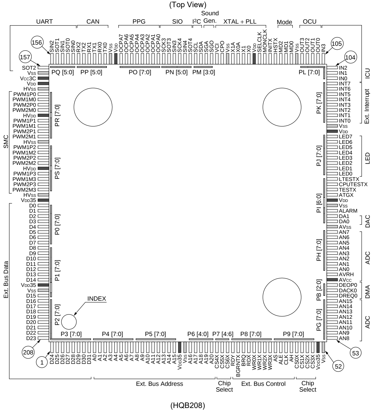
Figure 2-1. CY91F362GB
