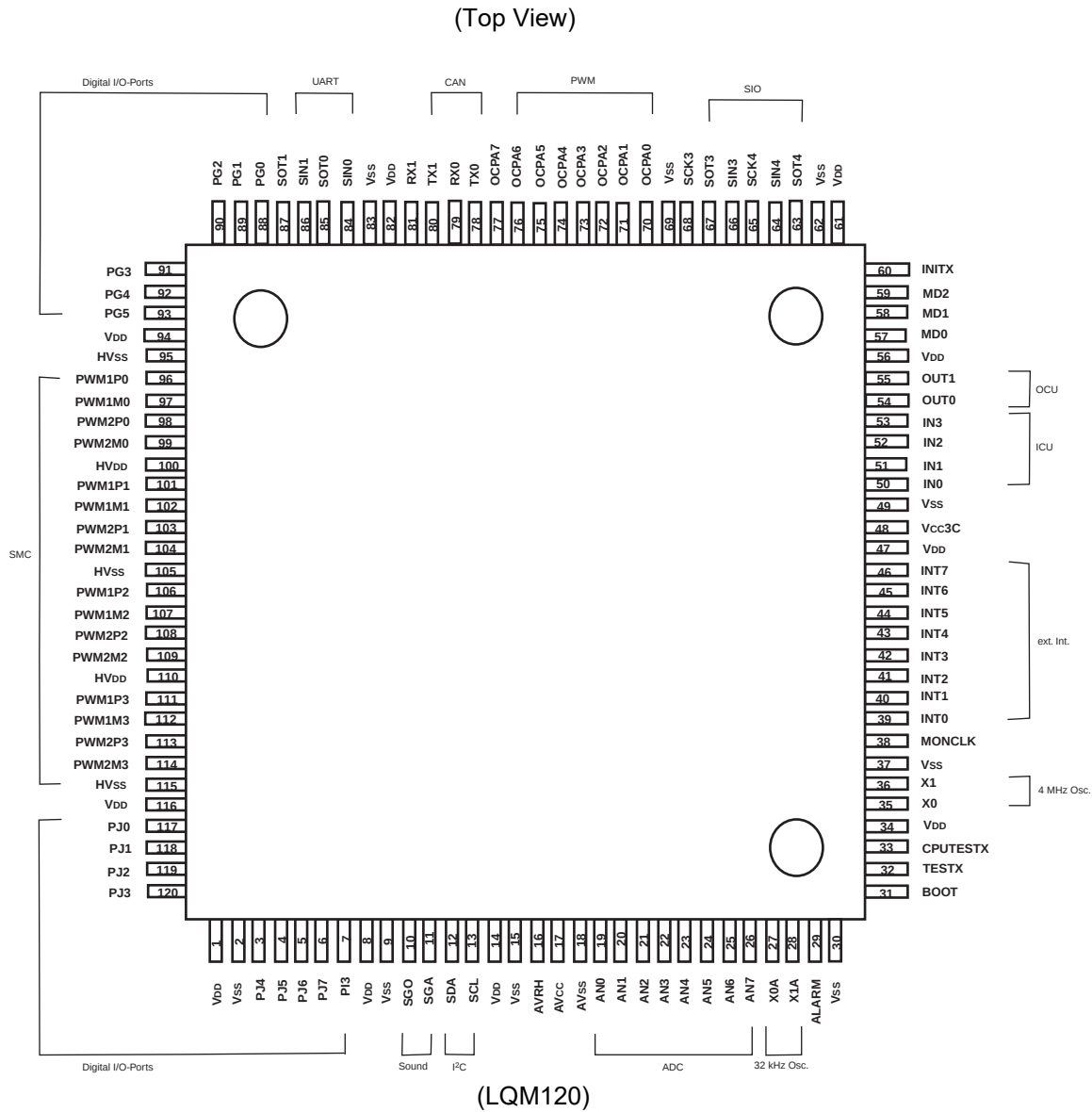
Figure 2-8. CY91366GA
