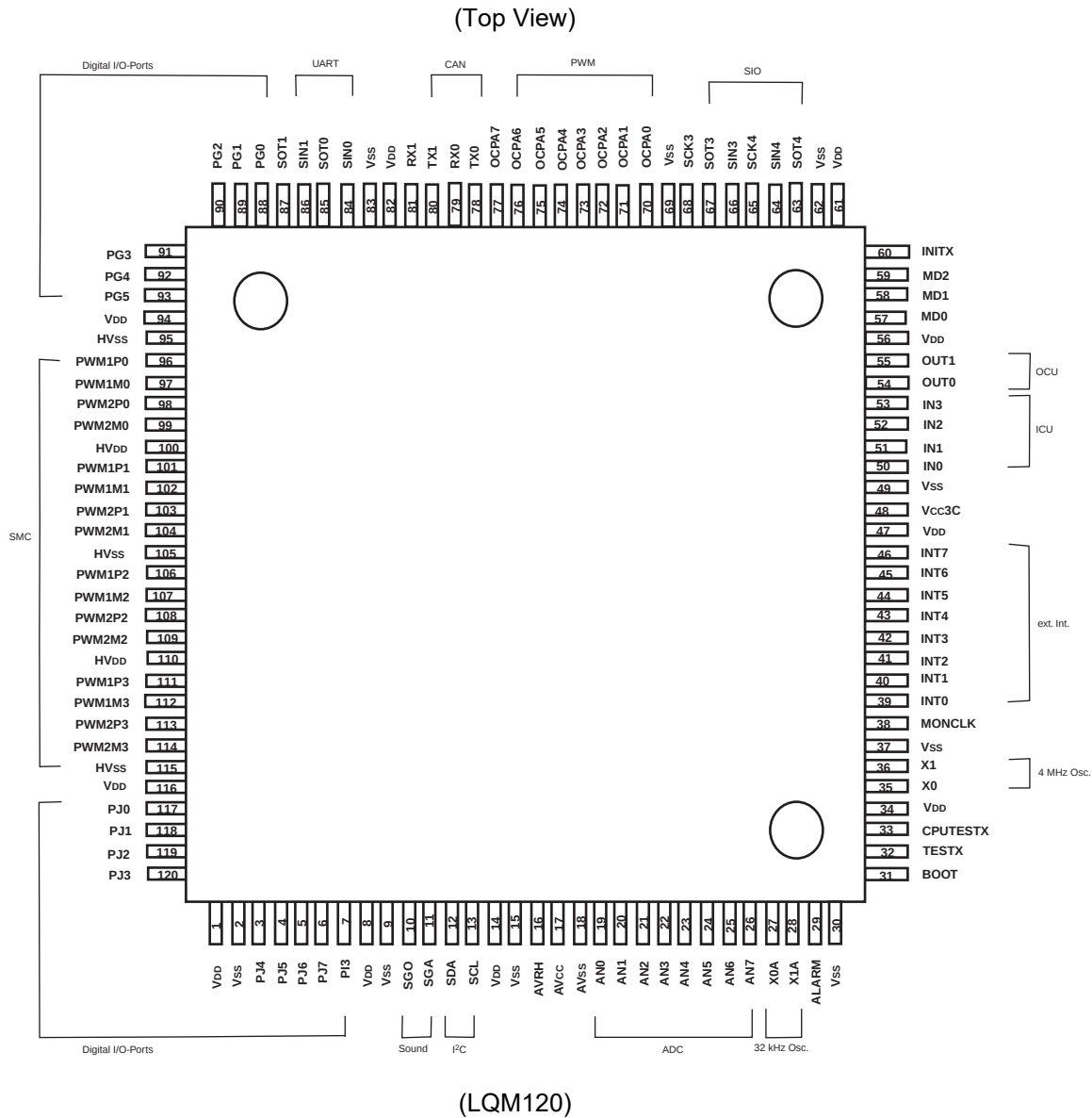
Figure 2-5. CY91F366GB/CY91F376G
