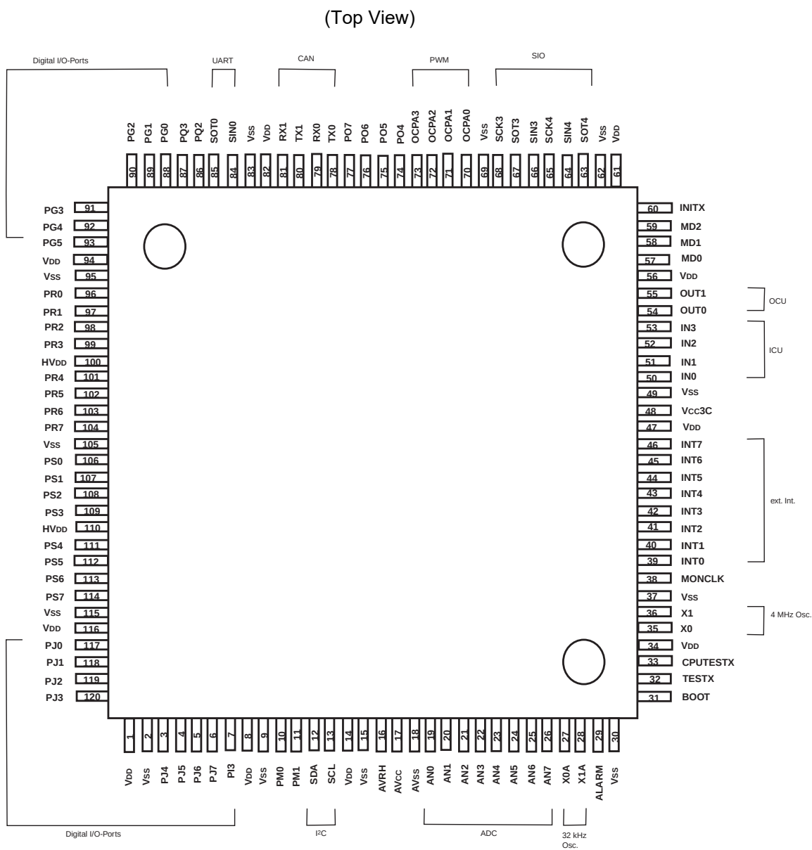
Figure 2-7. CY91F368GB
