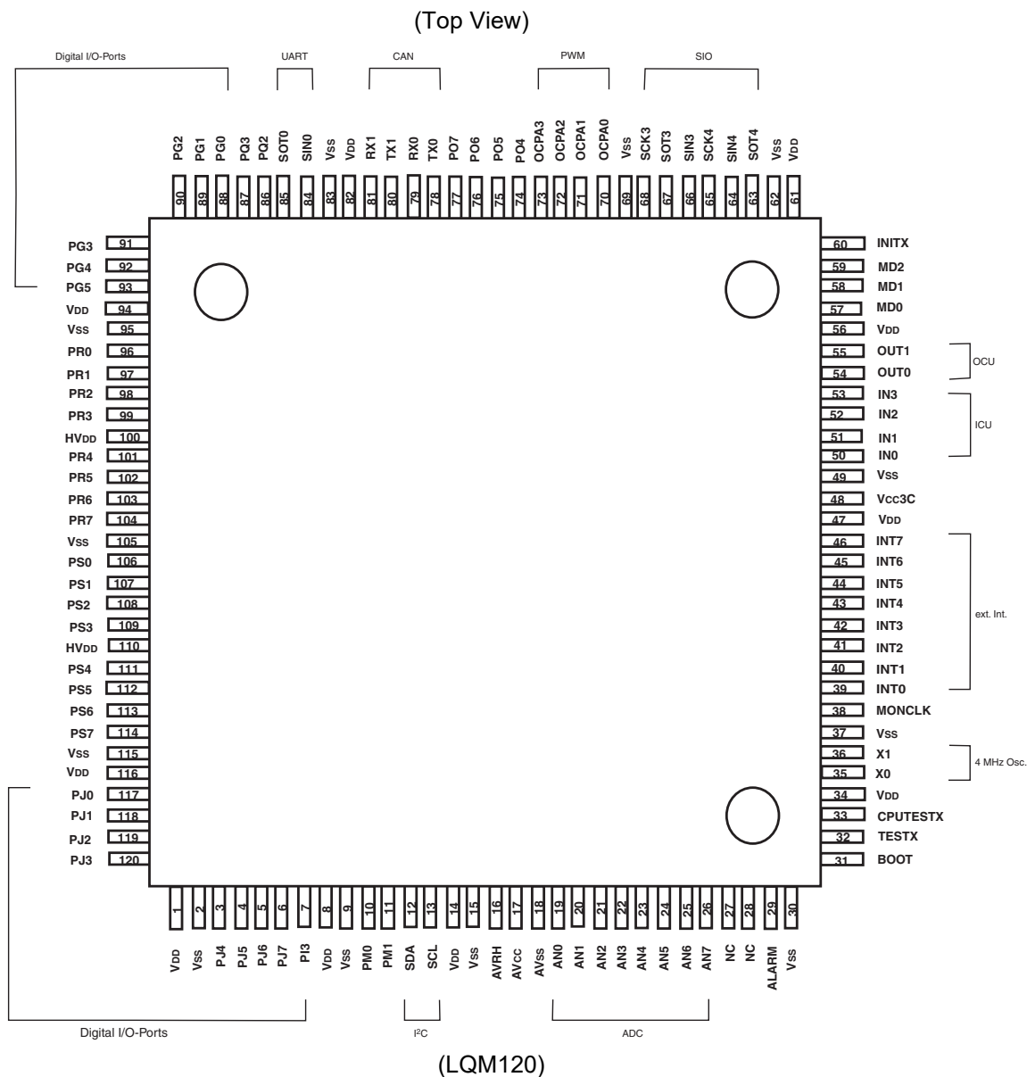
Figure 2-6. CY91F367GB
