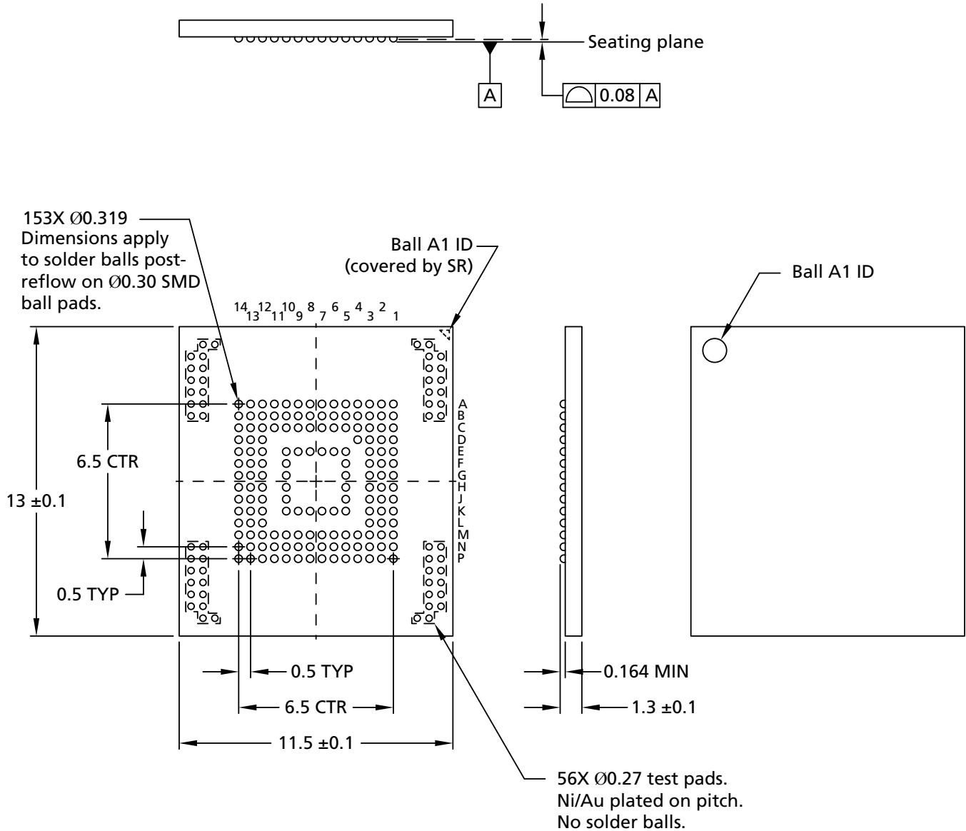
Figure 4: 153-Ball LFBGA – 11.5mm x 13.0mm x 1.4mm (Package code EY)
