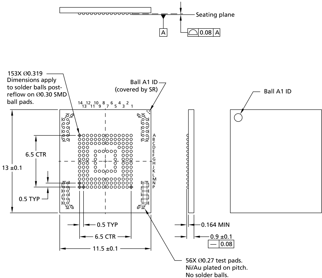
Figure 5: 153-Ball VFBGA – 11.5mm x 13.0mm x 1.0mm (Package code CN)
