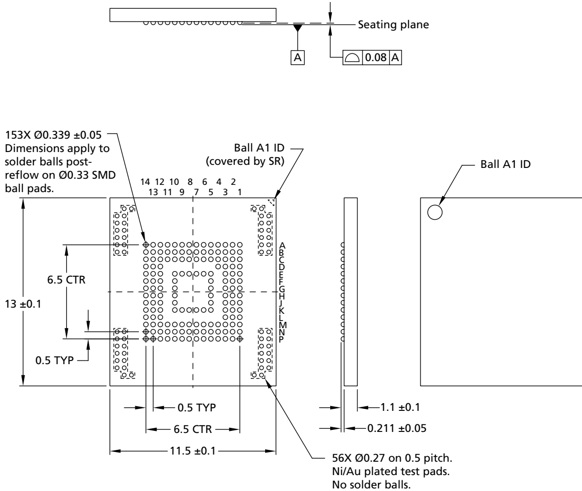
Figure 3: 153-Ball TFBGA – 11.5mm × 13.0mm × 1.2mm (Package Code: NS)
