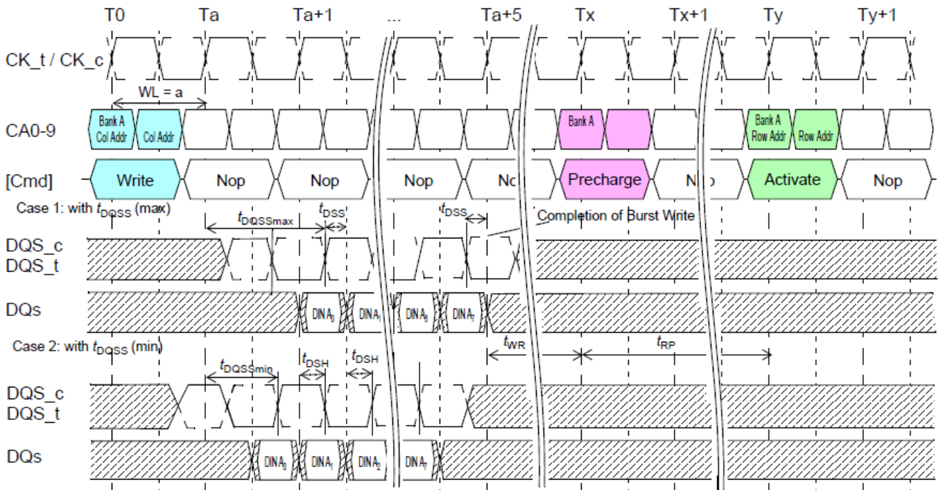
Burst Write
