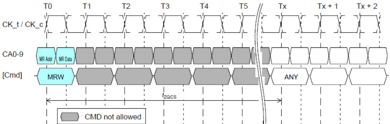
ZQ Calibration Short Timing
