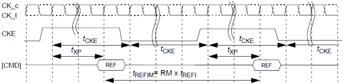
REFRESH-to-REFRESH Timing in CKE-Intensive Environments
