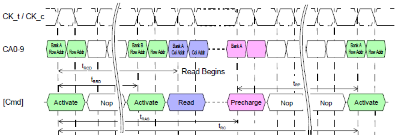
ACTIVATE Command
