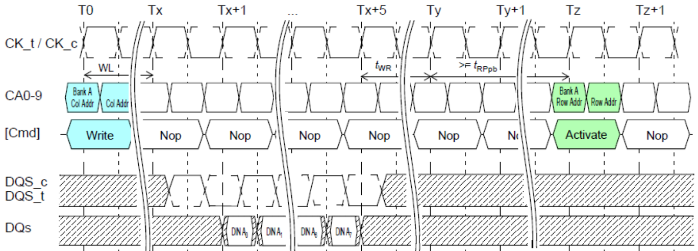
Burst Write with Auto Precharge
