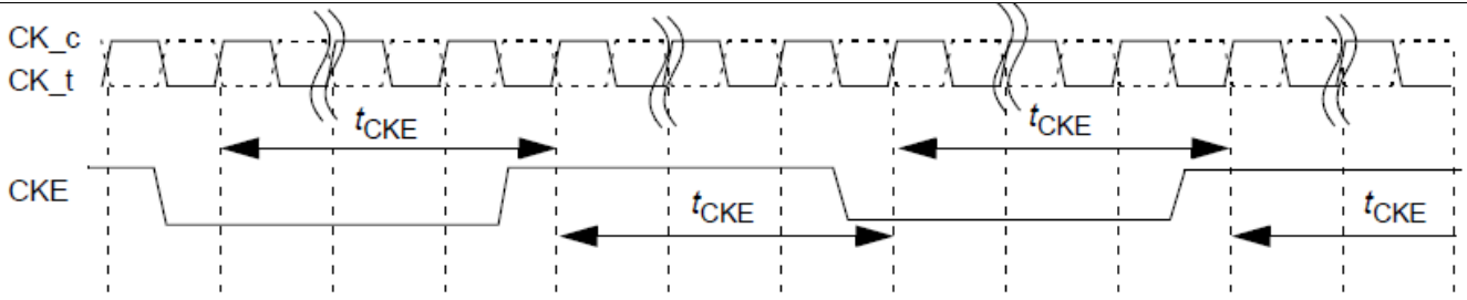
CKE-Intensive Environment
