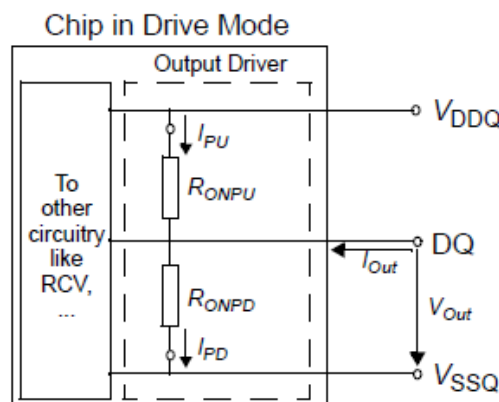
Output Driver: Definition of Voltages and Currents
