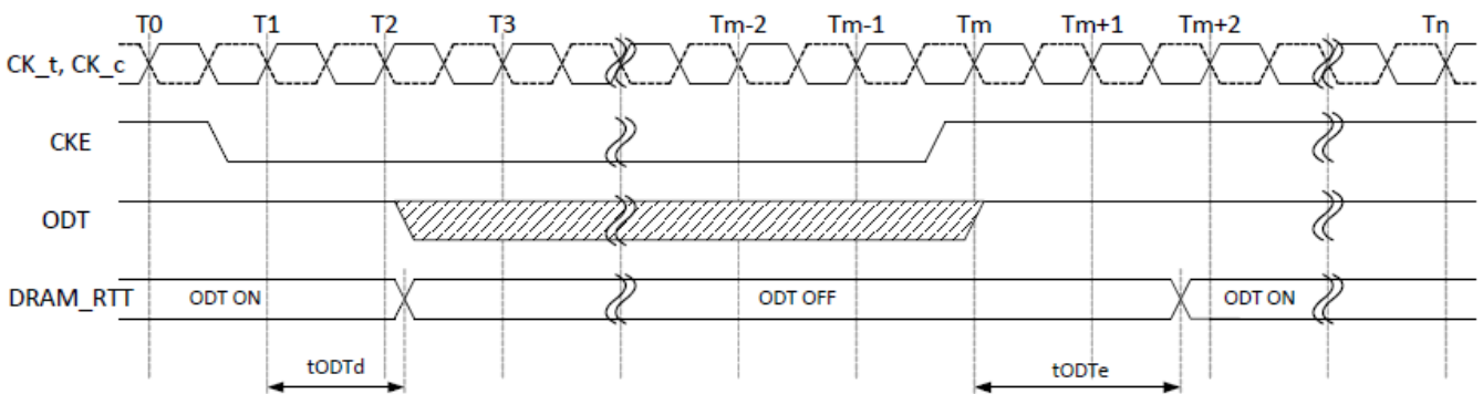
ODT Timing During Power Down, Self Refresh, Deep Power Down Entry/Exit Example
