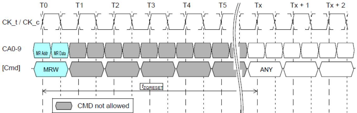
ZQ Calibration Reset Timing
