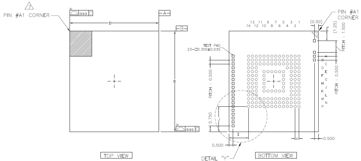
Figure 1. 11.5 x 13.0 x 1.0 (mm) Package Dimension
