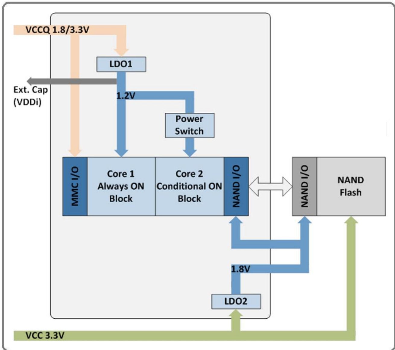
Figure 3. JSMC08AUM3HYAEA-H5 Block Diagram
