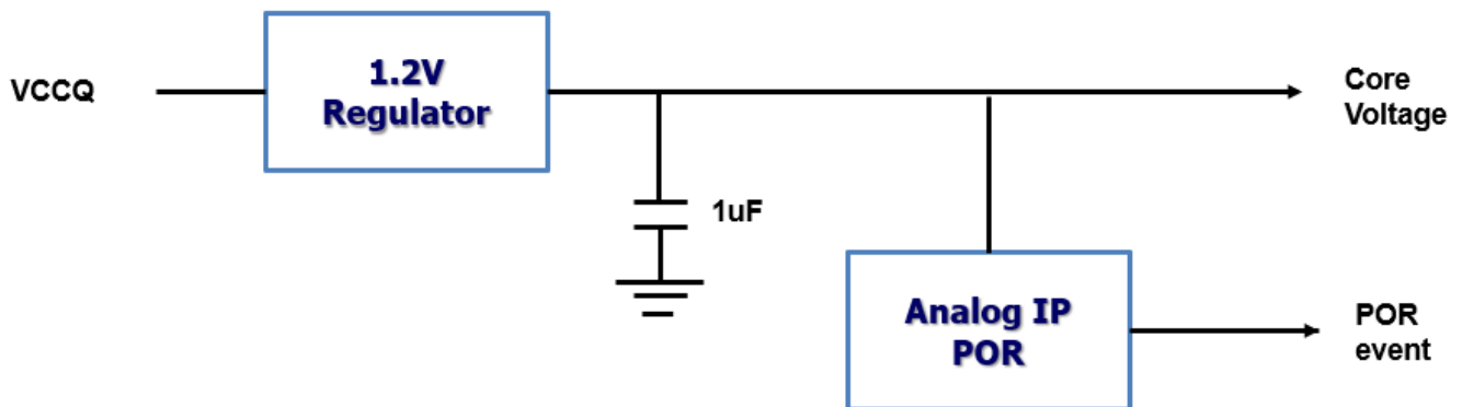
Figure Appendix 1. eMMC POR Circuit Block Diagram
