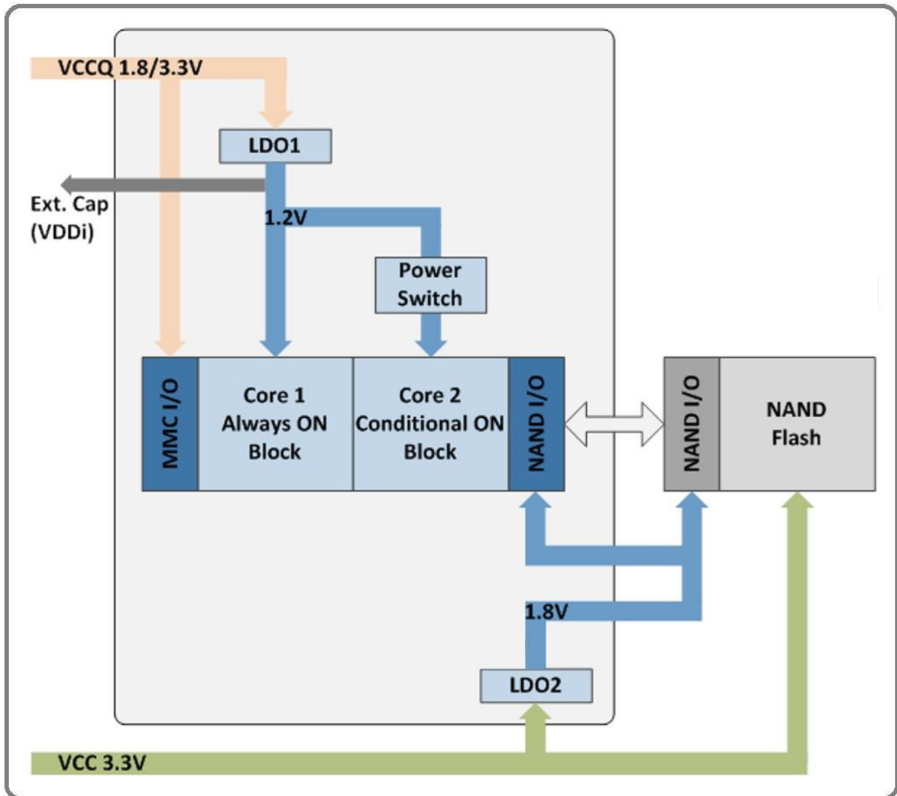
Figure 3. JSMC04AUM1HYAEA-H5 Block Diagram
