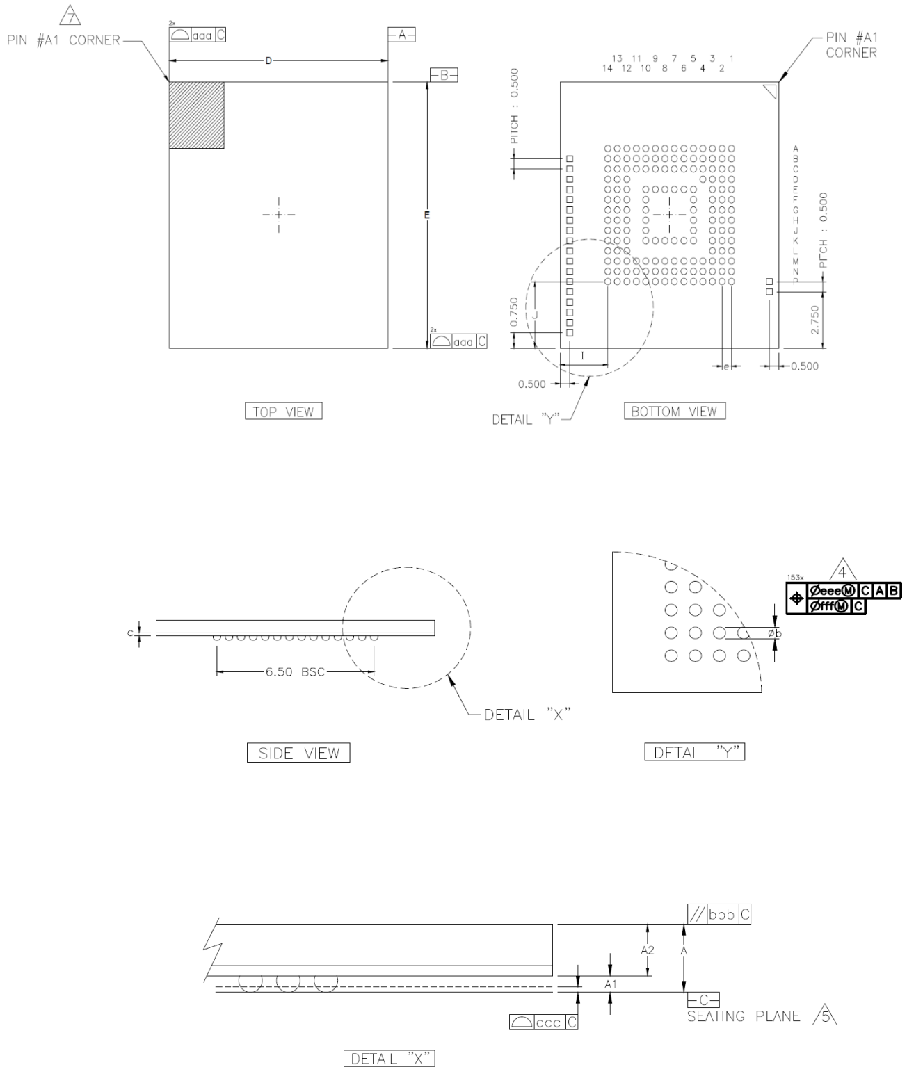
Figure 1. 11.5 x 13.0 x 1.0 (mm) Package Dimension
