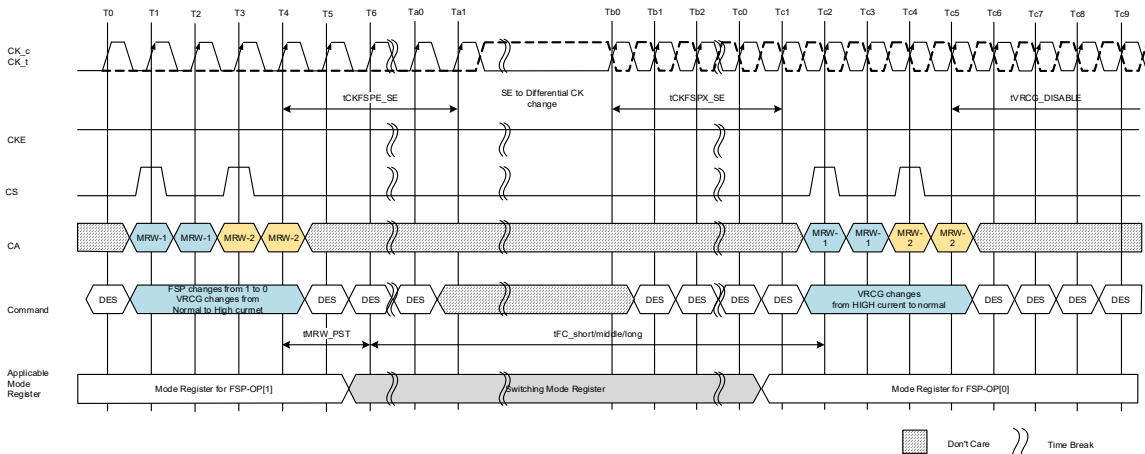
Figure 142 - SE to Differential CK and Write DQS -FSP Switching Timing CKE=High
