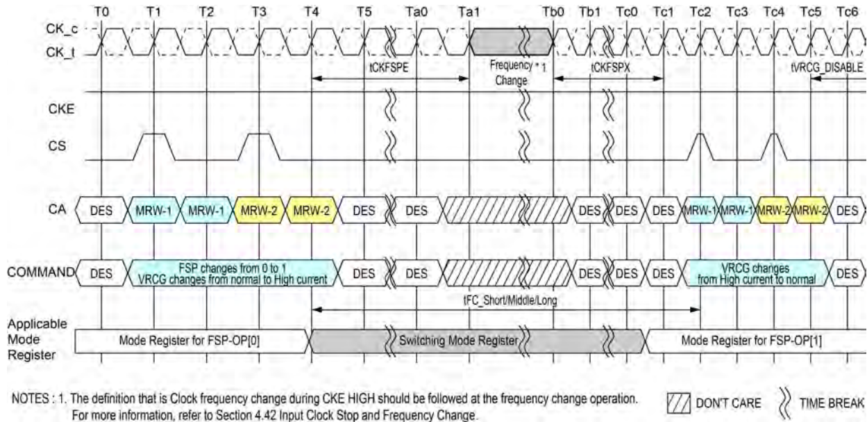
Figure 103 - Frequency Set Point Switching Timing
