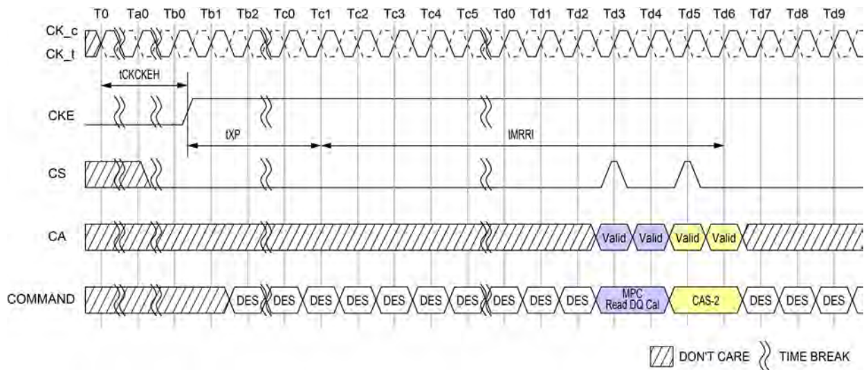
Figure 113 - MPC Read DQ Calibration Following Power-Down State
