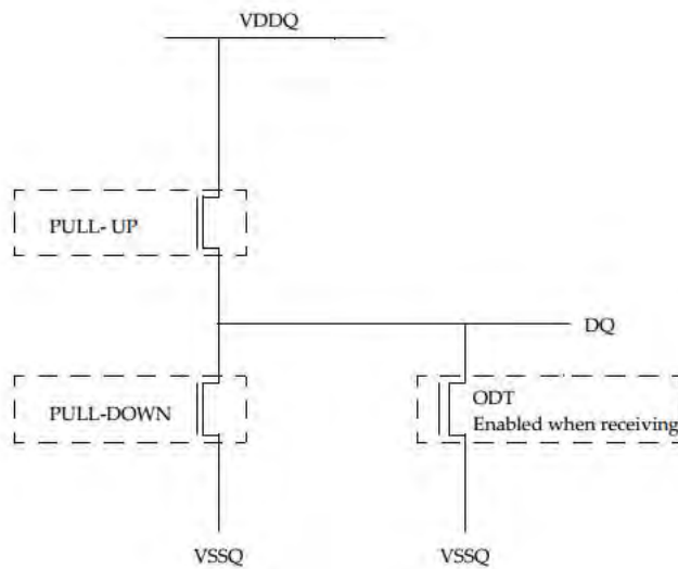
Figure 180 - LVSTL I/O Cell
