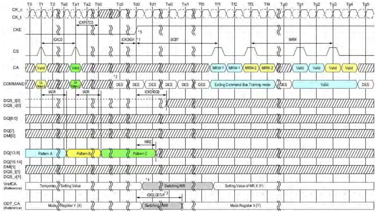
Figure 101 - Exiting Command Bus Training Mode with Valid Command
