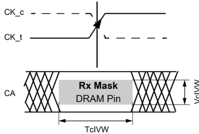
Figure 185 - CA Timing at the DRAM pins
