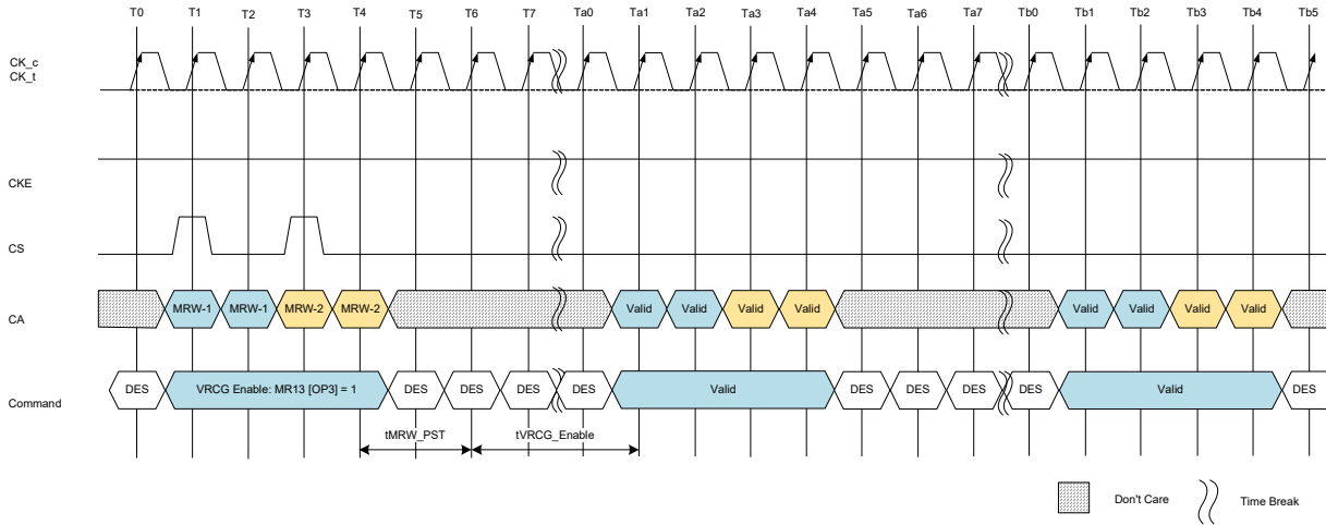
Figure 145 - VRCG status change to high current mode: Single-ended Clock case
