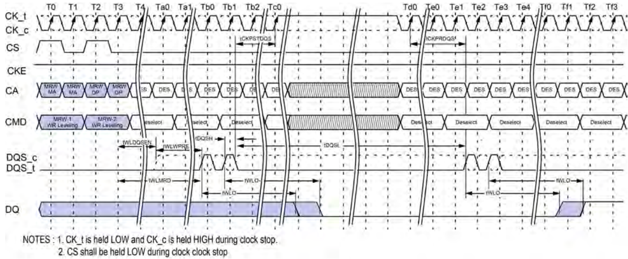
Figure 109 - Clock Stop and Timing during Write Leveling
