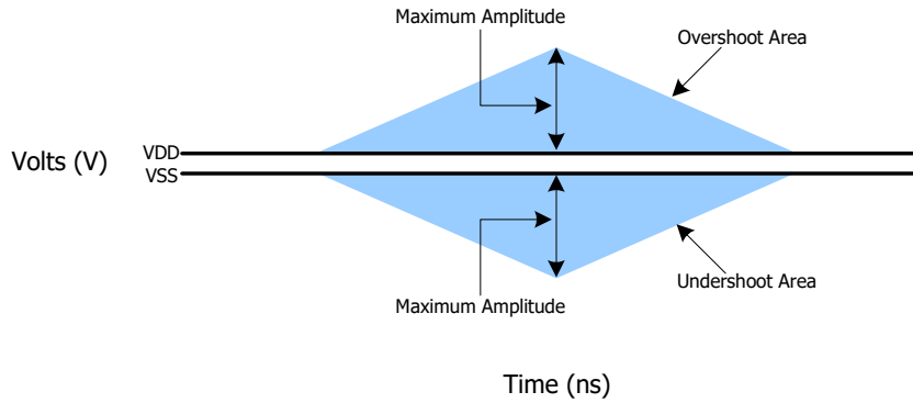
Figure 178 - AC Overshoot and Undershoot Definition
