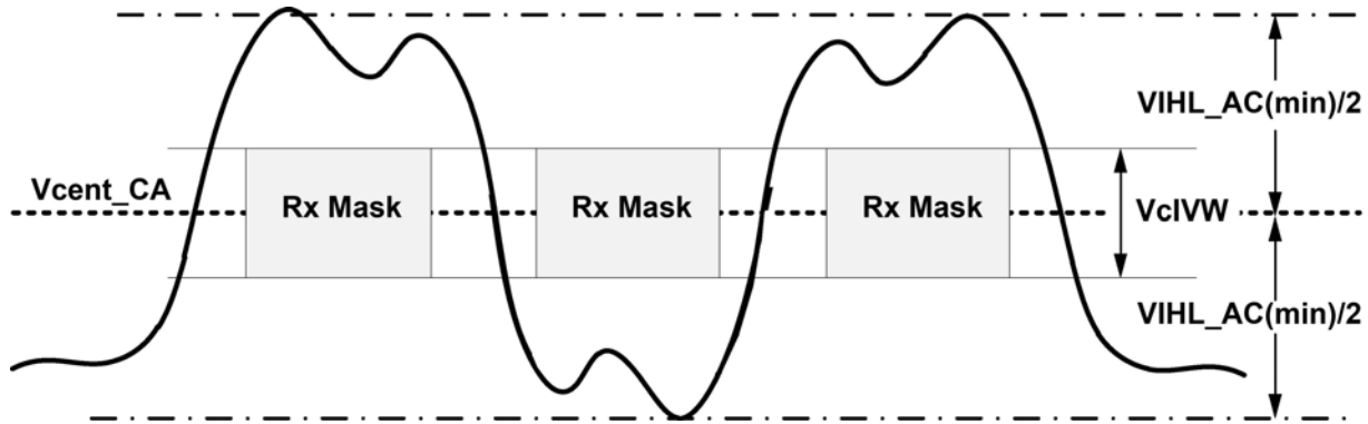
Figure 187 - CA VIHIL_AC definition (for each input pulse)
