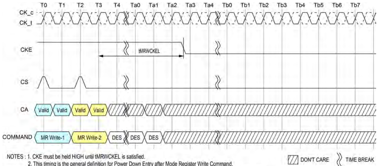
Figure 158 - MRW to Power-Down Entry
