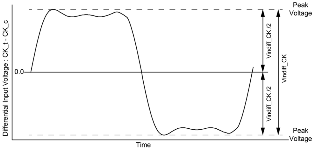
Figure 166 - CK Differential Input Voltage
