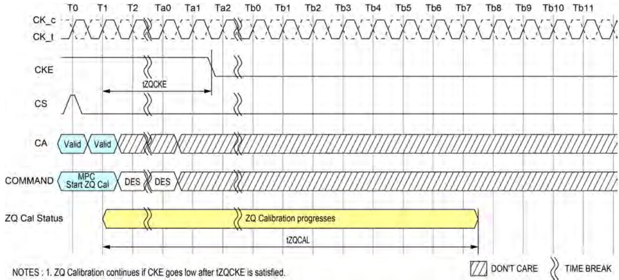
Figure 159 - MPC ZQCAL_start to Power-Down Entry
