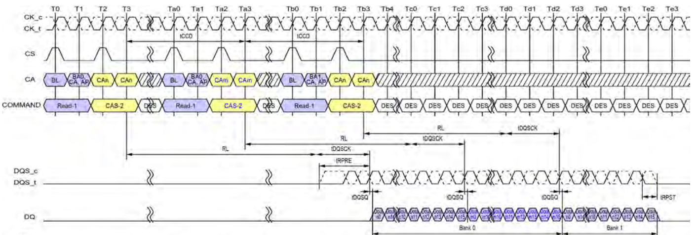
Figure 11 - Seamless Burst Read
