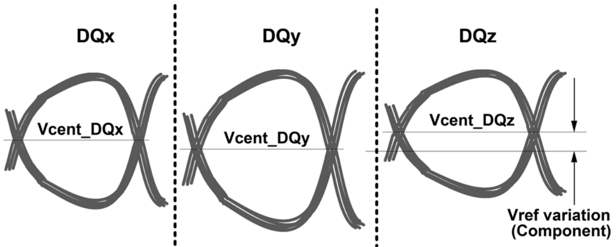
Figure 191 - Across pin V_{ref} DQ voltage variation
