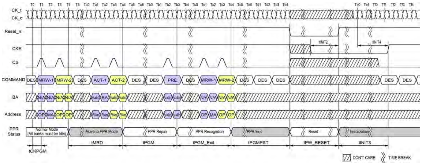
Figure 162 - PPR Timing
