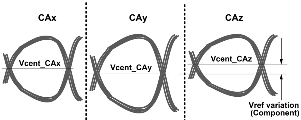
Figure 184 - Across pin Vref CA voltage variation
