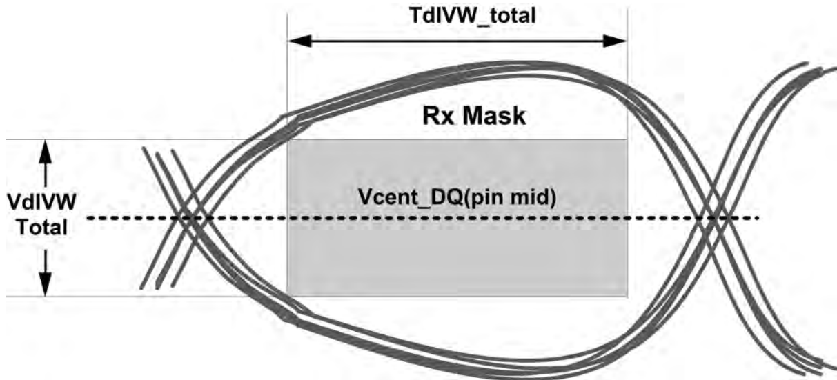
Figure 190 - DQ Receiver(Rx) mask
