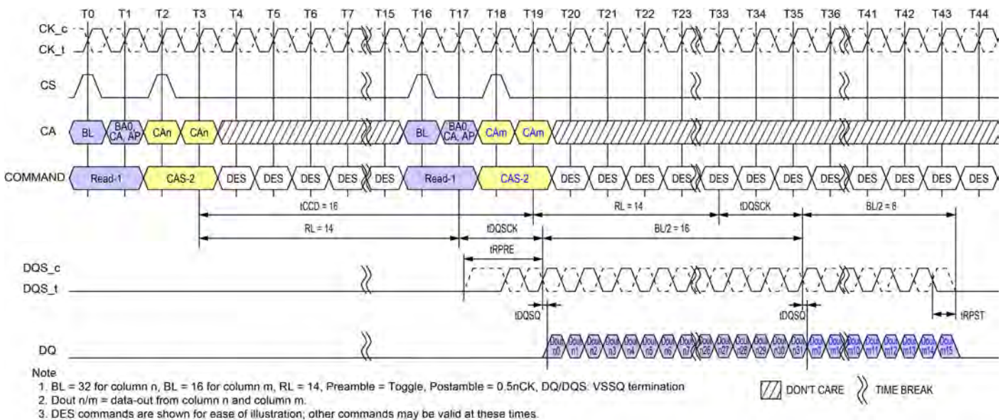
Figure 9 - Burst Read Timing
