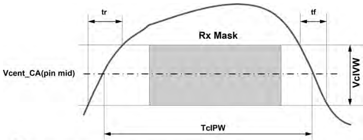
Figure 186 - CA TcIPW and SRIN_cIVW definition (for each input pulse)
