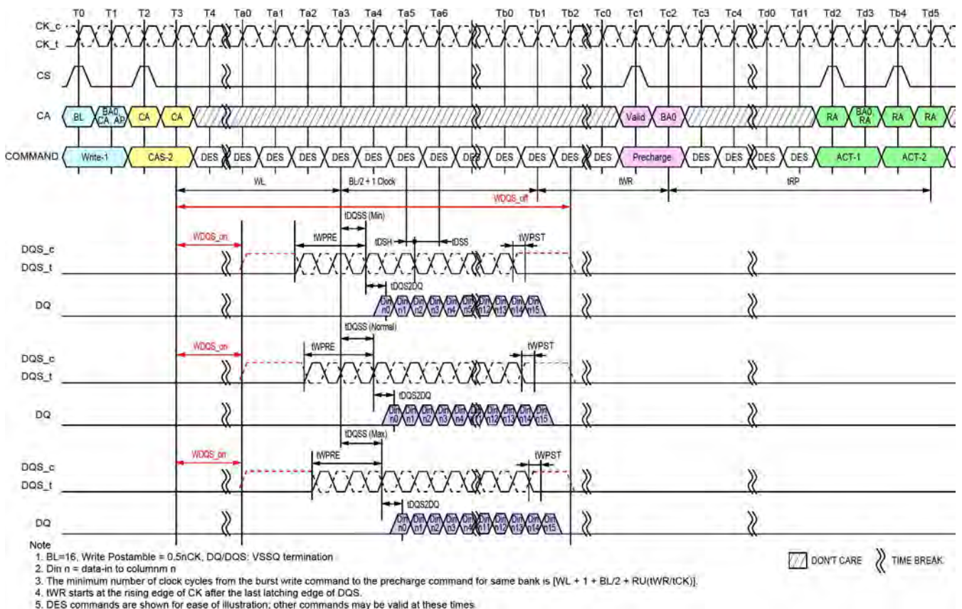
Figure 22 - Burst Write Operation
