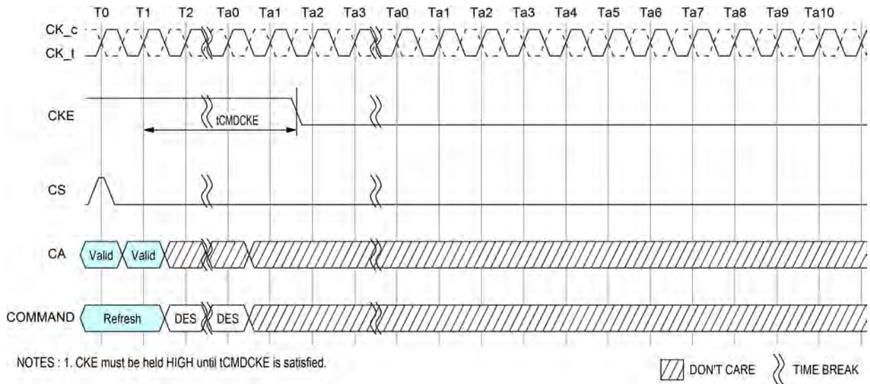
Figure 154 - Refresh entry to Power-Down Entry
