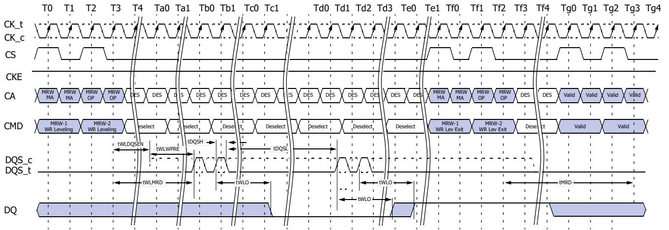
Figure 107 - Write Leveling Timing, tDQSL(max)
