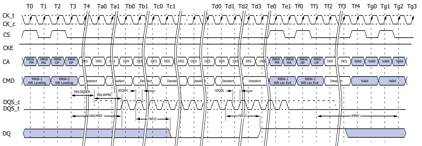
Figure 108 - Write Leveling Timing, tDQSL(min)
