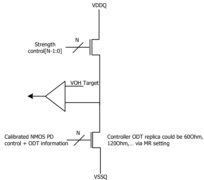
Figure 182 - Pull-up calibration
