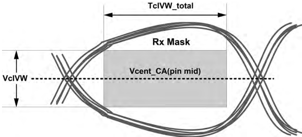
Figure 183 - CA Receiver(Rx) mask
