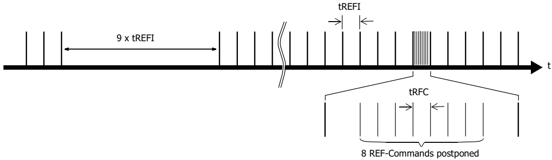
Figure 68 - Postponing Refresh Commands (Example)
