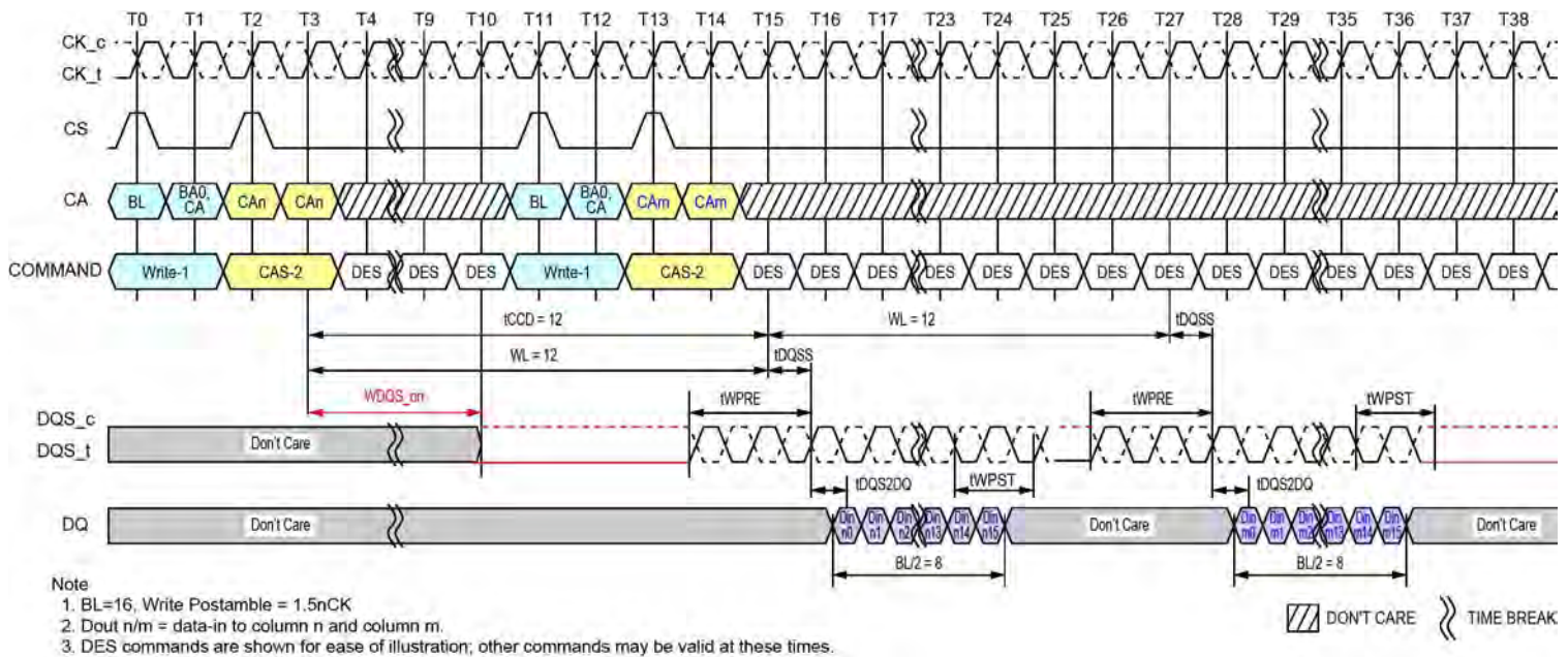
Figure 52 - Consecutive Writes Operation: t_{CCD} = \text{Min} + 4, 1.5n\text{CK} Postamble
