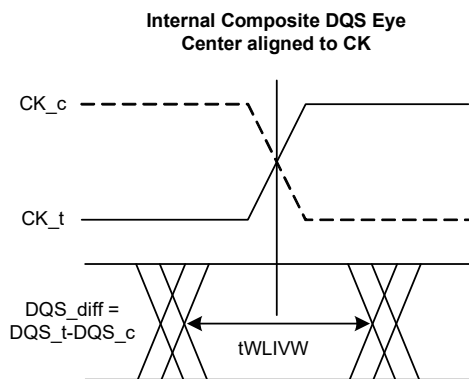
Figure 110 - DQS t /DQS c and CK t /CK c at DRAM Latch
