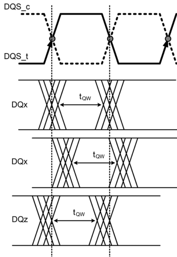
Figure 189 - Read data timing t_{QW} valid window defined per DQ signal
