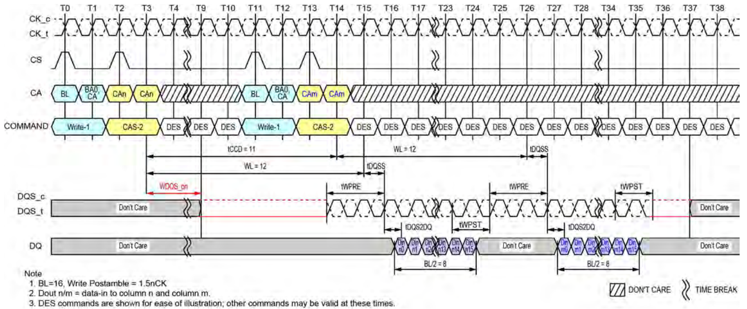
Figure 51 - Consecutive Writes Operation: t_{CCD} = \text{Min} + 3, 1.5n\text{CK} Postamble
