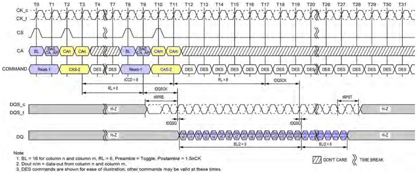
Figure 23 - Burst Write Followed by Burst Read
