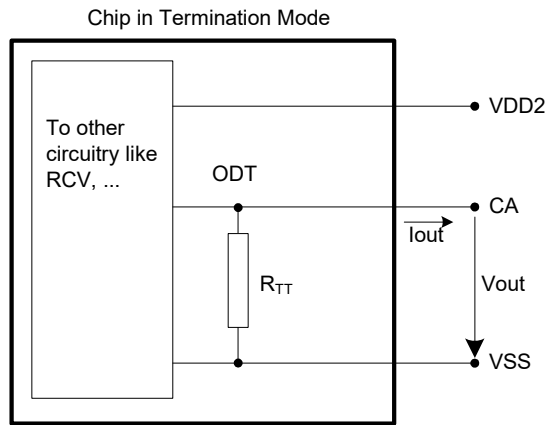
Figure 134 - On Die Termination for CA
