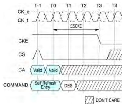
Figure 75 - tESCKE Timing
