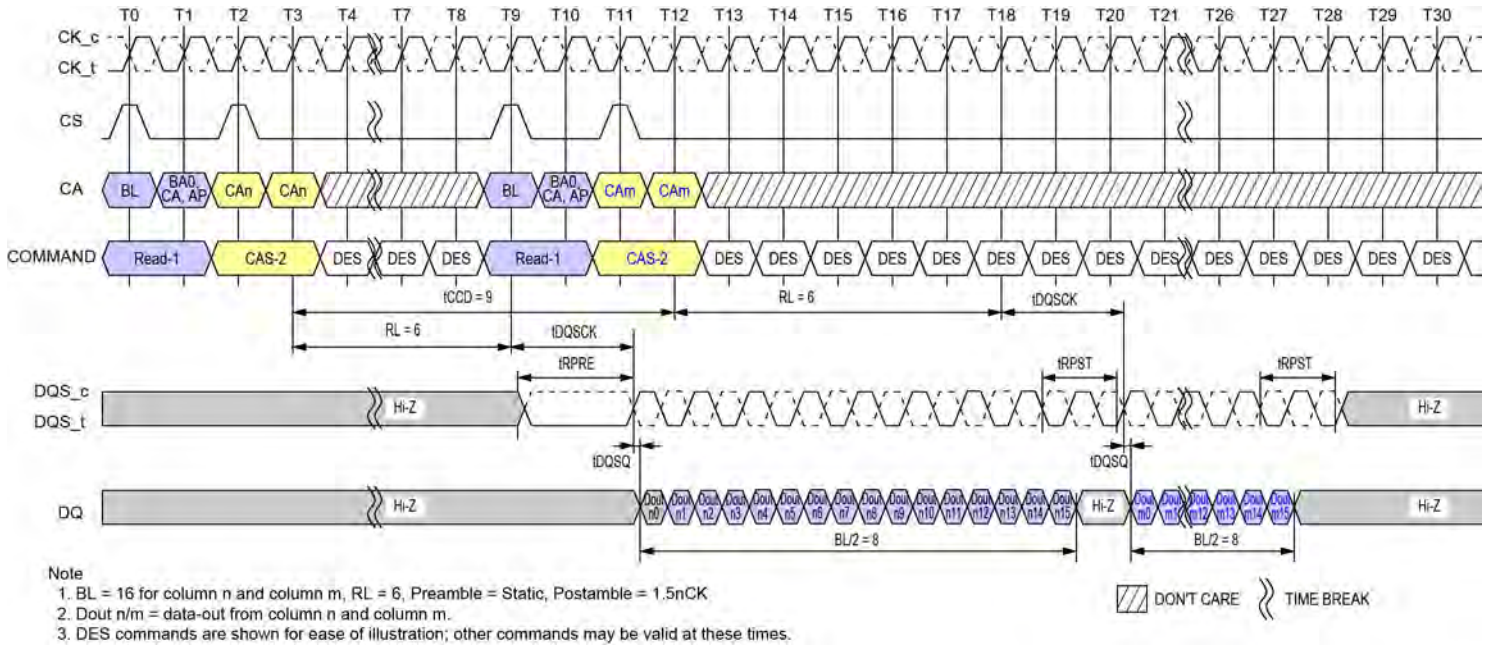
Figure 33 - Consecutive Reads Operation: t_{CCD} = \text{Min} + 1 , Preamble = Static, 1.5nCK Postamble
