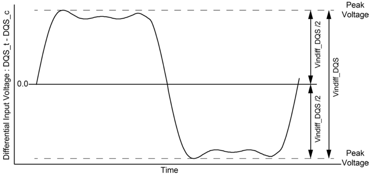
Figure 171 - DQS Differential Input Voltage
