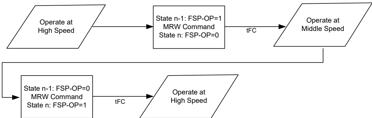
Figure 105 - Switching between two trained Frequency Set Points
