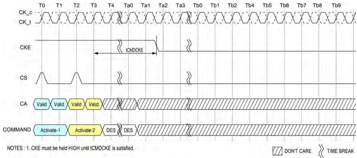
Figure 155 - Activate Command to Power-Down Entry
