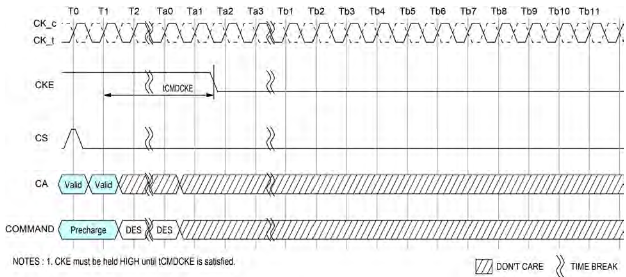
Figure 156 - Precharge Command to Power-Down Entry
