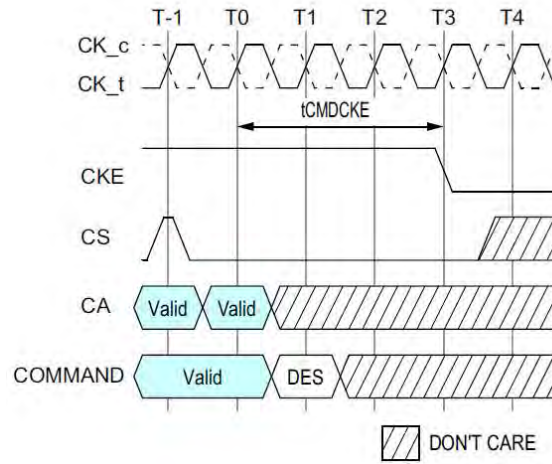
Figure 160 - tCMDCKE Timing
