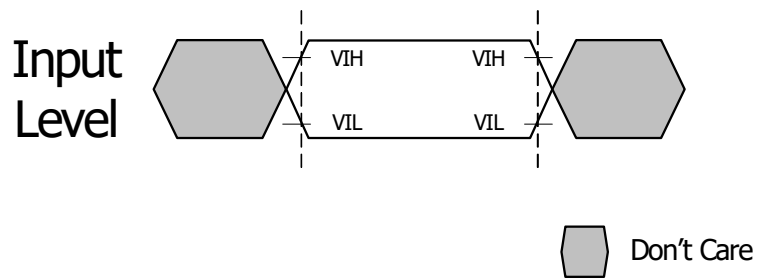
Figure 164 - Input AC timing definition
