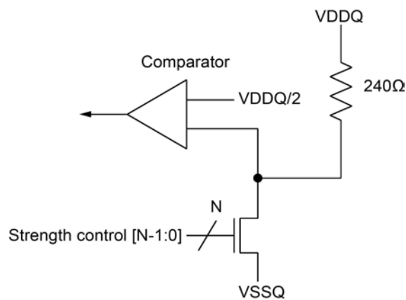
Figure 181 - Pull-down calibration
