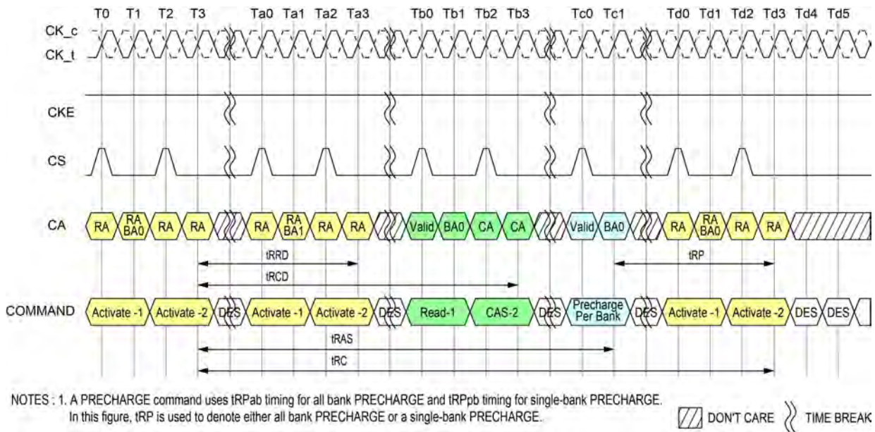
Figure 5 - Activate Command
