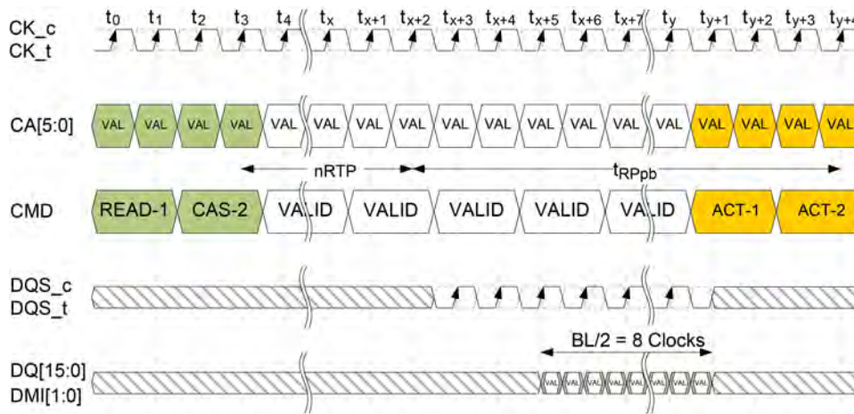
Figure 61 - Burst Read with Auto-Precharge (Shown with BL16, 2tCK preamble)
