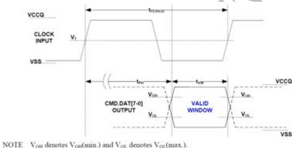
Figure 5-3-5 HS200 Device Output Timing
