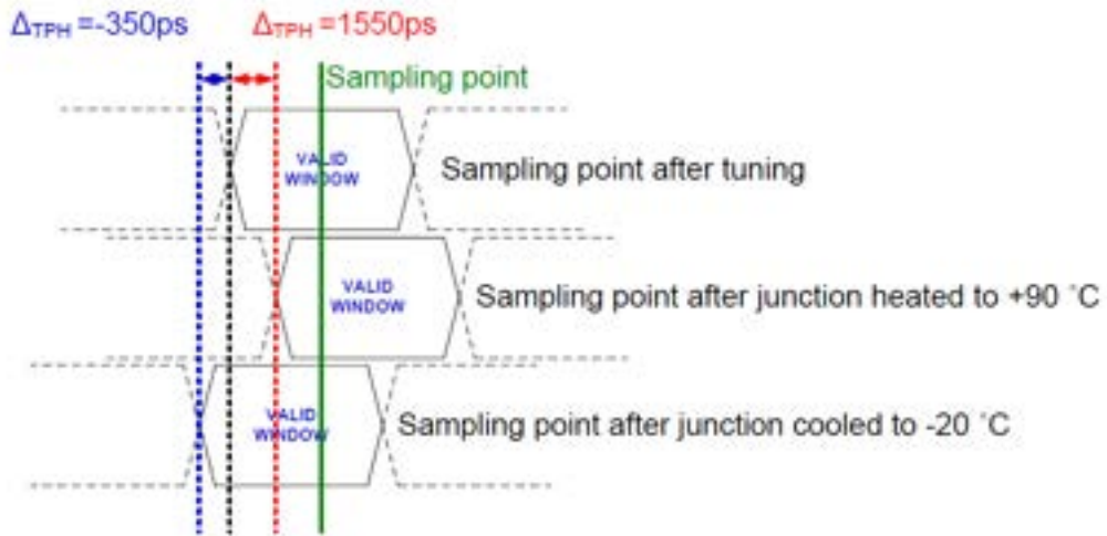
Figure 5-3-7 HS400 Device Input Timing
