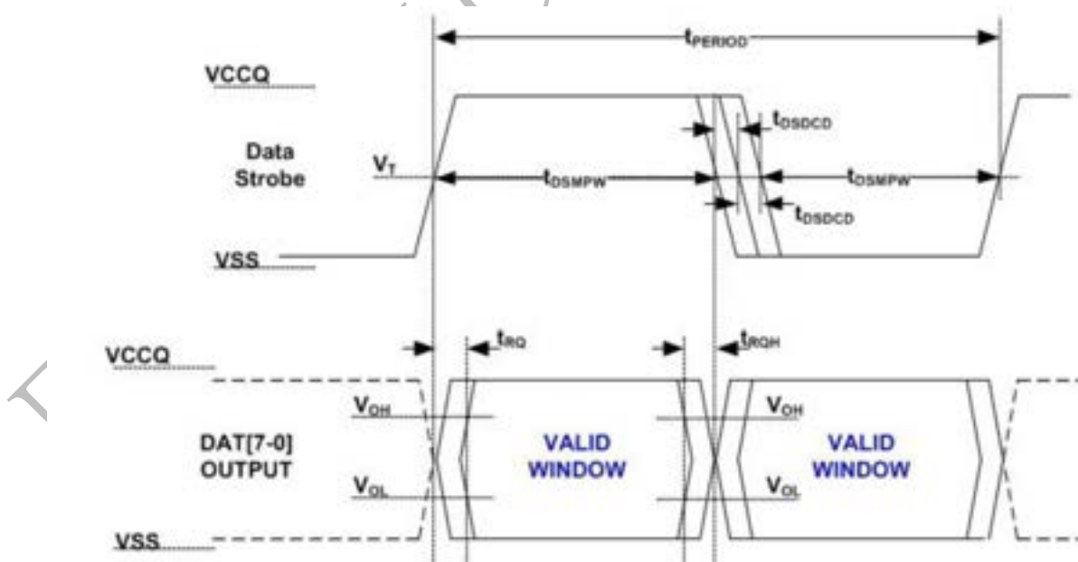
Figure 5-3-8 HS400 Device Output Timing
