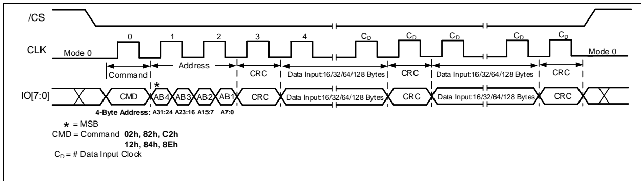
Figure 19-4h. CRC-In-Transit 8d-8d-8d Page Program Command Protocol (ODDR Mode) A 32-Bit Address is required when the device is operating in ODDR Mode
