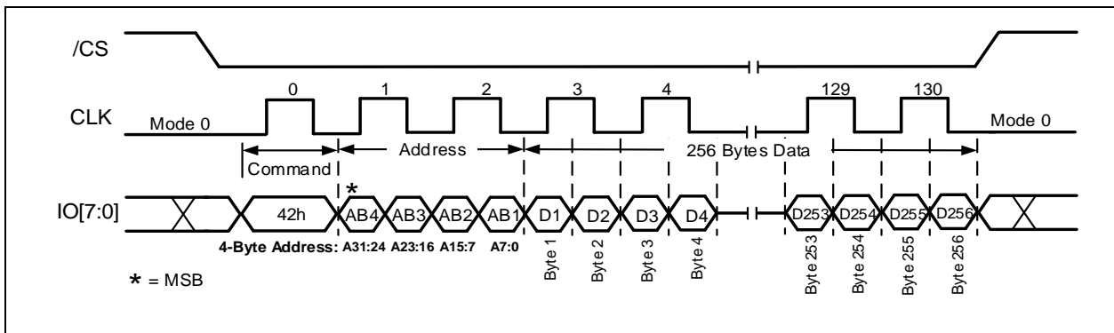
Figure 15-3b. Program Security Registers Command (ODDR Mode) A 32-Bit Address is required when the device is operating in ODDR mode
