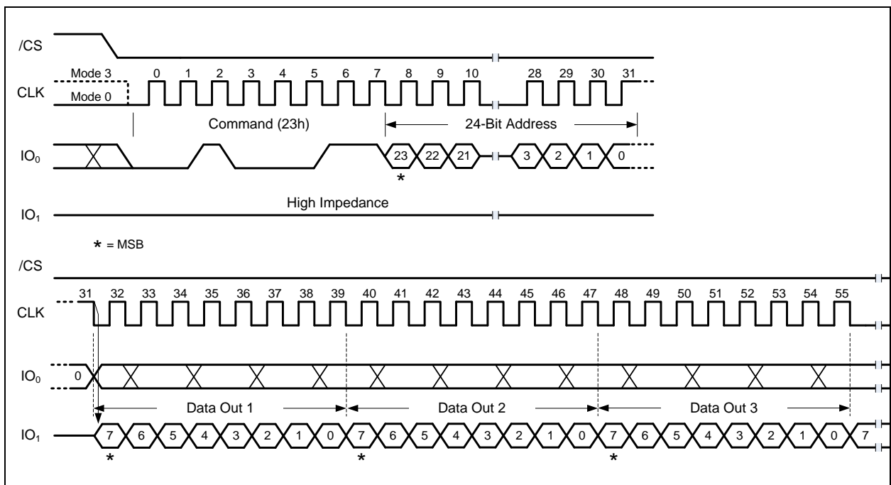
Figure 18-1. (1-1-1) Read DLP Command (1-1-1 SDR Mode) A 32-Bit Address is required when the device is operating in 4-Byte Address Mode
