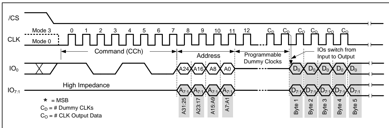
Figure 10-8. Fast Read Octal I/O Command with 4-Byte Address (1-8-8 SDR)
