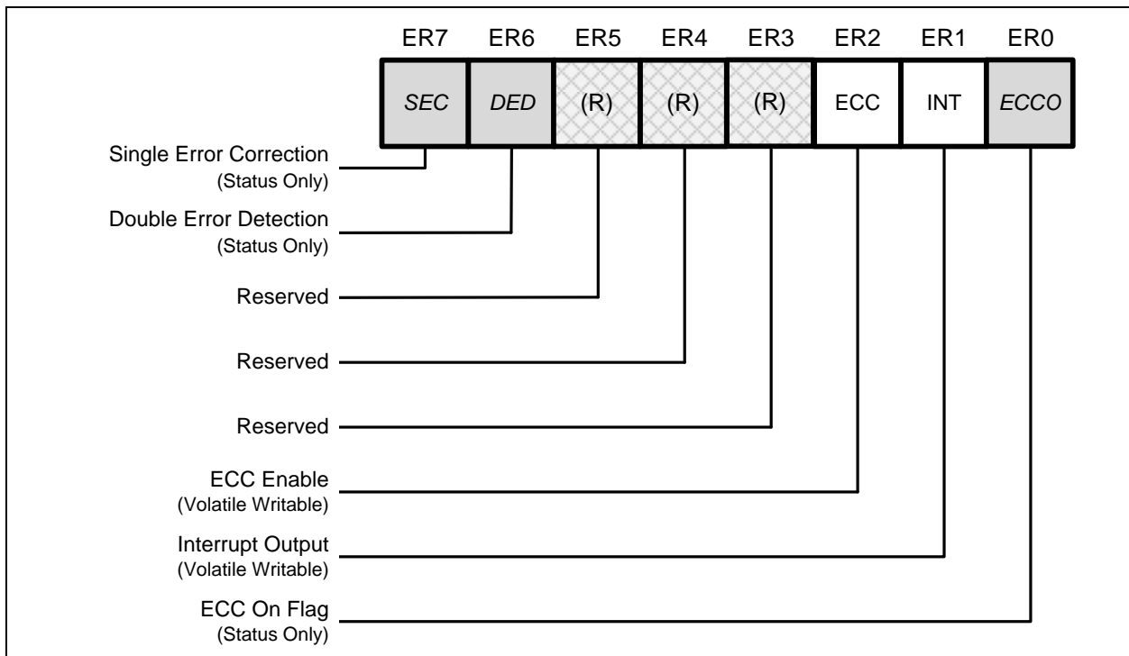
Figure 5-4. ECC Status Register
