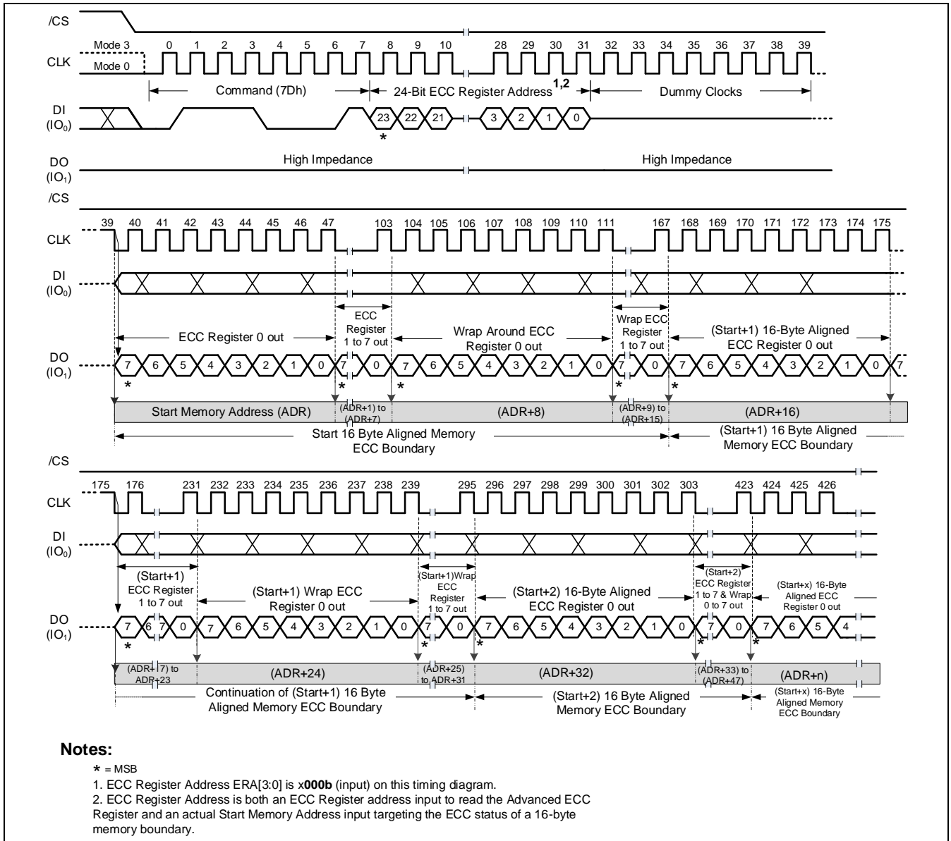
Figure 17-4a. Read Advanced ECC Status Register Command (SDR Mode) A 32-Bit Addressing is required when the device is operating in the 4-Byte Address Mode
