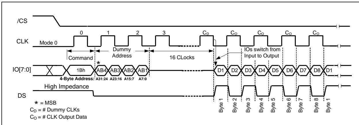
Figure 19-3b. ODDR Read 8-Byte CRC Code Command Sequence (ODDR Mode) A 32-Bit Address is required when the device is operating in ODDR Mode
