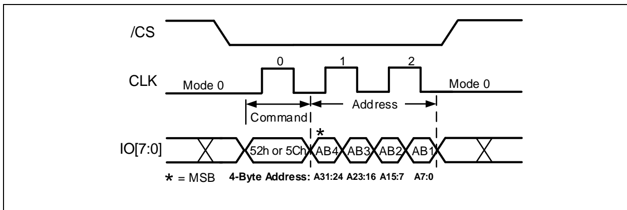
Figure 12-6. 32KB Block Erase Command (ODDR Mode) A 32-Bit Address is required when the device is operating in ODDR mode
