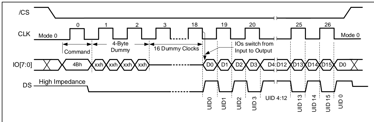
Figure 15-1b. Read Unique ID Command (ODDR Mode) A 32-Bit Dummy Input is required when the device is operating in ODDR mode
