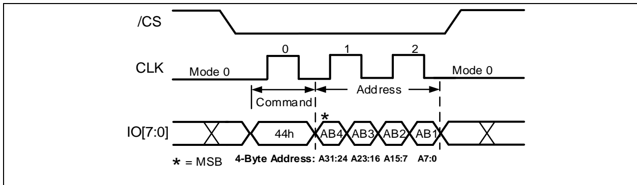
Figure 15-2b. Erase Security Registers Command (ODDR Mode) A 32-Bit Address is required when the device is operating in ODDR mode
