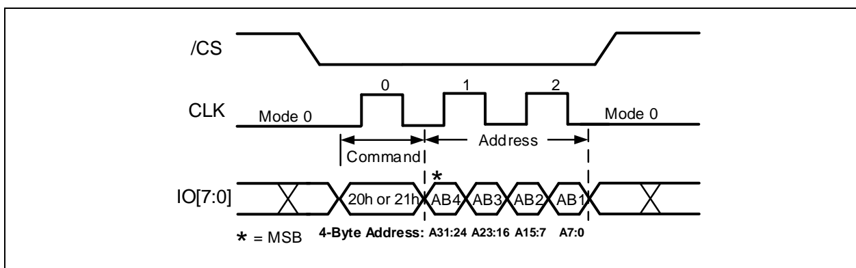
Figure 12-3. Octal DDR Sector Erase Command (ODDR Mode) A 32-Bit Address is required when the device is operating in ODDR mode
