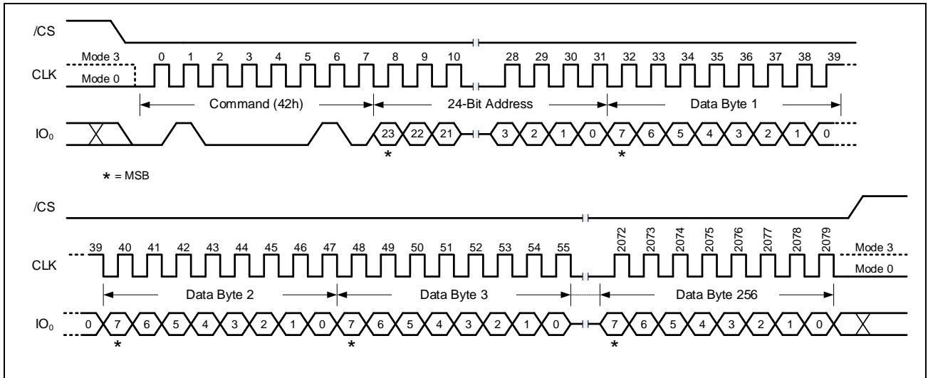
Figure 15-3a. Program Security Registers Command (SDR Mode) A 32-Bit Address is required when the device is operating in 4-Byte Address Mode
