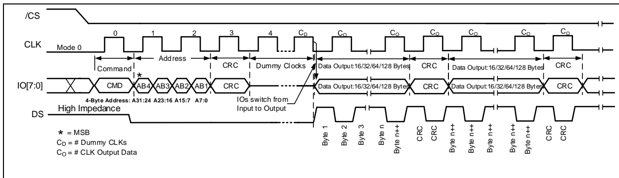
Figure 19-4g. CRC-In-Transit 8d-8d-8d Read SFDP Command Protocol (ODDR Mode) A 32-Bit Address is required when the device is operating in ODDR Mode
