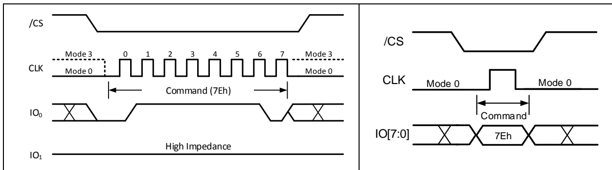
Figure 14-1. Global Block/Sector Lock Command for SDR Mode (left) or ODDR Mode (right)
