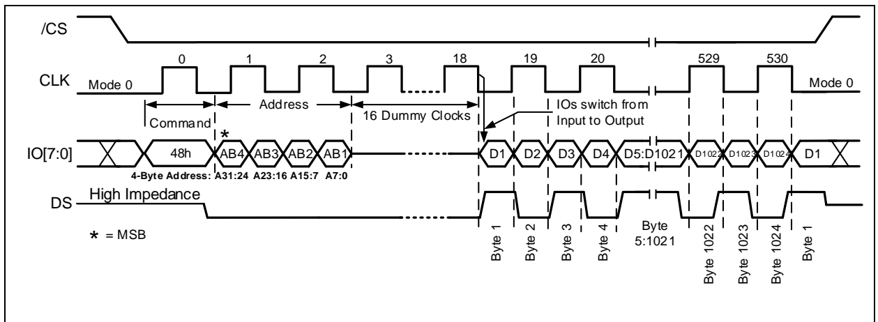
Figure 15-4b. Read Security Registers Command (ODDR Mode) A 32-Bit Address is required when the device is operating in ODDR Mode
