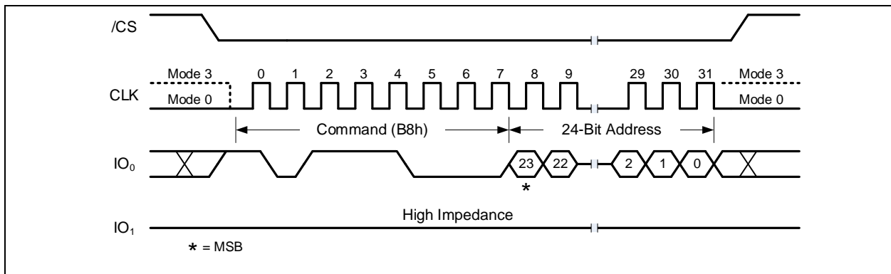
Figure 18-6a. (1-1-0) Erase DLP Register Command (1-1-0 SDR Mode) A 32-Bit Address is required when the device is operating in 4-Byte Address Mode
