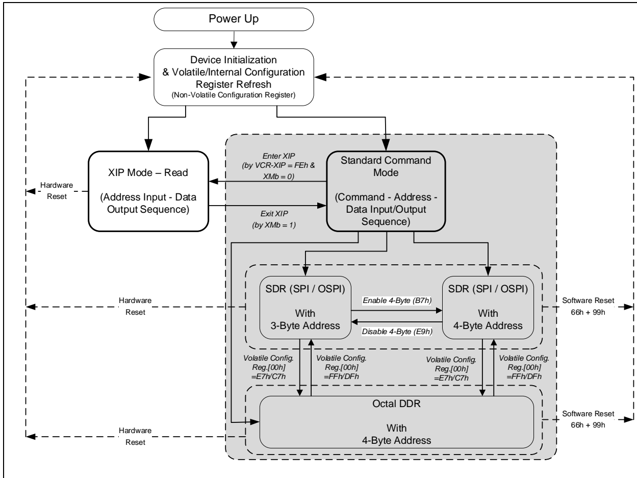
Figure 4-1. W35T25NW Serial Flash Memory Operation Diagram
