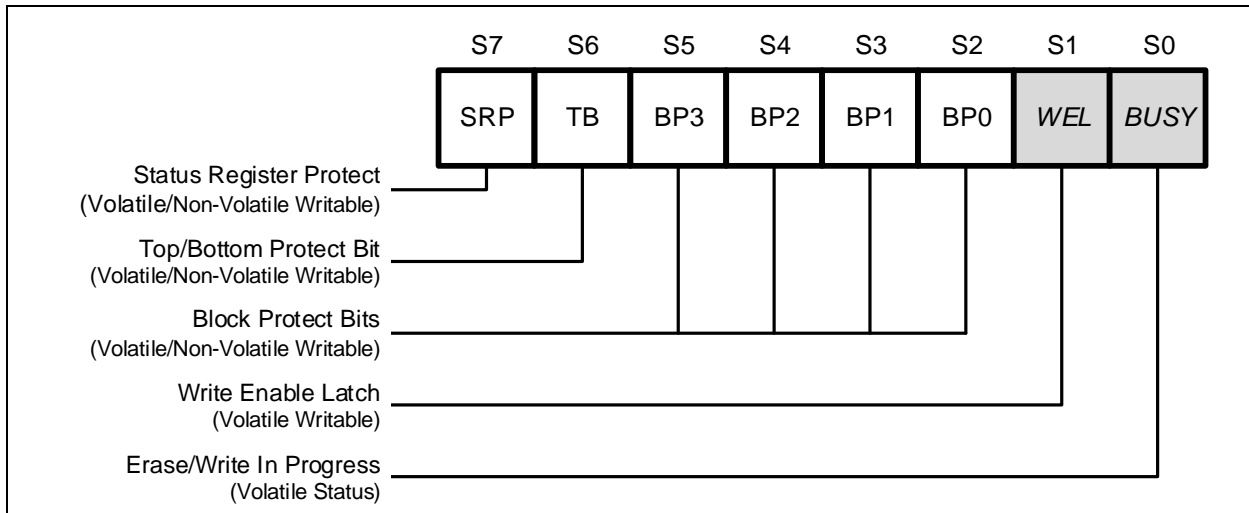
Figure 5-1. Status Register
