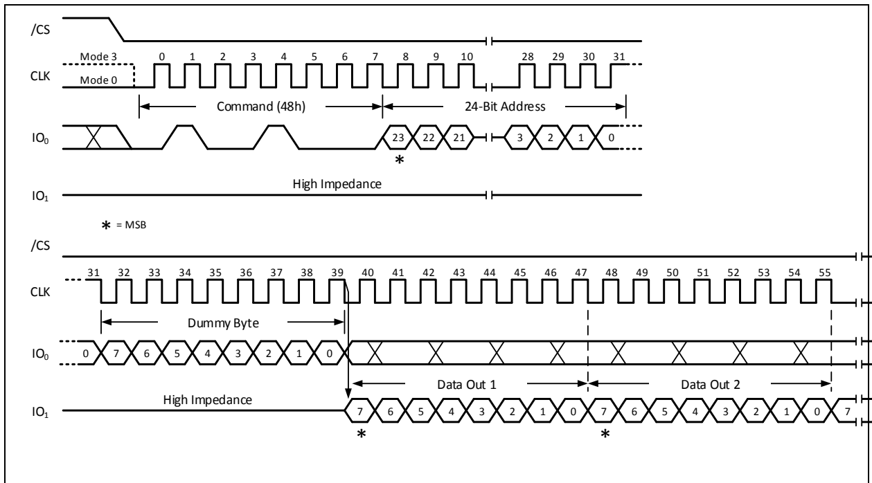
Figure 15-4a. Read Security Registers Command (SDR Mode) A 32-Bit Address is required when the device is operating in 4-Byte Address Mode
