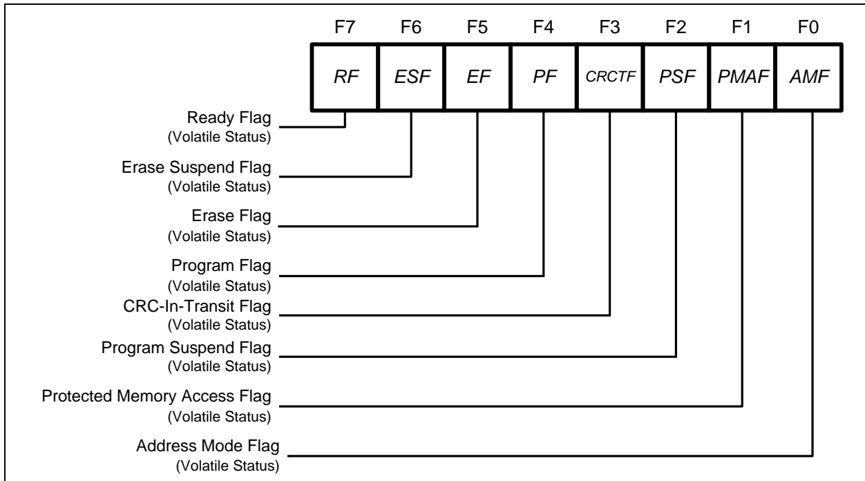
Figure 5-3. Flag Register
