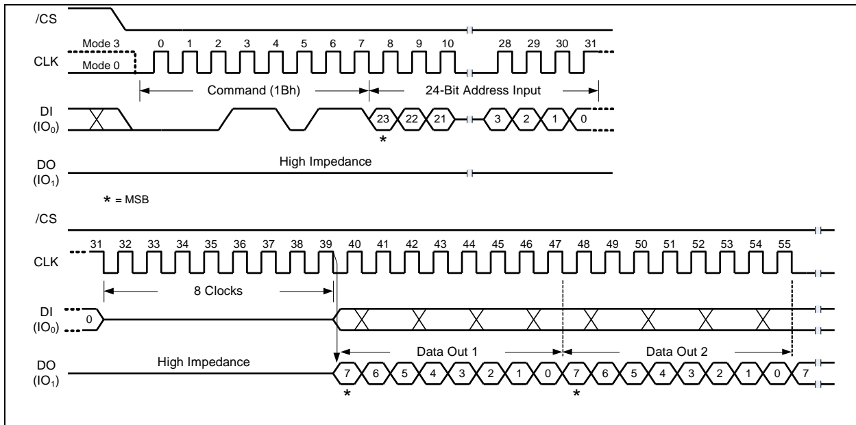
Figure 19-3a. Read 8-Byte CRC Code Command Sequence (1-1-1 SDR Mode) A 32-Bit Address is required when the device is operating in 4-Byte Address Mode
