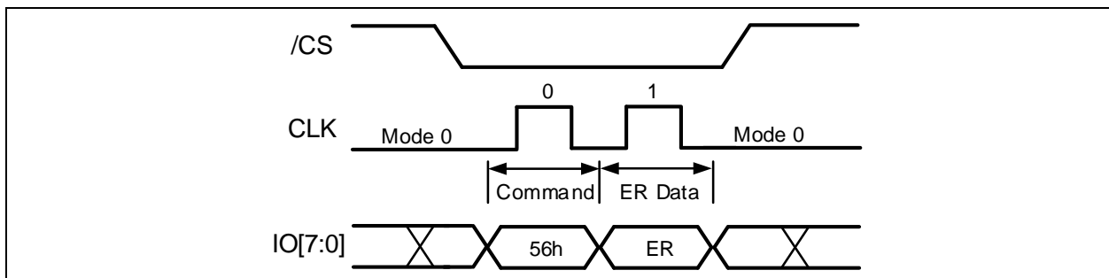
Figure 17-2b. Write ECC Status Register Command (ODDR Mode)
