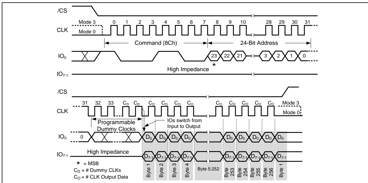
Figure 18-2. (1-1-8) Read DLP Command (1-1-8 SDR Mode) A 32-Bit Address is required when the device is operating in 4-Byte Address Mode
