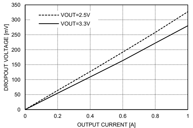
Dropout Voltage
