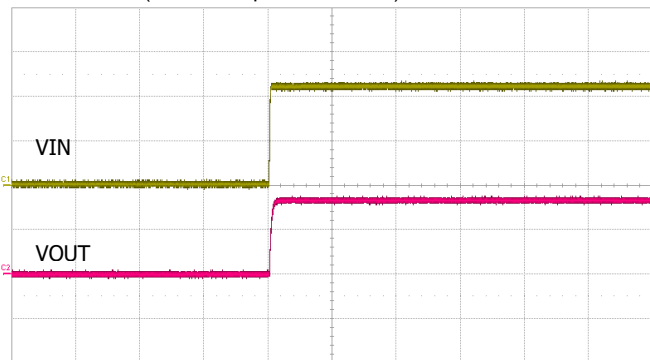
Start Up @ Iout=0A
