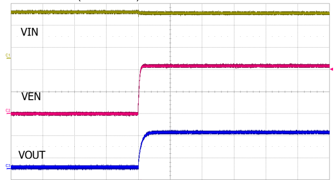
VIN : 2.0V/div, VEN : 2.0V/div, VOUT : 2.0V/div, Time : 5ms/div Start Up by External VEN @ Iout=1A
