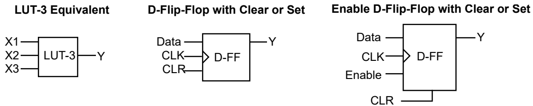
Figure 1-5. VersaTile Configurations
