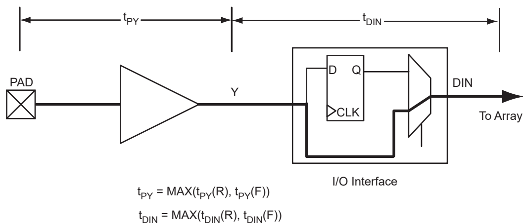
FIGURE 2-3: INPUT BUFFER TIMING MODEL AND DELAYS (EXAMPLE)
