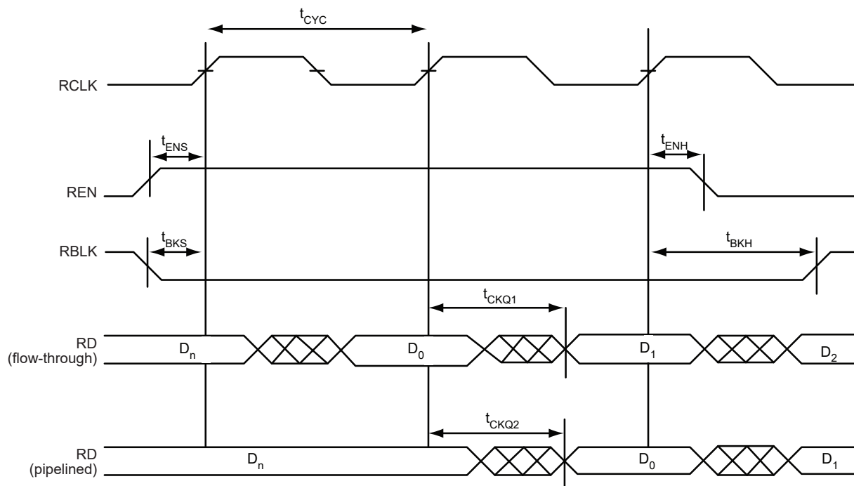
FIGURE 2-47: FIFO READ
