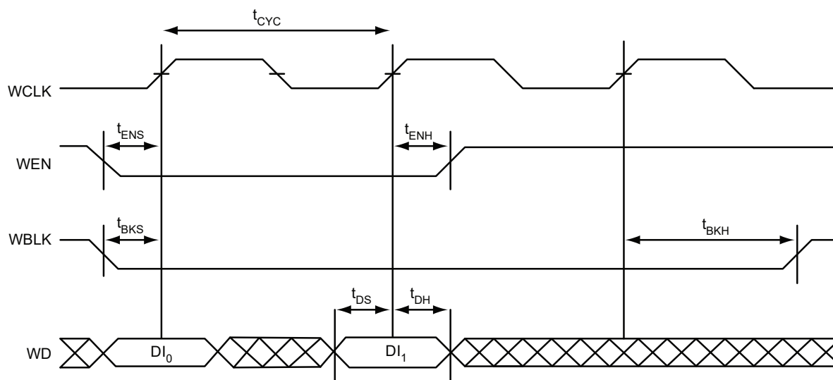
FIGURE 2-48: FIFO WRITE
