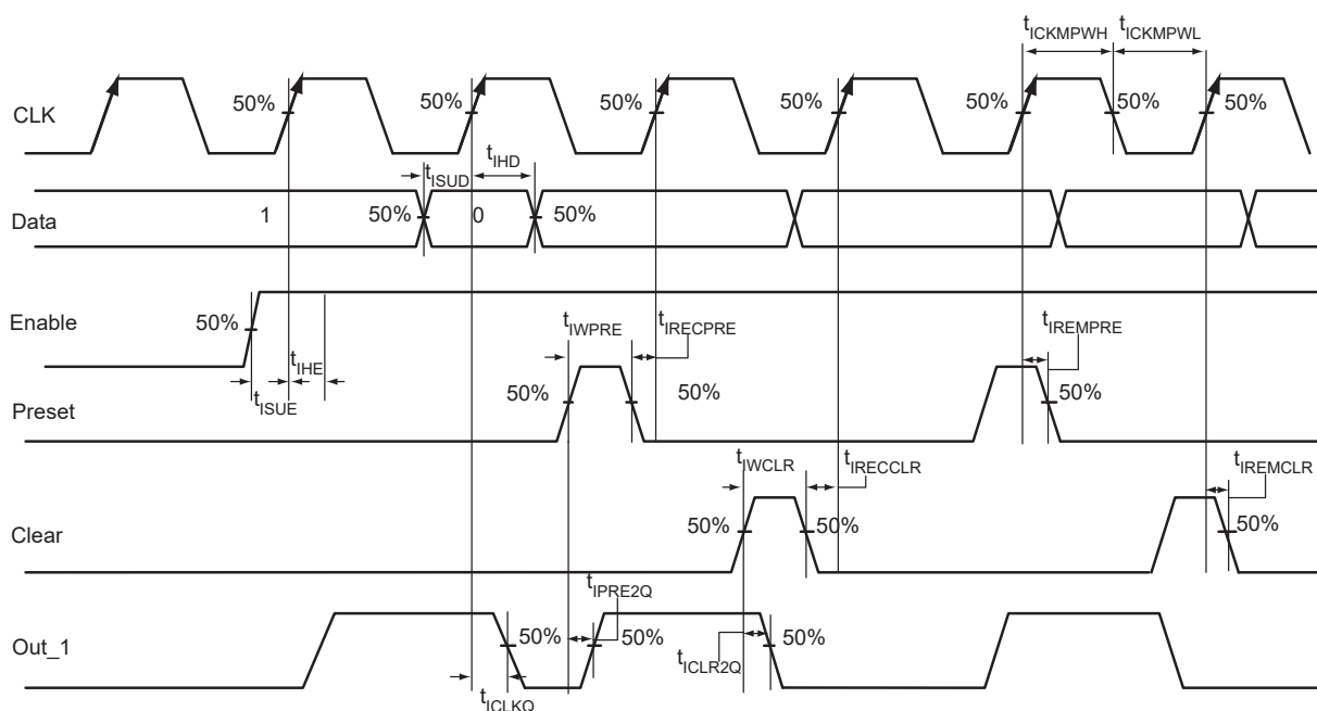
FIGURE 2-27: INPUT REGISTER TIMING DIAGRAM
