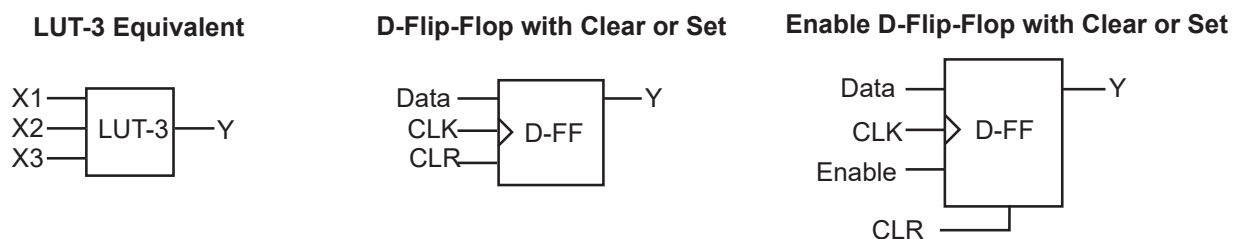
FIGURE 1-2: VERSATILE CONFIGURATIONS
