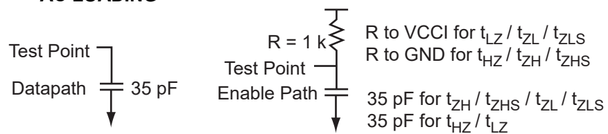
FIGURE 2-6: AC LOADING
