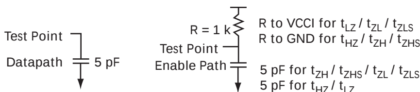
FIGURE 2-8: AC LOADING
