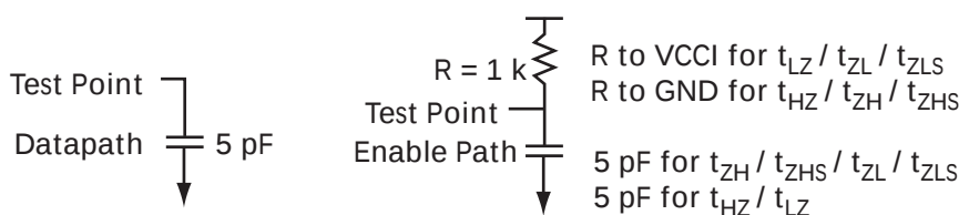
FIGURE 2-10: AC LOADING
