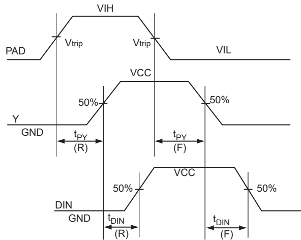
FIGURE 2-5: OUTPUT BUFFER MODEL AND DELAYS (EXAMPLE)
