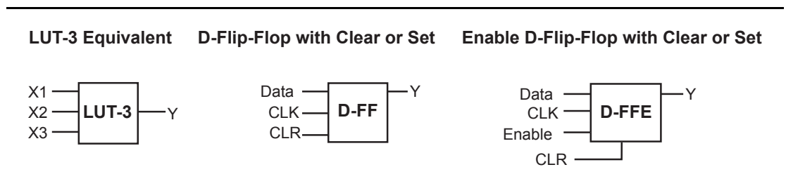
Figure 1-2 • VersaTile Configurations
