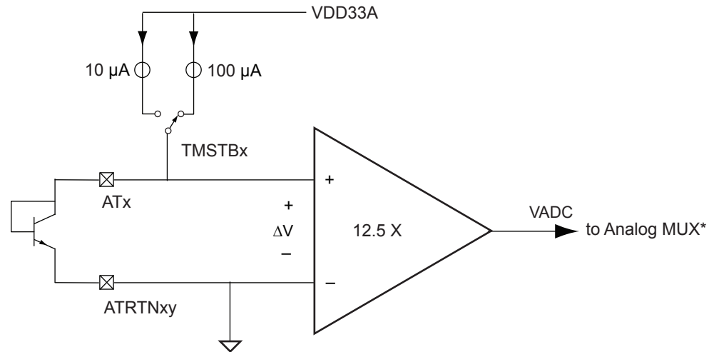
Figure 2-76 • Block Diagram for Temperature Monitor Circuit
