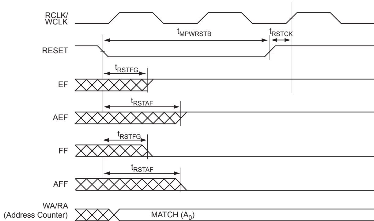
Figure 2-58 • FIFO Reset
