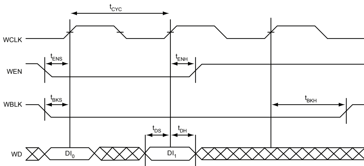
Figure 2-57 • FIFO Write
