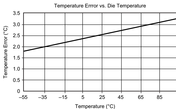
Figure 2-93 • Temperature Error
