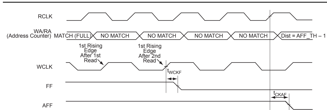
Figure 2-62 • FIFO FULL Flag and AFULL Flag Deassertion
