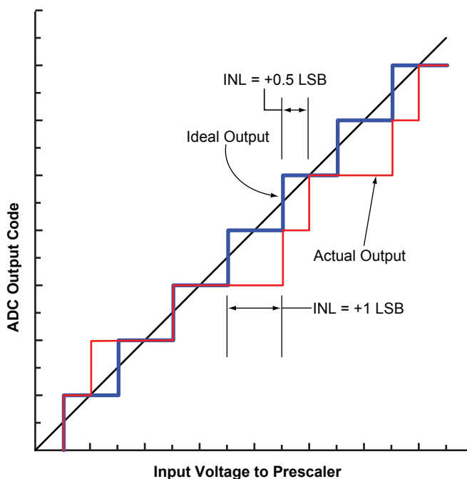
Figure 2-84 • Integral Non-Linearity (INL)
