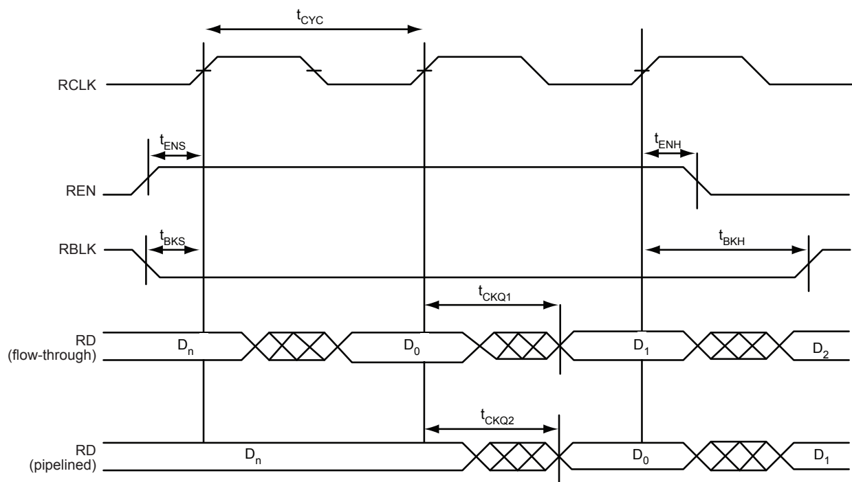
Figure 2-56 • FIFO Read
