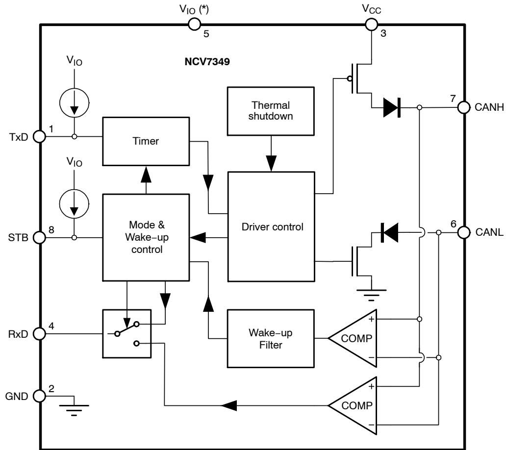
Figure 1. Block Diagram
