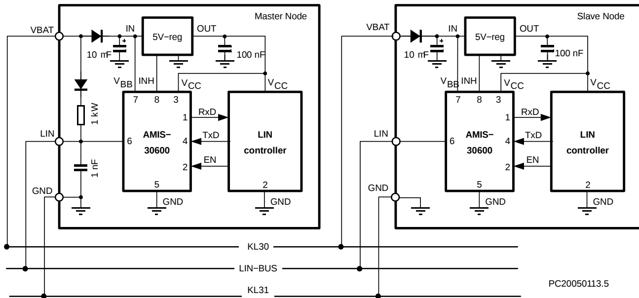
Figure 2. Application Diagram
