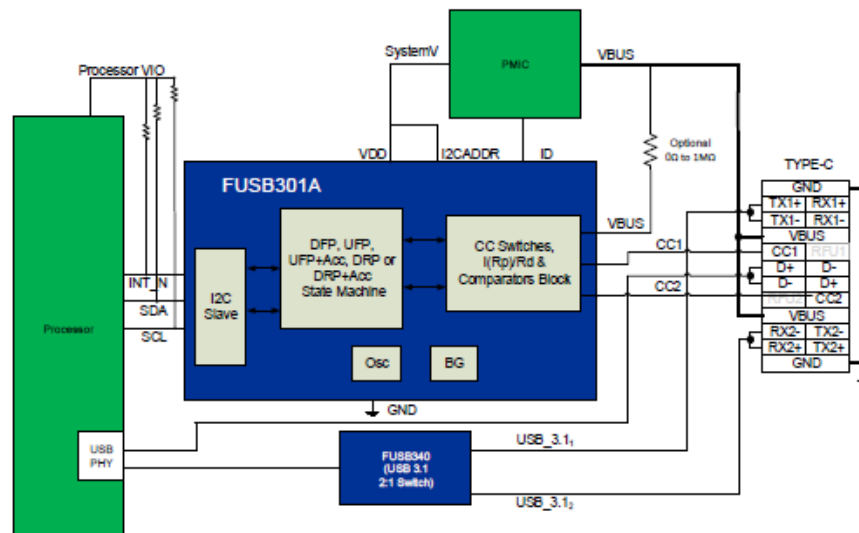
Figure 1. Typical Application
