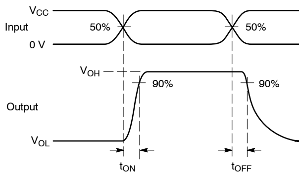
Figure 3. t_{ON}/t_{OFF}
