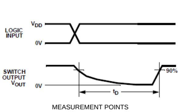
Figure 4. Break-Before-Make Time
