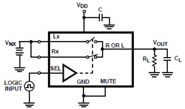
TEST CIRCUIT
