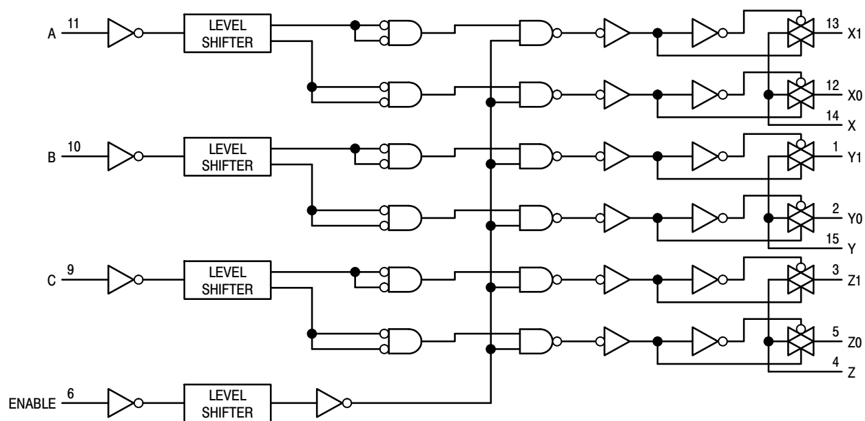
Figure 22. Function Diagram, 4053
